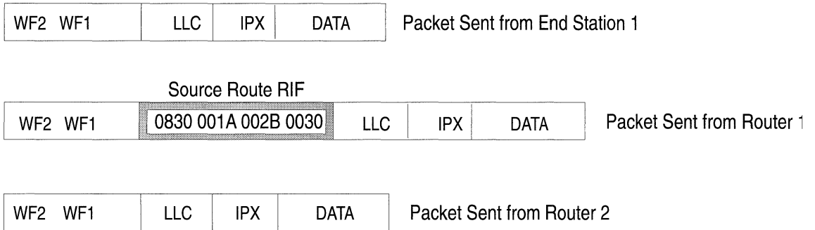
Figure 12-6. IPX Routers Source Routing Across a Token Ring Network
