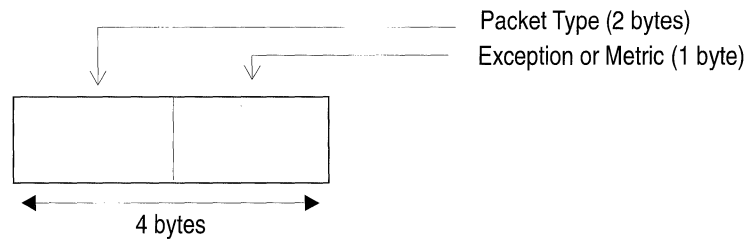
Figure 14-9. VINES Internet Control Protocol Header
