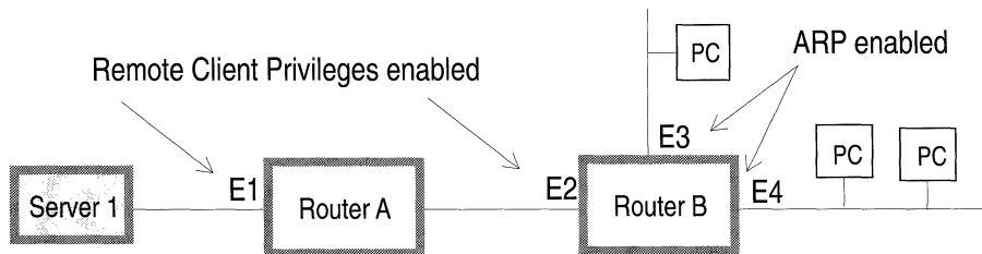
Figure 14-10. VINES Routers Configured on a Serverless Network Segment
