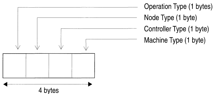
Figure 14-7. VINES Routing Update Protocol Header
