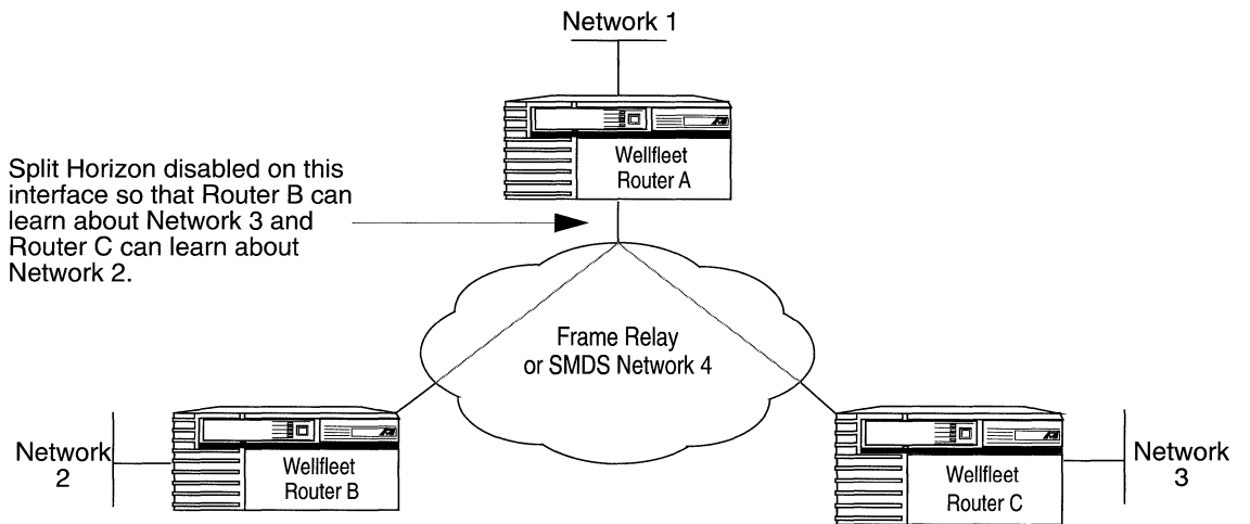
Figure 12-4. Split Horizon Disabled in a Non-Fully Meshed Network
