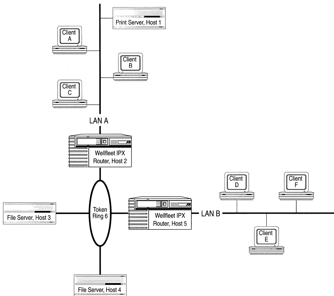
Figure 12-7. Sample IPX Network
