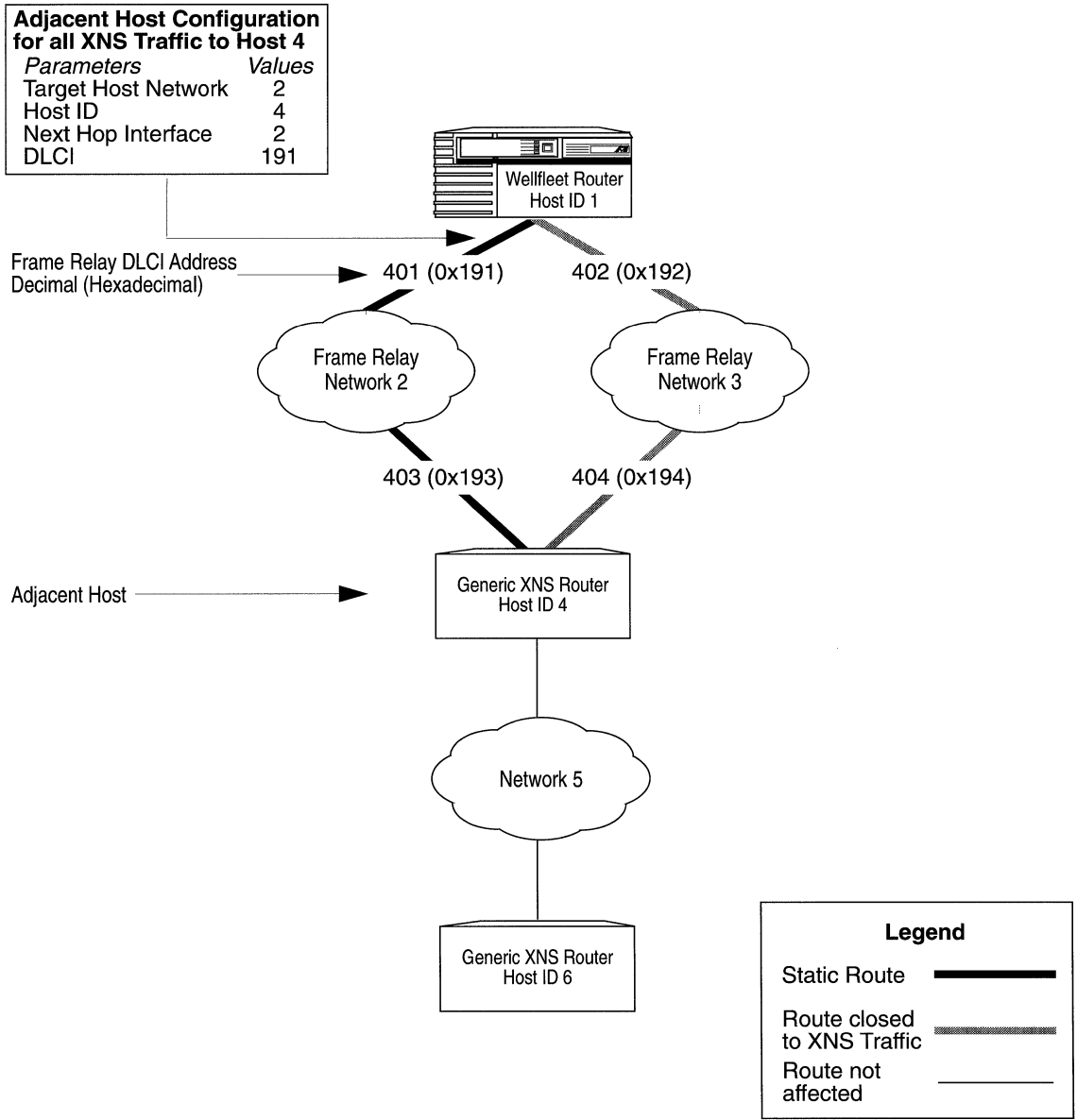
Figure 15-3. Static Adjacent Host in a Sample Network
