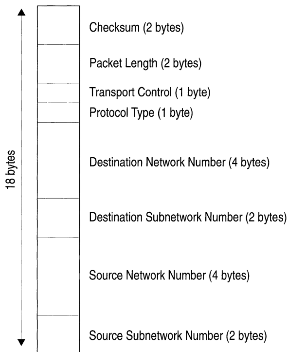
Figure 14-6. VINES Internet Protocol Header
