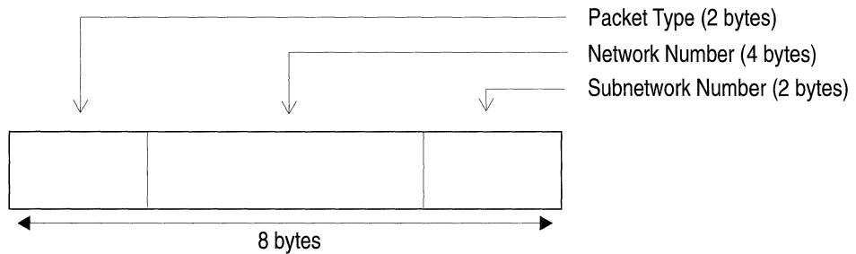
Figure 14-8. VINES Address Resolution Protocol Header
