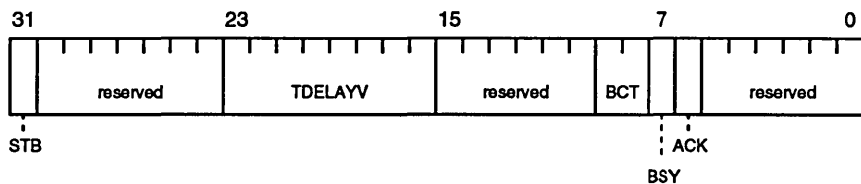
Figure 13-2 Parallel Port Status Register
