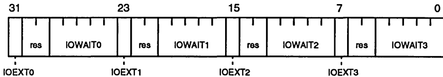
Figure 10-1 PIA Control Register 0 (PICT0, Address 8000020)
