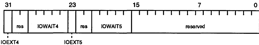
Figure 10-2 PIA Control Register 1 (PICT1, Address 8000024)
