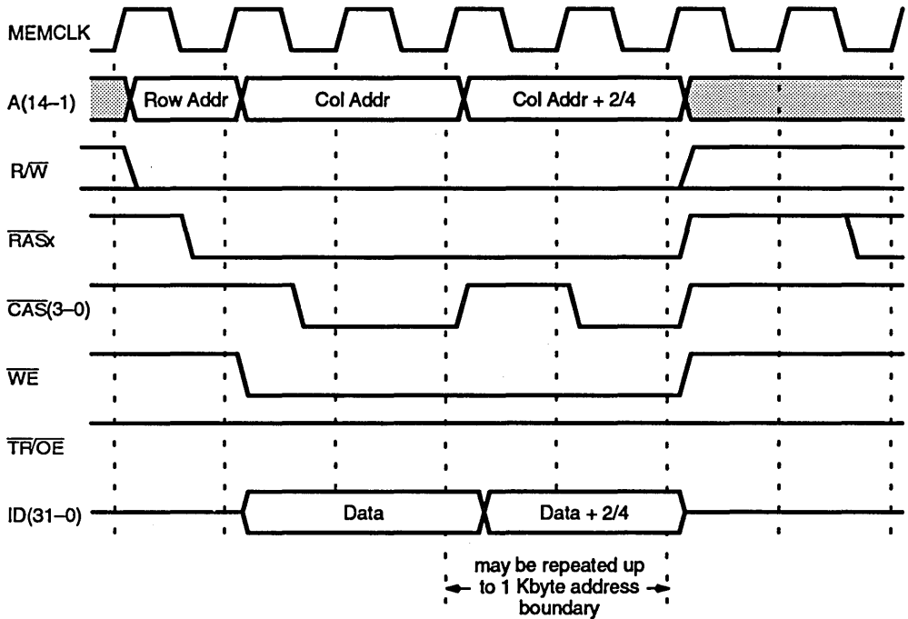
Figure 9-8 DRAM Page-Mode Write Cycle
