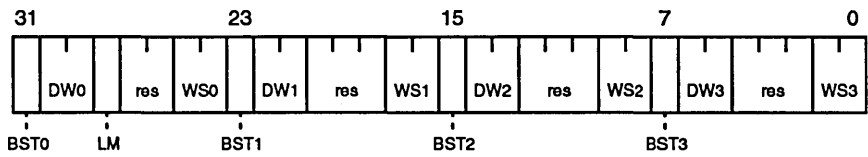
Figure 8-1 ROM Control Register
