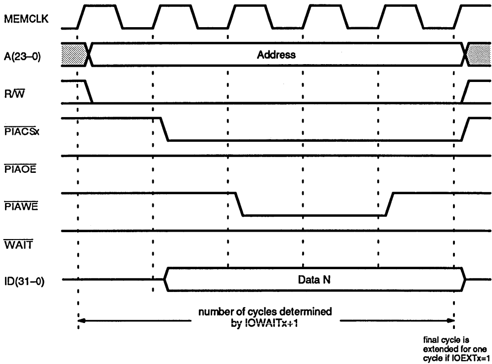
Figure 10-4 PIA Write Cycle
