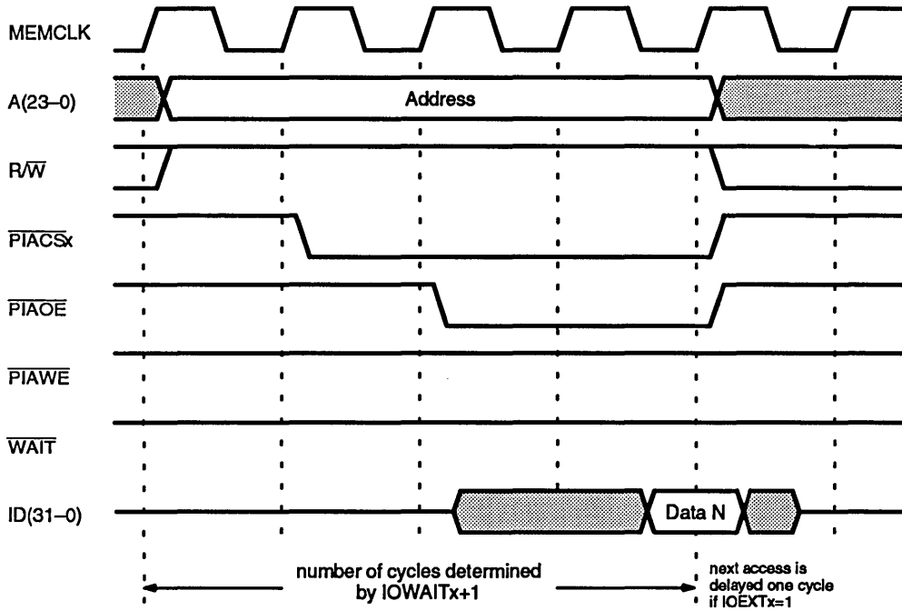
Figure 10-3 PIA Read Cycle
