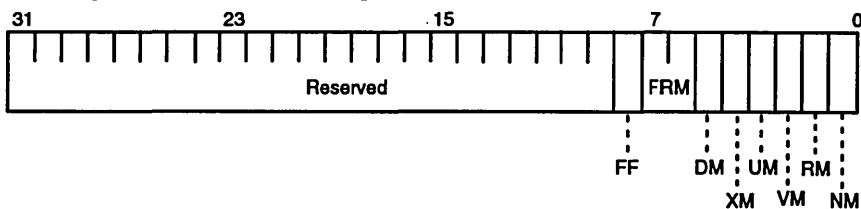
Floating-Point Environment Register
