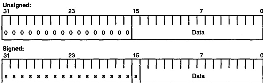
Figure 3-2 Half-Word Format
