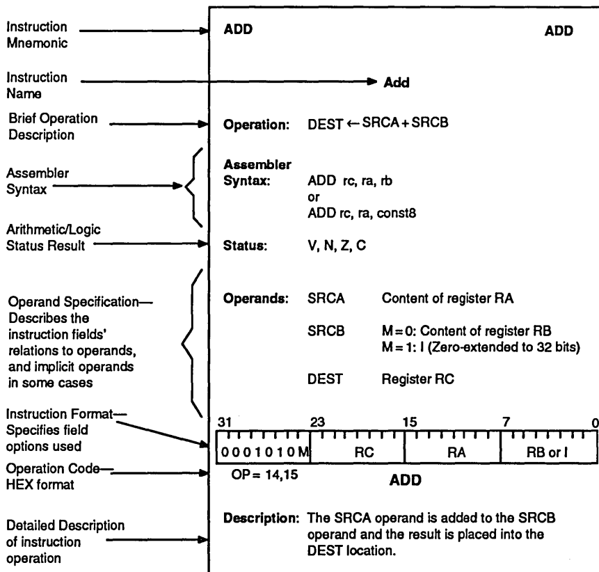
Figure 18-3 Instruction-Description Format
