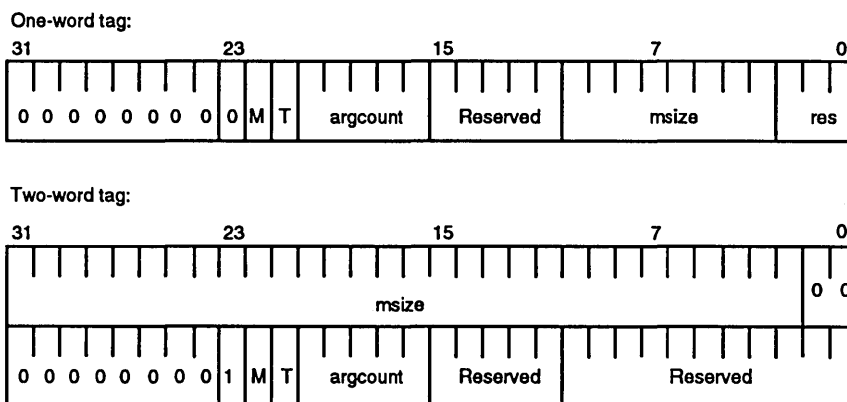
Figure 4-7 Trace-Back Tags
