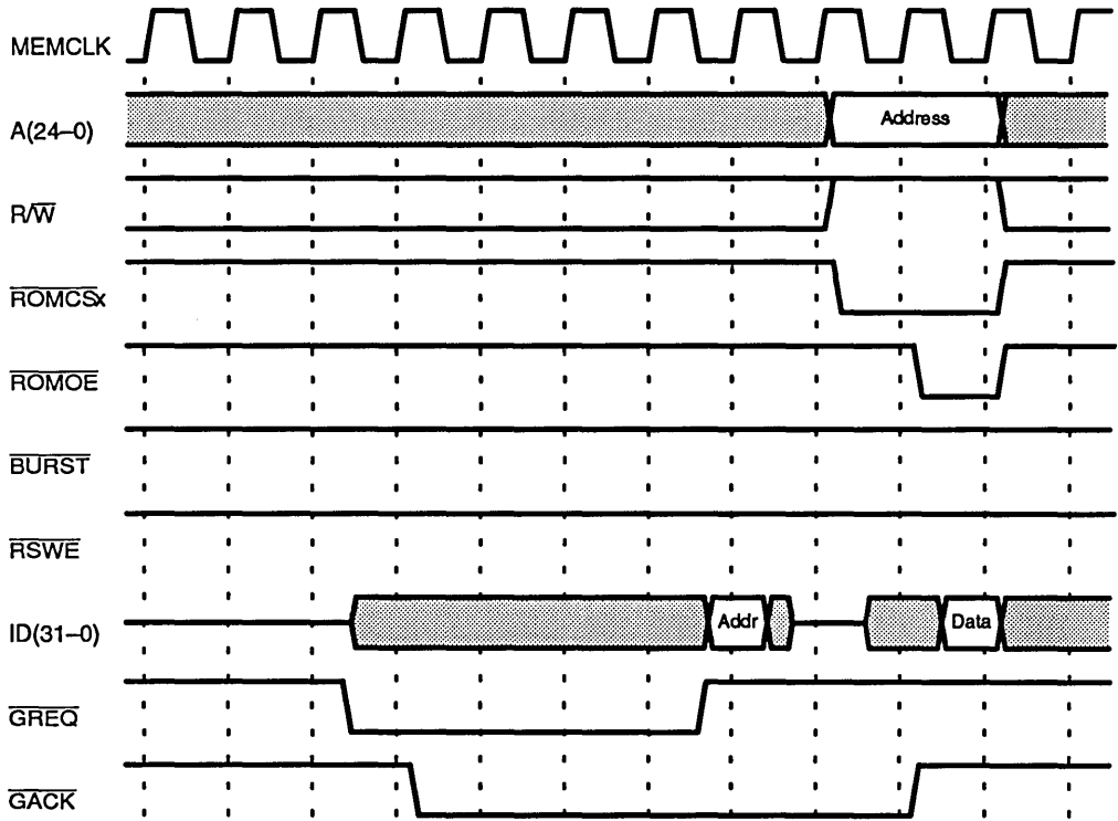
Figure 11-10 External Random ROM Read Cycle
