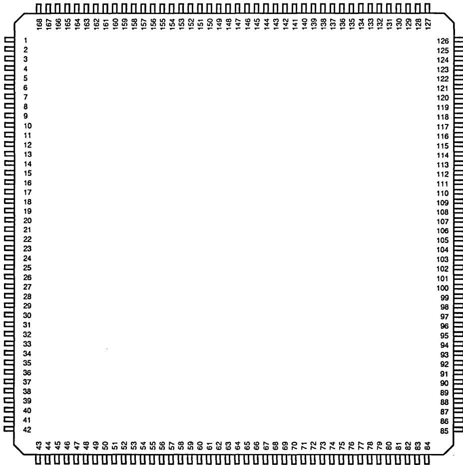
168-Pin PQFP
