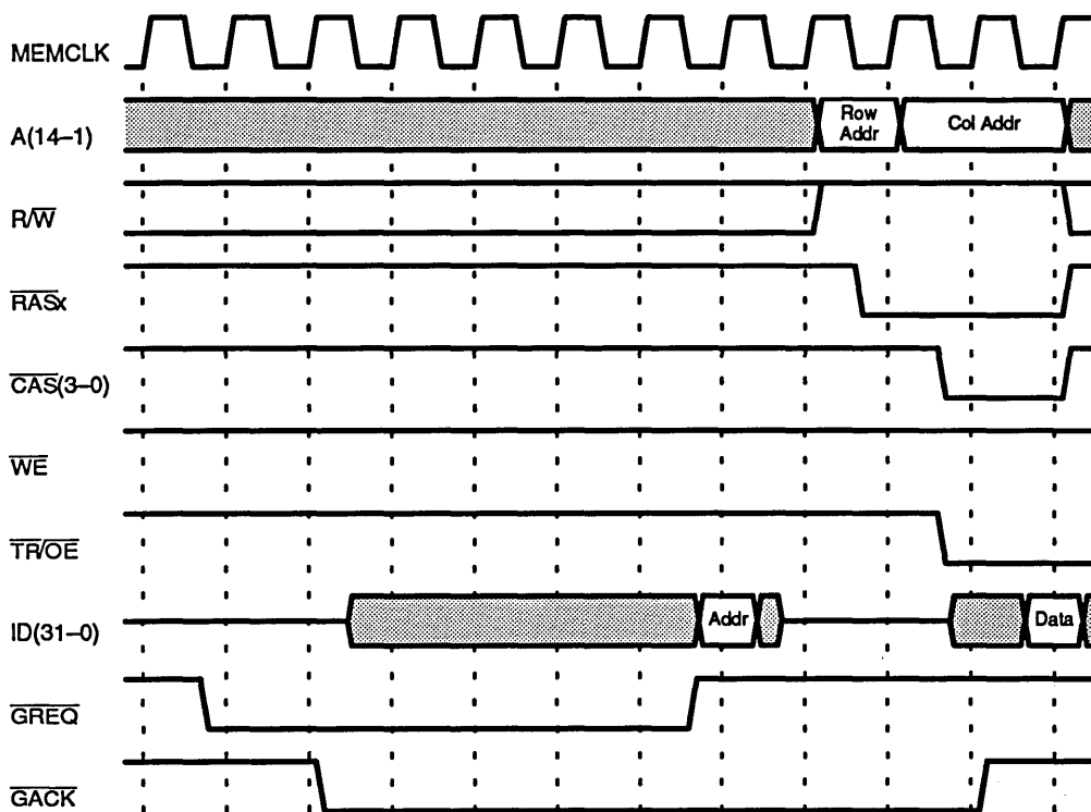
Figure 11-8 External Random DRAM Read Cycle
