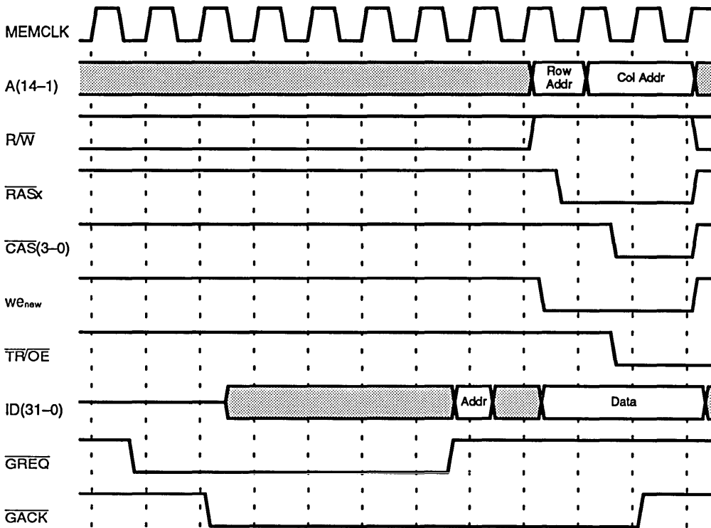
Figure 11-9 External Random DRAM Write Cycle
