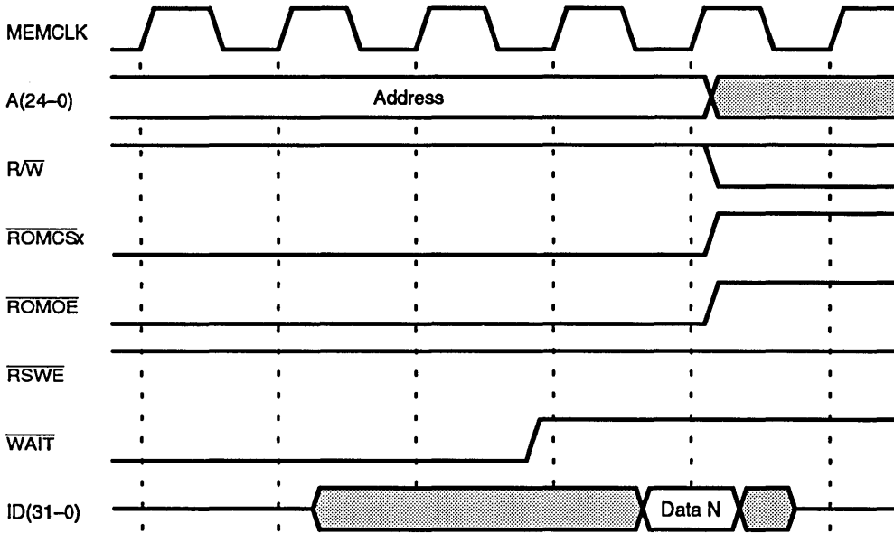
Figure 8-7 Extending a ROM Read Cycle with \overline{\text{WAIT}}
