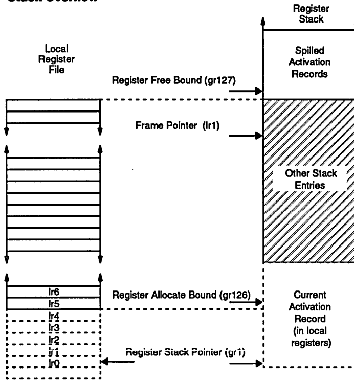
Figure 4-4 Stack Overflow
