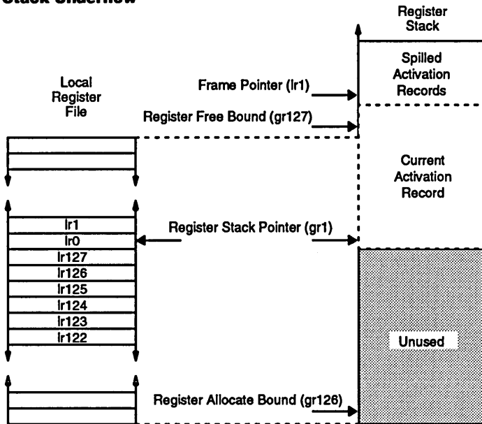
Figure 4-5 Stack Underflow
