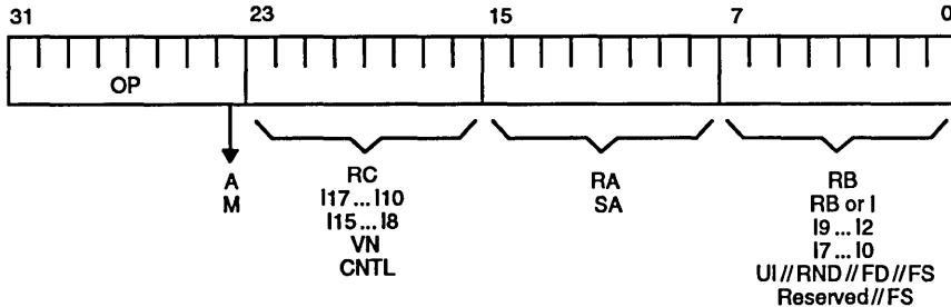
Figure 18-1 Instruction Format
