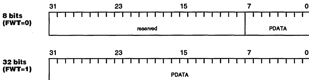
Figure 13-3 Parallel Port Data Register
