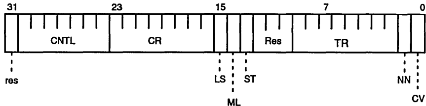
Figure 16-12 Channel Control Register
