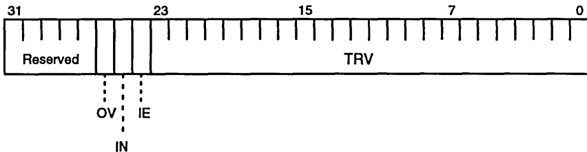
Figure 16-14 Timer Reload Register
