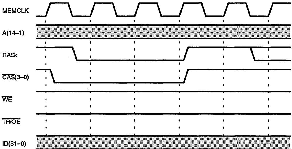
Figure 9-9 DRAM Refresh Cycle
