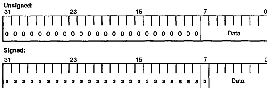
Figure 3-1 Character Format
