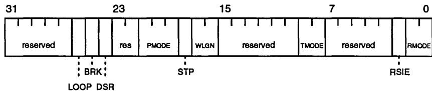
Figure 14-1 Serial Port Control Register
