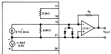
Figure 17. External Op Amp - Using External Feedback Resistors
