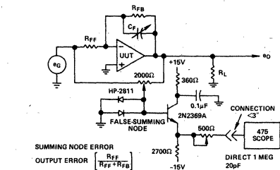
Figure 5. Settling Time Test Circuit for 0.1% Settling
