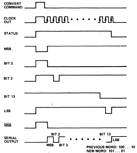
Figure 1. Timing Diagram
