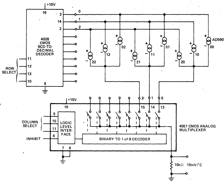
Figure 18. Matrix Multiplexer
