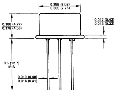
Figure 4. Outline Dimensions and Pin Designations. Dimensions shown in inches and (mm).
