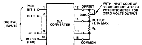
Figure 8. Bipolar Output Current
