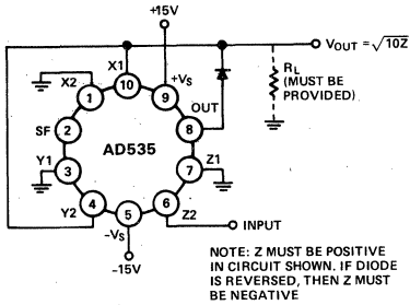
Figure 11. Square Rooter
