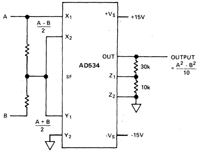
Figure 7. Difference-of-Squares
