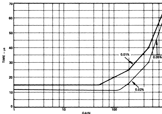
Figure 4. Typical Settling Time Curves for DAS1150
