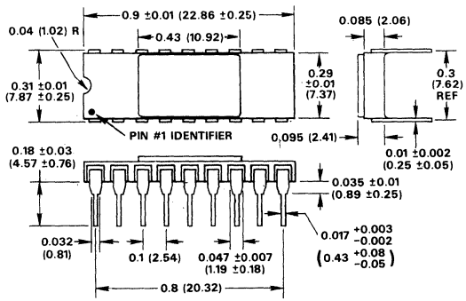
Figure 1. 18-Lead Ceramic Dual-In-Line Package
