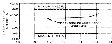
Figure 4. Model 450J: Nonlinearity Error Versus Input Signal
