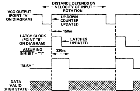
Timing Diagram
