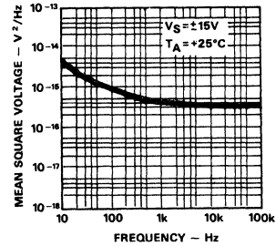
Figure 5. Input Noise Voltage vs. Frequency
