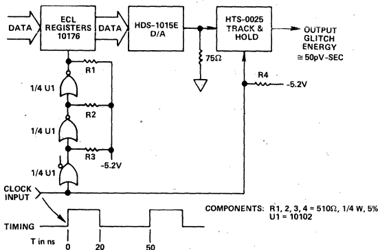
Figure 3. HTS-0025 Track & Hold Used with HDS-1015E D/A as Deglitcher @ 20MHz Update Rate
