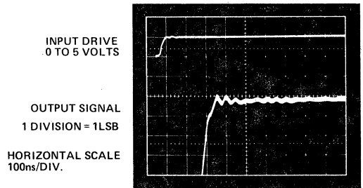
Figure 13. Settling Characteristic Detail
