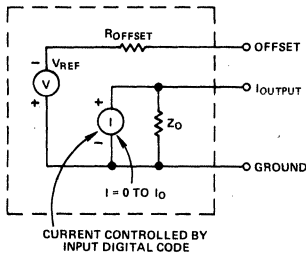
Figure 3. Current Equivalent Circuit
