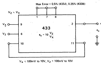
Figure 7. Divider
