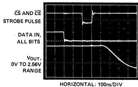
Figure 18. AD558 Logic Timing
