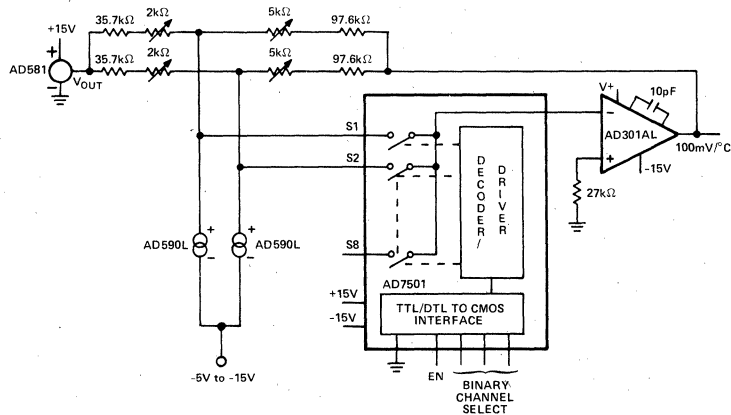
Figure 19. 8-Channel Multiplexer
