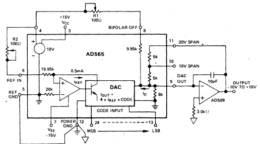
Figure 6. ±10V Voltage Output
