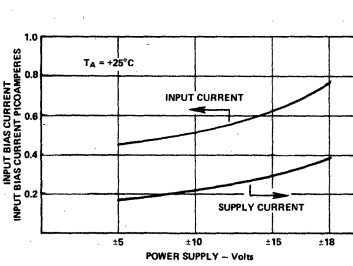
Figure 7. Input Bias Current and Supply Current Versus Supply Voltage
