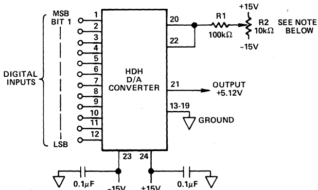
Figure 7. Unipolar Negative Output
