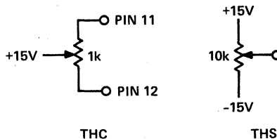
Figure 9. Optional Offset Adjustments
