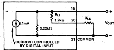
Figure 15. AD DAC80-CBI-1 Connected for Bipolar Output Voltage with Resistive Load
