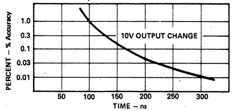
Figure 4a. Settling Accuracy vs. Acquisition Time – HTC-0300
