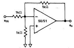
Figure 9. Recommended Circuit for Unity Gain Inverter
