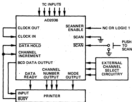
Figure 3. AD2036 with Printer
