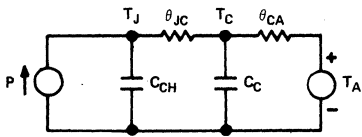
Figure 8. Thermal Circuit Model
