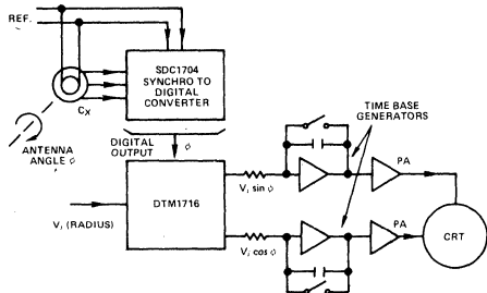
Figure 3. PPI Waveform Generation Using the DTM1716
