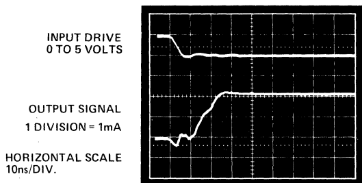
Figure 9. Full Scale Transition
