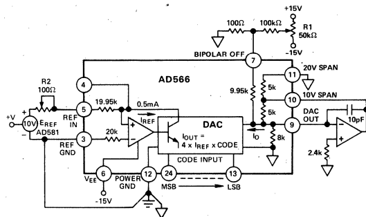
Figure 5. 0 to +10V Unipolar Voltage Output
