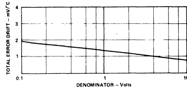
Figure 5. Total Error Drift vs. Denominator
