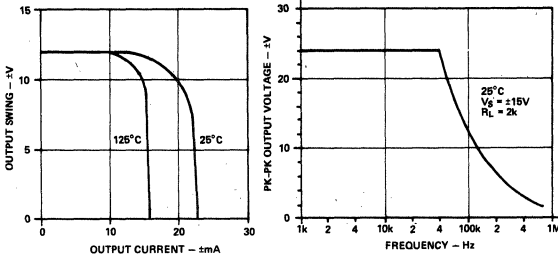
Figure 9. Current Limiting
