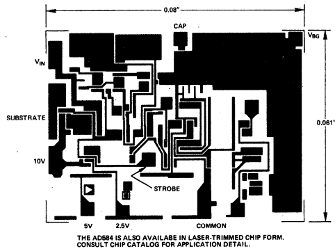
Figure 4. Bonding Diagram
