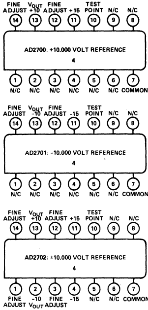
Pin Designations
