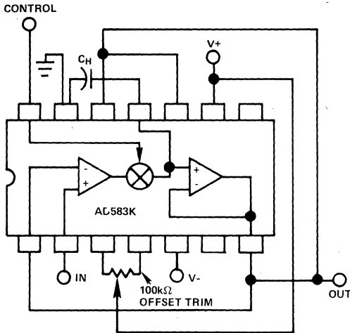
Figure 1. Basic Track-and-Hold/Sample-and-Hold
