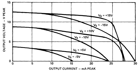
Figure 17. Output Characteristics
