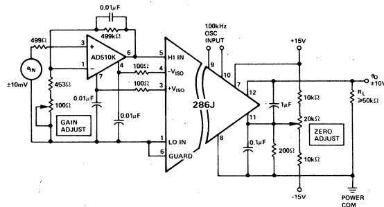
Figure 18. Input Signal Conditioning Using Isolated Power for Transducer Buffer Amplifier
