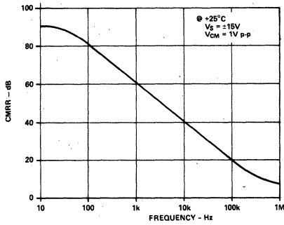
Figure 8. Common Mode Rejection
