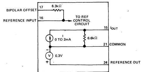
Figure 12. AD DAC85 Current Model Equivalent Output Circuit
