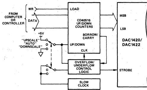
Figure 7. Block Diagram – Manual Incremental Control Scheme Using Up/Down Counters
