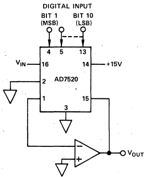
Figure 25. Analog/Digital Divider
