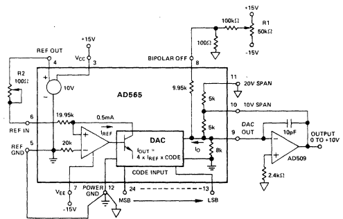
Figure 4. 0 to +10V Unipolar Voltage Output
