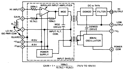
Figure 2. Block Diagram – Model 284J
