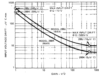
Figure 15. Max Input Offset Voltage Drift vs. Gain
