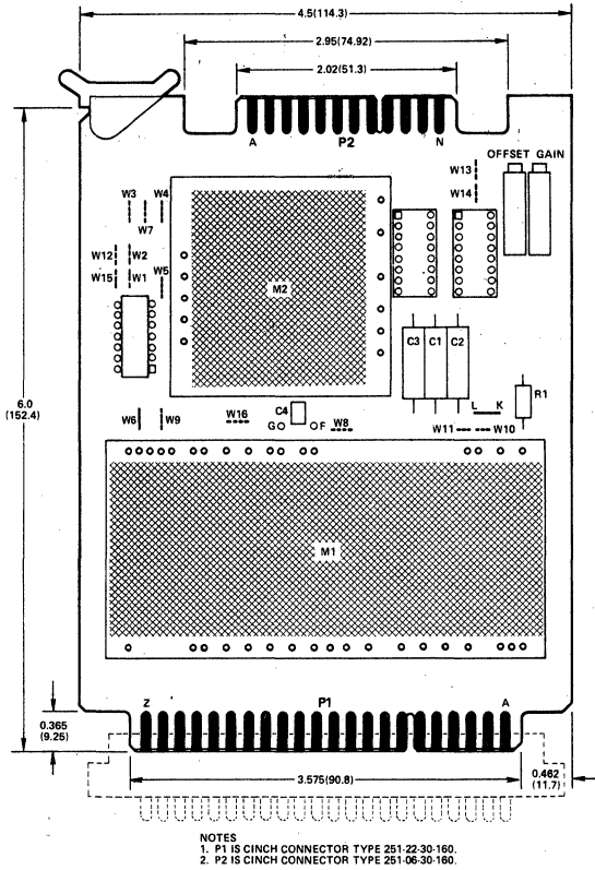
Figure 12. AC1580 Mounting Board
