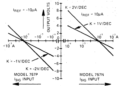
Log mode output voltage vs. input current for I_{REF} = 10\mu A . For voltage input calculate I_{SIG} as e_1/R_1 (see Figure 1).
