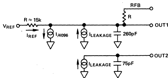
Figure 6. AD7542 DAC Equivalent Circuit All Digital Inputs HIGH
