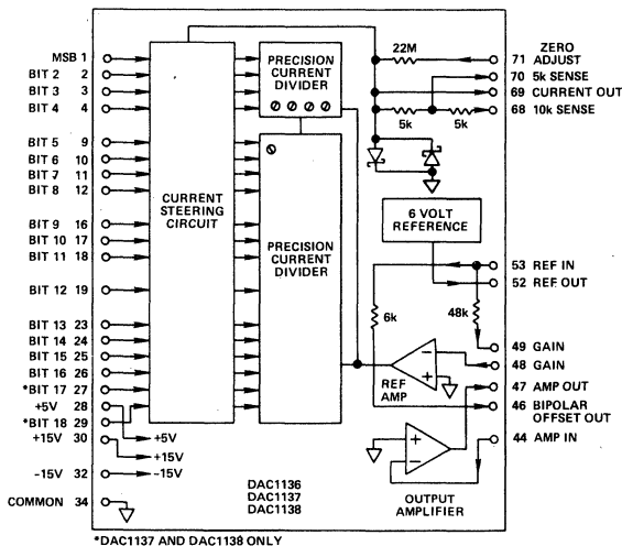
Figure 1. Block Diagram and Pin Designations
