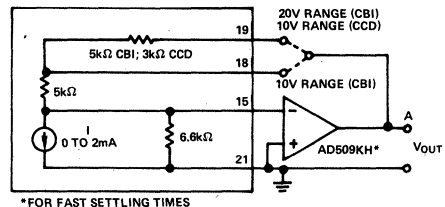
Figure 16. External Op Amp - Using Internal Feedback Resistors
