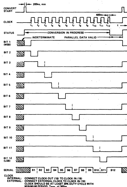
Figure 2. Timing Diagram (Binary Code 110101011001)
