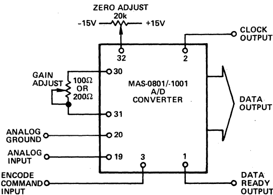
Figure 1. MAS-0801 and MAS-1001 Unipolar Operation
