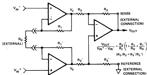
Figure 2. "Classic" 3 Op Amp Instrumentation Amplifier
