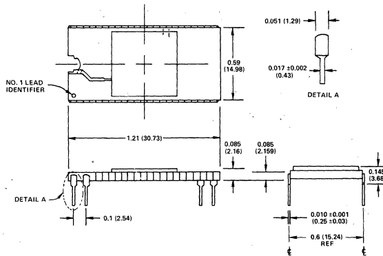
24 Lead Dual-in-Line Package
