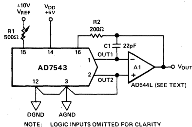
Figure 6. Unipolar Binary Operation (2-Quadrant Multiplication)
