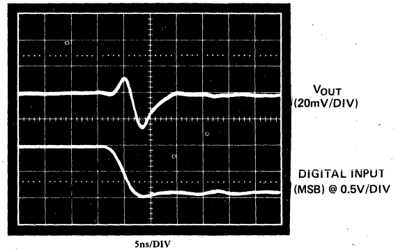
GLITCH ENERGY = 100\text{pV-SEC} ; FROM TEST CIRCUIT OF FIGURE 1.
