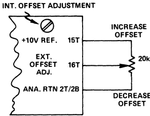
Figure 7. Ext. Offset Adjustment
