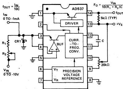
Figure 4. V-F Connections for Negative Input Voltage or Current
