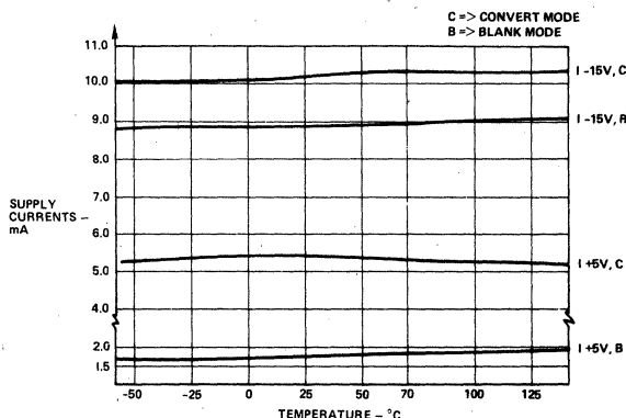
Figure 4. AD570 Power Supply Current vs. Temperature
