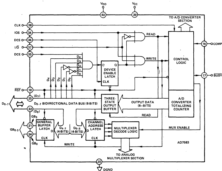
Figure 3. AD7583 Logic Section Functional Diagram
