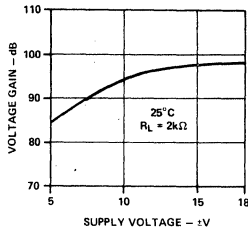
Figure 3. Voltage Gain
