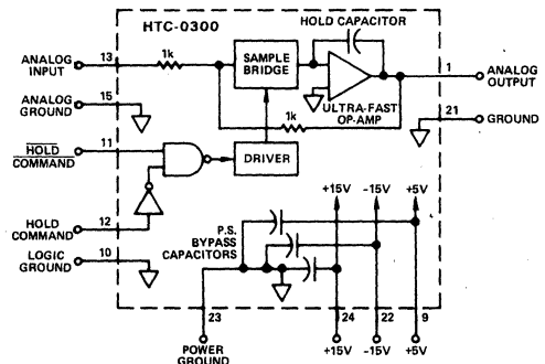
Block Diagram — HTC-0300
