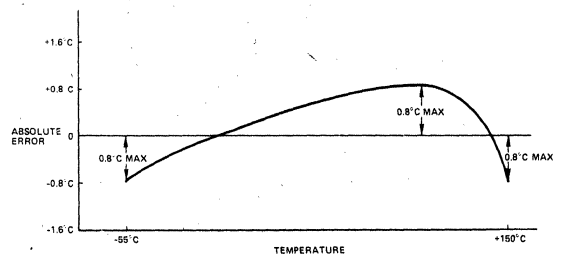
Figure 6. Nonlinearity
