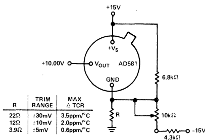
Figure 2. Optional Fine Trim Configuration
