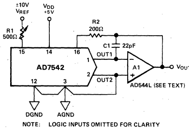
Figure 7. Unipolar Binary Operation (2-Quadrant Multiplication)
