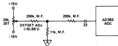
Figure 9. Low Tempco Zero Adj Circuit
