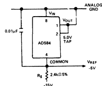
Figure 15. Two-Terminal -5 Volt Reference
