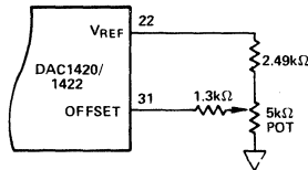
Figure 3. Offset Adjustment Circuit
