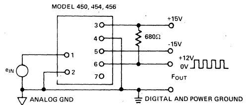
Figure 12. Driving High Noise Immunity Logic and CMOS
