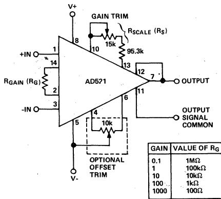
Figure 4. Operating Connections for AD521
