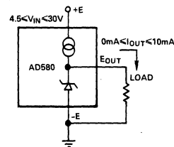
Figure 4. AD580 Connection Diagram
