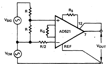
Figure 5. Ground Returns for "Floating" Transducers
