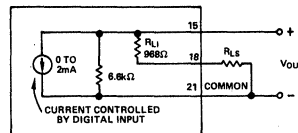
Figure 6a. Unipolar Voltage Output
