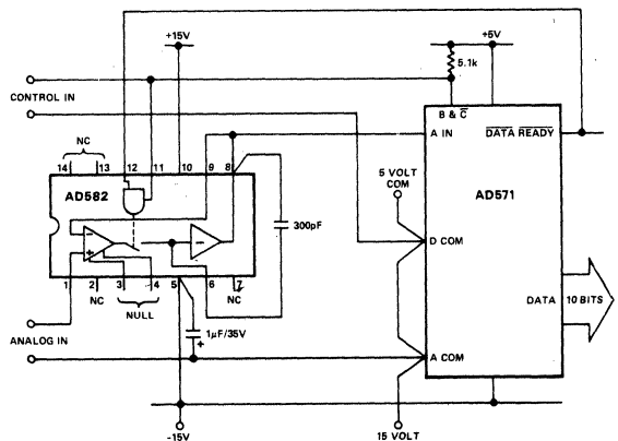
Figure 15. Sample-Hold Interface to the AD571
