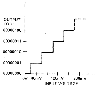
OFFSET CHARACTERISTICS WITH 10\Omega IN SERIES WITH ANALOG COMMON
