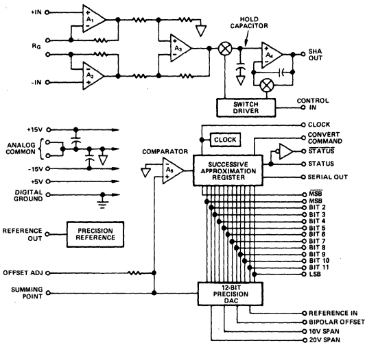
Figure 2. DAS1150 Block Diagram and Pin Designations
