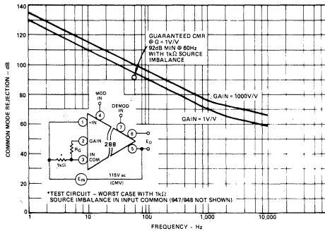
Figure 13. Common Mode Rejection vs. Frequency
