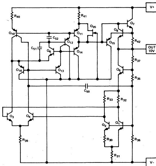
Figure 5. Simplified Schematic
