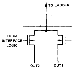
Figure 2. N-Channel Current Steering Switch
