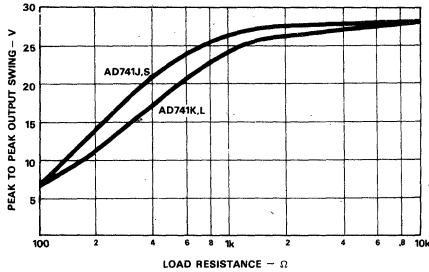
Figure 9. Output Voltage Swing vs. Load Resistance
