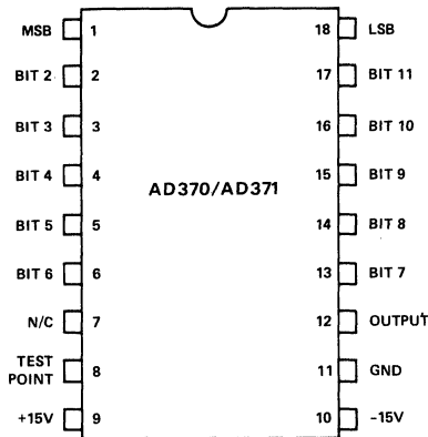
Figure 2. Pin Designations
