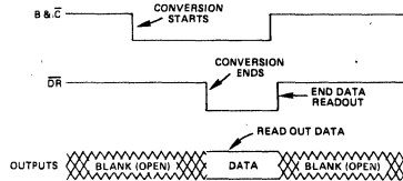
Figure 13. Multiplex Mode
