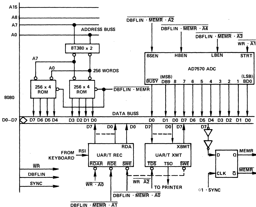
Figure 16. Microprocessor Controlled TTY/ADC Interface
