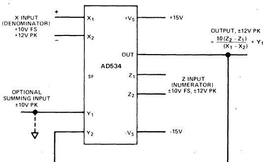
Figure 5. Basic Divider Connection
