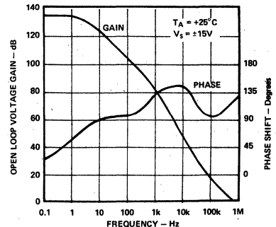
Figure 2. Open Loop Frequency Response
