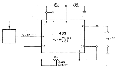
Figure 8. Transducer Linearization
