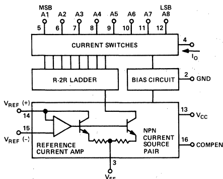
Figure 4. Simplified Block Diagram
