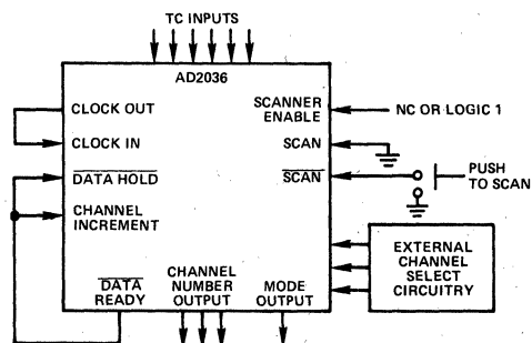
Figure 4. Stand-Alone Operation
