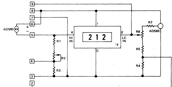
AD2040-dc Block Diagram
