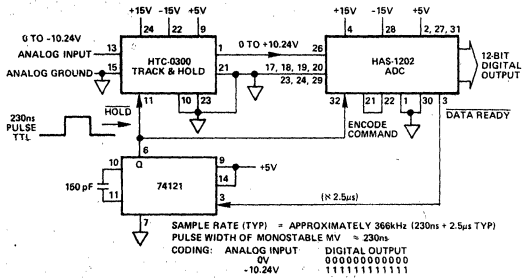
Figure 8. A/D Conversion System
