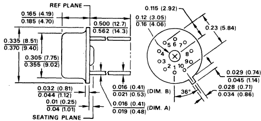
H-PACKAGE TO-100 (TOP VIEW)
