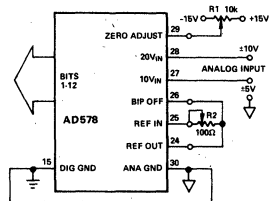
Figure 4. Bipolar Input Connections
