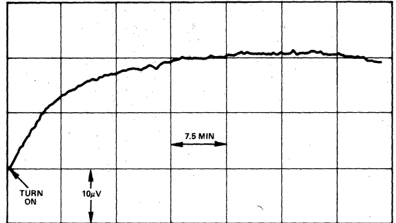
Figure 20. Warmup Voltage Drift for High Performance Modular Op Amp
