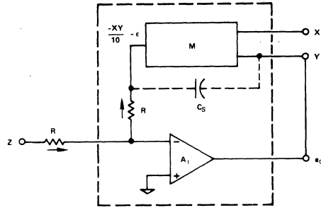
Figure 3. Divider Circuit
