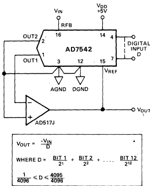
Figure 9. Divider (Digitally Controlled Gain)
