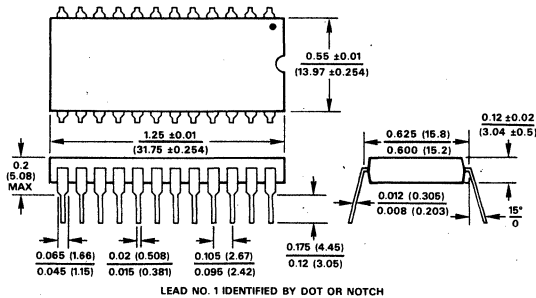
Figure 1. Molded Plastic Package (Type N) 24-Lead Dual-In-Line
