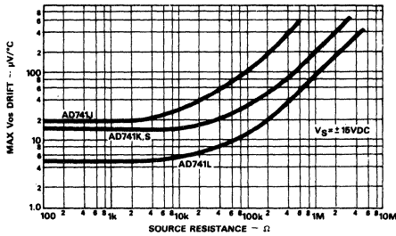
Figure 2. Max Equivalent Input Offset Drift vs. Source Resistance
