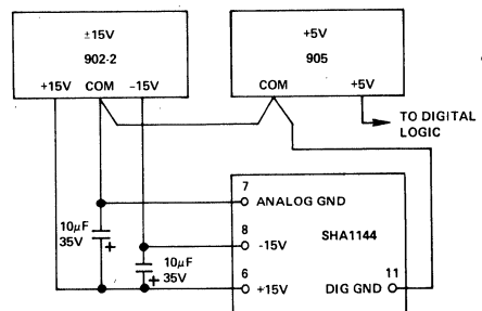
Figure 5. Power Supply and Grounding Connections
