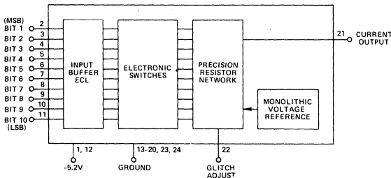
Block Diagram
