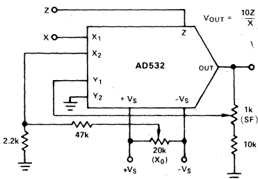
Figure 13. Divider Connection
