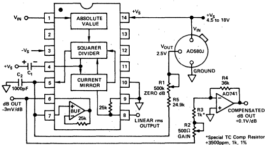
Figure 13. dB Connection
