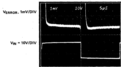
Figure 15b. Settling Characteristic Detail
