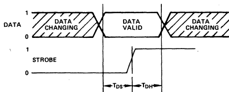
Figure 5. Input Timing
