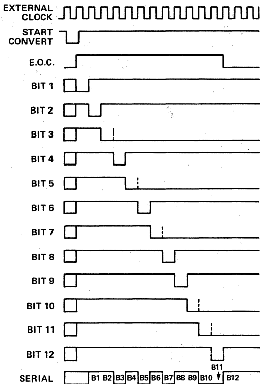
Figure 2. Timing Diagram
