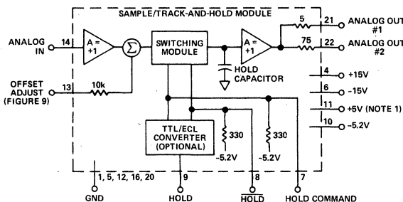
Figure 7. Sample/Track-and-Hold THC Series Block Diagram
