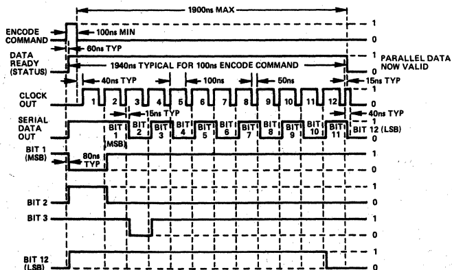
Figure 8. MAS-1202 Timing Diagram
