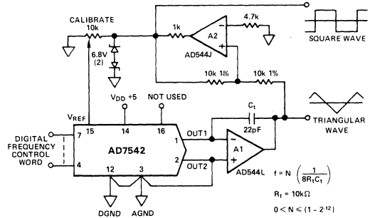
Figure 10. Programmable Function Generator
