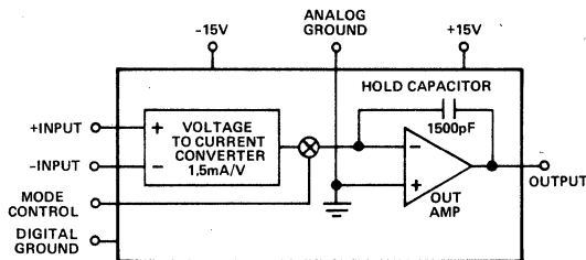
Figure 1. Block Diagram – SHA1144
