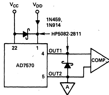
Figure 12. Diode Protection Scheme
