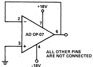
Burn-In Circuit
