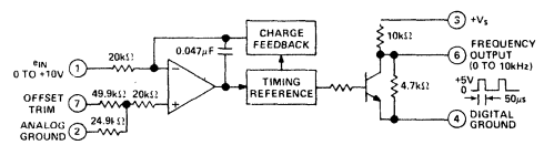
Figure 1. Block Diagram – Models 450 and 456
