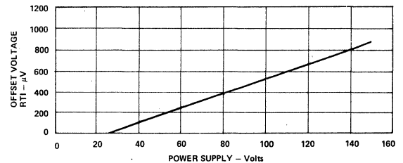
Figure 6. Input Offset Voltage vs. Power Supply Voltage
