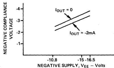
Figure 10. Typical Negative Compliance Range Vs. Negative Supply.
