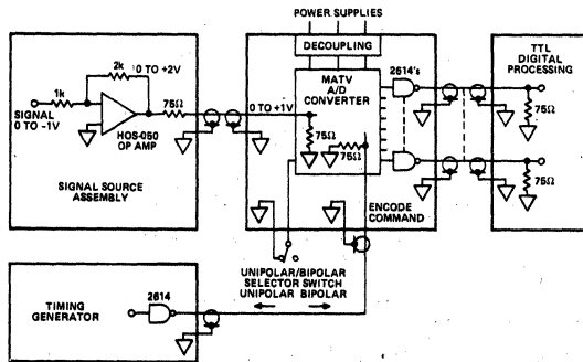
Figure 4. Typical System Application
