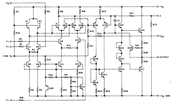
Figure 2. AD532 Schematic Diagram
