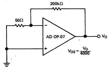
Offset Voltage Test Circuit
