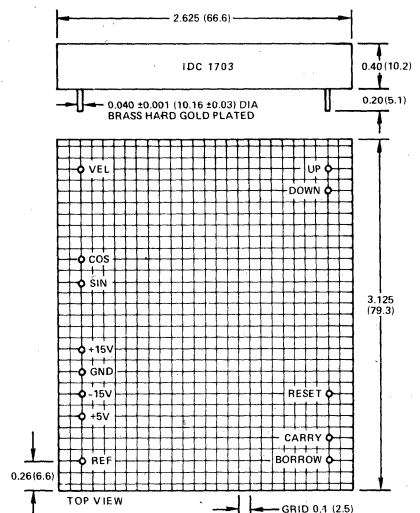
Pin Connections for IDC 1703. Dimensions shown in inches and (mm).
