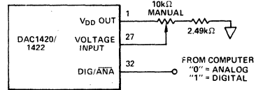
Figure 6. Potentiometer Backup Control
