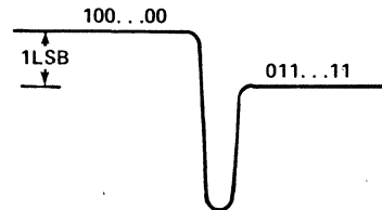
Figure 1. Switching Transient Caused by Time Skew
