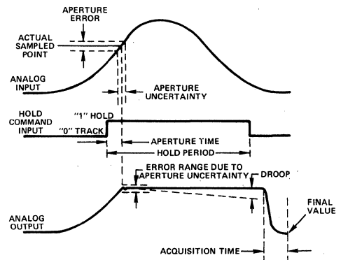
Figure 1. Track-and-Hold Operation
