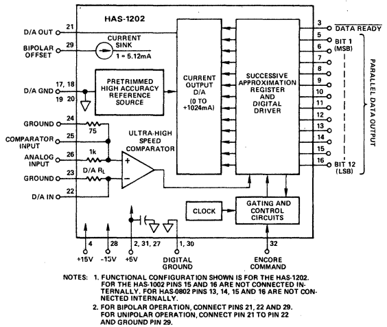
Block Diagram — HAS Series
