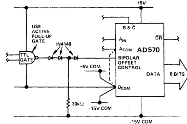
Figure 7. Bipolar Offset Controlled by Logic Gate
