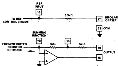
Figure 5. Output Amplifier Voltage Range Scaling Circuit
