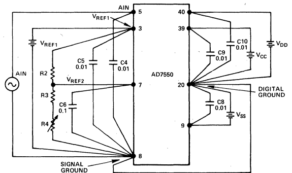
Figure 7. Ground System
