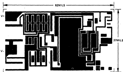
Metalization Diagram
