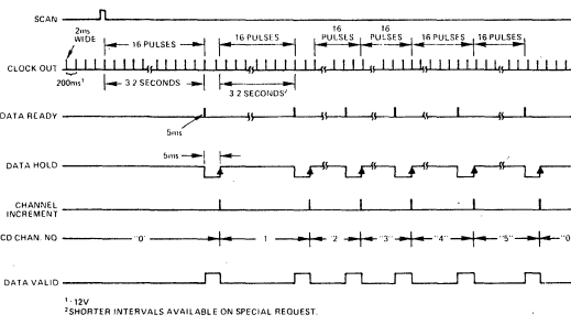
Figure 2. Scan Timing Diagram
