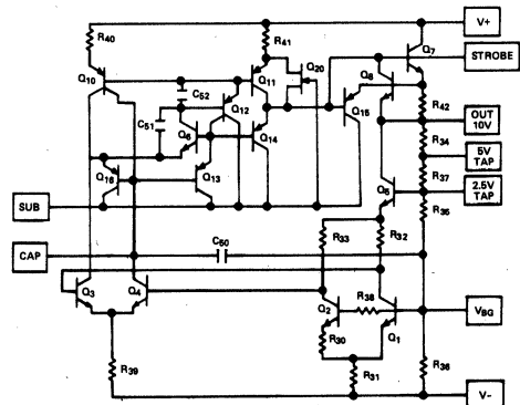
Figure 5. Schematic Diagram
