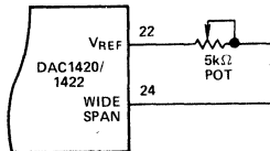
Figure 4b. Span Adjust
