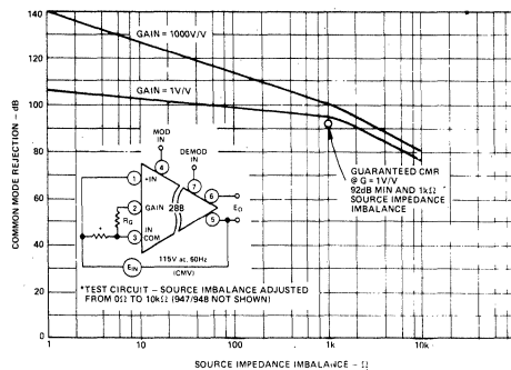
Figure 14. CMR vs. Source Impedance Imbalance
