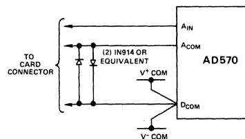
Figure 8. Differential Common Voltage Protection
