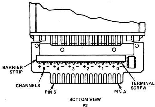
Figure 5. Thermocouple Connections
