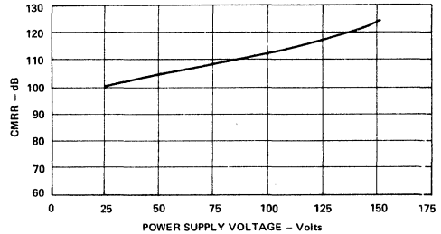
Figure 5. CMRR vs. Power Supply Voltage
