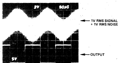
Figure 16. Performance of AD537 Linear Phase-Locked Loop
