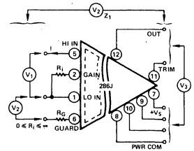
Figure 5. Model 286J Terminal Ratings
