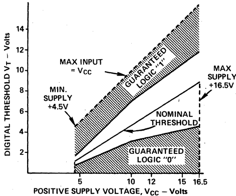
Figure 1. Digital Threshold Vs. Positive Supply
