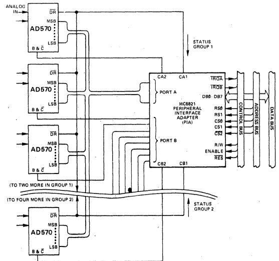
Figure 16. Multiplexing 10 AD570's Using Single PIA for \mu\text{P} Interface. No Other Logic Required (6800 Control Structure).
