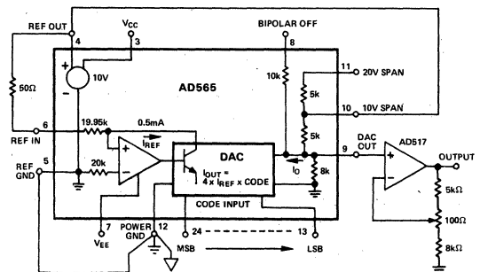
Figure 14. Complementary Output DAC
