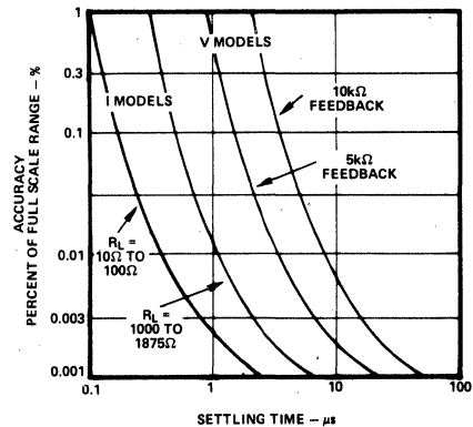
Figure 4. Full Scale Range Settling Time vs. Accuracy
