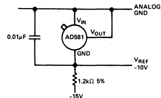
Figure 14. Two-Terminal -10 Volt Reference
