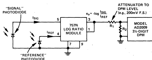
Figure 8. Model 757N Applied to Absorbance Measurements
