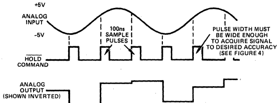
Figure 2. Sample/hold Operation – HTC-0300
