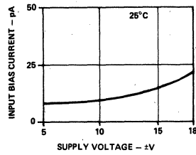
Figure 12. Input Bias Current vs. Supply Voltage
