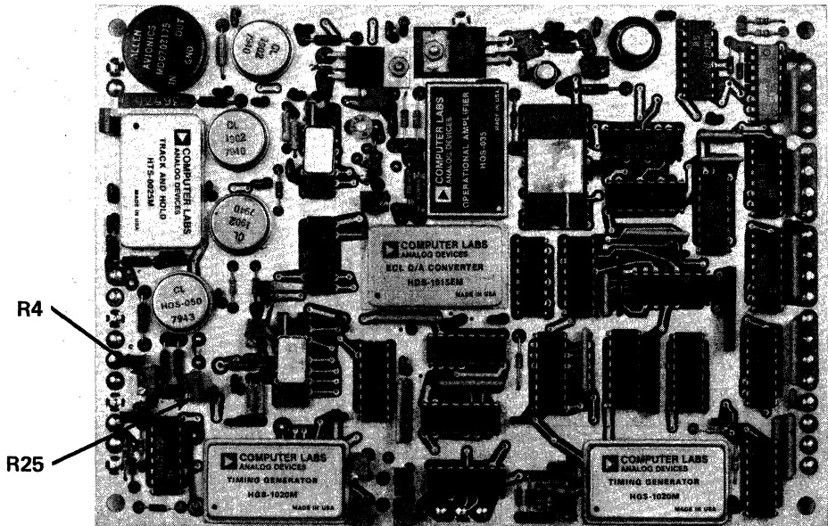
Location of Adjustment Potentiometers
