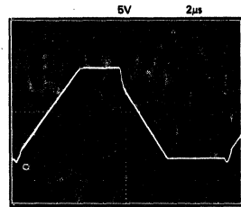
Figure 14a. Unity Gain Follower Pulse Response
