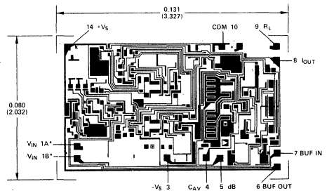
Figure 10. Physical Dimensions Dimensions shown in inches and (mm).
