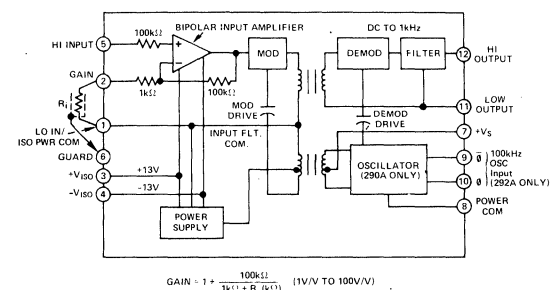
Figure 2. Block Diagram – Models 290A and 292A
