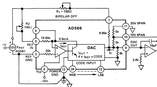
Figure 6. \pm 5\text{V} Bipolar Voltage Output
