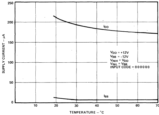
Figure 2. Power Supply Current vs. Temperature
