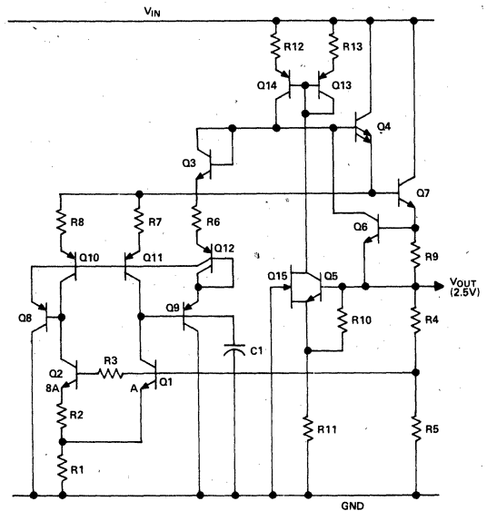
Figure 2. AD1403/AD1403A Schematic Diagram
