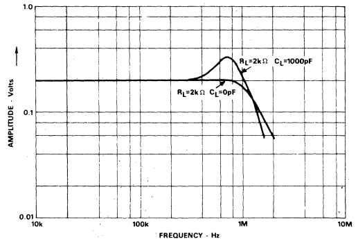
Figure 7. Frequency Response, Multiplying
