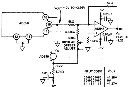
Figure 11. Bipolar Operation of AD558 from ±5V Supplies
