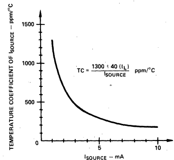
Figure 10b. Typical Temperature Coefficient of Current Source
