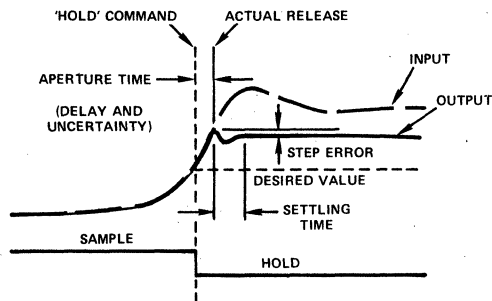
Figure 4c.
