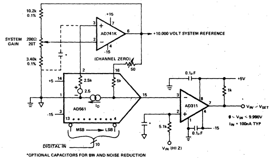
Figure 14. Digitally Programmable Set Point Comparator
