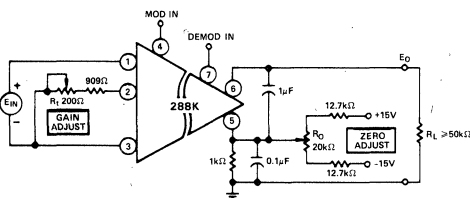
Figure 4. Gain and Offset Adjustment
