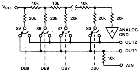
Figure 7. DAC Circuit
