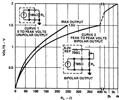
Figure 5. V_{OUT} vs. Load Resistance MDS-0815, -1020
