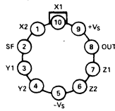
H-PACKAGE TO-100 (TOP VIEW)
