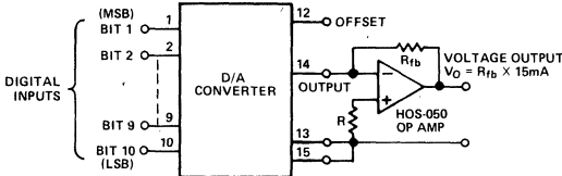
Figure 11. Voltage Output
