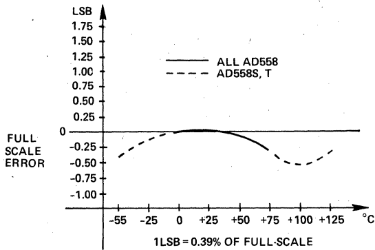
Figure 13. Full Scale Accuracy vs. Temperature Performance of AD558
