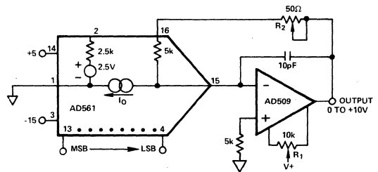
Figure 5. 0 to +10V Unipolar Voltage Output
