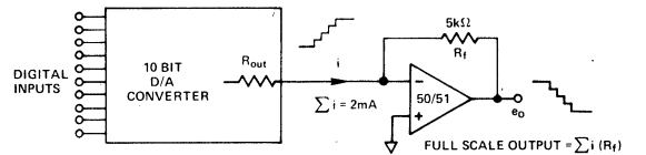
Figure 1. High Speed Current to Voltage Buffer
