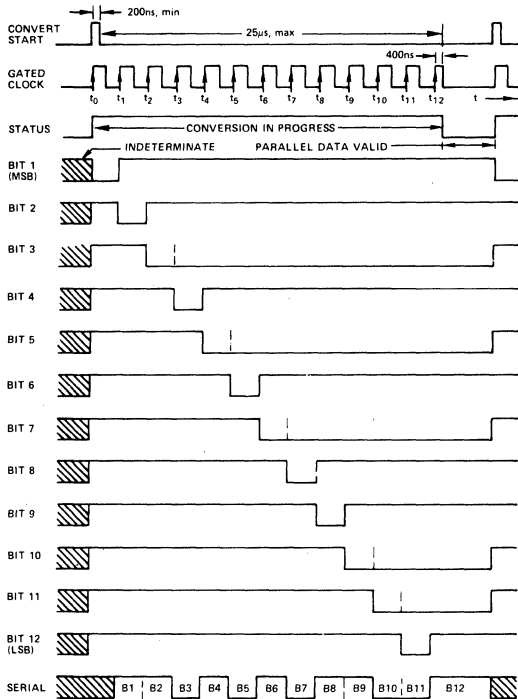
Figure 5. ADC Timing Diagram (Binary Code 110101011001)
