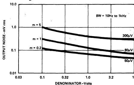
Figure 6. Model 433 Noise vs. Denominator for Various Exponents, m
