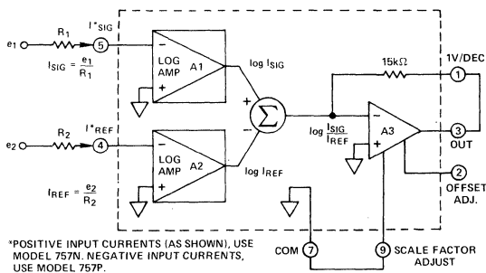
Figure 1. Functional Block Diagram of Model 757
