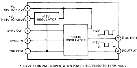
Figure 12. Model 281 Block Diagram
