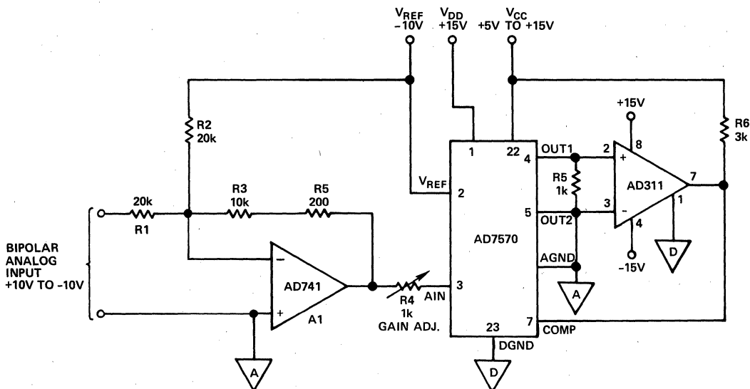
Figure 10. Unipolar Operation
