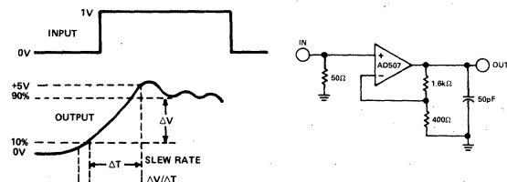
Slew Rate Definition and Test Circuit
