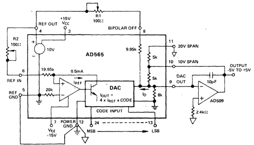
Figure 5. ±5V Bipolar Voltage Output
