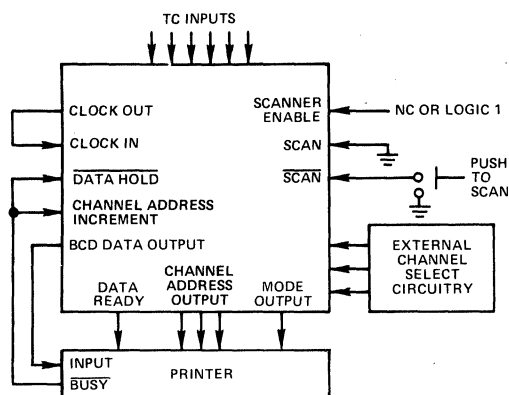
Figure 4. Operation with Printer
