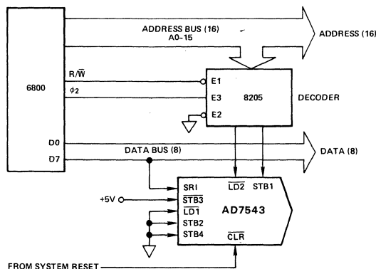
Figure 8. AD7543-MC6800 Interface
