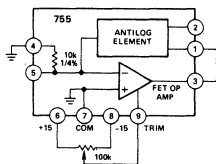
Figure 3. Trimming E_{OS} in Log Mode
