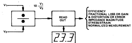
Figure 10. Ratio Measurements
