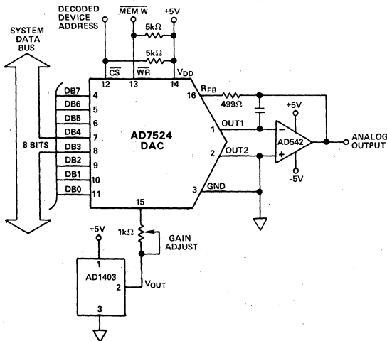
Figure 9. Low Power, Low Voltage Reference for the AD7524 Microprocessor-Compatible 8-Bit DAC
