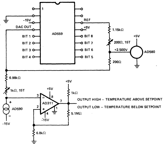
Figure 16. DAC Setpoint
