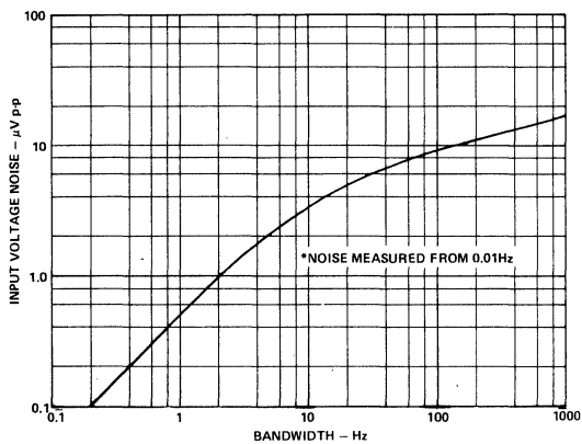
Figure 3. Input Voltage Noise vs. Bandwidth for Model 235
