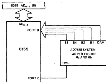
Figure 8. AD7555 as a Polled Input Device
