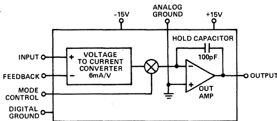
Figure 1. Block Diagram
