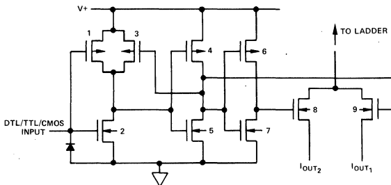
Figure 12. CMOS Switch
