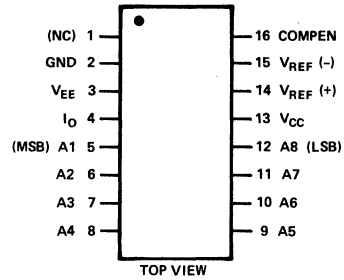
Figure 1. Pin Connections
