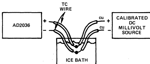
Figure 8. Calibration Diagram
