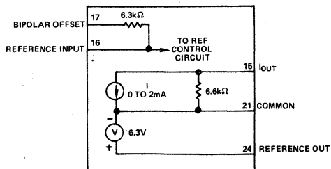
Figure 12. AD DAC80 Current Model Equivalent Output Circuit
