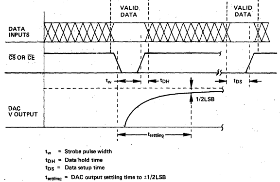
Figure 8. AD558 Timing
