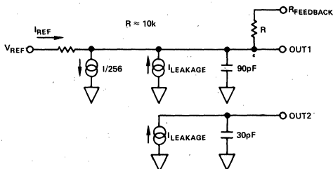
Figure 4. AD7524 DAC Equivalent Circuit - All Digital Inputs High
