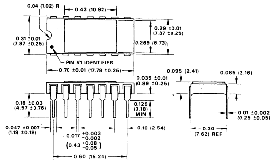
Figure 2. Physical Dimensions. Dimensions shown in inches and (mm).
