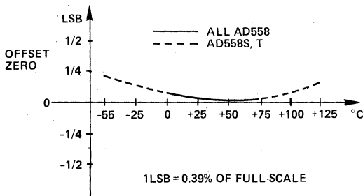
Figure 14. Zero Drift vs. Temperature Performance of AD558
