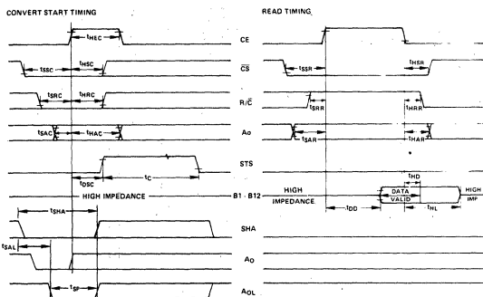
Figure 3. AD364 Timing Diagram
