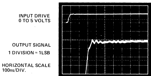
Figure 10. Settling Characteristic Detail
