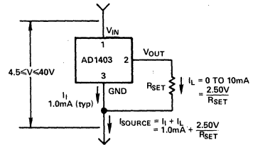
Figure 10a. The AD1403 as a Precision Programmable Current Source
