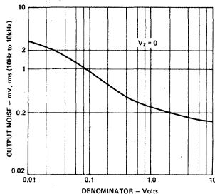
Figure 8. Output Noise vs. Denominator – 5Hz to 10kHz
