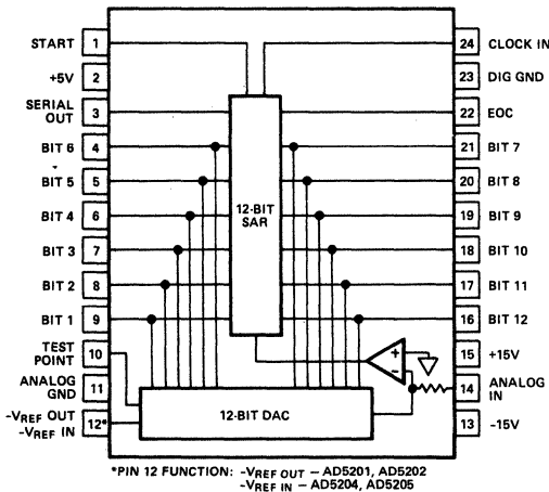
Figure 1. Pin Designations
