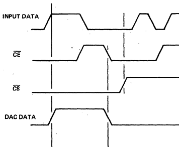
Figure 7. AD558 Control Logic Function
