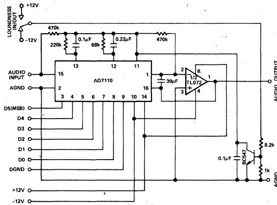
Figure 7. Single Channel Audio Attenuator with Loudness Compensation
