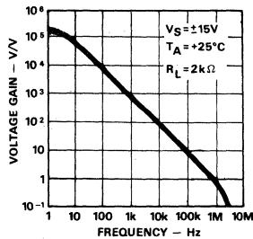
Figure 10. Open Loop Gain vs. Frequency
