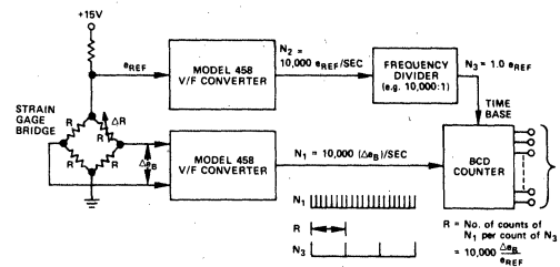
Figure 9. High Resolution, Wide-Range Ratiometer Using Model 458 V/F Converter
