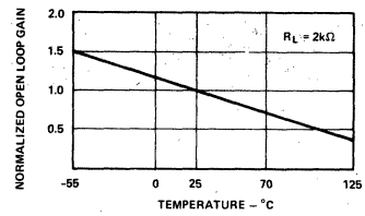
Figure 12. Open Loop Gain vs. Temperature
