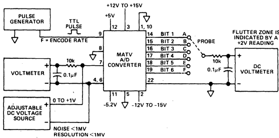
Figure 6. DC Calibration Set-Up
