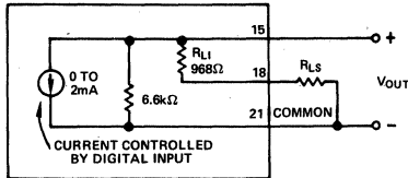
Figure 13. Equivalent Circuit AD DAC80-CBI-1 Connected for Unipolar Voltage Output with Resistive Load
