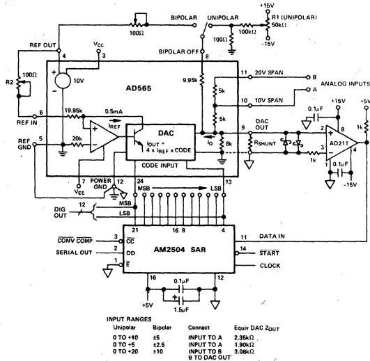
Figure 12. Fast Precision Analog to Digital Converter
