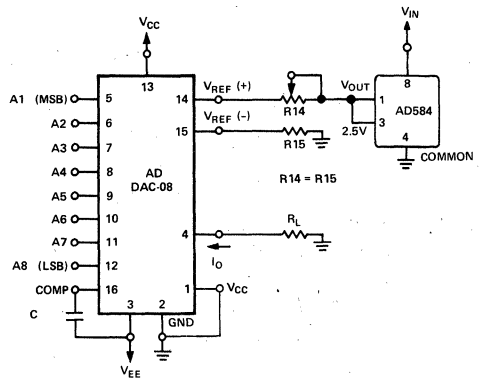
Figure 19. Current Output 8-Bit D/A
