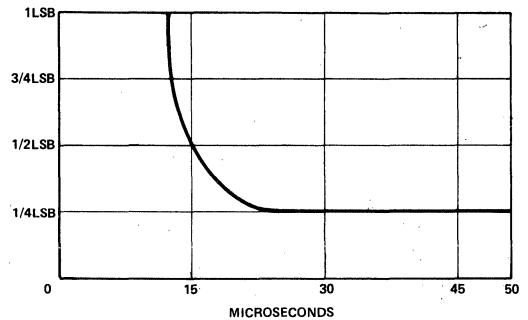
Figure 3. Linearity Error vs. Conversion Time (Normalized)
