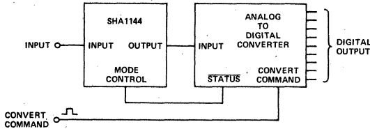
Figure 6. SHA1144 and A/D Connections
