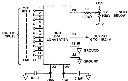
Figure 6. Noninverting Unipolar or Bipolar Voltage Output – HDS-1025
