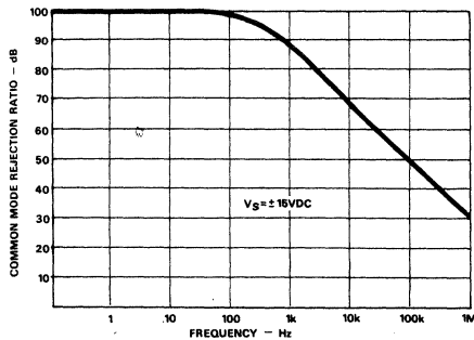
Figure 4. Common Mode Rejection vs. Frequency
