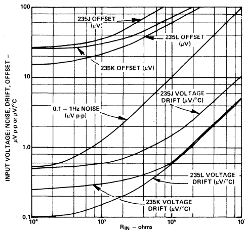
Figure 4. Uncompensated Offset, Drift and Noise vs. R_{IN}
