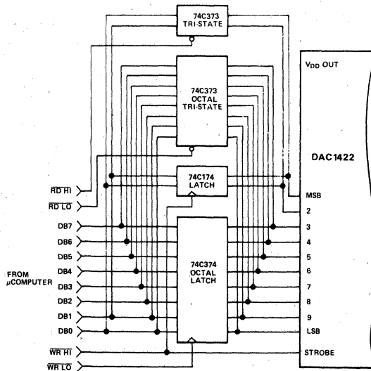
Figure 9. DAC1422 with \mu P Interface and Readback Capability
