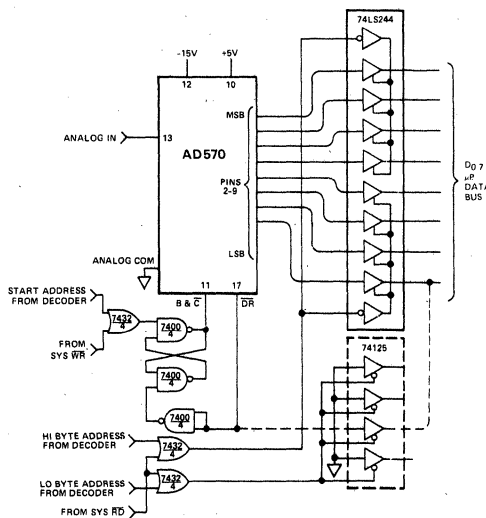
Figure 15. Interfacing AD570 to an 8-Bit Bus (8080 Control Structure)
