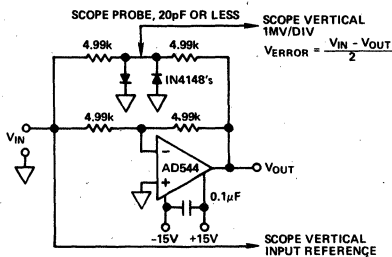
Figure 15a. Settling Time Test Circuit
