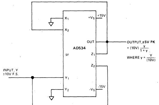
Figure 12. Bridge-Linearization Function
