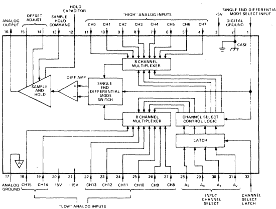
Figure 2. AD363 Analog Input Section Functional Block Diagram and Pinout
