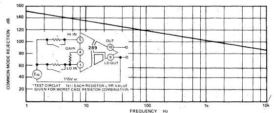
Figure 11. Typical Common Mode Rejection vs. Frequency
