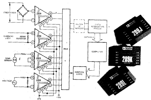
4 CHANNEL ISOLATED DATA ACQUISITION SYSTEM
