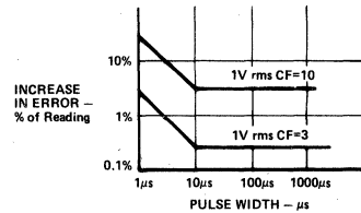
Figure 16. AD536A Error vs. Pulse Width Rectangular Pulse
