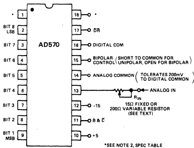
Figure 6. Standard AD570 Connections
