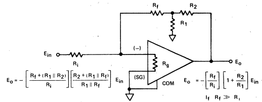
Figure 7. "T" Network
