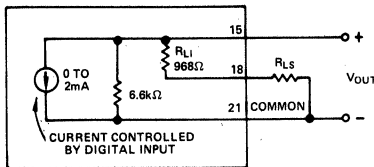
Figure 13. Equivalent Circuit AD DAC85-CBI-I Connected for Unipolar Voltage Output with Resistive Load
