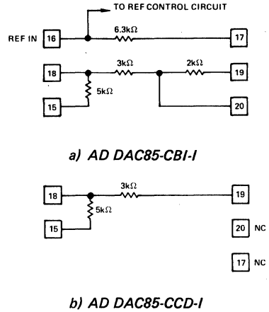
Figure 11. Internal Scaling Resistors
