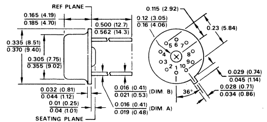
Figure 10. Physical Dimensions Dimensions shown in inches and (mm).
