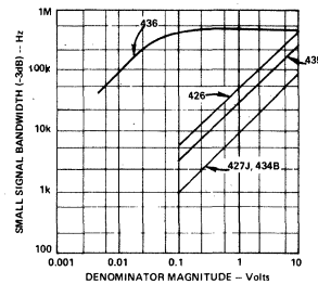
Figure 9. Bandwidth (-3dB) vs. Denominator
