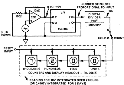
Figure 8. Models 458/460 as Long Term Integrator with Arbitrary Display Calibration. Frequency Division Ratio can Otherwise be Chosen to Provide Direct Readout in any Desired Units.
