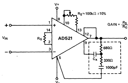
Figure 7. Optional Compensation Circuit
