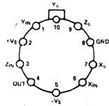
AD533H TO-100
