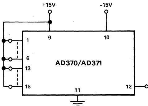
Figure 4. Burn-In Circuit
