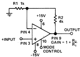
Figure 3. Noninverting Operation
