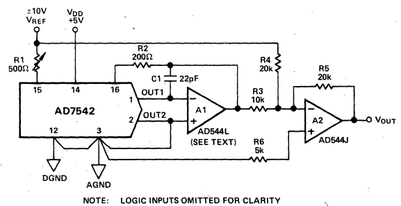
Figure 8. Bipolar Operation (4-Quadrant Multiplication)
