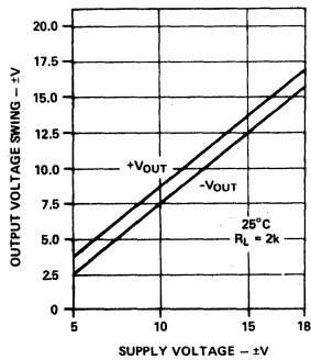
Figure 2. Output Swing
