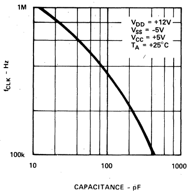
Figure 4. f_{CLK} vs. C_3
