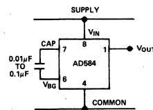
Figure 9. Additional Noise Filtering with an External Capacitor
