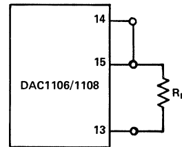
Figure 6. Voltage Output with Load Resistor (Bipolar)
