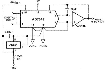
Figure 12. 0 to +10V Fixed Reference DAC
