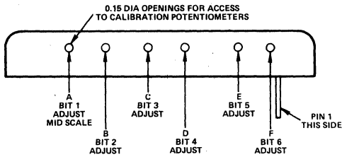
Figure 5. Location of Calibration Potentiometers
