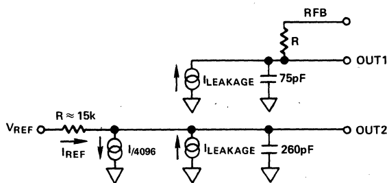
Figure 5. AD7542 DAC Equivalent Circuit All Digital Inputs LOW
