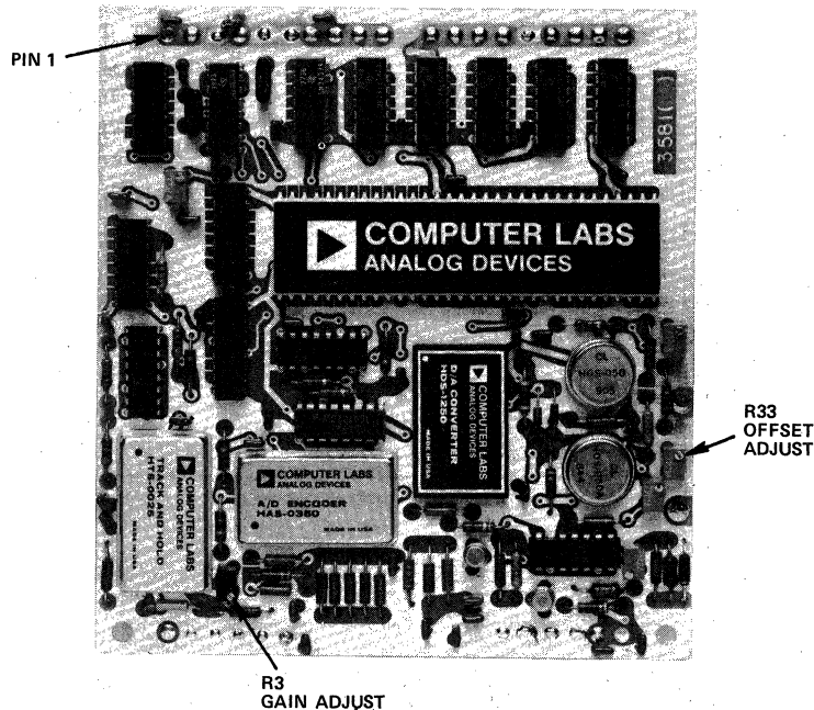
A/D Converter Assembly
