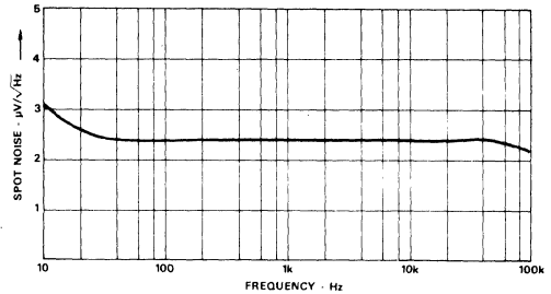
Figure 10. Spot Noise vs. Frequency
