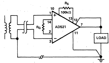
a). Transformer Coupled, Direct Return
