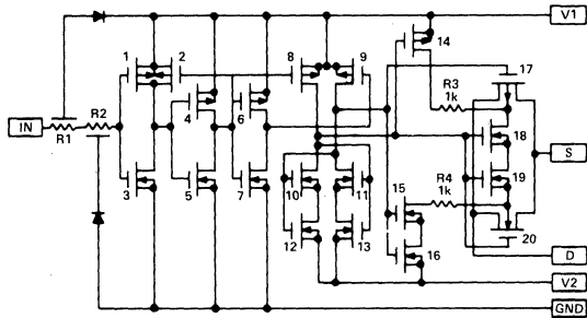
Figure 1. Schematic Diagram, 1 of 4 Channels
