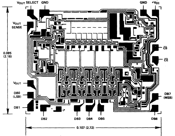
Figure 2. AD558 Chip Bonding Diagram (Dimensions shown in inches and (mm))
