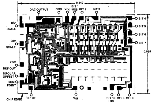
Figure 3. Chip Bonding Diagram
