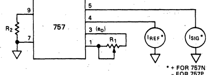
Figure 2. Scale Factor Adjustment
