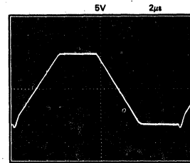
Figure 14b. Unity Gain Inverter Pulse Response
