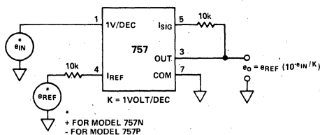
Figure 7. Model 757 Antilog Connection
