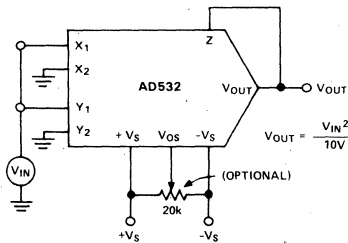
Figure 12. Squarer Connection
