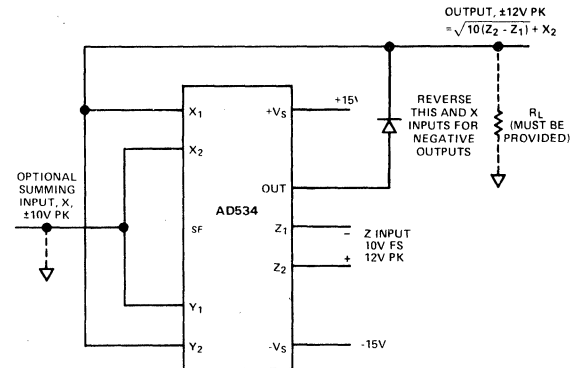
Figure 6. Square-Rooter Connection
