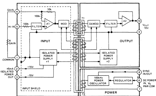
Figure 2. Model 289 Block Diagram
