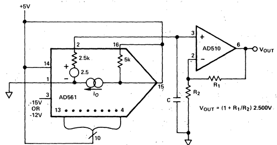
Figure 9. Precision Ultra Low Noise Reference
