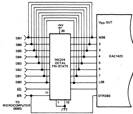
Figure 8. DAC1420 with \mu P Interface and Readback Capability
