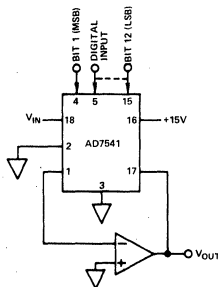
Figure 18. Analog/Digital Divider
