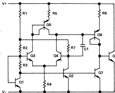
Figure 4. Schematic Diagram
