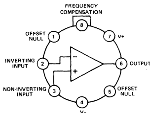
TO-99 PIN CONFIGURATION
