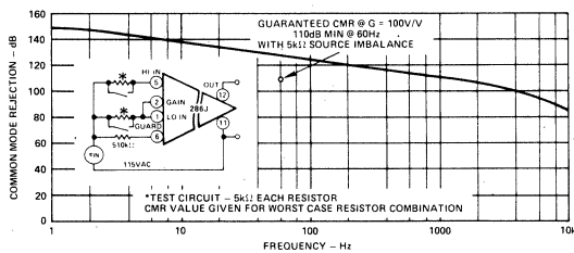
Figure 7. Common Mode Rejection vs. Frequency
