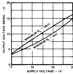
Output Swing
