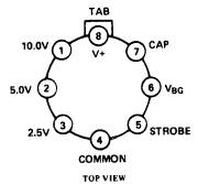
Figure 3. Pin Designations
