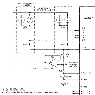
Figure 12. Linear Thermistor Thermometer
