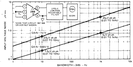
Figure 16. Input Voltage Noise vs. Bandwidth
