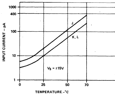
Figure 4a. Input Current vs. Temperature
