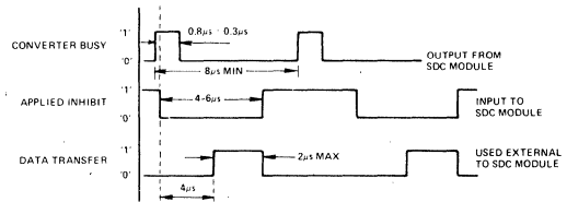
Data Transfer Waveforms
