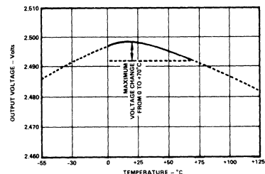
Figure 5. Typical AD580K Output Voltage vs. Temperature
