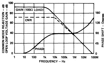
Figure 6. Model 50 Frequency Response
