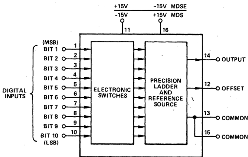
MDS and MDSE Block Diagram
