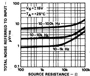
Figure 7. Broadband Noise vs. Source Resistance
