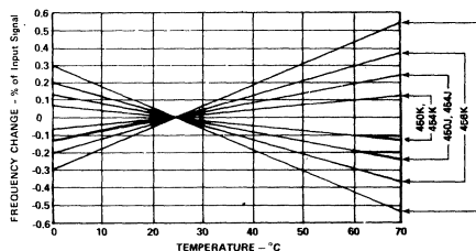
Figure 5. Gain Frequency Drift (Worst Case)
