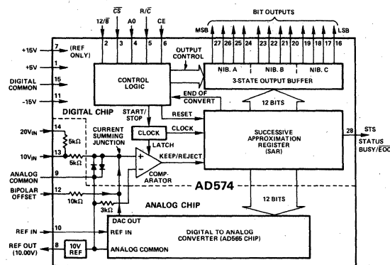
Figure 3. Block Diagram of AD574 12-bit A-to-D Converter
