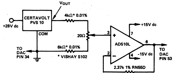
Figure 5. DAC1136/1137/1138 with External Precision Reference
