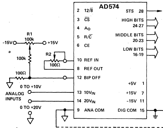
Figure 4. Unipolar Input Connections
