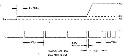
Figure 13. Timing Waveforms; Input/Output
