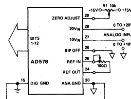
Figure 3. Unipolar Input Connections
