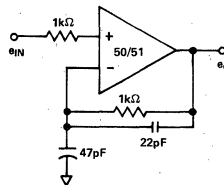
Figure 8. Recommended Circuit for Unity Gain Noninverting Buffer
