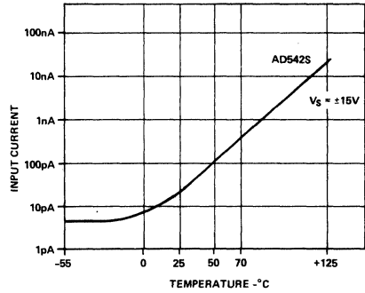
Figure 4b. Input Current vs. Temperature
