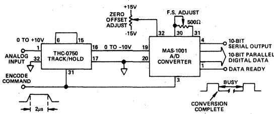
Figure 6. A/D Conversion System (THC)
