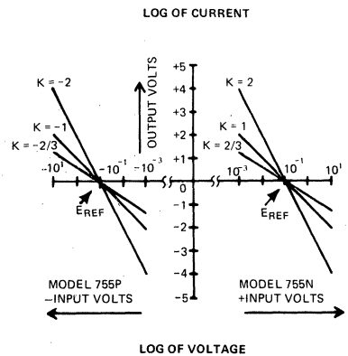
Output vs. Input of Model 755N & 755P in Log Connection (Log Input Scales), Showing Voltages, and Polarity Relationships
