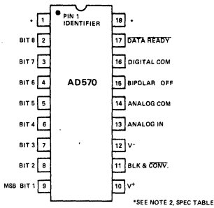
Figure 5. AD570 Pin Connections
