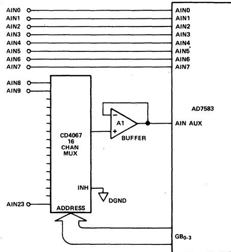
Figure 8. Channel Expansion Scheme
