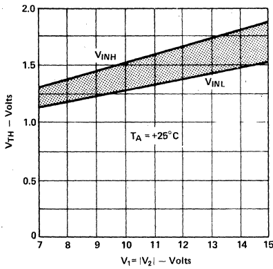
Figure 4. Input Logic Threshold vs. Power Supply Voltage
