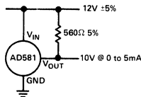
Figure 12. 12 Volt Supply Connection
