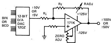
Figure 8. Programmable Power Supply
