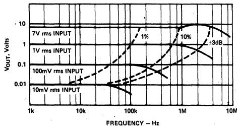
Figure 14. High Frequency Response
