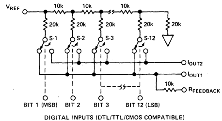
Figure 5. AD7541 Functional Diagram (Inputs "HIGH")
