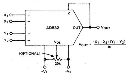
Figure 11. Multiplier Connection
