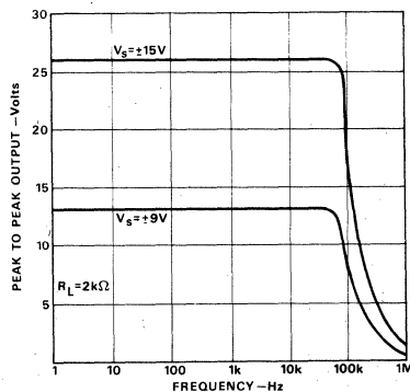
Figure 9. P-P Output vs. Frequency
