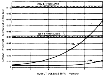
Figure 12. Gain Linearity Error vs. Output Voltage
