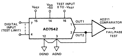
Figure 11. Digitally Programmable Limit Detector
