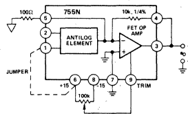
Figure 5. Trimming E_{OS} in Antilog Mode
