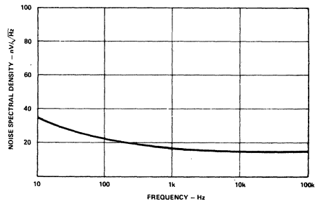
Figure 7. Input Noise Voltage Spectral Density
