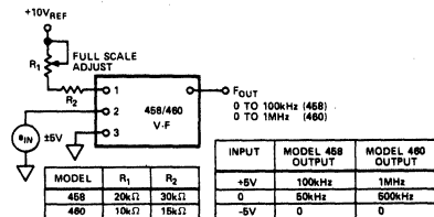
Figure 5. Offsetting Input to Accept ±5V Bipolar Inputs
