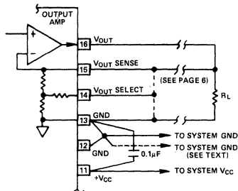
Figure 6. Recommended Grounding and Bypassing
