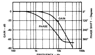
Figure 3. Output Stage Gain and Phase vs. Frequency
