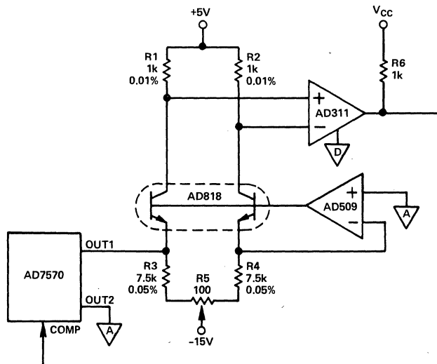
Figure 9. Current Comparator With Low Input Impedance
