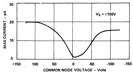
Figure 7. Bias Current vs. CMV for Model 171K
