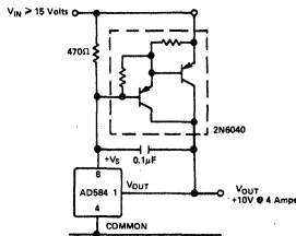
Figure 12. High Current Precision Supply
