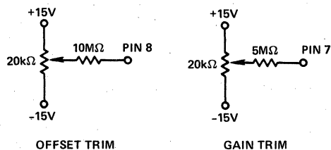
Figure 5. Optional External Trims
