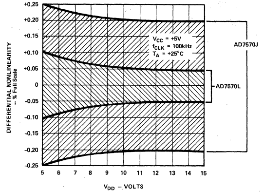
Figure 3. Differential Nonlinearity vs. V_{DD}
