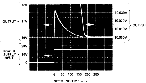
Figure 8a. Output Settling Characteristic
