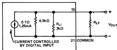
Figure 14. AD DAC80-CCD-1 Connected for Voltage Output with Resistive Load
