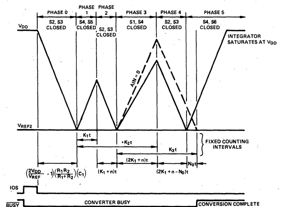
Figure 2. Quad Slope Timing Diagram
