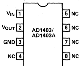
Figure 1. AD1403/AD1403A Connection Diagram
