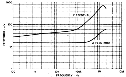
Figure 5. Feedthrough vs. Frequency
