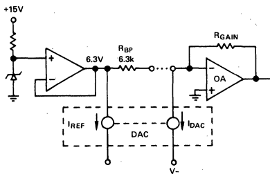
Figure 5. Bipolar Configuration
