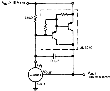
Figure 11. High Current Precision Supply
