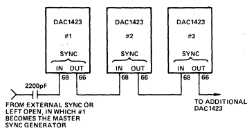
Figure 6. Synchronizing Multiple DAC1423's
