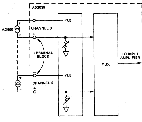
Figure 3. AD2038 Diagram
