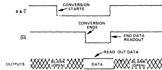
Figure 14. Multiplex Mode
