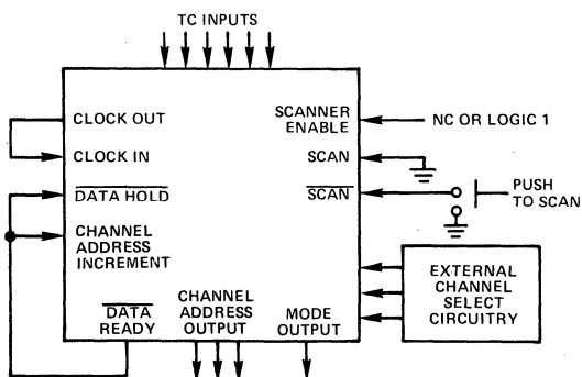
Figure 5. Stand-Alone Operation
