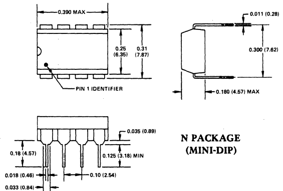
Figure 8. AD1403/1403A Package Specifications (Dimensions shown in inches and (mm))
