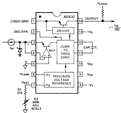
Figure 5. Scale Adjustment for Current Inputs
