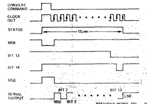
ADC1131 TIMING DIAGRAM
