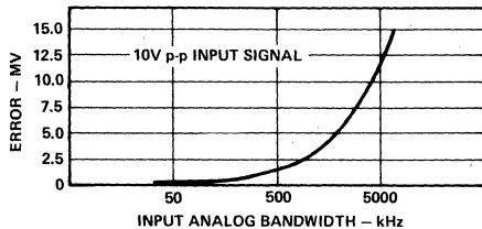
Figure 3. HTC-0300 Error Due to Aperture Uncertainty
