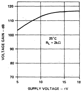
Figure 3. Voltage Gain
