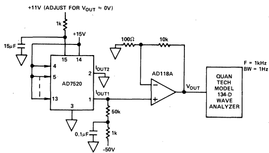
Figure 7. Noise
