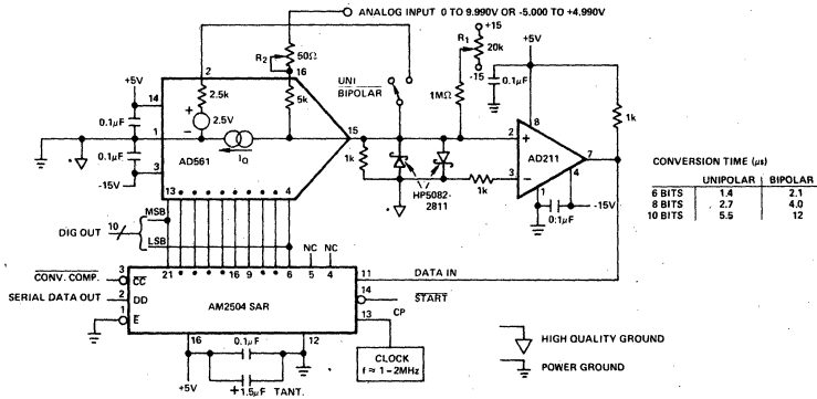
Figure 12. Fast Precision Analog to Digital Converter
