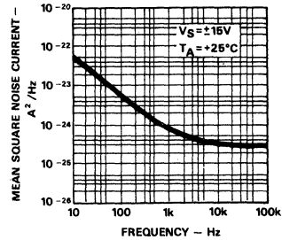
Figure 6. Input Noise Current vs. Frequency
