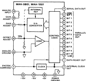
MAH-0801 and MAH-1001 Block Diagram
