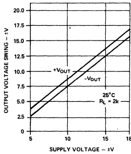
Figure 2. Output Swing
