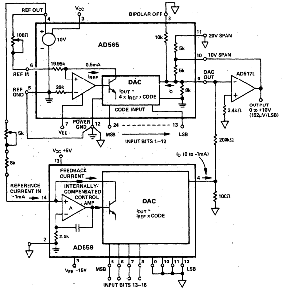
Figure 13. 16-Bit Binary DAC
