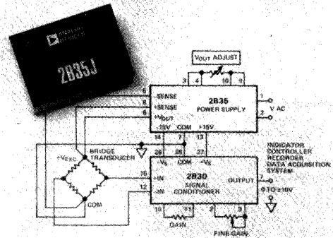
BRIDGE TRANSDUCER SIGNAL CONDITIONING
