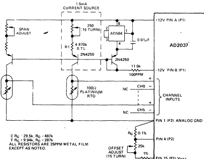
Figure 10. RTD Thermometer
