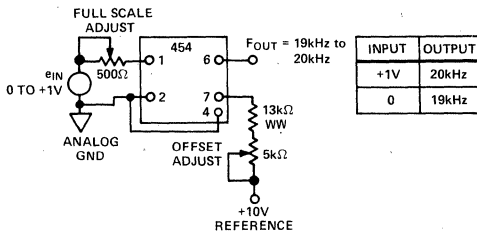
Figure 10. Offsetting Model 454 Output for Improved Dynamic Response
