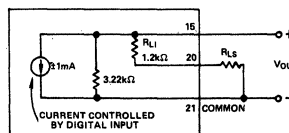
Figure 6b. Bipolar Voltage Output
