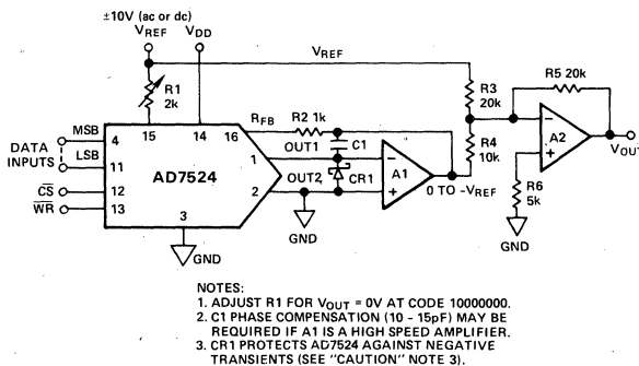
Figure 6. Bipolar (4-Quadrant) Operation
