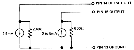
Figure 3. Equivalent Circuit DAC (Unipolar)
