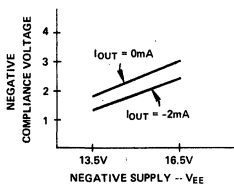
Figure 9. Typical Neg. Compliance Range vs. Neg. Supply
