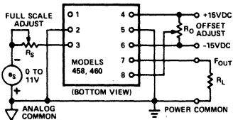
Figure 3. Negative Input Signal
