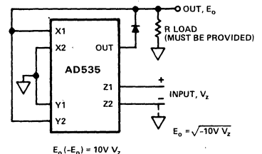
Square Rooter
