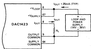
Figure 5. Operation with Common Supply DAC1423
