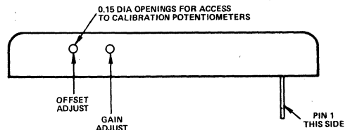
Figure 8. Location of Calibration Potentiometers
