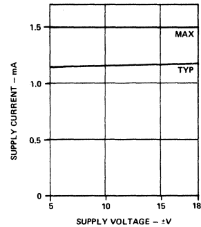
Figure 5. Supply Current
