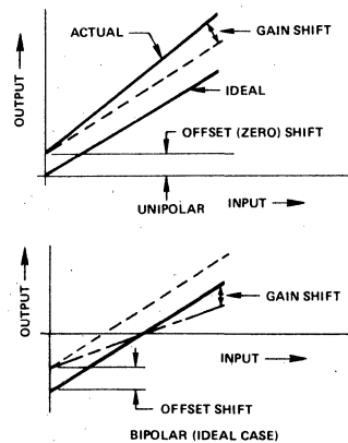
Figure 4. Unipolar and Bipolar Drifts
