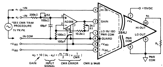
Figure 14. Application of 284J as Instrumentation Amplifier
