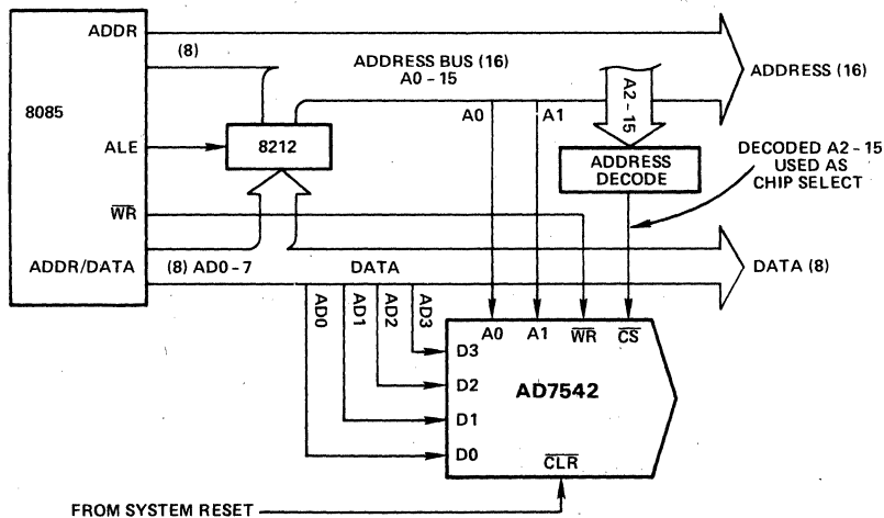
Figure 1. 8085/AD7542 Interface (Memory Mapped Output)
