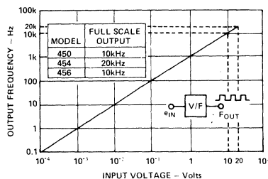
Figure 3. Voltage-to-Frequency Transfer Curve
