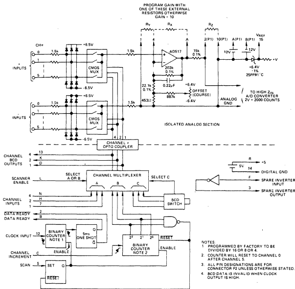
Figure 1. AD2037 Block Diagram
