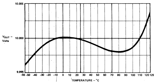
Figure 6. Typical Temperature Characteristic
