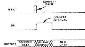
Figure 13. Convert Pulse Mode
