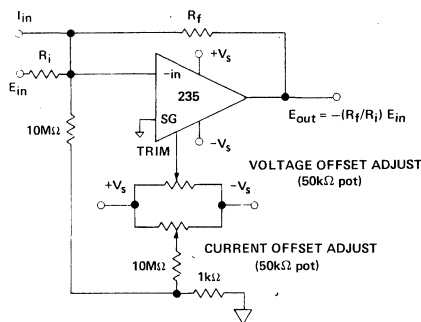
Figure 5. Offset Current Voltage Cancellation
