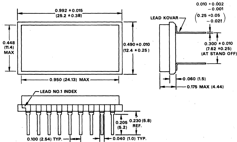
Figure 1. Hermetically-Sealed Ceramic Package Dimensions shown in inches and (mm).
