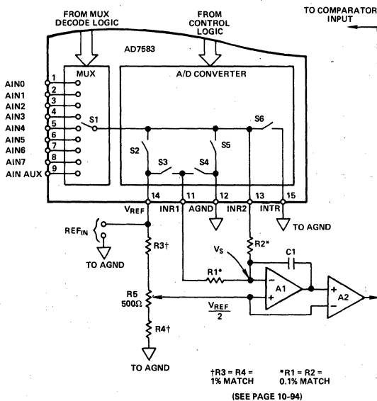
Figure 1. Functional Diagram of AD7583 Analog Circuitry
