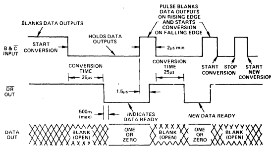
Figure 11. AD570 Timing and Control Sequence
