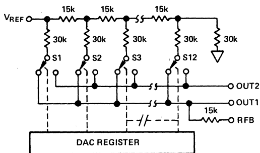
Figure 3. AD7542 Functional Diagram
