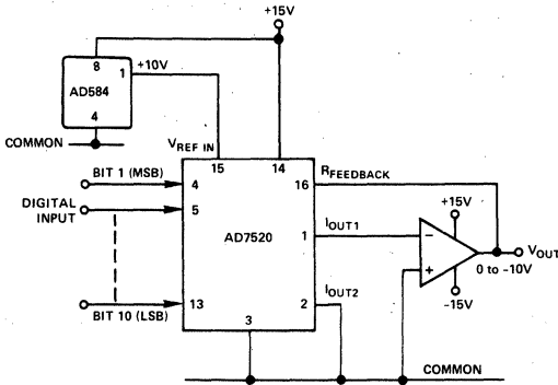
Figure 16. Low Power 10-Bit CMOS DAC Application
