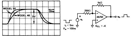
Figure 4. Pulse Response, Model 46/Model 50
