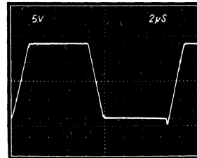
Figure 14b. Unity Gain Inverter Pulse Response
