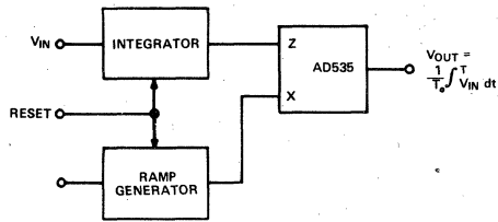
Figure 10. Time Average Computation Circuit
