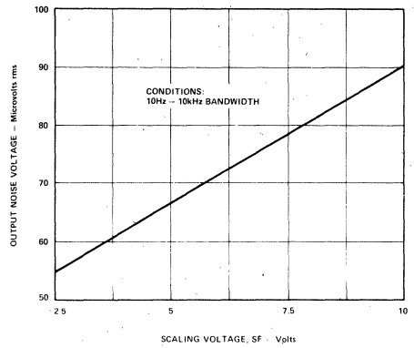
Curve 6. Wideband Noise Vs. Scaling Voltage
