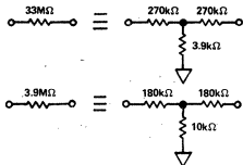
Figure 4. Equivalent Resistances
