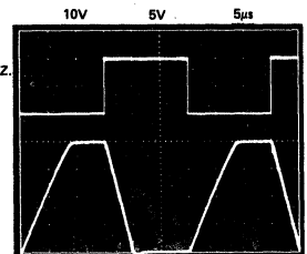
Figure 15b. Voltage Output DAC Settling Characteristic
