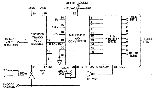
Figure 4. Depicts the MAH-1001-2 A/D Converter Used with the THS-0300 Track-and-Hold
