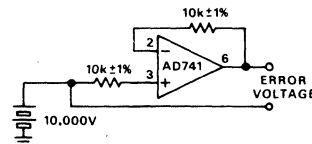
Figure 1. Error Budget Analysis Circuit
