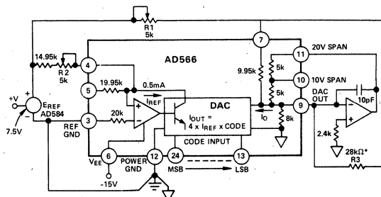
Figure 6. \pm 5\text{V} Bipolar Voltage Output
