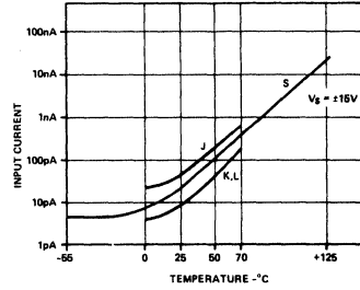
Figure 5. Input Current vs. Temperature
