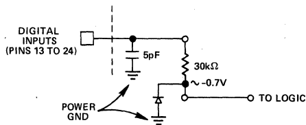
Figure 7. Equivalent Digital Input Circuit
