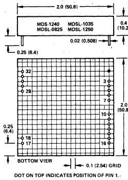
MATING SOCKET MSA-1
