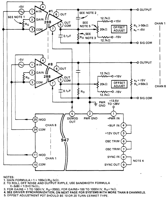
Figure 3. 8-Channel System
