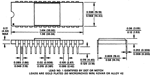
28 Pin Ceramic Dip
