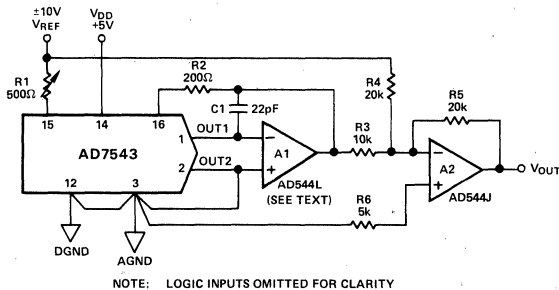
Figure 7. Bipolar Operation (4-Quadrant Multiplication)
