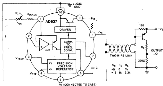
Figure 9. True Two-Wire Operation
