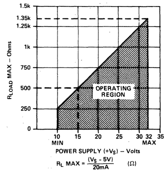
Figure 1. Maximum Load Resistance vs. Power Supply
