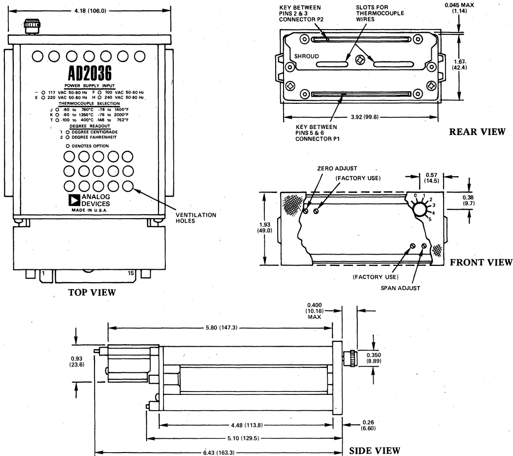
Figure 9. AD2036 Mechanical Outline (Dimensions shown in inches and (mm))
