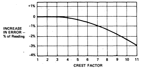
Figure 15. Error vs. Crest Factor
