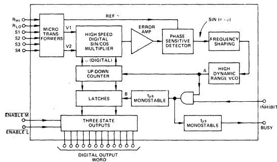
Functional Diagram SDC1741 and SDC1742
