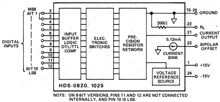
Block Diagram – HDS-0820 and HDS-1025
