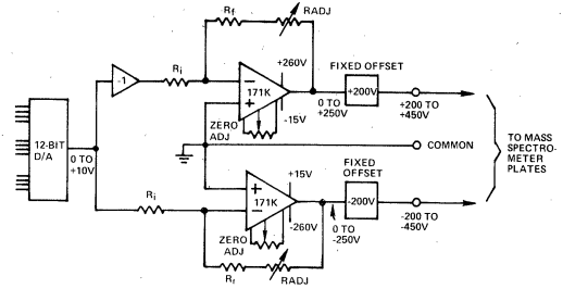
Figure 9. Programmable Mass Spectrometer Voltage Source
