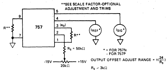
Figure 3. Output Voltage Offset Adjustments
