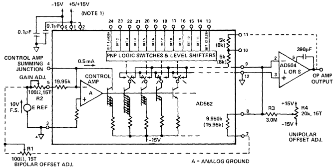
AD562 in Typical Unipolar and Bipolar Connection Scheme
