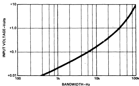
Figure 3. 433 Small Signal Bandwidth vs. Input Voltage
