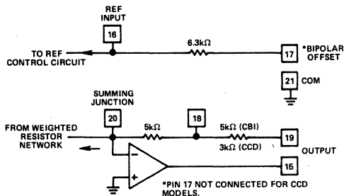
Figure 10. Output Amplifier Voltage Range Scaling Circuit
