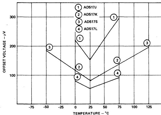
Untrimmed Offset Voltage vs. Temperature
