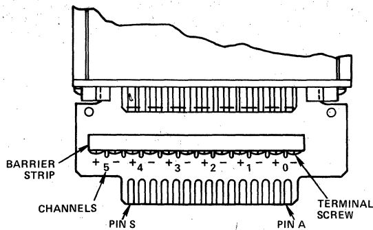
BOTTOM VIEW P2
