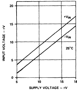
Figure 1. Input Voltage Range
