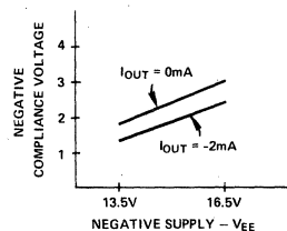
Figure 8. Typical Negative Compliance Range vs. Negative Supply
