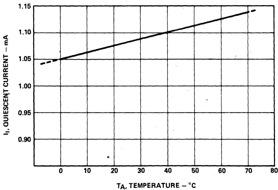
Figure 5. Quiescent Current vs. Temperature ( V_{IN} = 15V , I_{OUT} = 0mA )
