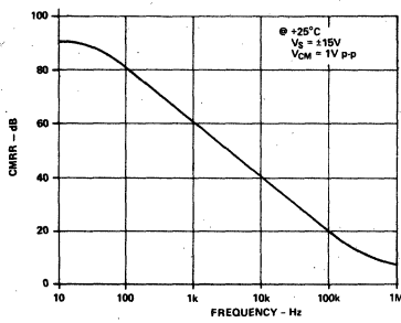
Figure 9. Common Mode Rejection
