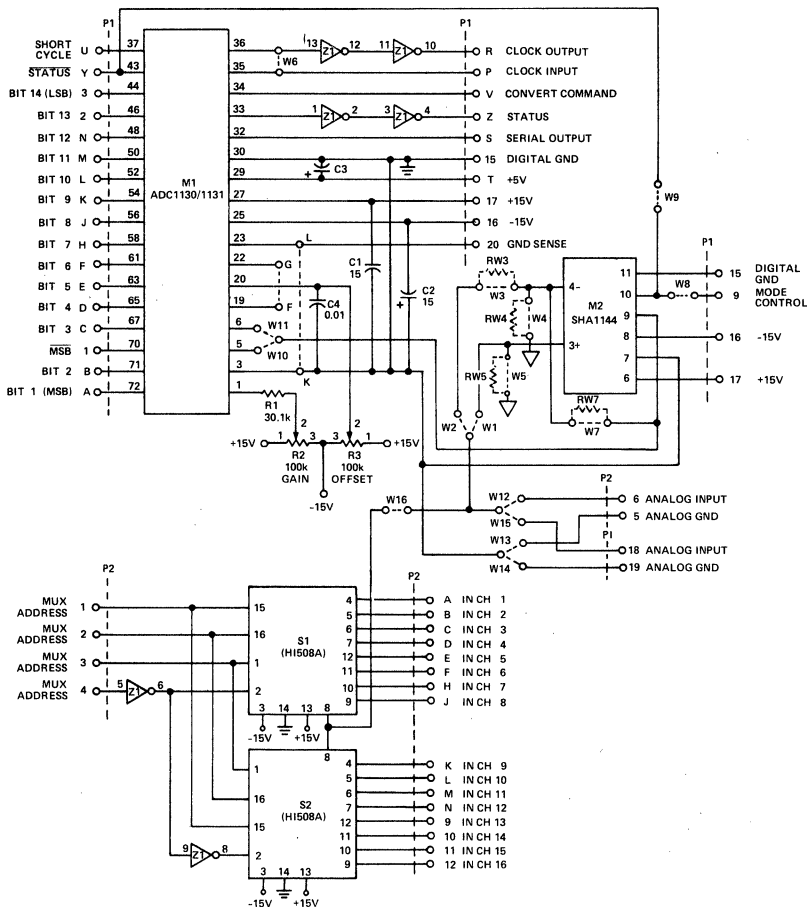
Figure 11. Schematic and Pin Designations
