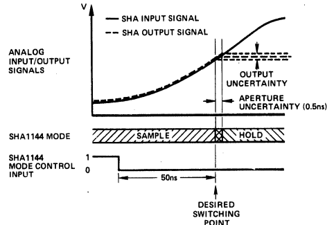
Figure 4. Aperture Uncertainty
