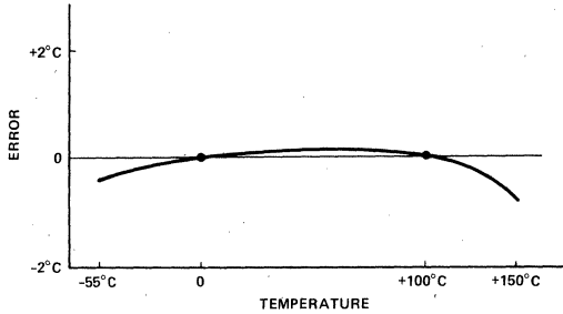
Figure 4. Typical Two-Trim Accuracy (AD590 and 2B57)
