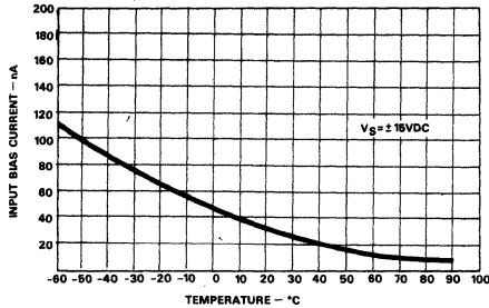
Figure 3. Input Bias Current vs. Temperature
