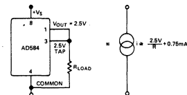
Figure 14. A Two-Component Precision Current Limiter
