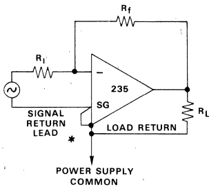
Figure 6. Ground Connection
