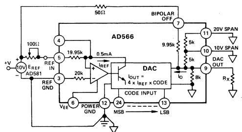
Figure 10. Unbuffered Bipolar Voltage Output
