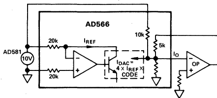
Figure 3. Bipolar Configuration
