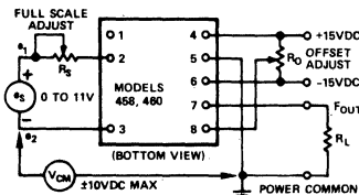
Figure 4. Floating Input Signal
