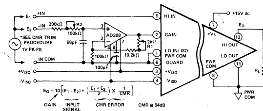
Figure 15. Application of 290A as Instrumentation Amplifier
