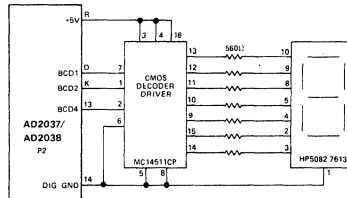
Figure 11. Remote Channel Indicator
