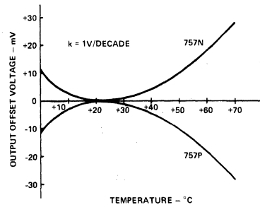
Figure 6. Output Offset Voltage vs. Temperature
