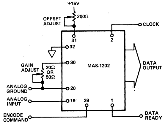
Figure 3. MAS-1202 Unipolar Operation
