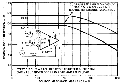
Figure 7. Typical Common Rejection vs. Source Impedance Imbalance
