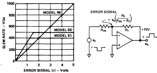
Figure 3. Slew Rate vs. Error Signal
