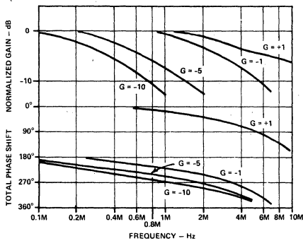
Figure 4. Closed Loop Gain & Phase vs. Frequency
