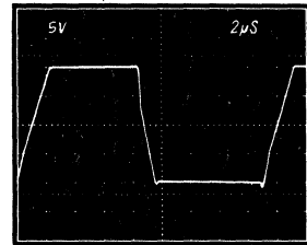
Figure 14a. Unity Gain Follower Pulse Response
