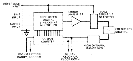
Functional Diagram of the IDC 1703 Tracking Converter
