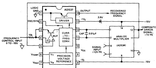
Figure 15. Linear Phase-Locked Loop
