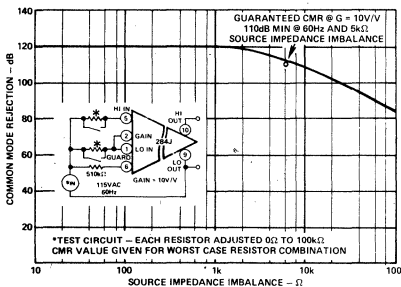
Figure 7. Common Mode Rejection vs. Source Impedance Imbalance
