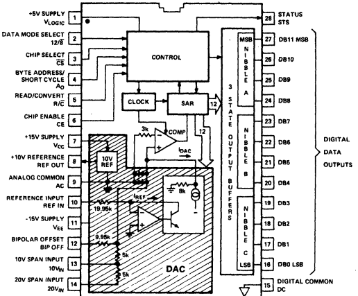
Figure 2. ADC Section Functional Block Diagram and Pinout
