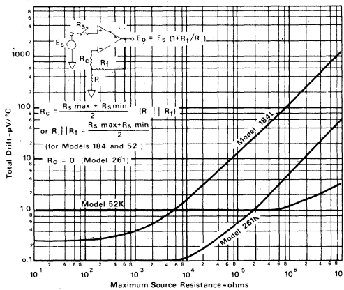
Figure 3. Offset Drift vs. Variable Source Resistance
