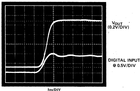
Photo 1. Voltage Output — Positive Going
