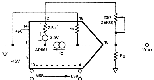
Figure 11. Unbuffered Bipolar Voltage Output
