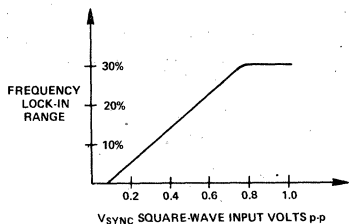
Figure 14. Maximum Frequency Lock-In Range Versus Sync. Signal
