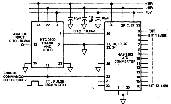
Figure 4. DC to 350kHz, 12-Bit, A/D Conversion System
