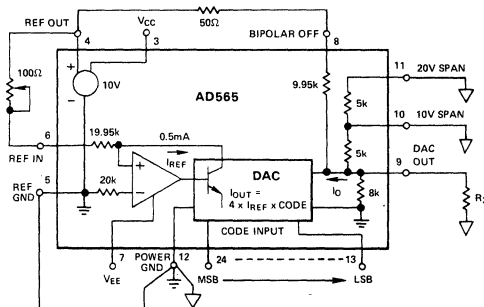
Figure 11. Unbuffered Bipolar Voltage Output
