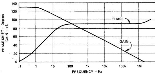
Figure 3. Gain and Phase Shift vs. Frequency
