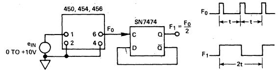
Figure 11. Square Wave Output Using Type D Flip-Flop
