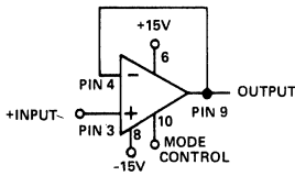
Figure 2. Unity Gain Follower
