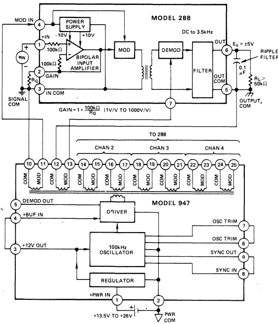
Figure 2. 4-Channel, 3-Port Isolated System
