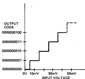
OFFSET CHARACTERISTICS WITH 2.7Ω IN SERIES WITH ANALOG COMMON
