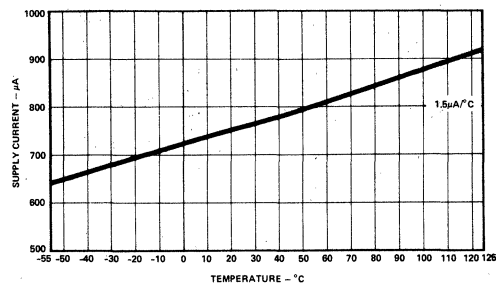
Figure 10. Quiescent Current vs. Temperature
