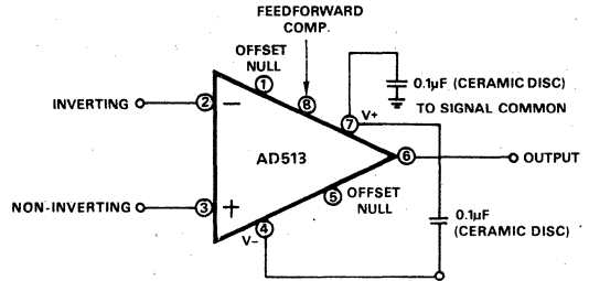
Figure 6. General Purpose Connection Diagram
