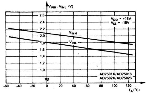
vs. Temperature
