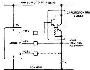
Figure 13. NPN Output Current Booster
