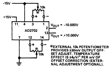
Fine Trim Connections
