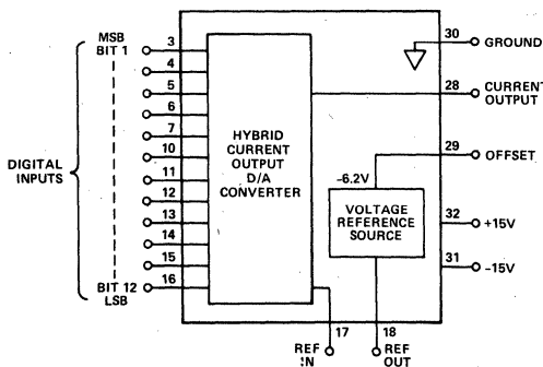
MDS-1240 and MDSL Series Block Diagram
