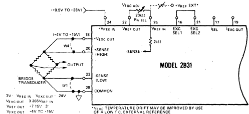
Figure 2. Constant Voltage Excitation Connections
