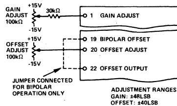
Figure 5. Adjustment Connections
