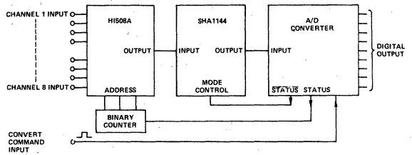
Figure 9. A/D, SHA, and MPX Connections
