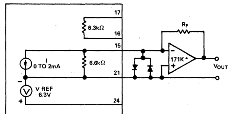
Figure 17. External Op Amp - Using External Feedback Resistors
