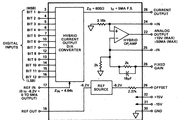
MDH Series Block Diagram
