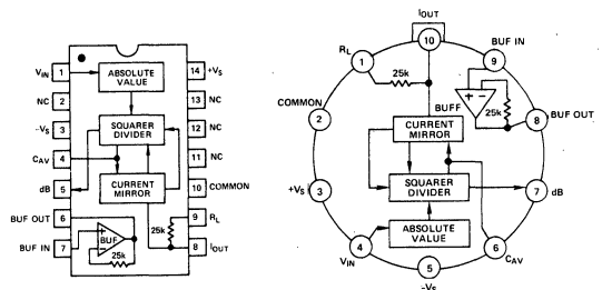
Figure 12. AD536A Pin Connections and Functional Diagram
