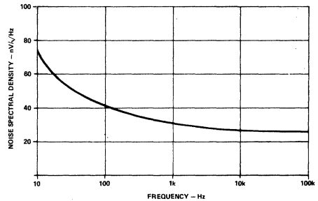
Figure 6. Input Noise Voltage, Spectral Density
