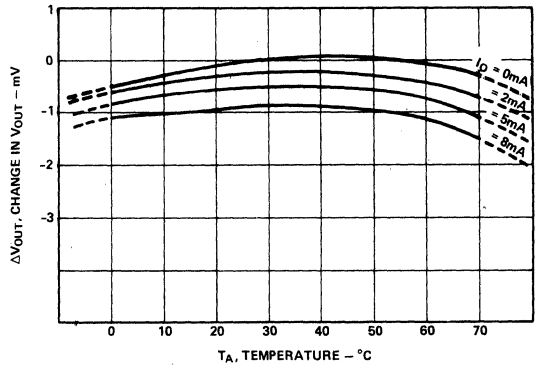
Figure 7. Change in V_{OUT} vs. Temperature (Normalized to V_{OUT} @ V_{IN} = 15V , I_{OUT} = 0mA )
