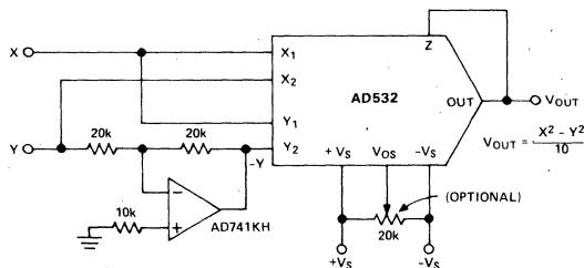
Figure 15. Difference of Squares Connection
