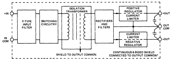
Block Diagram — Models 940, 941, 945, 951 and 953
