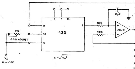
Figure 10. True rms
