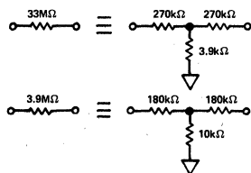
Figure 7. Equivalent Resistances
