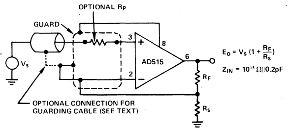
Figure 3. Very High Impedance Non-Inverting Amplifier
