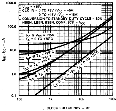
Figure 1. I_{DD} , I_{CC} vs. f_{CLK} at Different Temperatures
