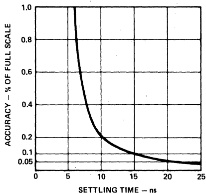
Figure 1. HDS-0810E & HDS-1015E – Accuracy vs. Settling Time
