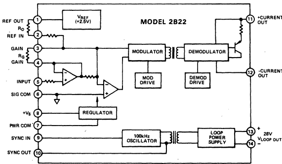
Figure 2. Block Diagram - Model 2B22
