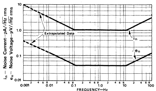
Figure 5B. Spectral Density of Current and Voltage
