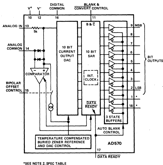
Figure 2. AD570 Functional Block Diagram
