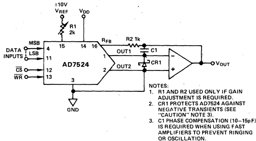
Figure 5. Unipolar Binary Operation (2-Quadrant Multiplication)
