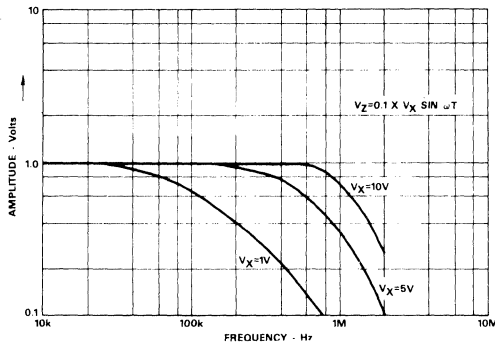
Figure 8. Frequency Response, Dividing
