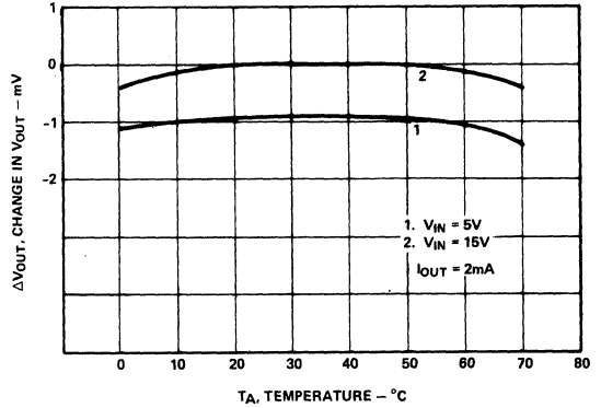
Figure 6. Change in V_{OUT} vs. Temperature (Normalized to V_{OUT} @ V_{IN} = 15V )
