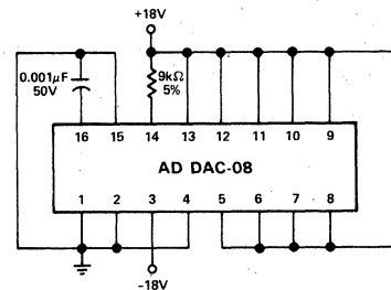
Figure 10. Burn-In Circuit
