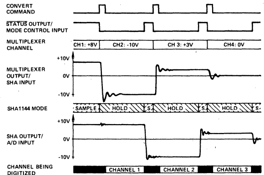
Figure 10. A/D, SHA, and MPX Timing
