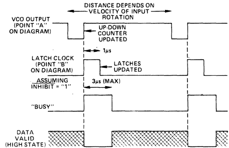
Timing Diagram
