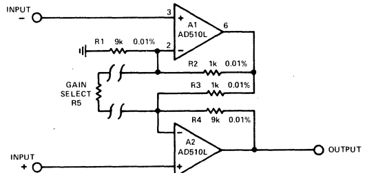
Figure 2. Instrumentation Amplifier
