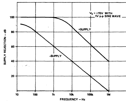
Figure 7. Power Supply Rejection
