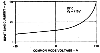
Figure 13. Input Bias Current vs. CMV
