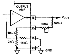
Figure 5. 10.24V Full-Scale Connection
