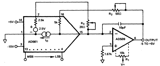
Figure 6. ±5V Buffered Bipolar Voltage Output
