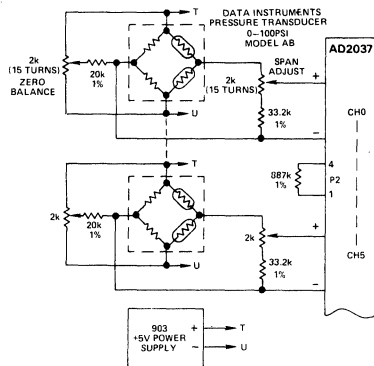
Figure 9. Pressure Meter
