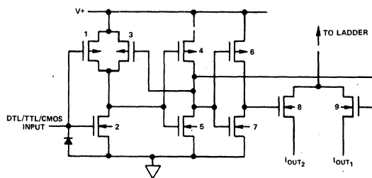
Figure 2. CMOS Switch
