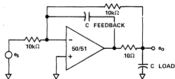
Figure 10. Isolation of Load Capacitance
