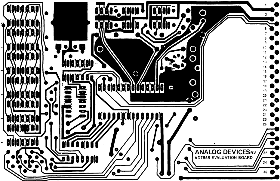
Figure 5a. Component Side
