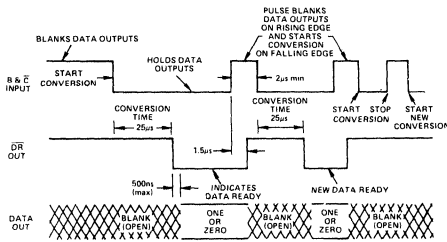
Figure 12. AD571 Timing and Control Sequence
