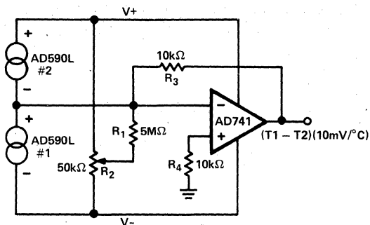
Figure 12. Differential Measurements
