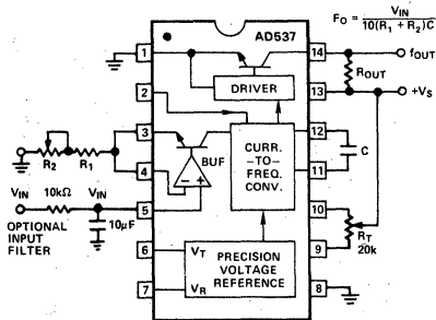
Figure 3. Standard V-F Connection for Positive Input Voltages V-F CONNECTIONS FOR NEGATIVE INPUT VOLTAGE OR CURRENT
