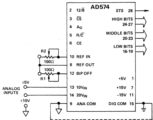
Figure 5. Bipolar Input Connections
