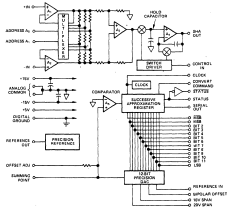
Figure 1. DAS1151 Block Diagram and Pin Designations
