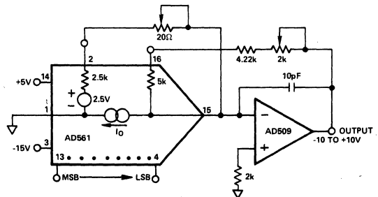
Figure 7. ±10V Buffered Voltage Output
