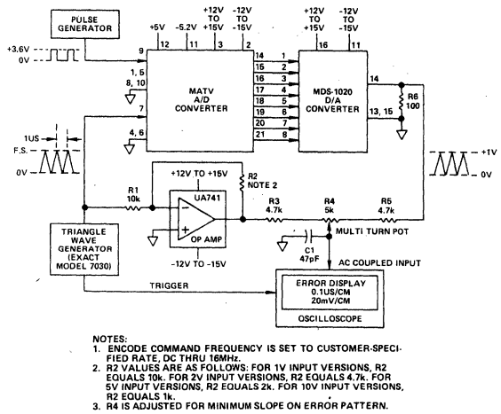
Figure 7. Dynamic Linearity Adjustment Set-Up
