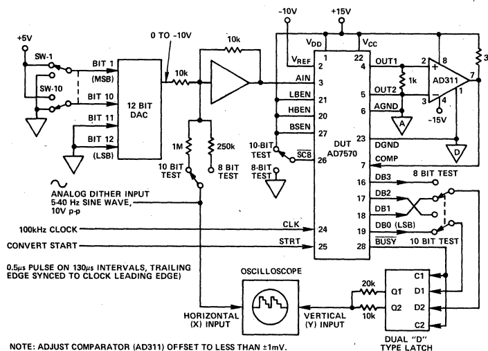
Figure 5. Dynamic Crossplot Accuracy Test
