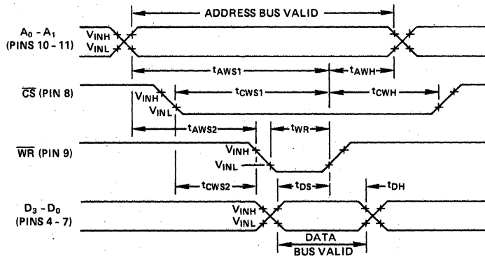
Figure 2. WRITE Cycle Timing Diagram (One 4-Bit Byte)
