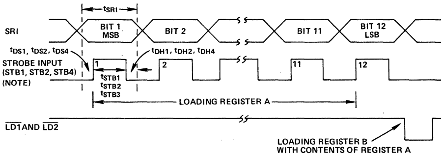
Figure 5. Timing Diagram
