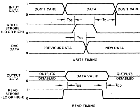
Figure 9. Read/Write Timing
