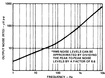
Figure 4. Output Voltage Noise vs. Bandwidth
