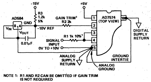
Figure 18. AD584 as Negative 10 Volt Reference for CMOS ADC
