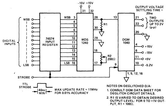
Figure 14. Ultra High-Speed Deglitched D/A
