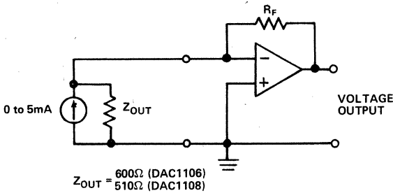
Figure 7. Voltage Output with an Op Amp Simplified Diagram
