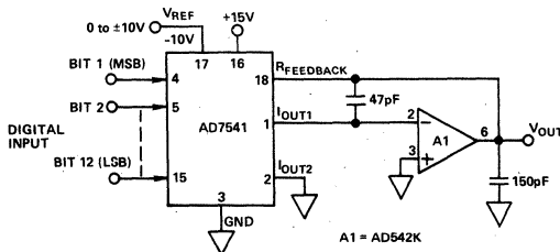
Figure 15a. AD542 Used as DAC Output Amplifier
