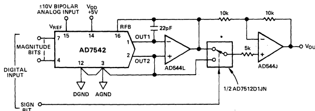
Figure 13. 12-Bit + Sign Multiplying DAC
