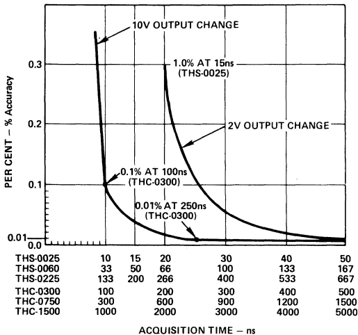
Figure 2. Acquisition Time vs. Settling Accuracy
