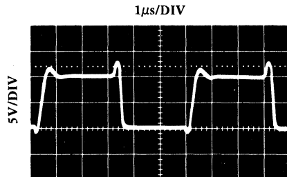
Figure 24. Output Waveform
