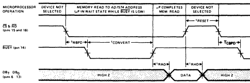
Figure 3. Slow Memory Mode Timing Diagram (CS and RD Tied Together)
