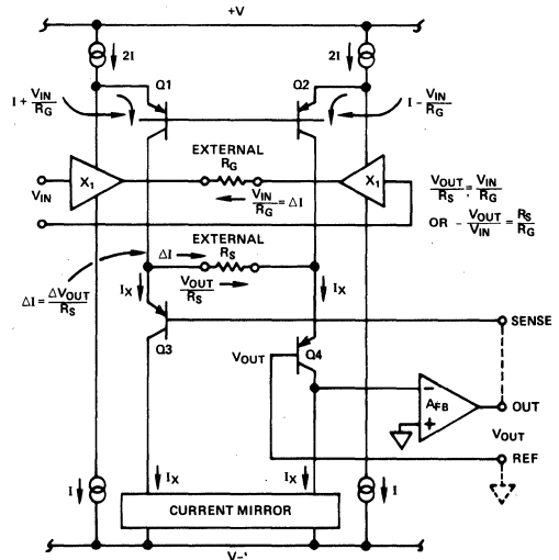
Figure 3. Simplified AD521 Schematic
