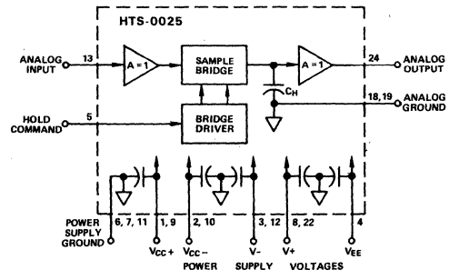
Block Diagram — HTS-0025
