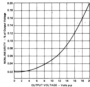
Figure 9. Gain Nonlinearity vs. Output Voltage
