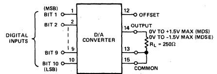
Figure 7. Unipolar Output Current
