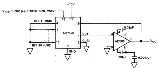
Figure 9. Feedthrough Error
