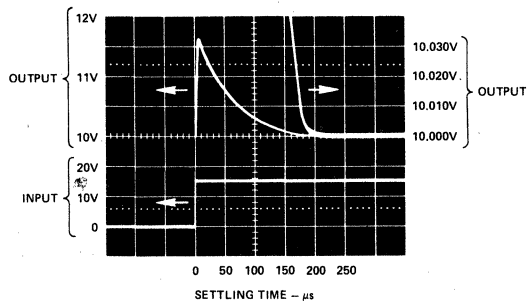
Figure 8. Output Settling Characteristic
