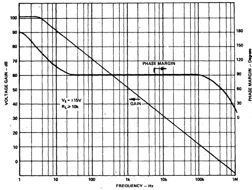
Figure 5. Open Loop Frequency Response
