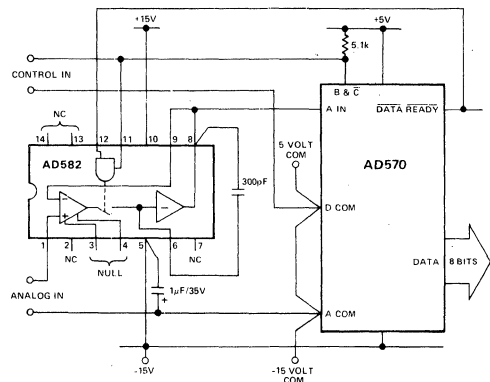
Figure 14. Sample-Hold Interface to the AD570
