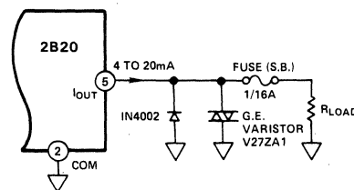
Figure 5. Output Protection Circuitry Connections
