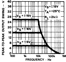
Figure 8. Output Voltage Swing vs. Frequency
