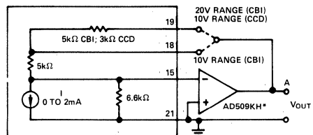
Figure 16. External Op Amp - Using Internal Feedback Resistors
