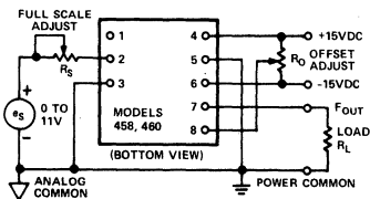
Figure 2. Positive Input Signal
