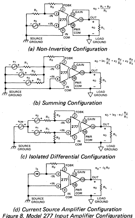
Figure 8. Model 277 Input Amplifier Configurations
