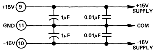
Figure 3. Power Supply Decoupling
