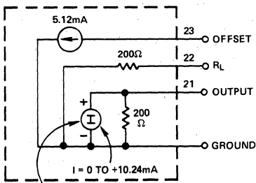
CURRENT CONTROLLED BY DIGITAL INPUT CODE
