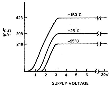
Figure 2. V-I Plot
