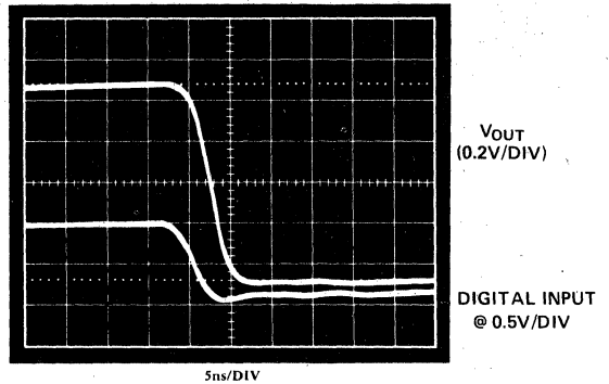
Photo 2. Voltage Output — Negative Going
