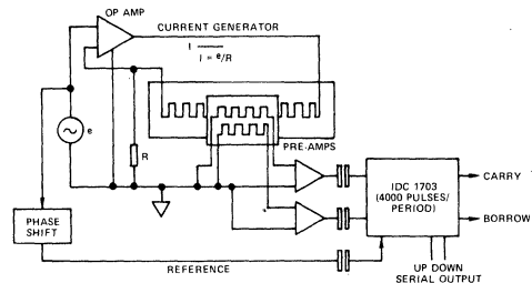
The Inductosyn Used Simulating a Resolver Control TX
