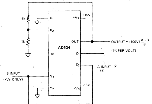
Figure 11. Percentage Computer
