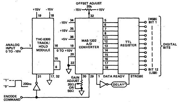
Figure 6. Depicts the MAS-1202 A/D Converter used with the THC-0300 Track-and-Hold
