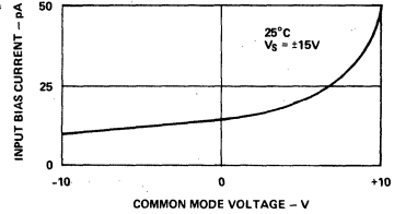
Figure 13. Input Bias Current vs. CMV
