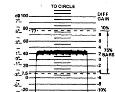
Differential Gain – Generator and Vectorscope Back-to-Back No A/D Conversion
