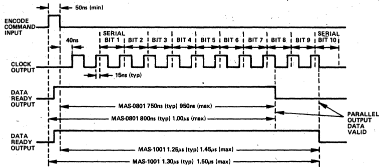
Figure 7. MAS-0801 and MAS-1001 Timing Diagram
