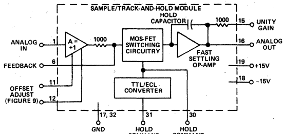
Figure 7. Sample/Track-and-Hold THC Series Block Diagram
