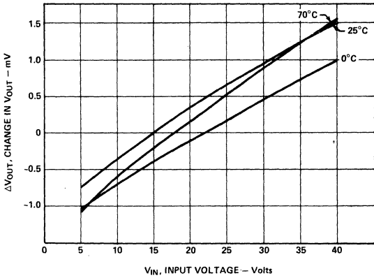
Figure 3. Typical Change in V_{OUT} vs. V_{IN} (Normalized to V_{OUT} @ V_{IN} = 15V @ T_C = 25^\circ C )
