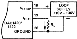
Figure 2. Output/Power Connections
