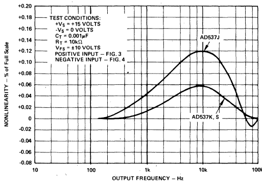
Figure 7b. Typical Nonlinearity Error with 100kHz F.S. Output
