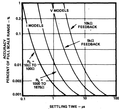
Figure 4. Full Scale Range Settling Time vs. Accuracy
