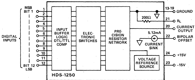
Block Diagram – HDS-1250
