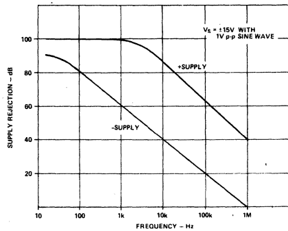
Figure 8. Power Supply Rejection
