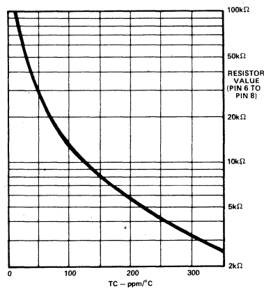
Figure 6. Positive T.C. Induced Versus Correction Resistance
