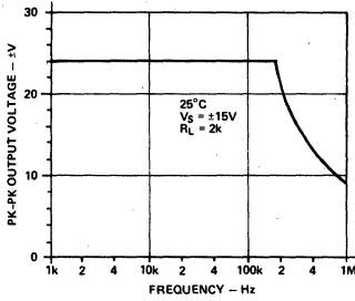
Figure 10. Large Signal Frequency Response
