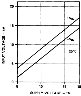
Figure 1. Input Voltage Range
