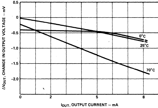
Figure 4. Change in Output Voltage vs. Load Current (Normalized to V_{OUT} @ V_{IN} = 15V , I_{OUT} = 0mA )
