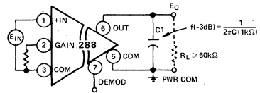
Figure 6a. Selecting Bandwidth with External Capacitor (C)
