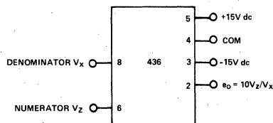
Figure 2. Divide Mode Connections
