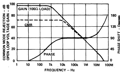
Figure 7. Model 51 Frequency Response
