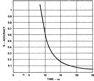
Figure 6. Accuracy vs. Time - MDS and MDSE
