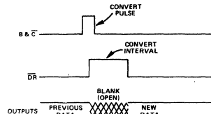
Figure 12. Convert Pulse Mode
