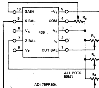
Figure 3. Optional Trim Connections
