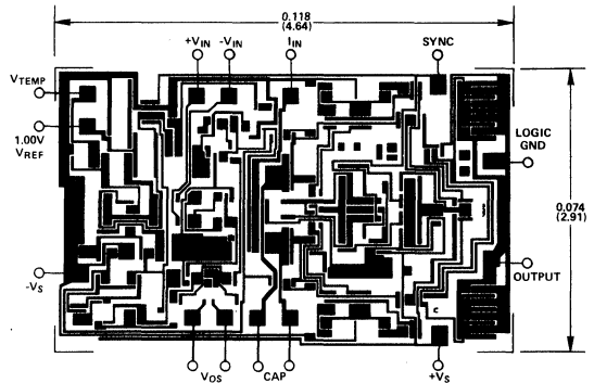
Figure 2. Chip Bonding Diagram
