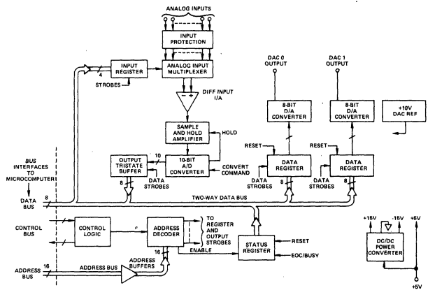
RTI-1225 Block Diagram
