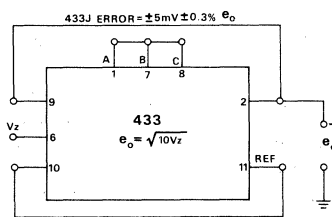
Figure 9. Square Root
