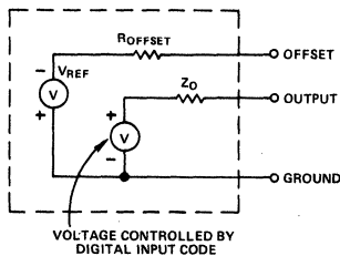
Figure 4. Voltage Equivalent Circuit
