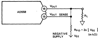
Figure 10. Improved Settling Time
