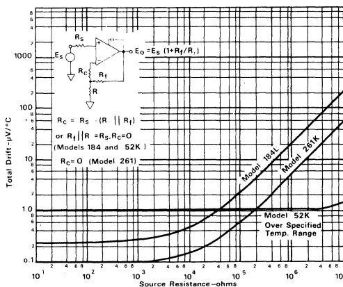
Figure 2. Offset Drift vs. Fixed Source Resistance
