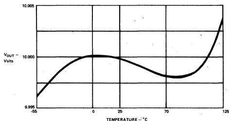
Figure 6. Typical Temperature Characteristic
