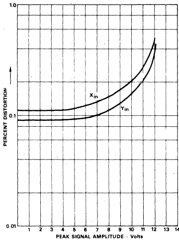
Figure 3. Percent Distortion vs. Input Signal
