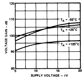
Voltage Gain
