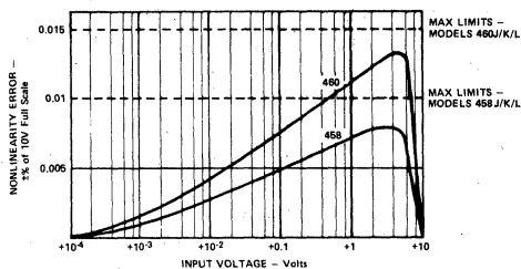
Figure 7. Nonlinearity Error Versus Input Voltage
