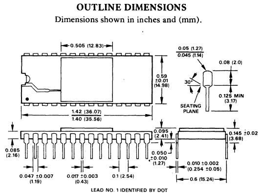
Figure 2. 28 Lead Dual-in-Line Package
