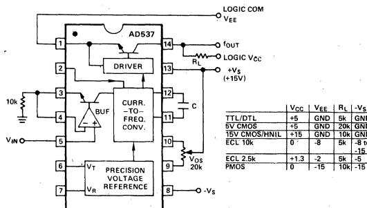
Figure 8. Interfacing Standard Logic Families
