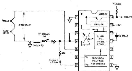
Figure 17. Thermocouple Interface with First-Order Linearization
