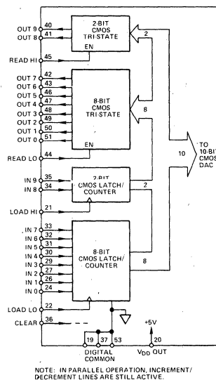
Figure 7. DAC1423 Digital Interface Architecture
