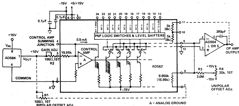
Figure 17. Precision 12-Bit D/A Converter
