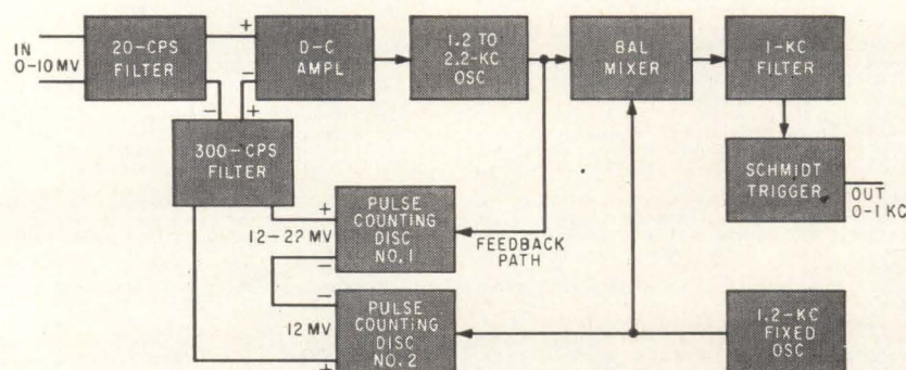
FIG. 1 —With high loop gain, oscillator circuit performance depends on feedback discriminator
