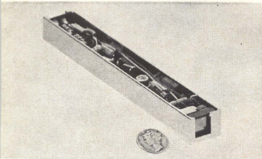
Semiconductor detector with miniature amplifier. These units may be stacked to form array
