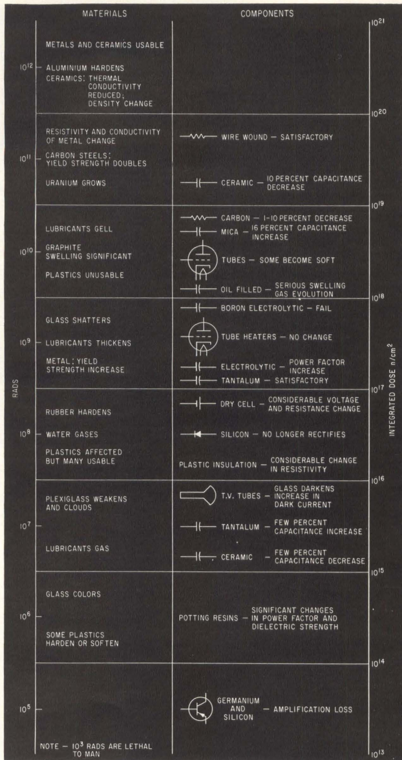
FIG. 5—Radiation damage to materials and electronic components
