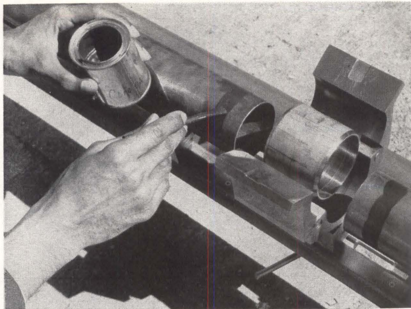
Sealing compound is applied to waveguide sections prior to assembly in grooved stainless steel coupling
