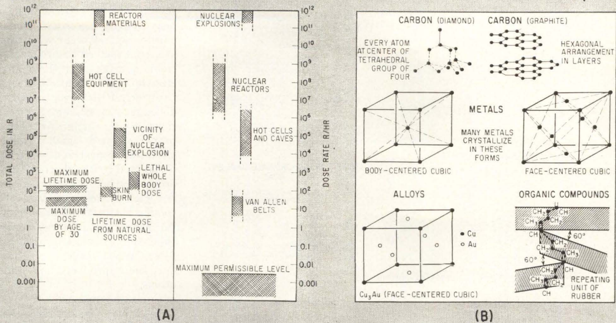
FIG. 1—Comparison of total doses and dose rates (A). Typical structures (B)
