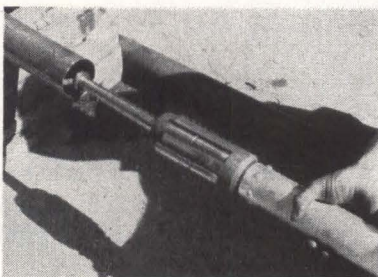
Rolling tool with extension is being inserted into waveguide section
