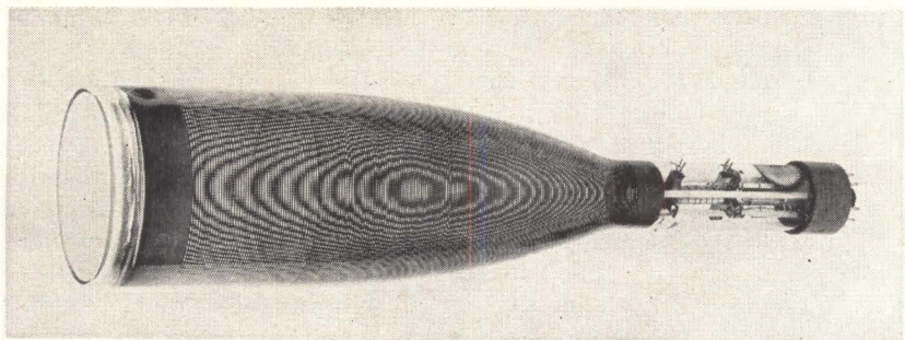
La Radiotechnique 1-Gc crt prototype. Helical post-acceleration gives sensitivity of 30 v/cm horizontal and 10 v/cm vertical
