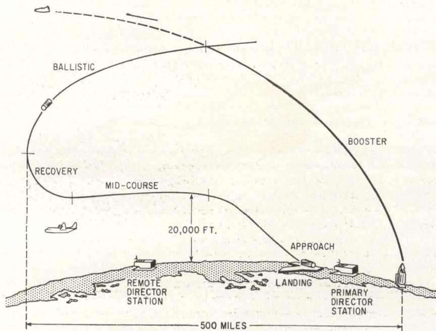
Sperry system may require two ground stations for optimum control
