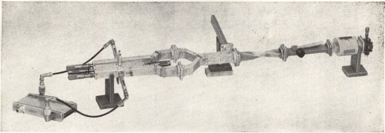
FIG. 2—Varactors are in the waveguide section in the center. The 9,000-Mc klystron is at the right
