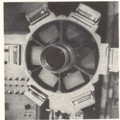
Six Kerr cell shutters and film holders surround central lens
