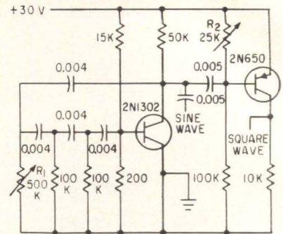
FIG. 2—Phase shift oscillator provides sine-wave and square-wave outputs simultaneously
