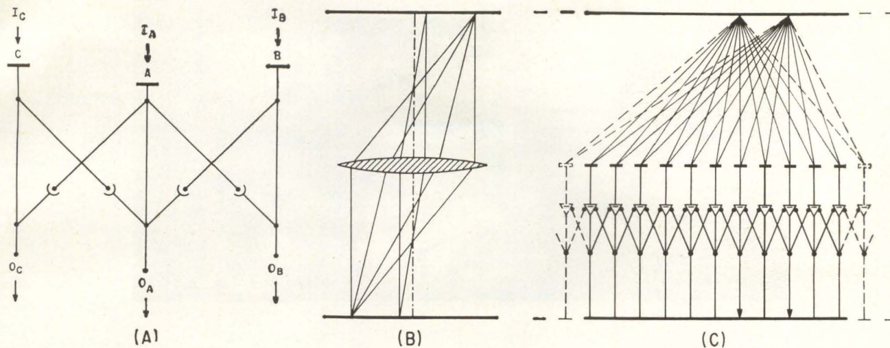
FIG. 5—Mutually inhibitory network is basis for contrast sharpener being developed by GE, Ithaca (A). Diagrams show how two point sources of light are imaged by a lens (B) and by a multifaceted eye in which neural inhibition compensates for diffraction and overlapping field effects (C)
