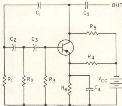
FIG. 1—Three-section R-C network provides required phase shift to obtain positive feedback
