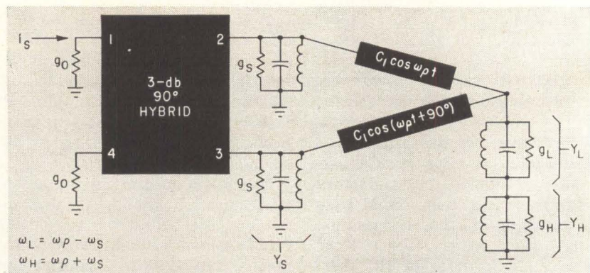
FIG. 1—Power gain in this parametric amplifier circuit is from ports 1 to 4. In the reverse direction, gain is less than unity
