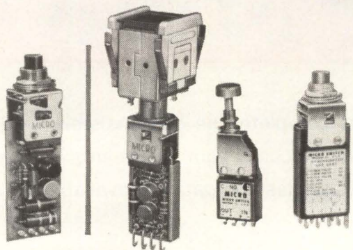
Three additional lines of pulse circuits are available, with or without actuators.
