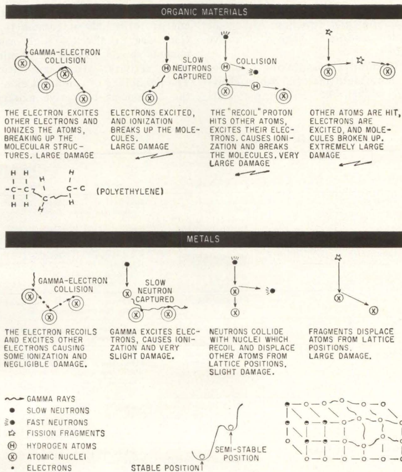
FIG. 3—Radiation damage mechanisms in organics and metals
