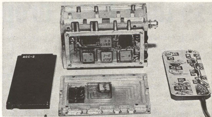
Westinghouse Electric and the Air Force this month showed a molecular circuit version of the AN/ARC-63 emergency communications receiver. It weighs ½-lb, compared to 5 lb for the conventional set. The number of parts was reduced from 219 to 82, including nine functional blocks (mixer-oscillator, three i-f and two a-f amplifiers, audio detector, differential and two-stage a-gc d-c amplifiers)
