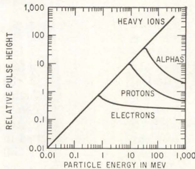
Range of linearity of pulse height vs energy for nuclear particles
