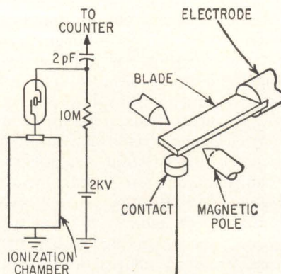
Charge buildup triggers movement of blade in CSF relay, integrating low-level outputs
