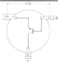
FSP-128 Device similar to 2N1613 Package: TO-51 Corning Glass non-magnetic hard glass package—platinum leads
