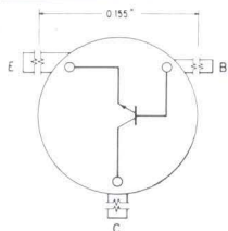
FSP-133 Device similar to 2N914 Package: TO-51 Corning Glass non-magnetic hard glass package—platinum leads
