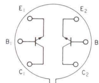
SP-8309—SP-8310 Devices similar to 2N1613 and 2N1711 Package: TO-5 (all leads isolated from header)
