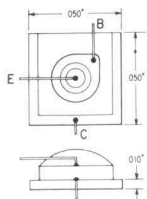
FSP-165 Device similar to 2N914 Package: gold-plated kovar tab 1 mil gold leads
