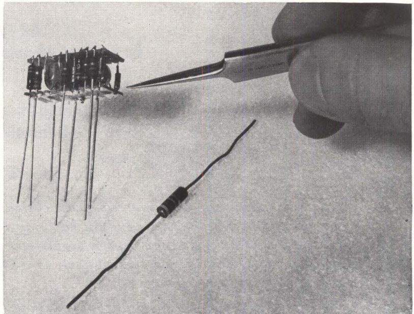
AMPLIFIER circuit for communications equipment uses three new solid tantalum capacitors. One is indicated by tweezers. In foreground is metallized paper capacitor equivalent
