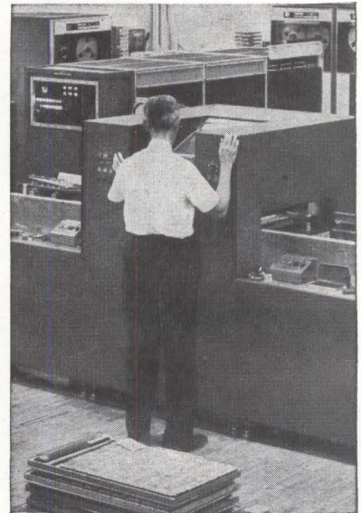
OVERALL checking equipment includes handler unit (in front of operator), data processor and core memory (behind handler unit), tape drives and typewriter
