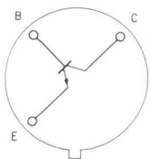
FSP-105 Active Junction: B-E Package: TO-5 photo can
