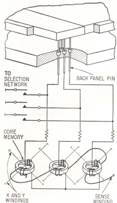
DESTRUCTIVE READOUT checks existence of required connections as indicated when all memory cores contain zeros. If they contain extra bits, extra wires or shorts are indicated
