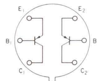
SP-8307 Devices similar to 2N995 Package: TO-5 (all leads isolated from header)
