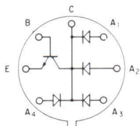
FSP-170 Devices similar to 2N709 and FD-100 Package: TO-5
