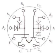
FSP-354-1 Devices similar to 2N1613 and FD300 Package: TO-5 four-island 10-lead header (all leads isolated from header)
