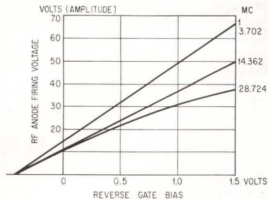
(A) ANODE PROTECTION BY GATE BIAS
