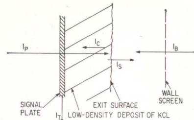
TARGET operation for SEC vidicon is shown schematically
