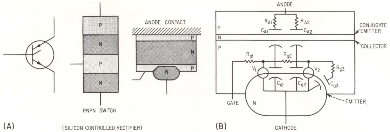
(A) EMITTER or cathode junction, collector junction and conjugate emitter or anode junction of a pnpn switch (A), and r-f equivalent circuit of an unfired controlled rectifier (B)—Fig 1
