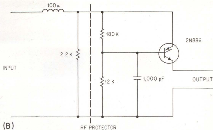
GATE-bias protection of anode (A), and circuit that provides r-f protection (B)—Fig. 3
