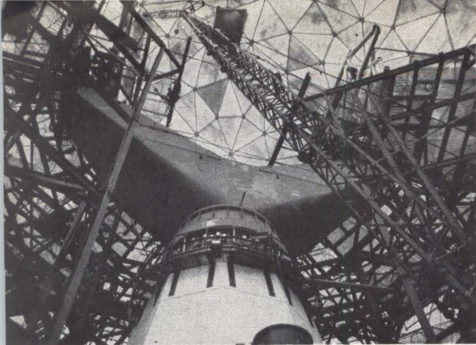
LATEST PHOTO of Haystack antenna being constructed under radome. In an operational orbital scatter system, this facility could provide many voice channels
