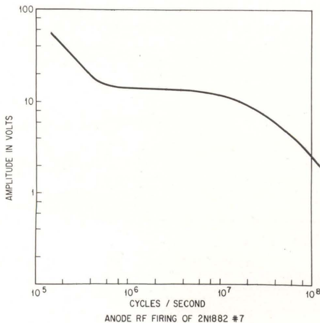
ANODE radio-frequency firing of a 2N1882 rectifier—Fig. 2
