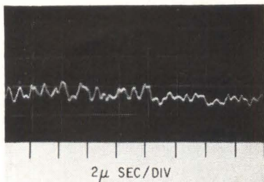
POWER OUTPUT (not signal waveform) of 23-Gc beam-plasma amplifier fluctuates at about 1 Mc—Fig. 3
