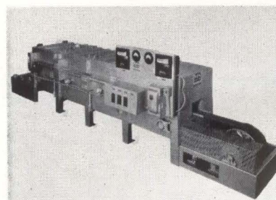
SILVER-FIRING furnace used by National Resistronics in making microcircuit substrates
