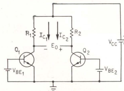
DIFFERENTIAL amplifier achieves low thermal drift by balancing with V_{BE1} = V_{BE2} —Fig. 1
