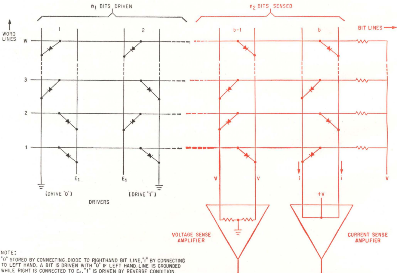
DIODE ARRAY is composed of w word lines and b pairs of bit lines, thus storing w words each b bits long. Sense amplifiers may be either voltage or current amplifiers—Fig. 3
