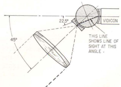
ROTATING fiber optics assembly is mounted in gimbals, with springs moving the ball (center) through half the deflection angle
