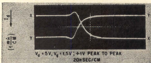
Typical drain current transitions occur in about 30 nsec.
