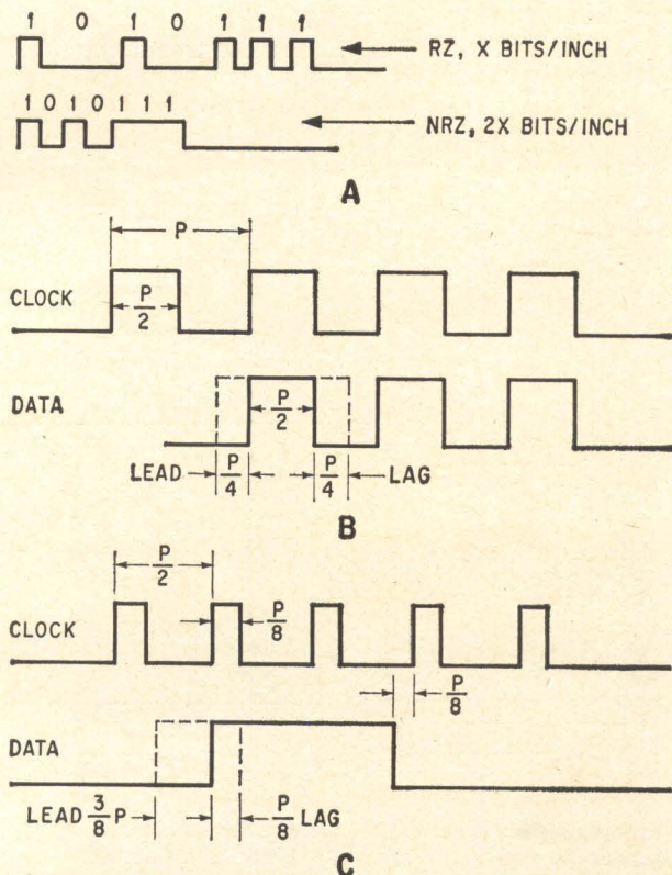
Recording comparisons: data formats (A); tolerable pulse phase error for RZ (B) and NRZ (C) modes.
