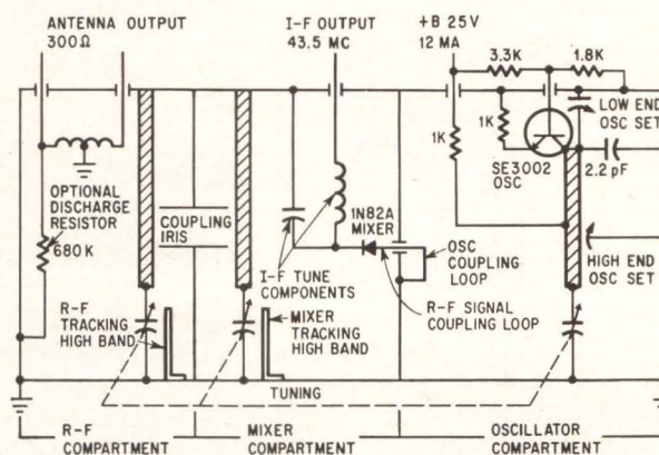
A silicon, point-contact diode mixer and a silicon planar epitaxial transistor oscillator are used in this uhf tuner developed by the Sickles Division.
