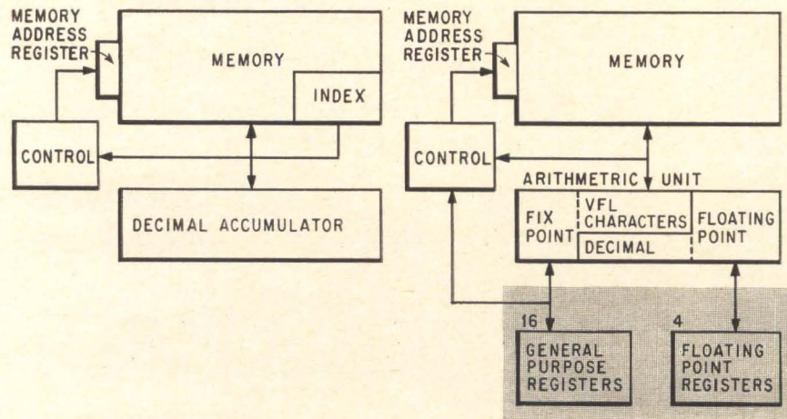
Architecture of new computer system shows the big innovation: the addition of a three-part arithmetic unit connected to general and floating point registers, compared to a former IBM computer.
