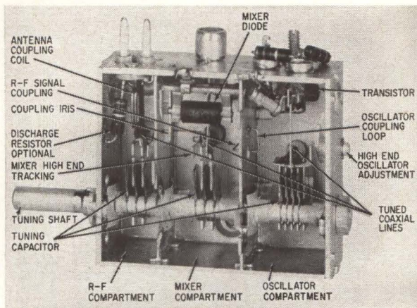
Compact transistor uhf tuner by the Sickles Division of General Instrument Corp. uses capacitance tuning to select stations. Coaxial lines form tuned circuits.
