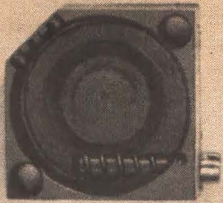
Non-conductive case Non-conductive adjusting screw with metal cap
