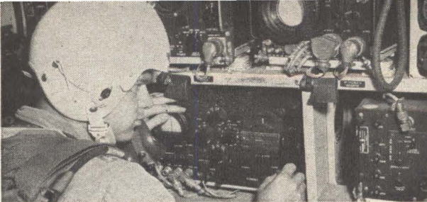
Raven position No. 1 of an RB-66C. The Electronics Warfare Officer is searching for radar signals with an Apr-14 intercept receiver. Next to it is an APR-8B panoramic intercept adapter. Top row of equipment consists of another APR-8B, an ALA-5 pulse analyzer, an ALA-6 direction finder and an aircraft instrument panel. Most of this gear is of late World War II vintage.
