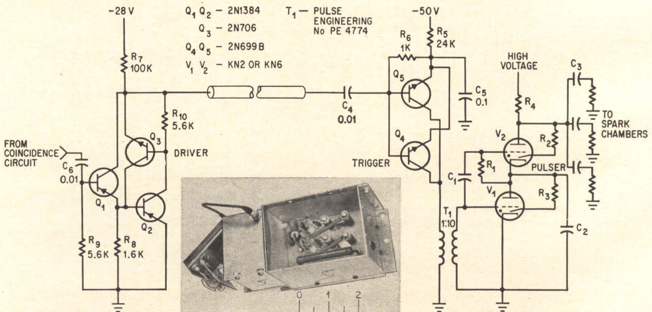
High-voltage pulser. Inset shows construction of trigger circuit attached to the side of the spark-chamber pulser. One side of the aluminum box for pulser circuit is made of Rexolite upon which are mounted the pulser components.
