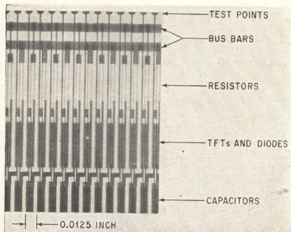
Enlarged portion of thin-film scan generator.
