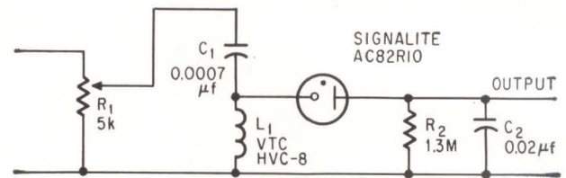
Square-wave voltage, developed across L_1C_1 , breaks down neon tube and provides current to resistor R_2 , charging capacitor C_2 until accumulated charge breaks down the tube in the opposite direction.
