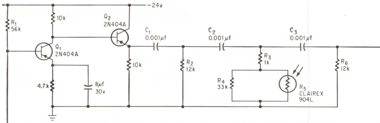
Variable frequency , phase-shift oscillator is controlled by light-sensitive resistor R 5 . Emitter follower Q 2 makes circuit more sensitive to resistance changes than a conventional phase-shift oscillator.
