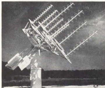
TELEMETRY ANTENNAS
