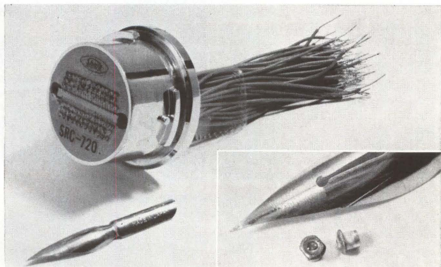
Character-recognition sensor has two rows of 36-cells on a single silicon wafer about \frac{3}{4} -inch long. Light output of tiny GaAs diodes closely matches sensor's response.
