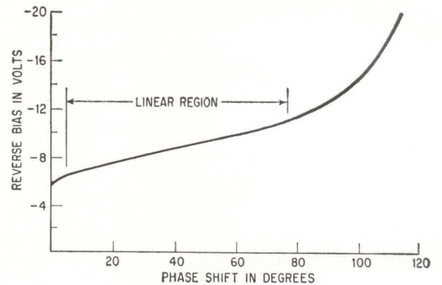
Resistance of zener diode D_1 remains linear during nearly 80^\circ of phase shift. The slope of the linear portion indicates that phase-shift selectively is 15^\circ per volt.
