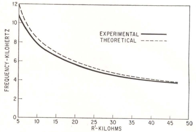
Frequency variation is plotted as a function of R' , the resistance of the shunt leg which is a combination of R_3 , R_4 and R_5 . Discrepancy between experimental and theoretical curves results from assuming zero input impedance for Q_1 .
