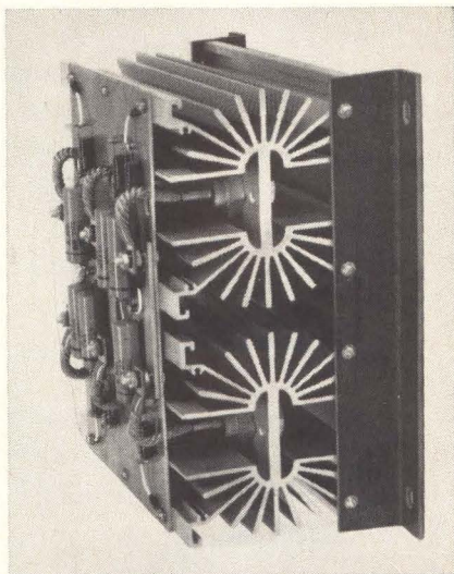
Typical Tung-Sol high current silicon rectifier stack assembly.
