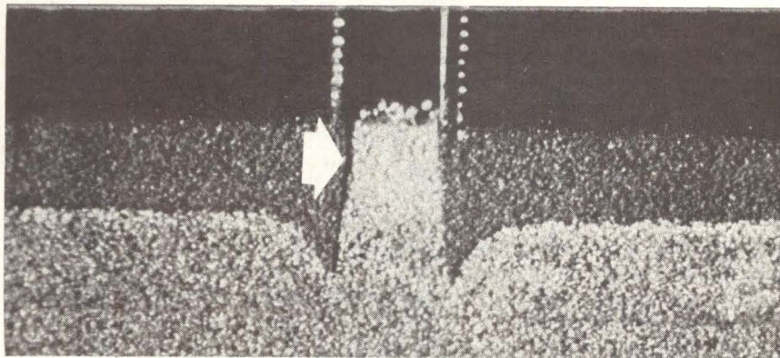
Active region. Planar Gunn diode structure has an active region in the form of stripes, as shown in cross section (above). Dark layers are the electrodes—tin-doped N^{++} regions. Photolithographic techniques are used to delineate the active region, which can be from 3 to 27 microns wide.
