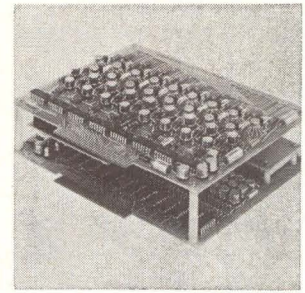
Plug-in random access core memory system FI-23 has capacities of 80 or 160 words with up to 17 bits per word. With a 2 \mu sec access time, this 8 \mu sec full cycle system incorporates the newest DTL semiconductors for logic, sense, timing and interface circuits. Power required is +5 v at 3 amps max. -5 v at 0.6 amp max. Ferrocube Corp., Englewood, Colo. [424]
