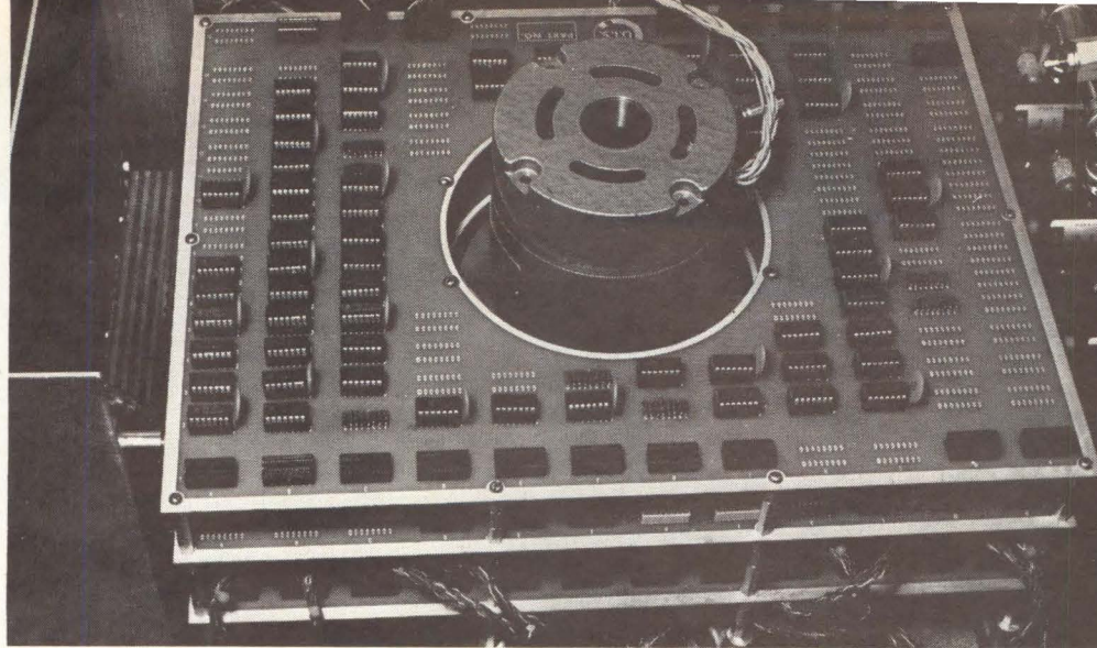
Three layers. All electronic components are mounted on three 12-by-16-inch printed-circuit boards. Two boards carry the electronics common to all machines; the top board is tailor-made for a particular computer. Large center holes permit all three boards to fit over the housing for the floating piston and shaft.
