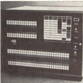
Data concentrator ADS-660 can multiplex up to 45 or more remote terminals over a single telephone line. A key feature is its ability to intermix up to 3 baud rates simultaneously. Channel capacity is determined by the baud rate speeds of the terminal devices used and the transmission line of the telephone line modems. American Data Systems, Chatsworth, Calif. [425]
