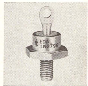
Silicon power rectifiers come in stud mounted DO-5 packages. A double diffused, passivated junction technique assures stable electrical characteristics. Both standard and bulk avalanche types in voltage ratings from 50 to 1,000 piv are available. The F3, F4 and F5 series offer max. forward current of 31, 37 and 50 amps, respectively. Edal Industries Inc., East Haven, Conn. [439]
