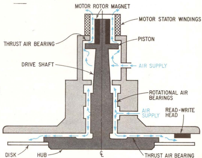
Anti-wobble. The undesirable motions that can occur with ball bearings (left) are avoided in the DDR-1 with air bearings, shown at right. The shaft spins in a rotational bearing, and the hub and piston bear upward against thrust bearings, all films of air under pressure.
