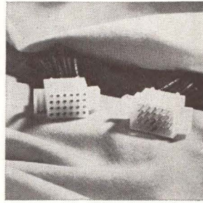
Miniature connector 1625-24 is a 24-circuit device having a nylon body with integrally molded mounting ears on both plug and receptacle. It accepts crimp-type terminals available in tin-plated brass, phosphorous bronze, and gold or silver-plated brass. The connector has applications in business machines and computers. Molex Products Co., Katrine Ave., Downers Grove, Ill. [348]
