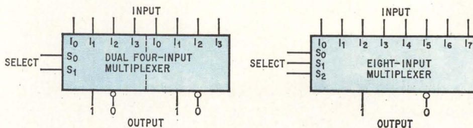
Anything goes. Dual, four-input multiplexer, left, and eight-input unit, right, are used as universal logic circuits. Binary signals on the select lines determine which input line is tied to the output.
