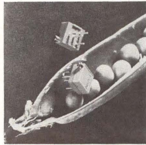
Center-tap ¾-inch trimmer potentiometer model 75SCT features resistance values from 100 ohms to 20 kilohms and stand-offs for easy board washing. Its diallyl phthalate case is impervious to all normal cleaning solvents. An "O" ring seals the adjustment shaft to protect internal parts against severe environments. Techno-Components, 7803 Leona Ave., Van Nuys, Calif. [347]
