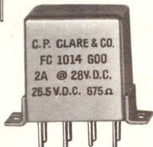
Type FC. Full size; low-level to 2 amp.
