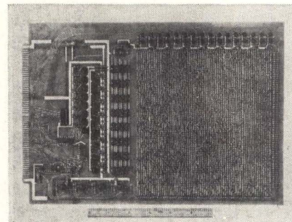
Microprogramed. Memory card, bottom photo, carries diodes that perform microprogramming in the 812. Diodes take up right half of card.
