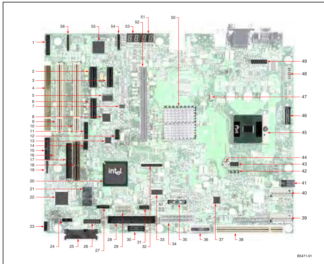
Figure 2. Intel® 945GM Express Chipset Component Locations
