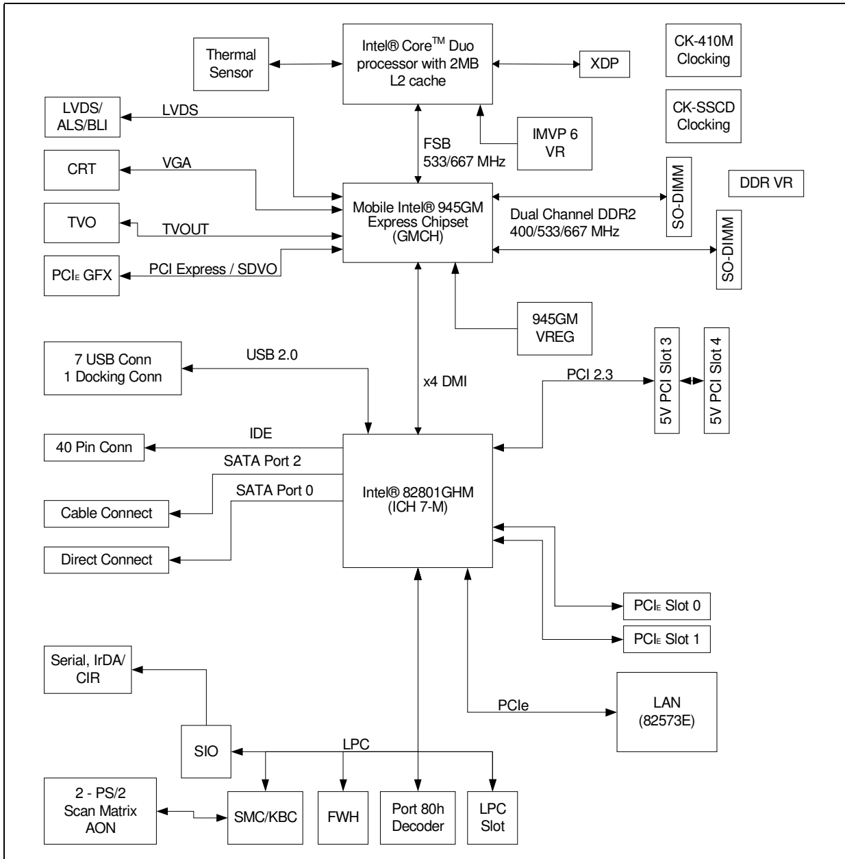
Figure 1. Intel® 945GM Express Chipset Development Kit Block Diagram
