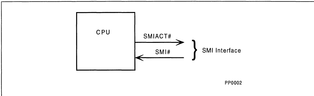
Figure 14-2. Basic SMI# Hardware Interface
