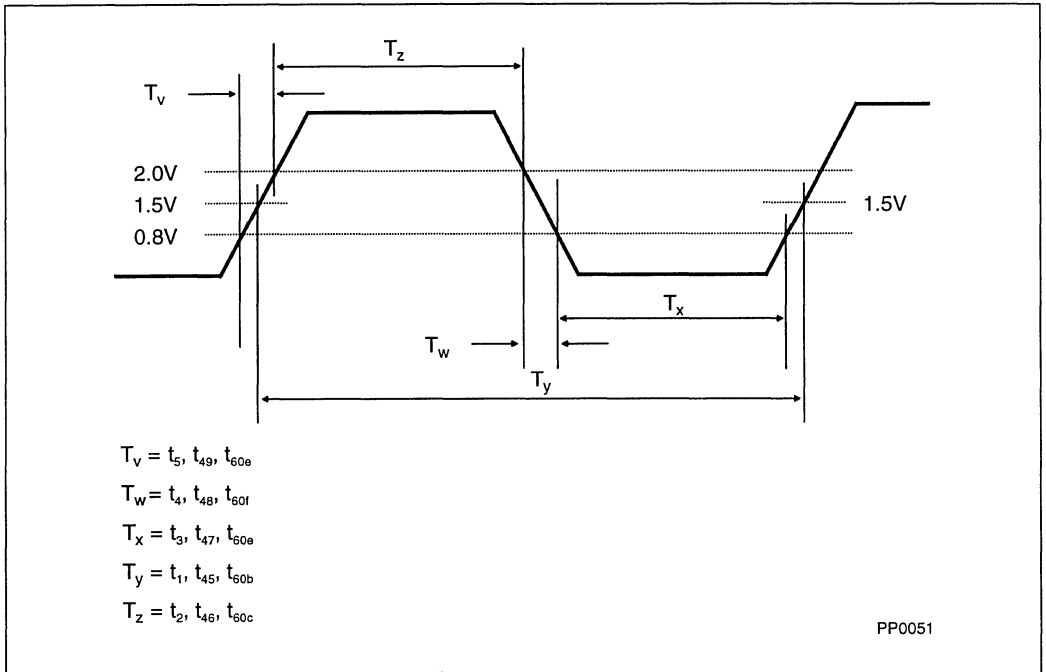
Figure 23-1. Clock Waveform
