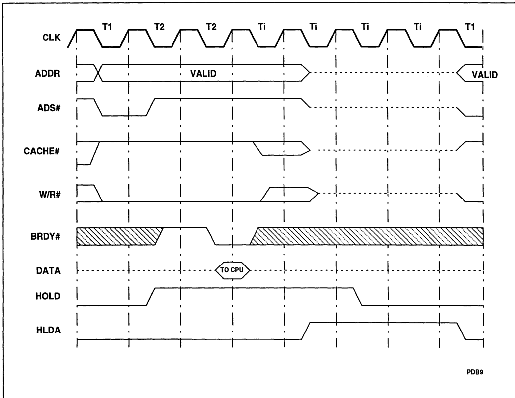
Figure 6-15. HOLD/HLDA Cycles
