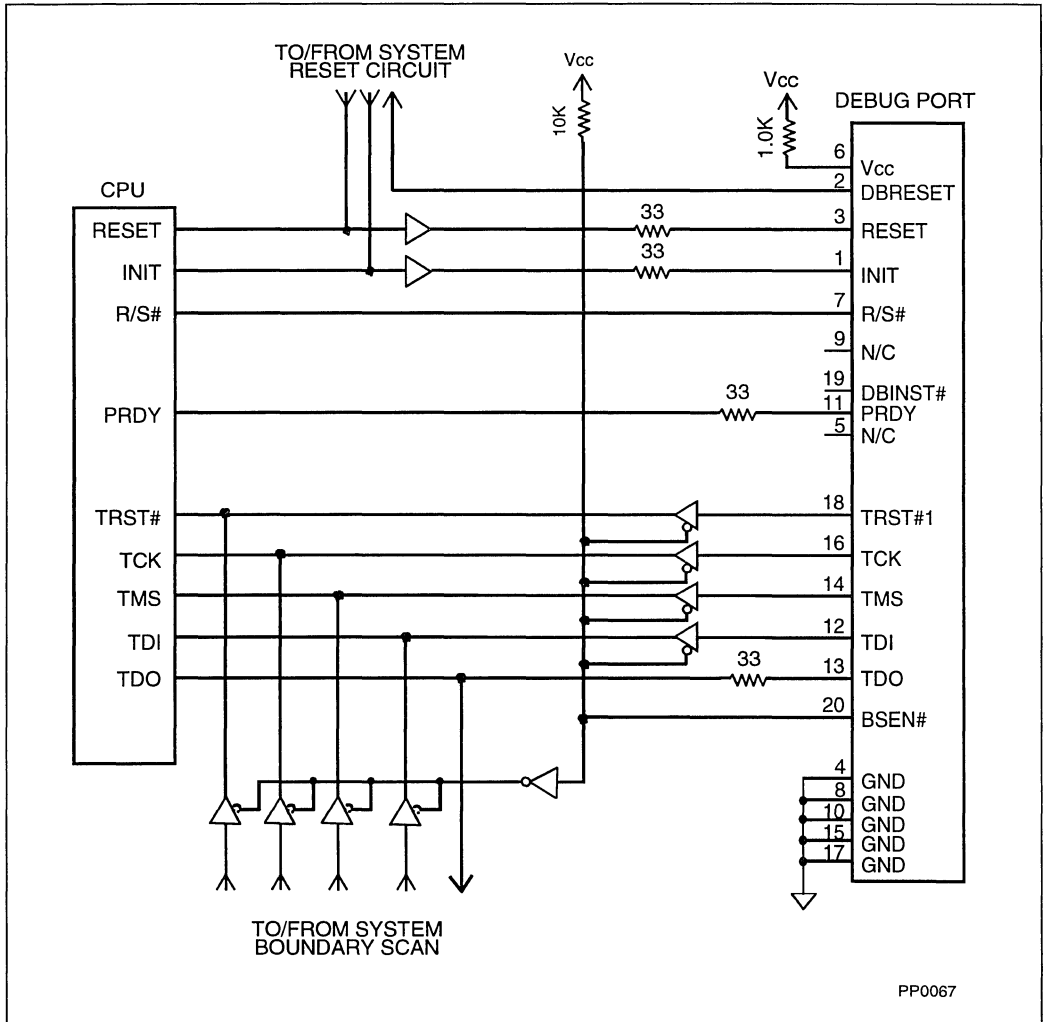
Figure 31-3. Single CPU — Boundary Scan Used
