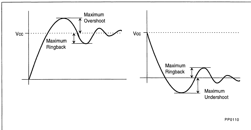
Figure 24-4. Overshoot/Undershoot and Ringback Guidelines
