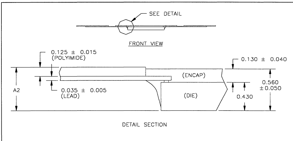
Figure 34-5. One TCP Site (Cross-Sectional Detail)
