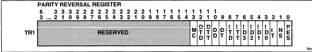
Figure 33-5. Parity Reversal Register (TR1)
