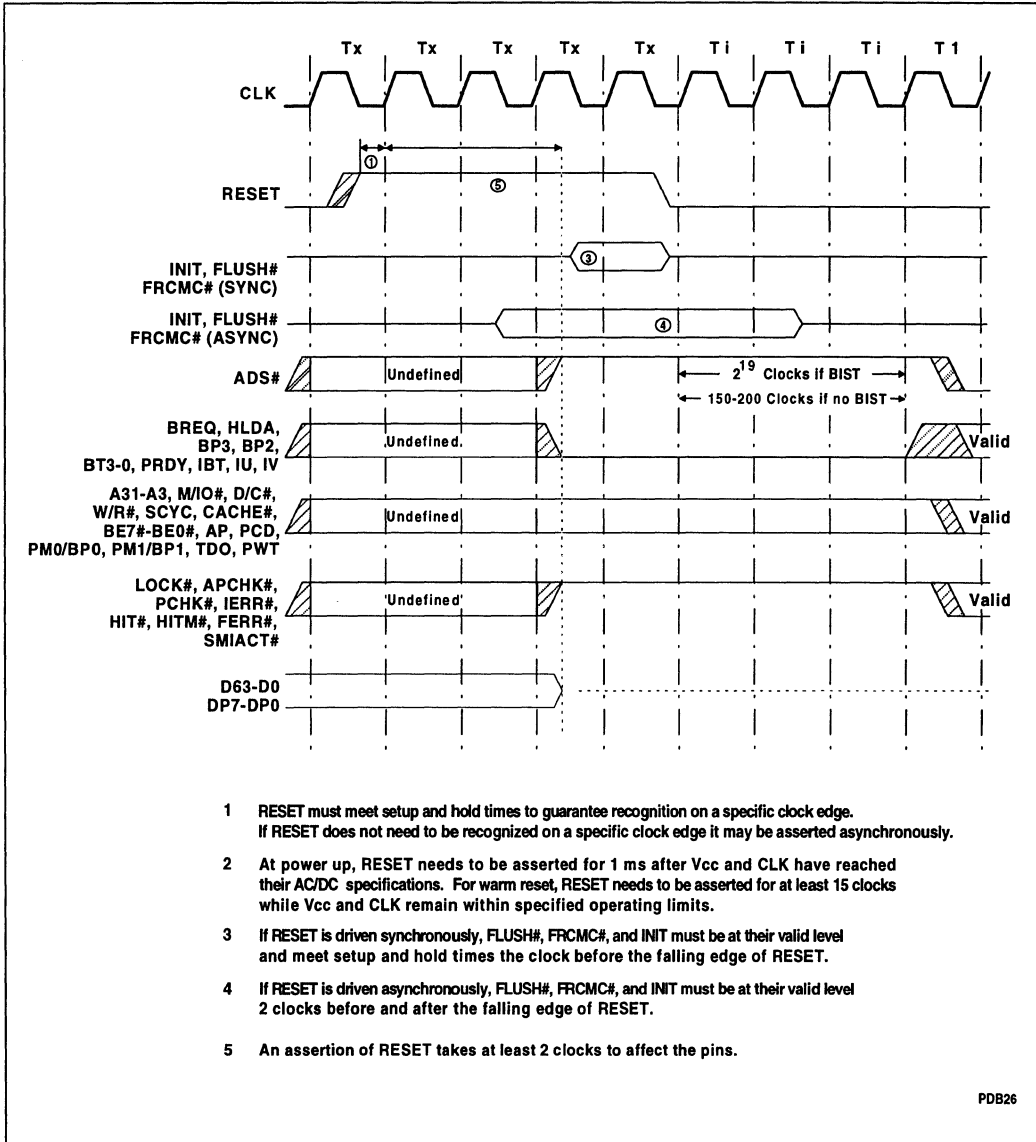
Figure 4-1. Pin States during RESET
