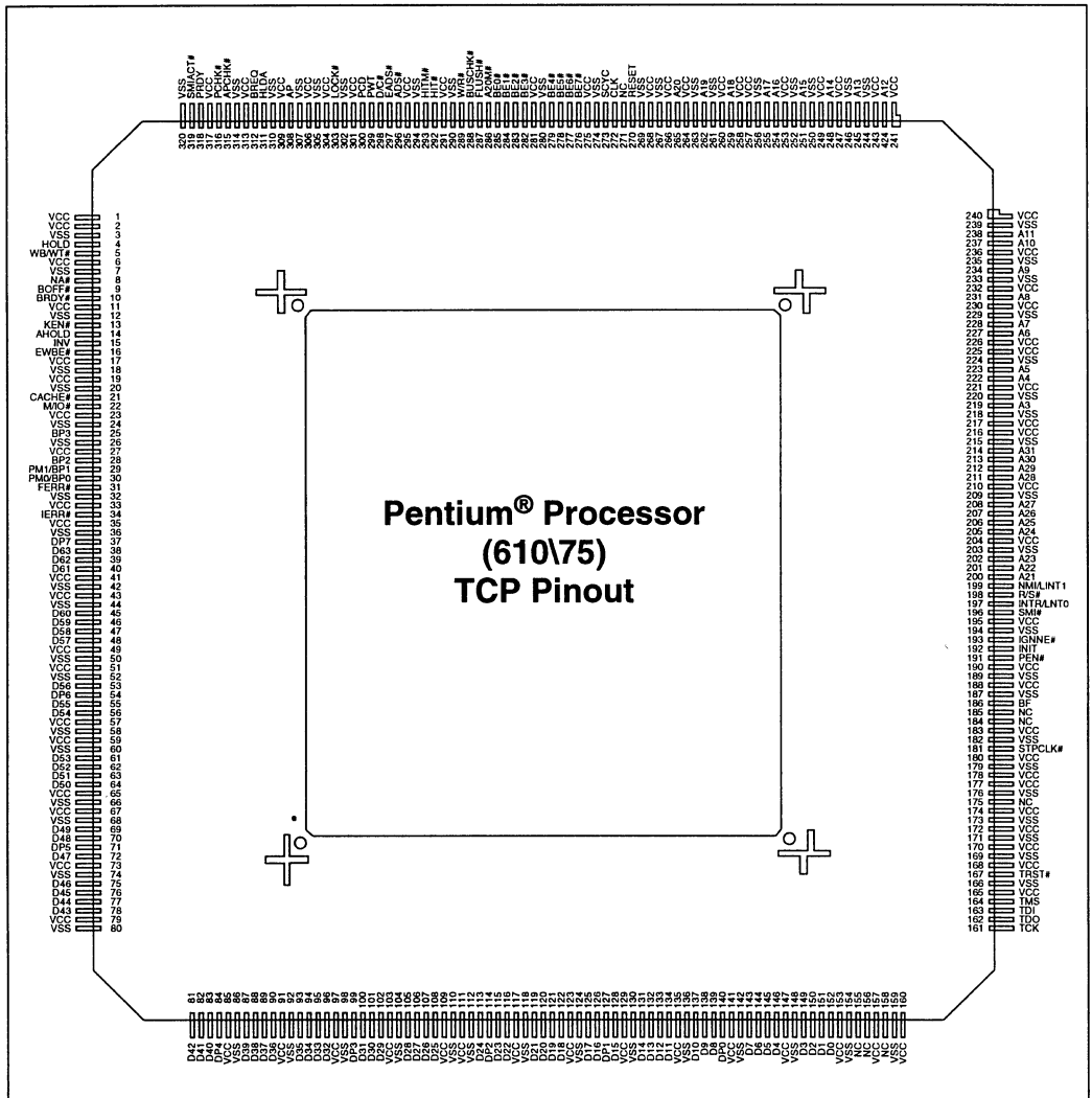
Figure 34-1. Pentium® Processor (610\75) TCP Pinout
