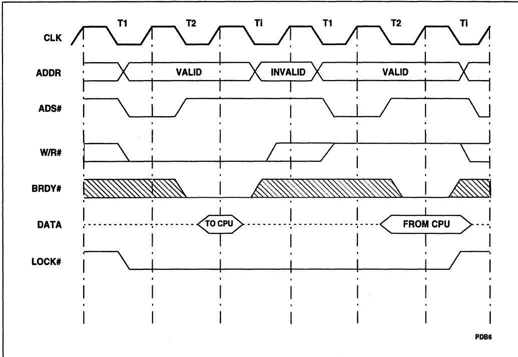
Figure 6-11. LOCK# Timing
