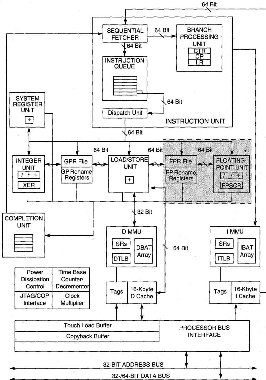
Figure 8-1. Block Diagram
