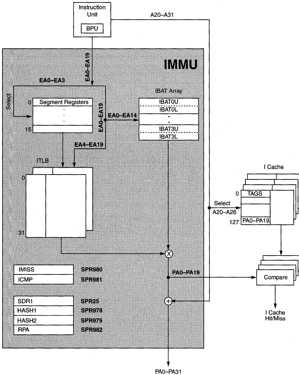
Figure 5-2. IMMU Block Diagram
