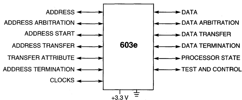
Figure 1-6. System Interface
