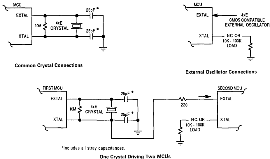
Figure 1. Oscillator Collections
