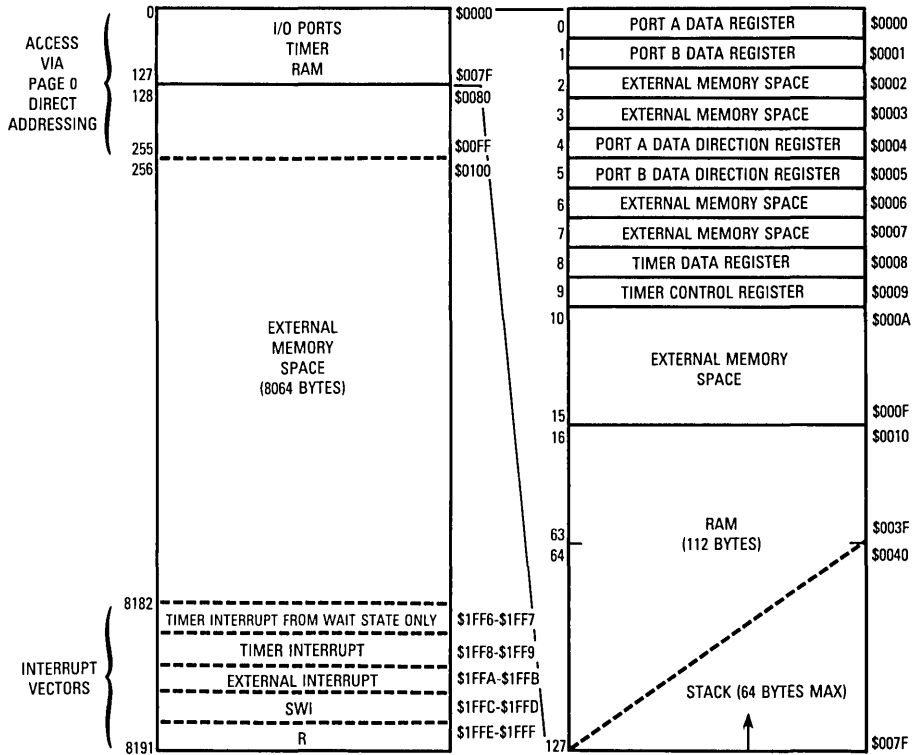
Figure 4. Memory Map
