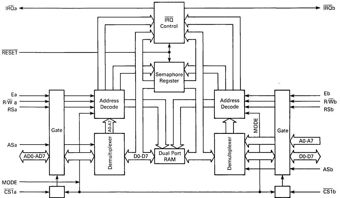
FIGURE 1 — BLOCK DIAGRAM
