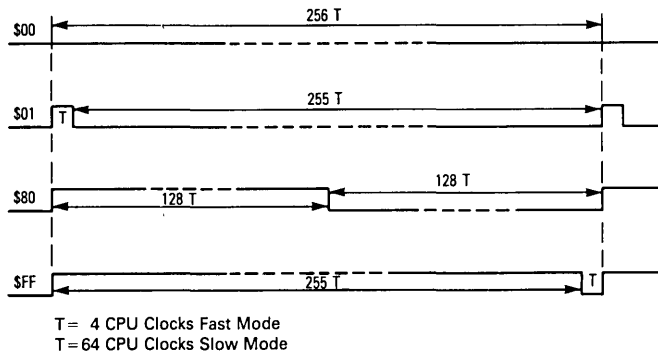
Figure 20. PLM Output Waveform Examples
