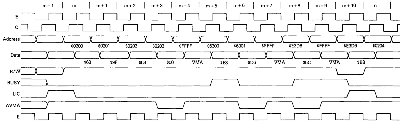
FIGURE 12 — BUSY TIMING
