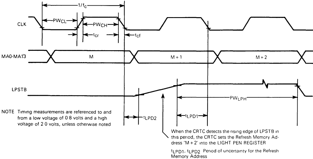
FIGURE 5 — CRTCLK, MA0-MA13, AND LPSTB TIMING DIAGRAM
