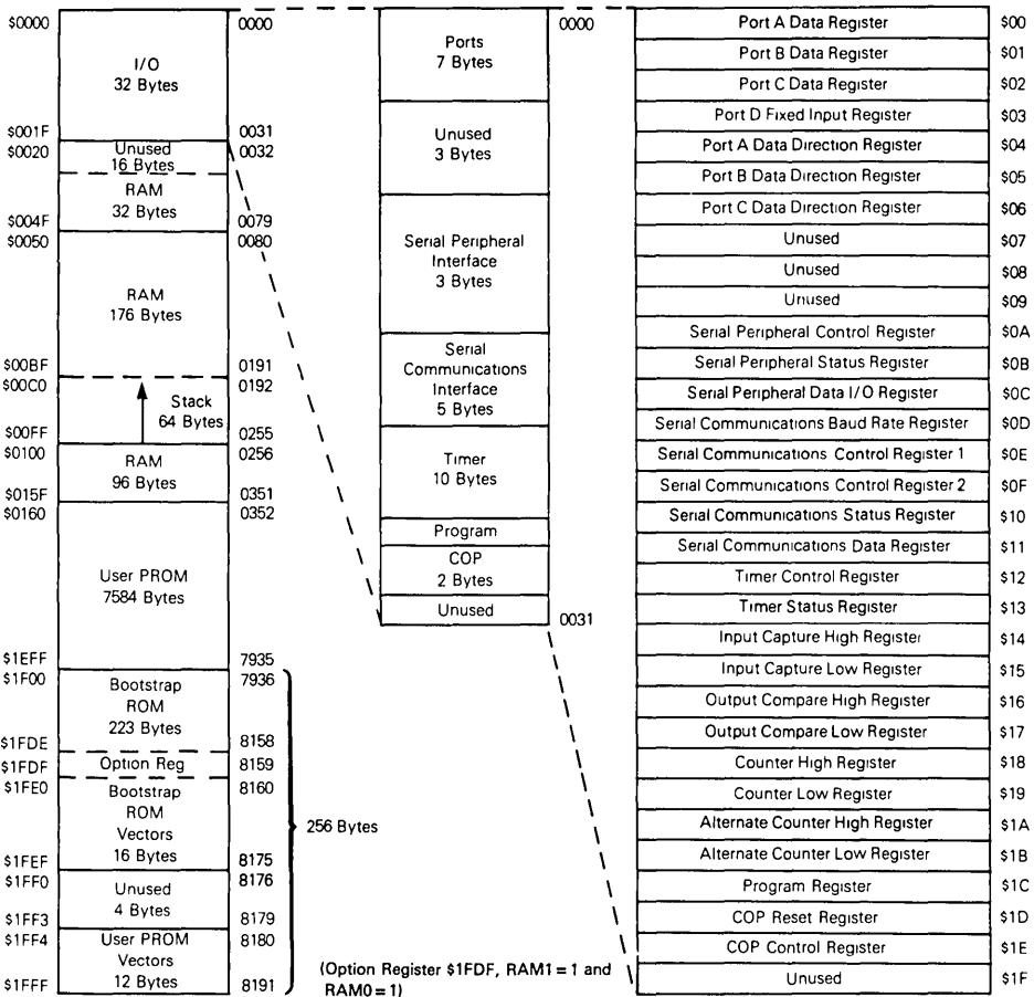
Figure 7. Memory Map #4
