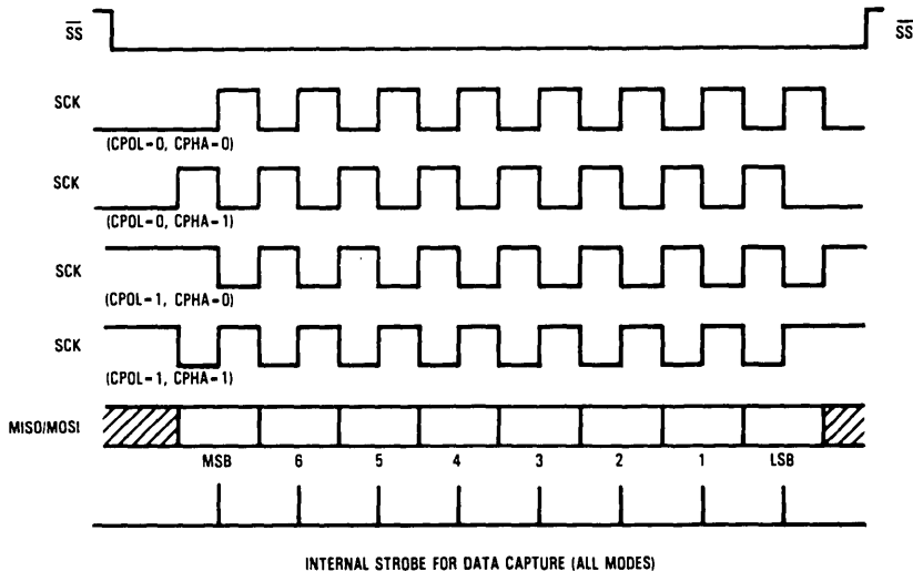
INTERNAL STROBE FOR DATA CAPTURE (ALL MODES)
