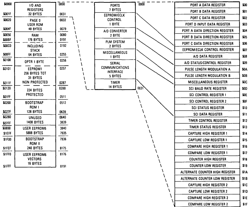
Figure 3. Memory Map
