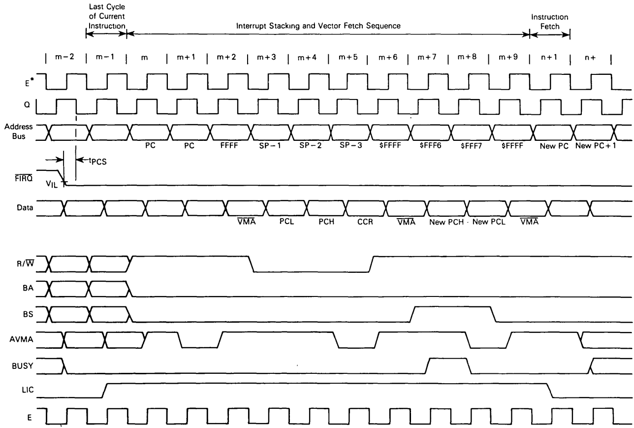
FIGURE 9 - \overline{\text{FIRQ}} INTERRUPT TIMING
