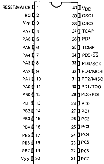
40-PIN DUAL-IN-LINE PACKAGE
