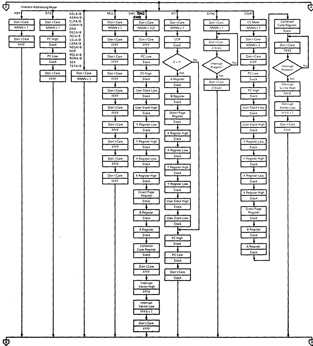
FIGURE 17 — CYCLE-BY-CYCLE PERFORMANCE (Sheet 2 of 5)
