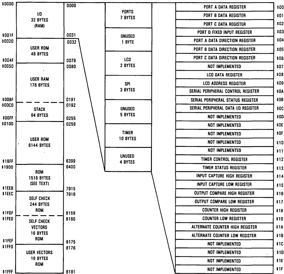
Figure 4. Memory Map
