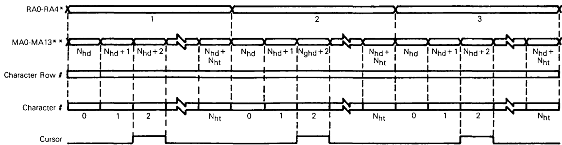
FIGURE 17 – CURSOR TIMING
