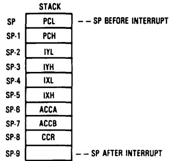
Figure 4. Stacking Order
