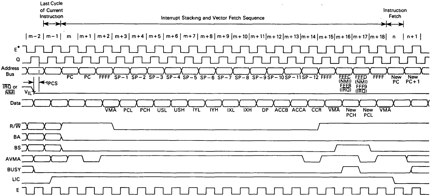
FIGURE 8 — \overline{IRQ} AND \overline{NMI} INTERRUPT TIMING
