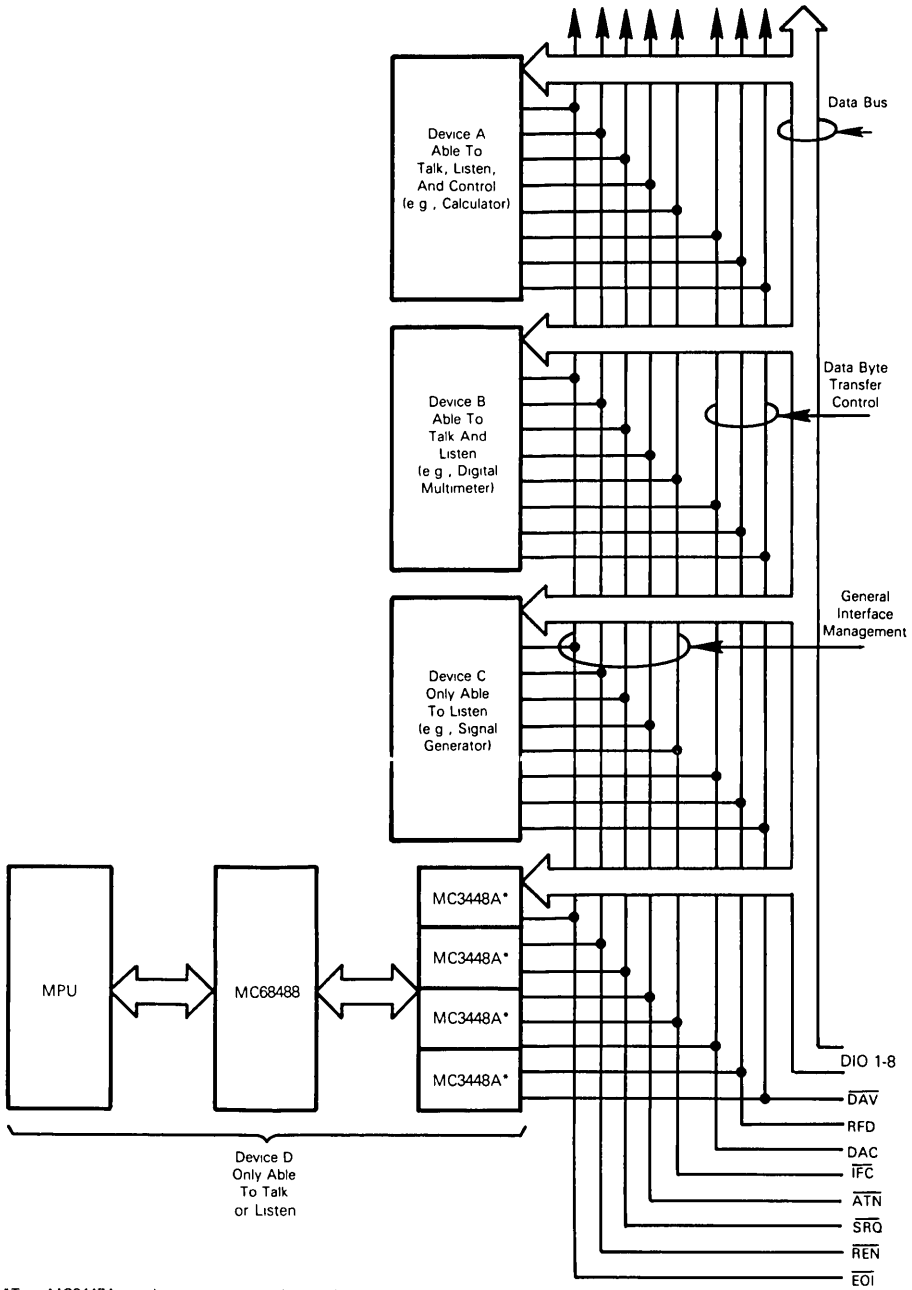
FIGURE 6 — GPIB SYSTEM
