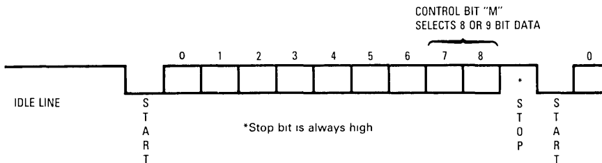
Figure 15. Data Format
