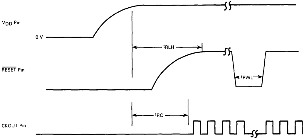
FIGURE 7 — POWER-UP
