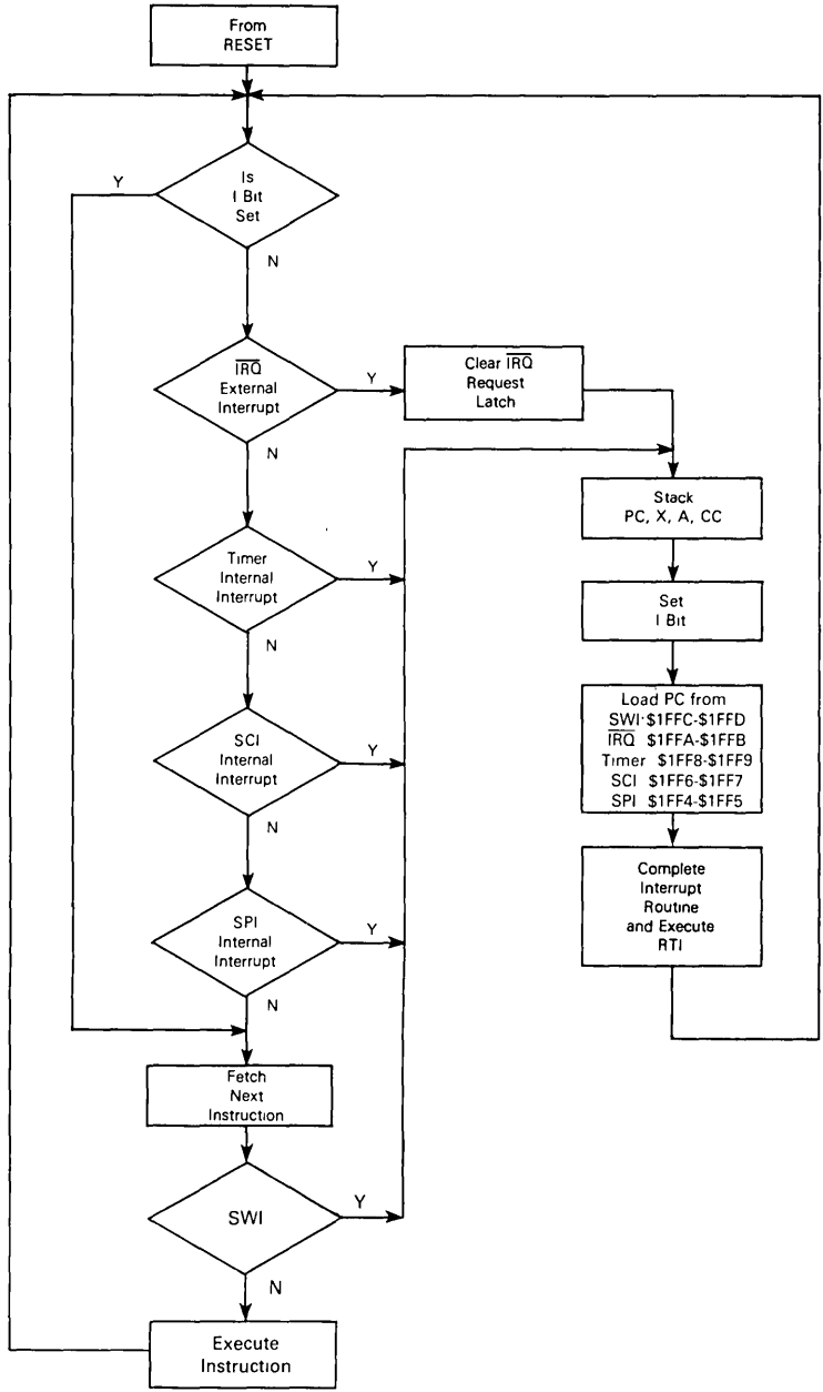
Figure 9. Reset and Interrupt Processing Flowchart
