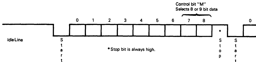
Figure 16. Data Format
