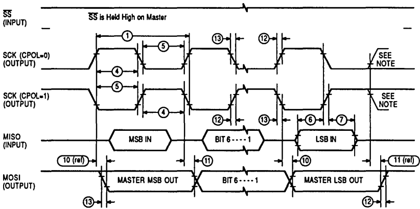
b) SPI MASTER TIMING (CPHA = 1)
