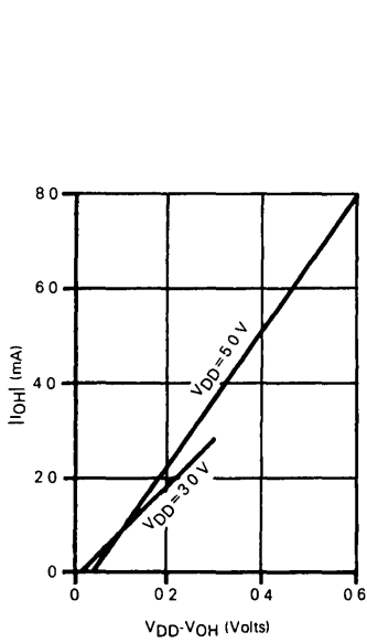
Figure 22. Typical V_{OH} vs I_{OH} for PD1-PD4
