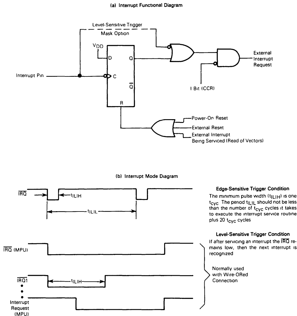
Figure 6. External Interrupt
