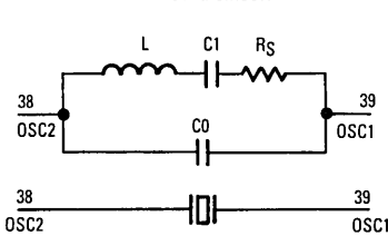
CRYSTAL CIRCUIT
