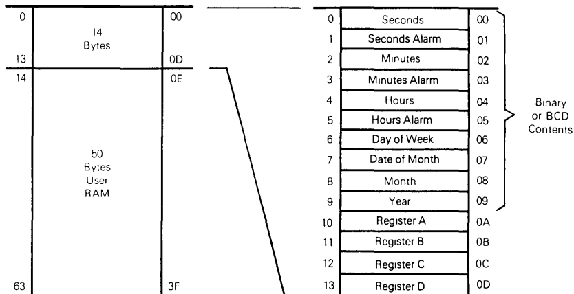
FIGURE 14 — ADDRESS MAP
