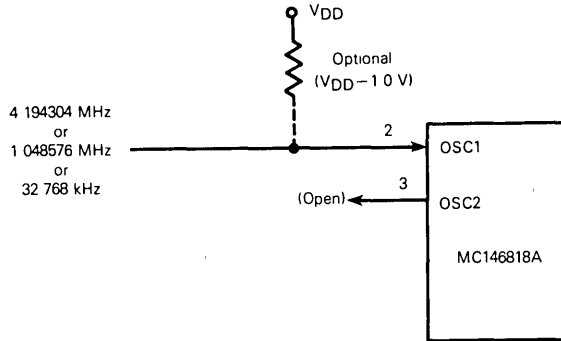
FIGURE 9 — EXTERNAL TIME-BASE CONNECTION
