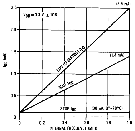
Figure 29. Maximum I_{DD} vs Frequency for V_{DD} = 3.3\text{ Vdc}
