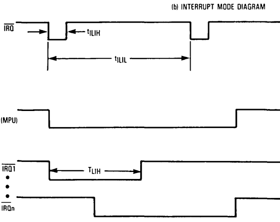
Figure 7. External Interrupt
