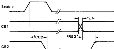
FIGURE 12 — CB2 DELAY TIME (Write Mode; CRB-5=1, CRB-3=CRB-4=0)
