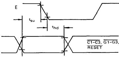
FIGURE 4 — INPUT SETUP AND HOLD TIMES
