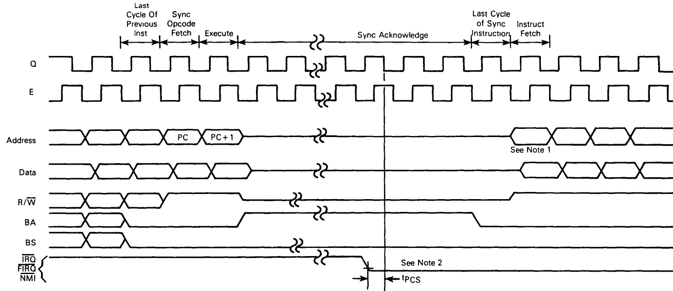
FIGURE 17 — SYNC TIMING
