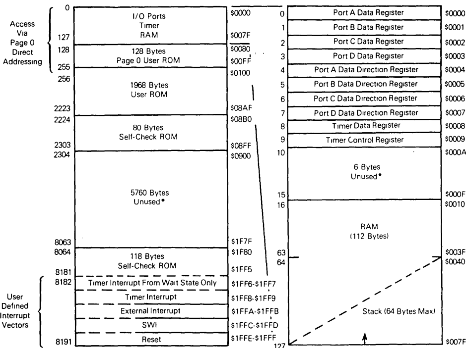
Figure 3. Memory Map
