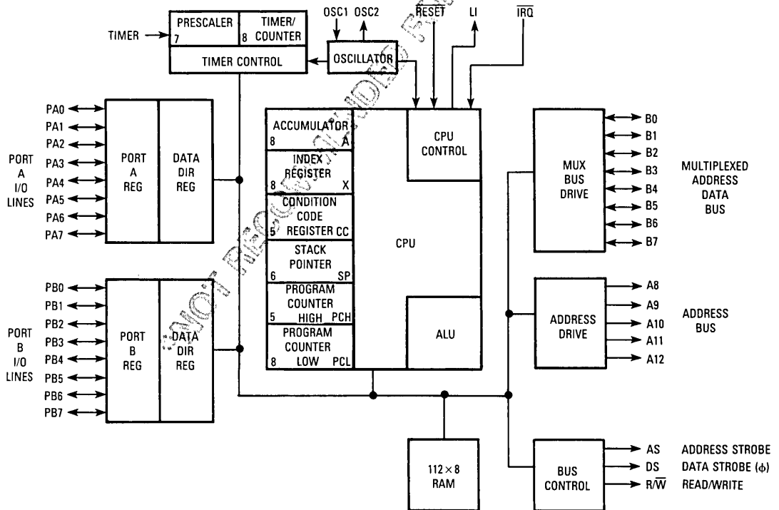
BLOCK DIAGRAM
