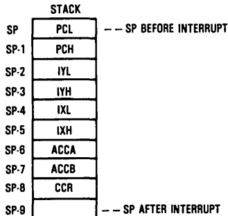
Figure 4. Stacking Order
