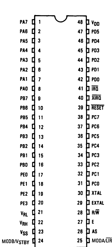
48-Pin Dual-in-Line Package
