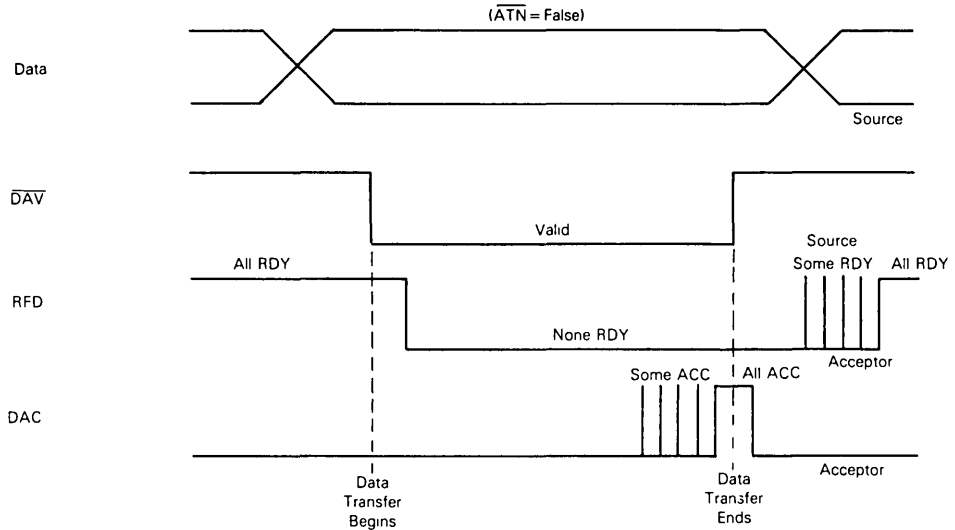
FIGURE 2 — SOURCE AND ACCEPTOR HANDSHAKE
