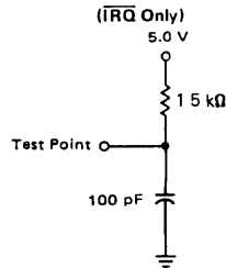
FIGURE 5 — NMOS EQUIVALENT TEST LOAD ( \overline{IRQ} Only)
