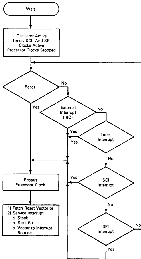
Figure 12. WAIT Function Flowchart
