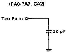
FIGURE 4 — CMOS EQUIVALENT TEST LOAD (PA0-PA7, CA2)
