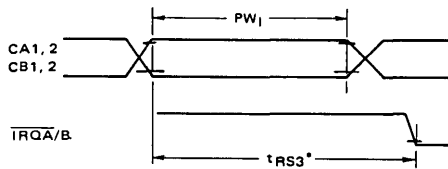
FIGURE 13 — INTERRUPT PULSE WIDTH AND \overline{IRQ} RESPONSE
