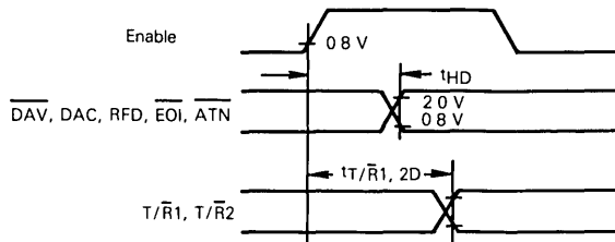
FIGURE 4 — OUTPUT BUS TIMING
