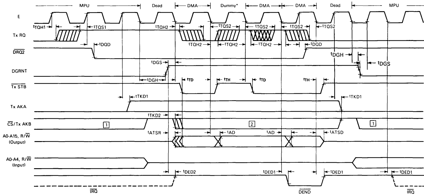
FIGURE 6 — MODE 3 TIMING (HALT BURST MODE)
