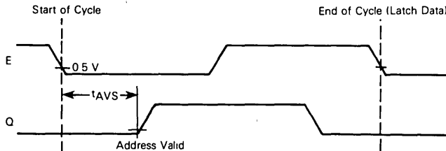
FIGURE 11 — E/Q RELATIONSHIP
