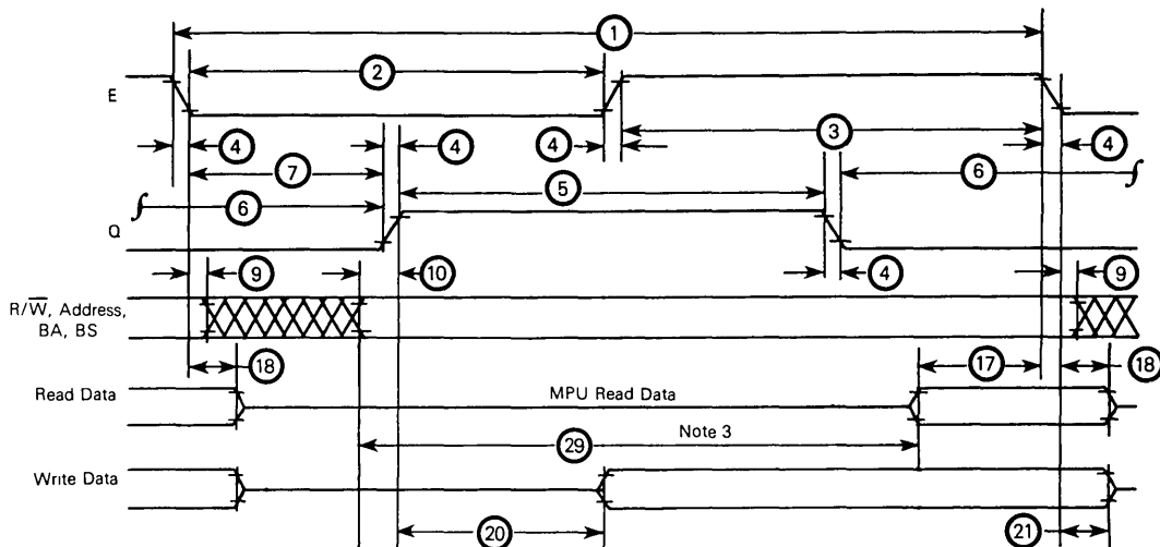
FIGURE 1 — BUS TIMING
