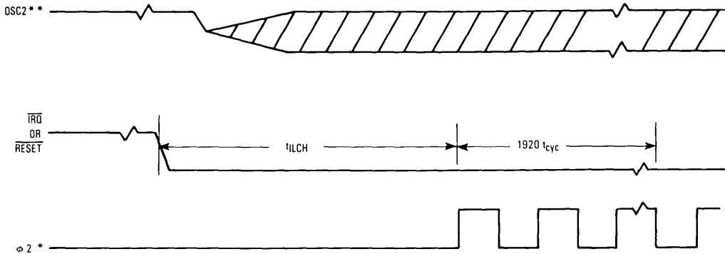
Figure 16. Stop Recovery
