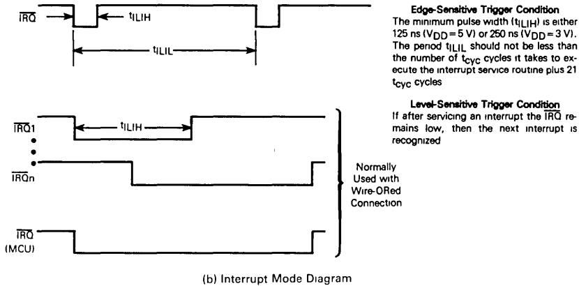
Figure 12. External Interrupt
