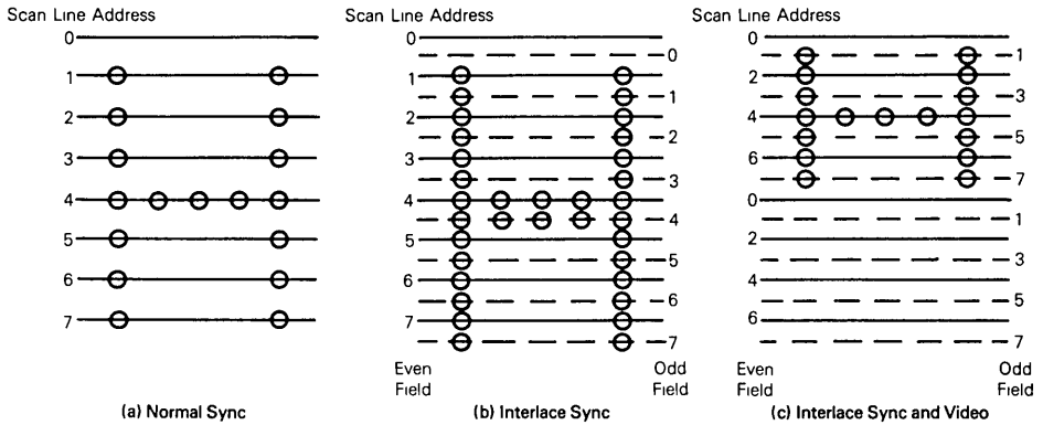
FIGURE 14 — INTERLACE CONTROL
