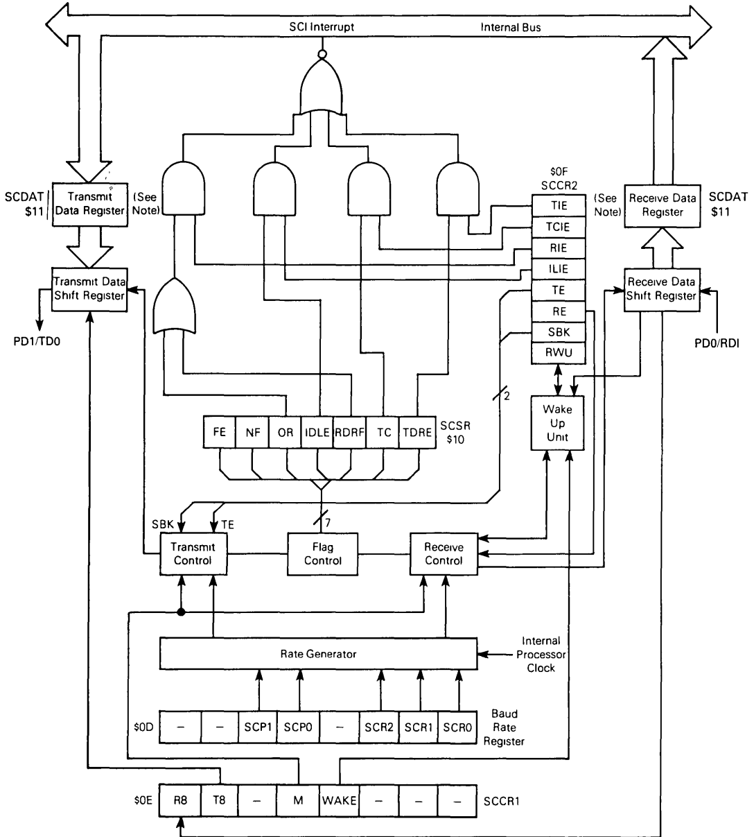
Figure 17. SCI Block Diagram
