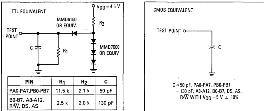
Figure 17. Equivalent Test Loads
