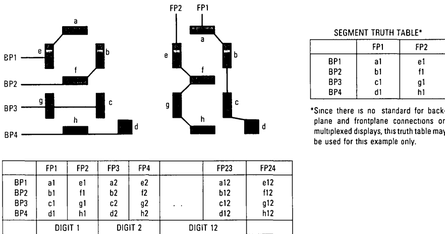
Figure 17. Frontplane and Backplane Connections to a Multiplexed-by-Four Seven-Segment LCD (Includes Decimal Point)
