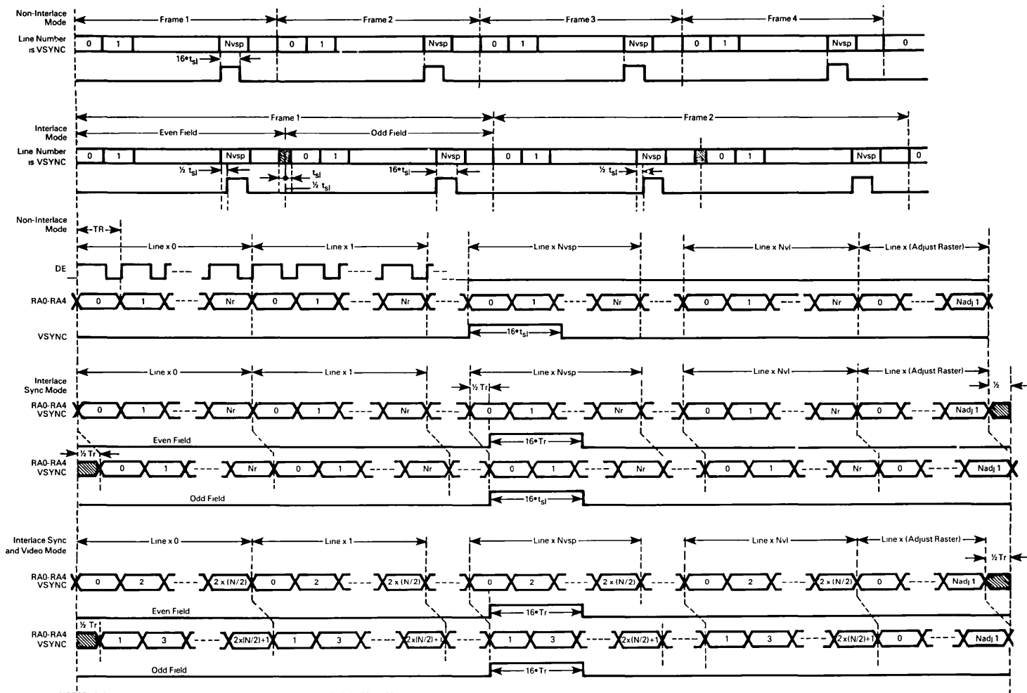
FIGURE 13 — CRTS VERTICAL TIMING
