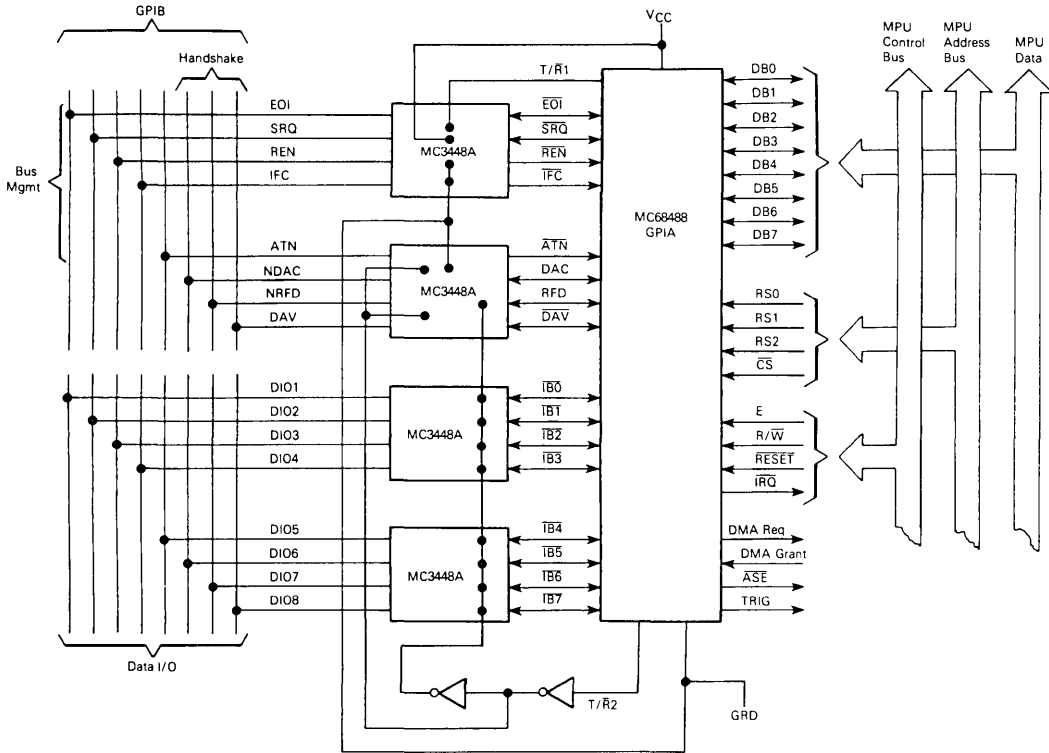
FIGURE 1 — GPIB INTERFACE
