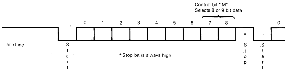
Figure 12. Data Format
