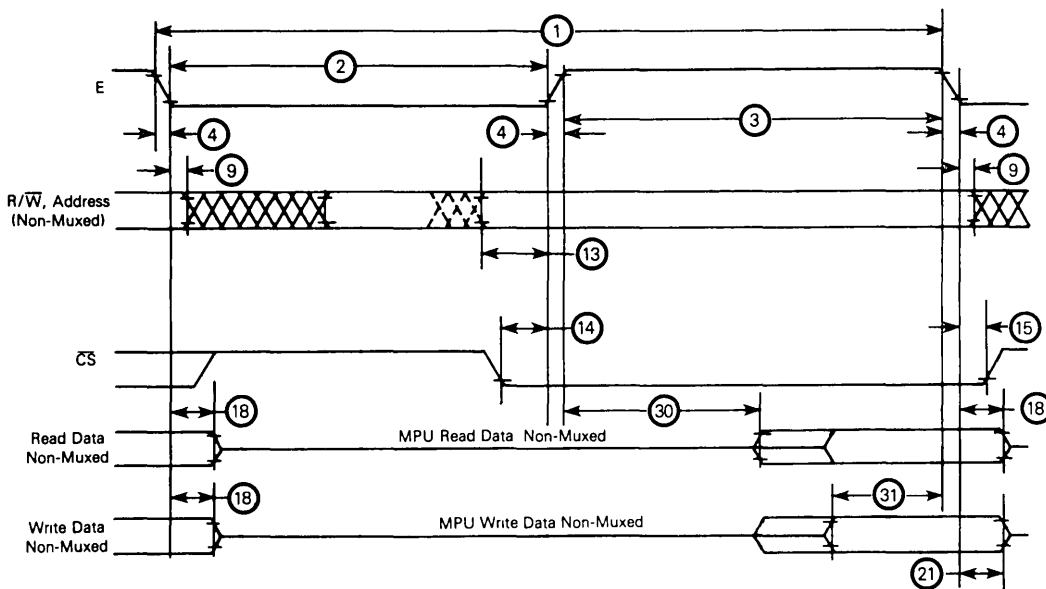
FIGURE 3 — BUS TIMING
