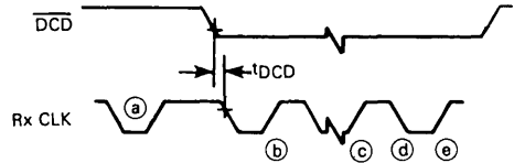
FIGURE 7 — DATA CARRIER DETECT SETUP TIME
