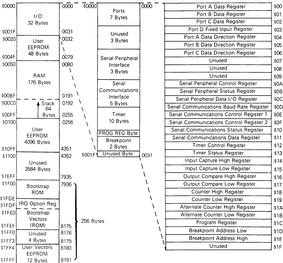
Figure 4. Memory Map
