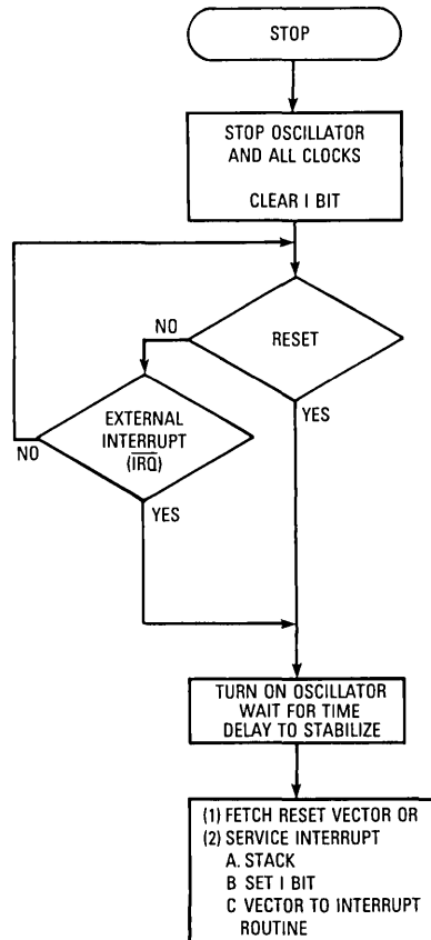
Figure 12. STOP Function Flowchart
