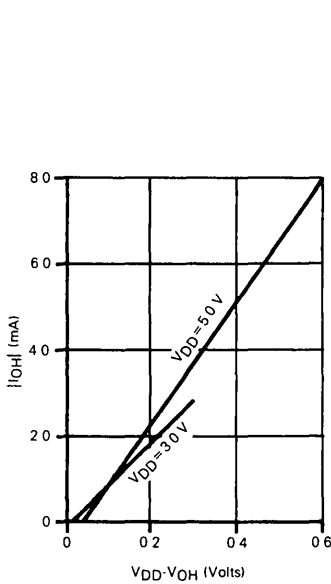
Figure 24. Typical V_{OH} vs I_{OH} for PD1-PD4
