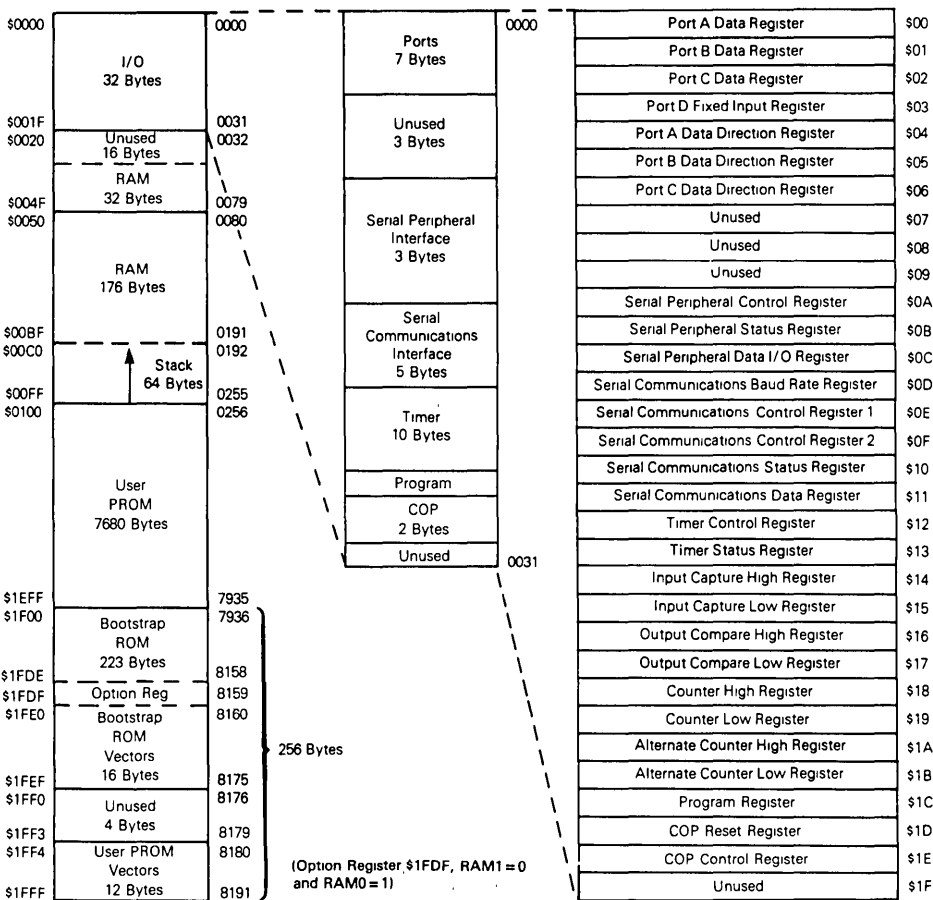
Figure 5. Memory Map #2
