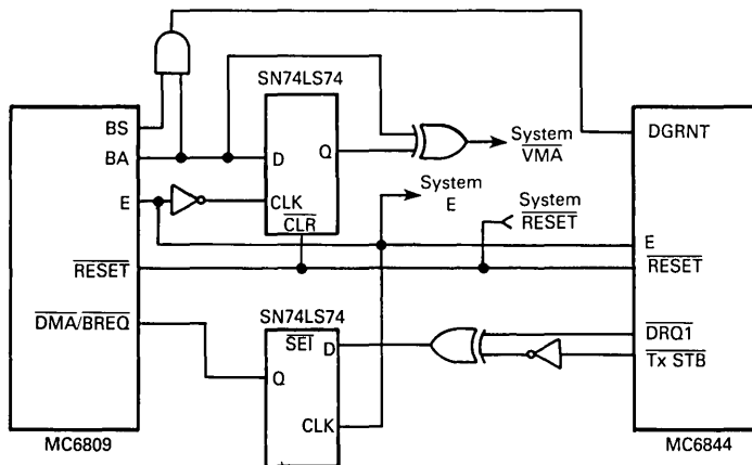
FIGURE 13 — MC6844/MC6809 INIFACE FOR MODE 1 DMA
