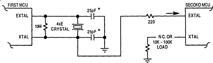
One Crystal Driving Two MCUs
