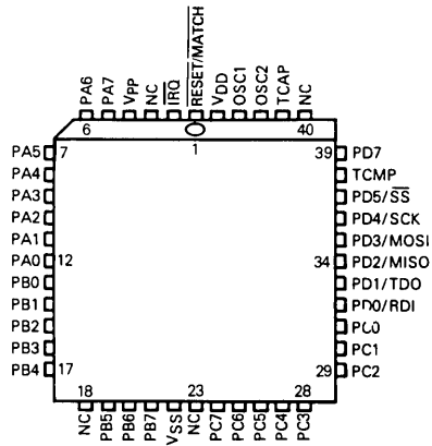
44-LEAD PLCC PACKAGE
