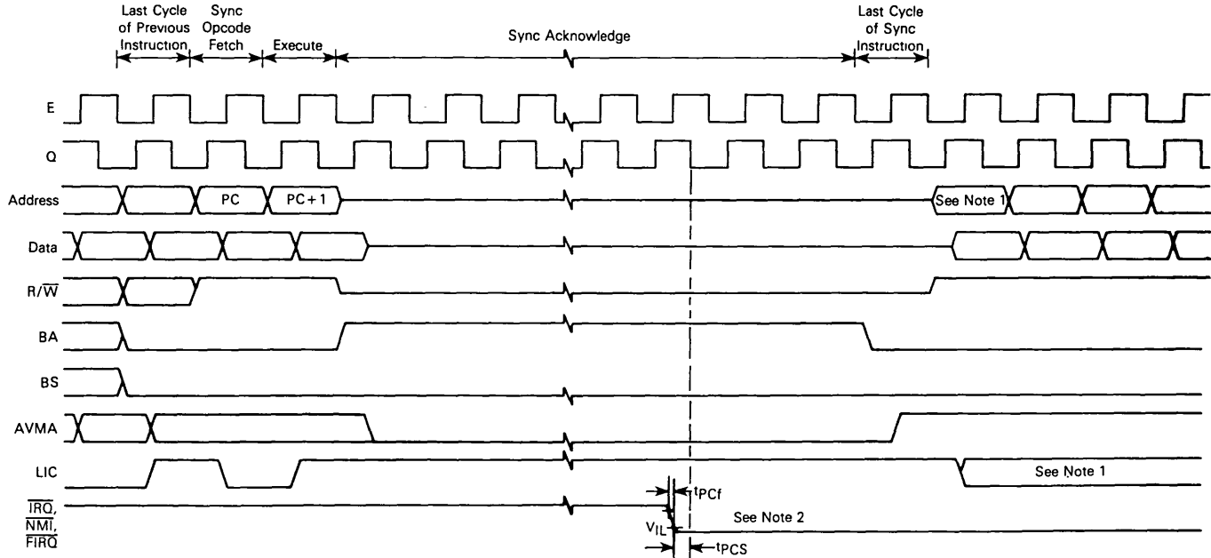
FIGURE 16 — SYNC TIMING
