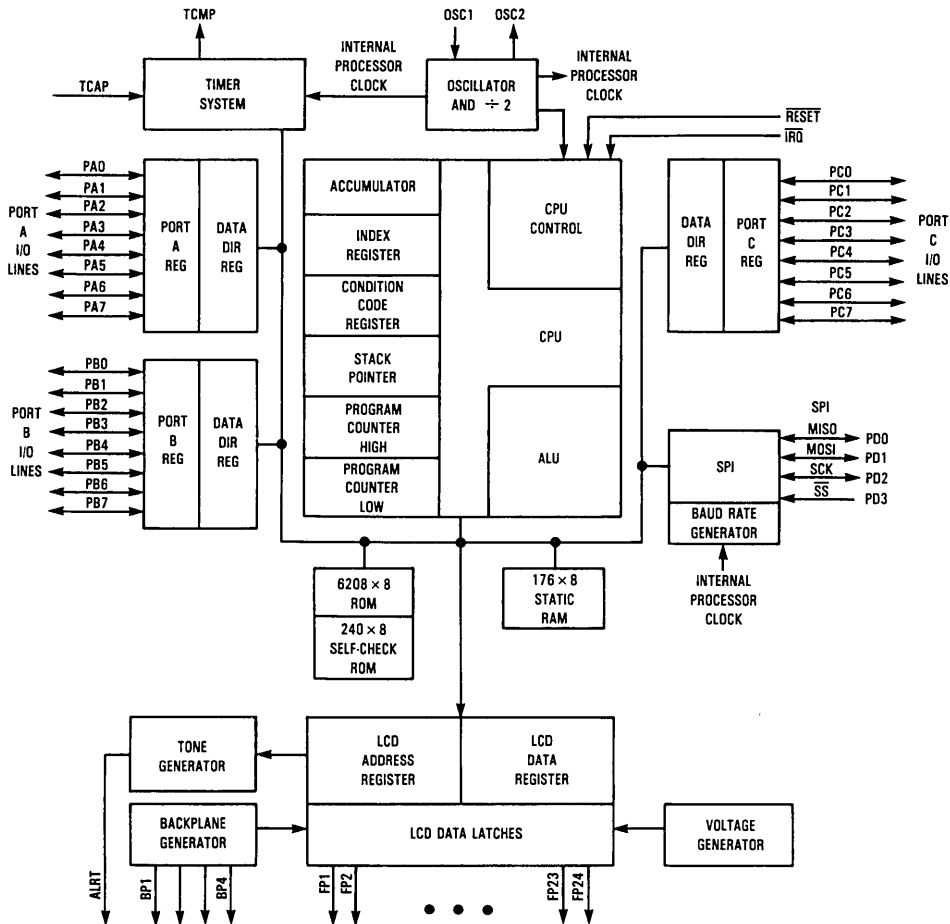
BLOCK DIAGRAM
