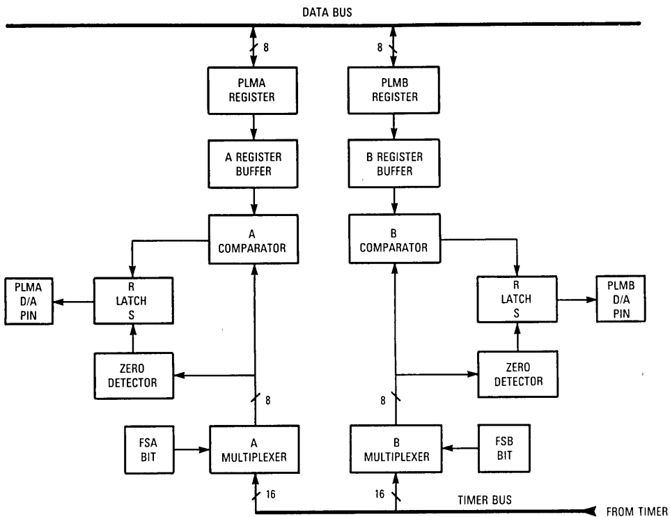
Figure 19. PLM Block Diagram
