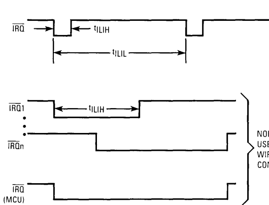
(b) Interrupt Mode Diagram
