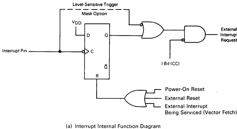
(a) Interrupt Internal Function Diagram
