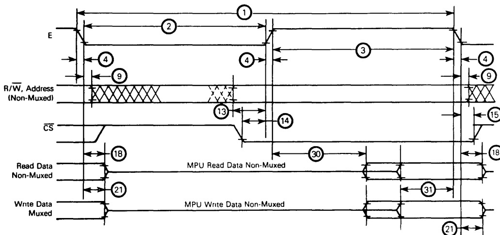
FIGURE 1 — BUS TIMING
