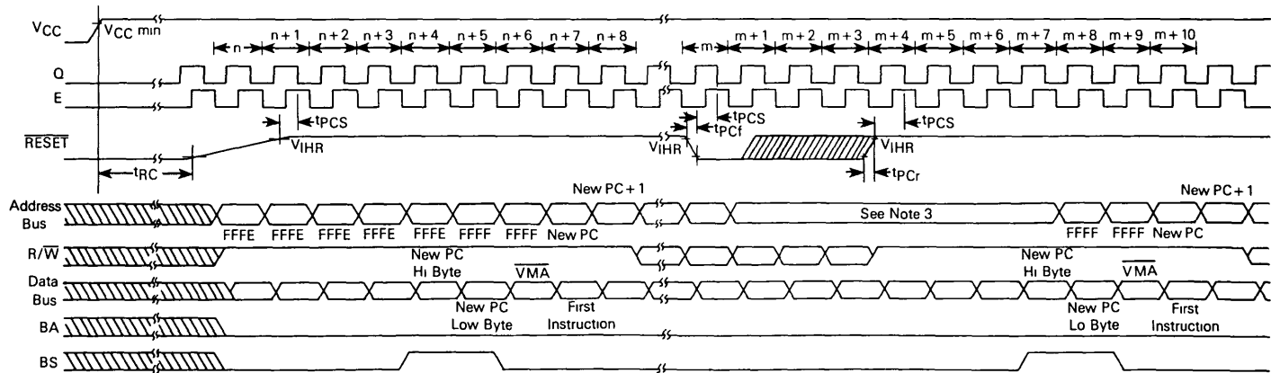
FIGURE 6 - RESET TIMING
