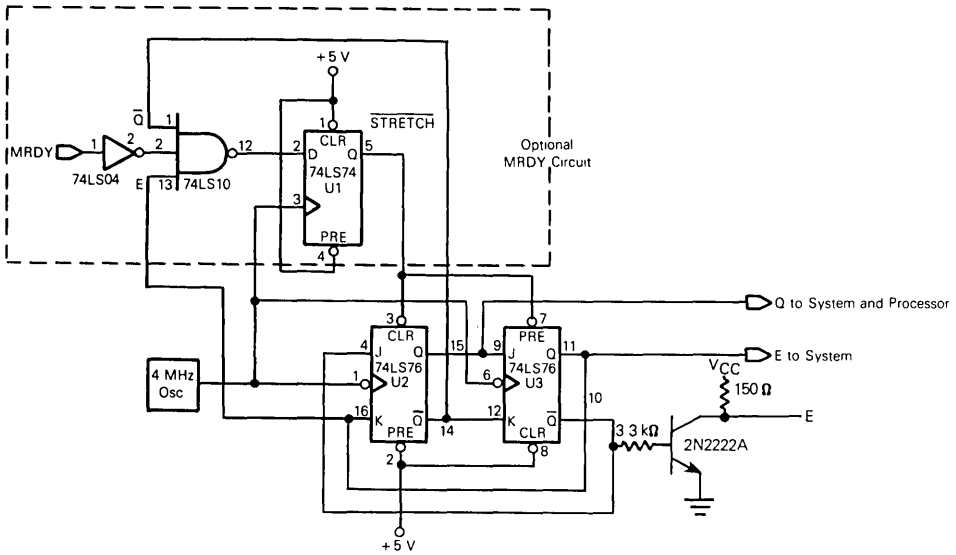
FIGURE 10 – CLOCK GENERATOR
