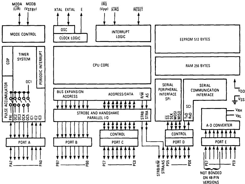
BLOCK DIAGRAM
