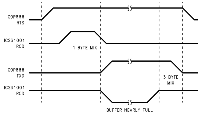
FIGURE 7. Serial Timing
