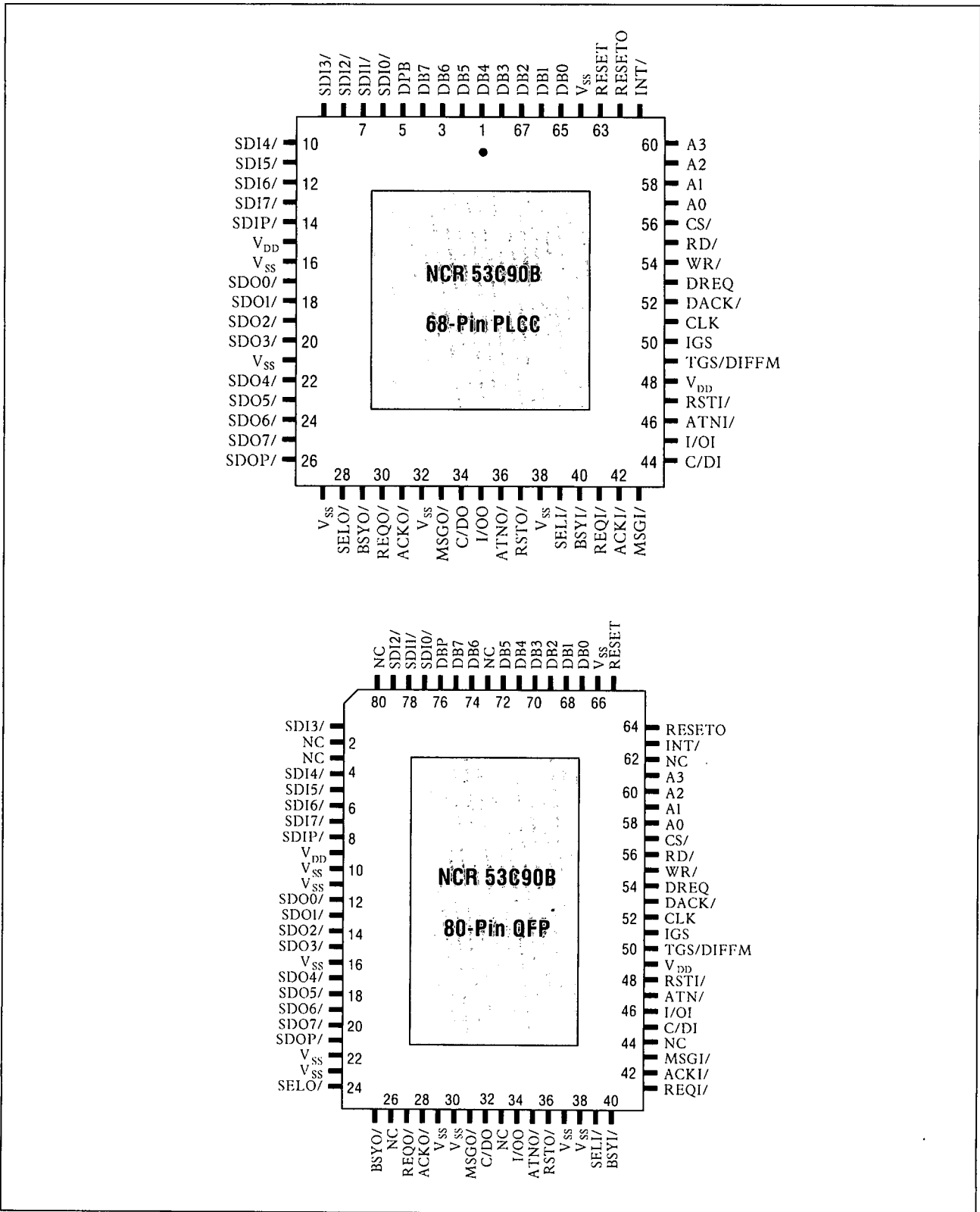
Figure 3. NCR 53C90B Pin Configurations
