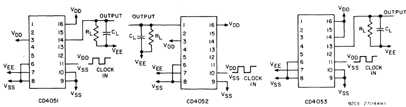
Fig. 18 - Propagation delay - address input to signal output.
