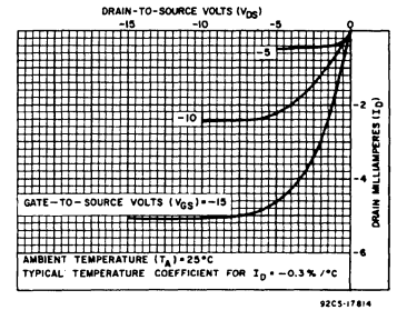
Fig. 5 - Typical output p-channel drain characteristics.
