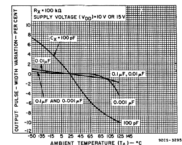
Fig. 23—Typical output pulse-width variations vs. ambient temperature.
