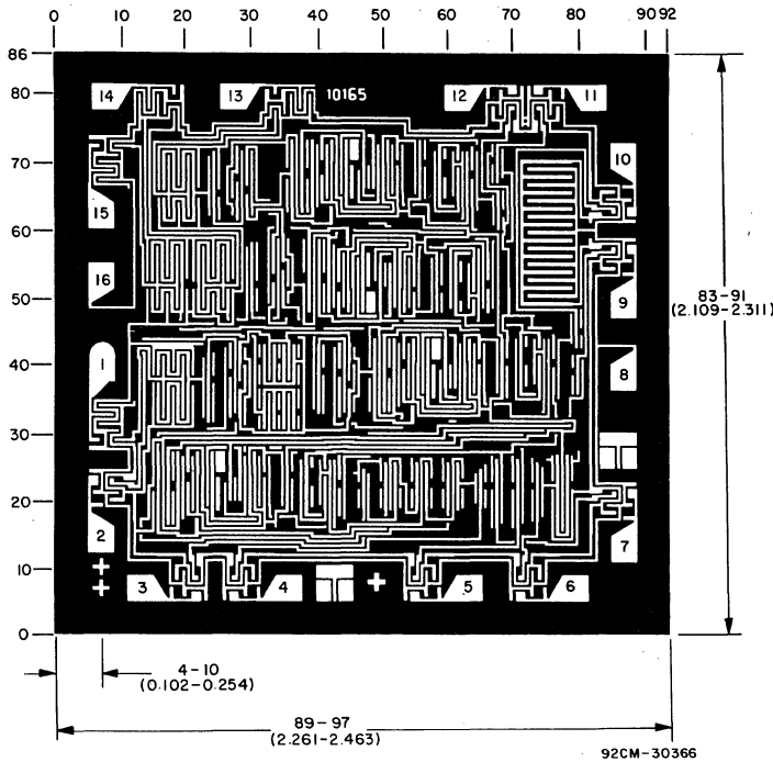
Dimensions and pad layout for CD4035BH.
