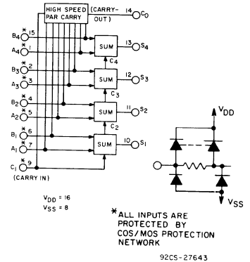
Fig.1 - CD4008B logic diagram.
