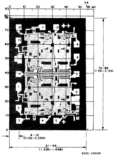
Dimensions and Pad Layout for CD40106BH
