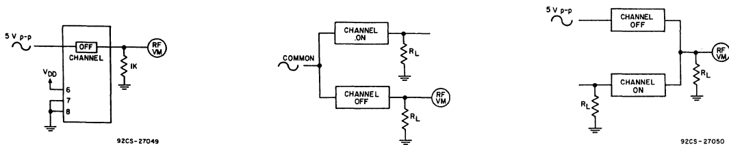
Fig. 25 - Crosstalk between any two channels (all types).
