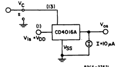
SWITCH THRESHOLD VOLTAGE IS DEFINED AS THE VOLTAGE APPLIED TO A TRANSMISSION GATE CONTROL WHICH CAUSES 10 \mu A OF TRANSMISSION GATE CURRENT.
