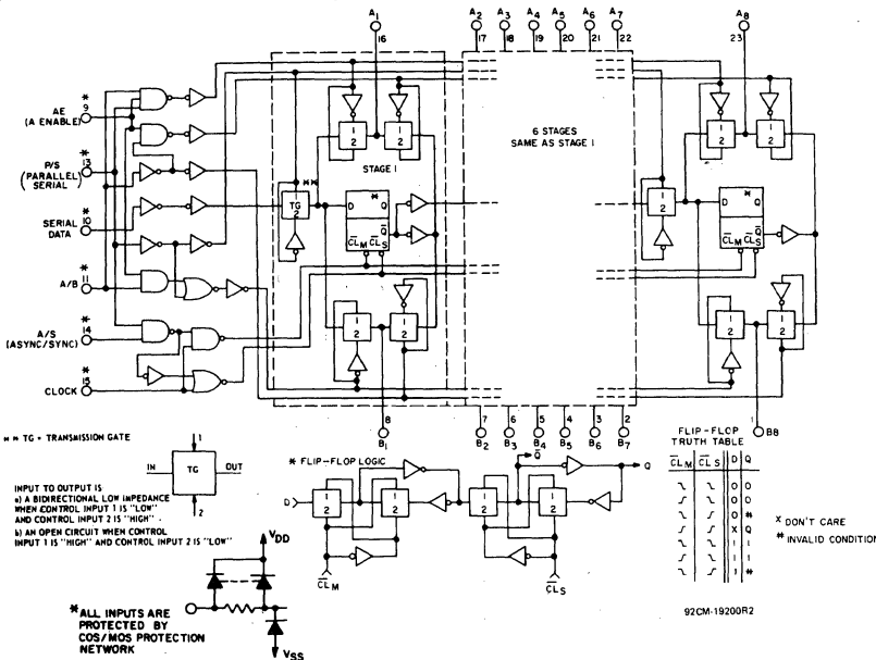
Fig. 2 — Logic diagram.
