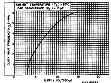
Fig. 2 — Typical clock input frequency vs. supply voltage.
