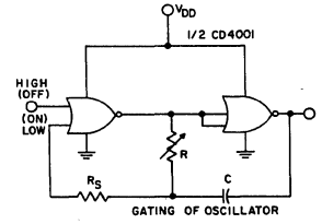
Fig. 7 - Astable multivibrator in which a NOR or NAND gate is used as the first inverter to permit gating of the multivibrator.
