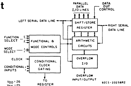
Fig. 1 — Block diagram — CD4057A.
