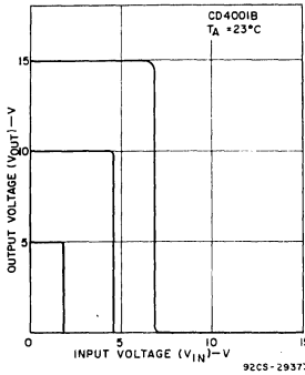
Fig. 3 CD4001B voltage transfer characteristic.
