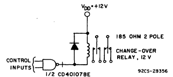
Fig. 10 - Relay driver circuit.
