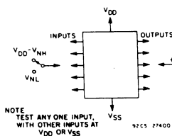
Fig. 10 - Noise immunity test circuit.
