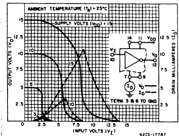
Fig. 2 - Typical current and voltage-transfer characteristics for inverter.
