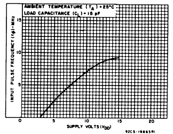
Fig. 11 — Typical input pulse frequency vs. V_{DD} .
