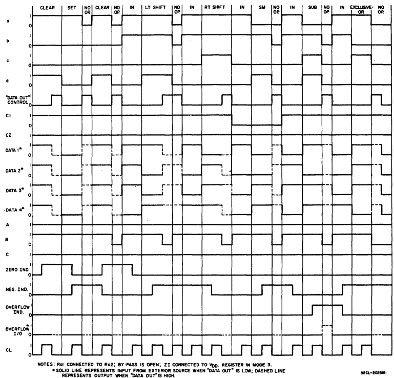
Fig. 12 — Timing diagram.
