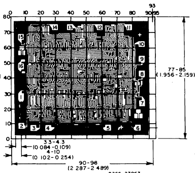
Dimensions and pad layout for CD4055BH
