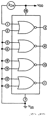
Fig. 13 - Input-current test circuit for the CD4001A, input high ( I_{IH} ).
