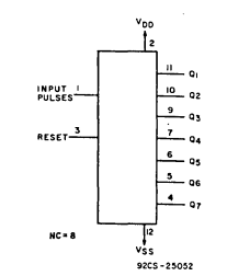
Fig. 2 - Functional diagram for CD4024AT.
