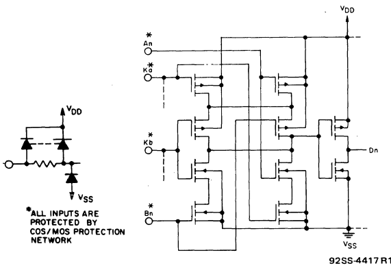
Fig. 1 — Schematic diagram for 1 of 4 identical stages.
