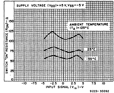
Fig. 3— Typical ON resistance as a function of input signal voltage at V_{DD} = +5\text{ V} , V_{SS} = -5\text{ V} .
