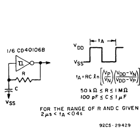
Fig. 18 - Astable multivibrator.
