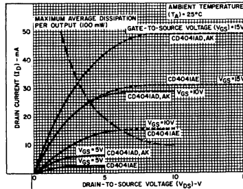
Fig. 6 - Minimum output n-channel drain characteristics - true output.
