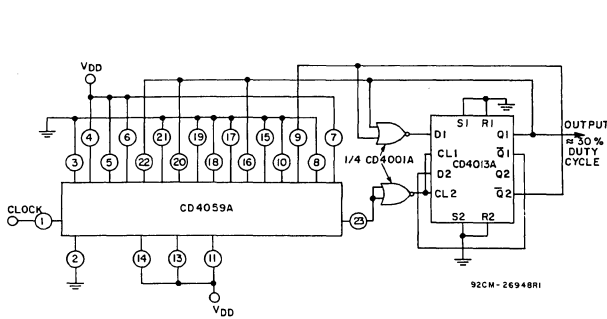
Fig. 16 – Division by 47,690 in ÷2 mode.
