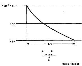
Fig. D-1 - Waveform for calculating power dissipation.
