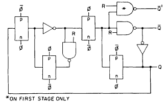
Fig. 4 — Detail of typical flip-flop stage.
