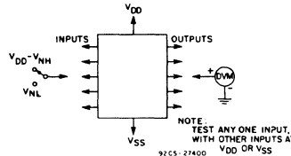
Fig. 8 — Noise immunity test circuit.
