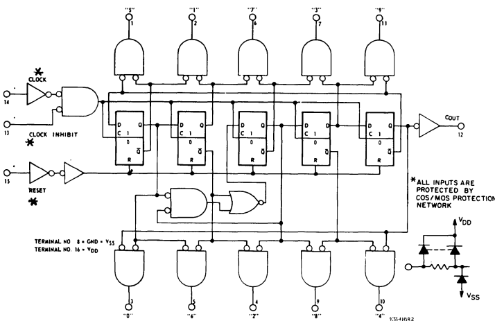
Fig. 1 - Logic diagram.
