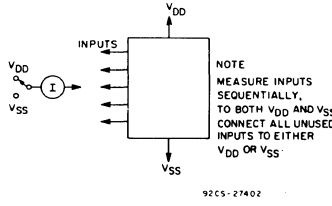
Fig. 15 - Input-leakage current.
