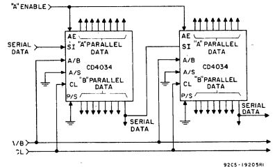
Fig. 18 — 16-bit serial in/gated parallel out register.
