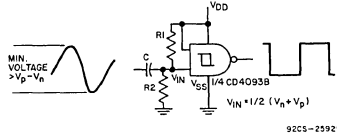
Fig.8 - Sine-wave to square-wave converter.
