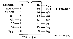
Fig. 1 — Terminal assignment.
