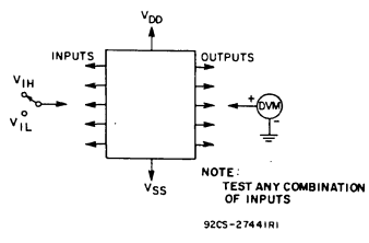
Fig. 11 – Input voltage test circuit.
