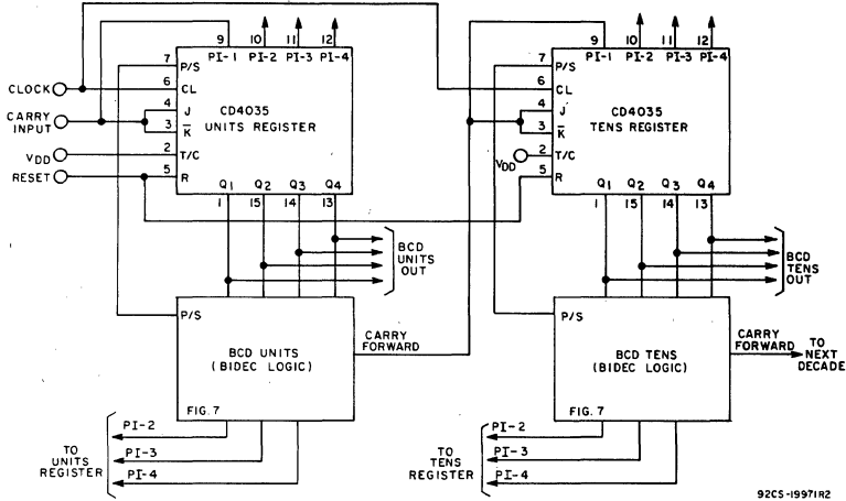
Fig. 17 - Binary-to-BCD converter.
