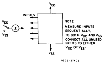
Fig. 20 — Input current test circuit.
