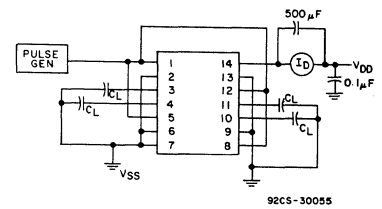
Fig. 13 - Dynamic power dissipation test circuit.
