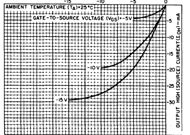
Fig. 4 - Typical output high (source) current characteristics.
