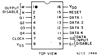
TERMINAL ASSIGNMENT
