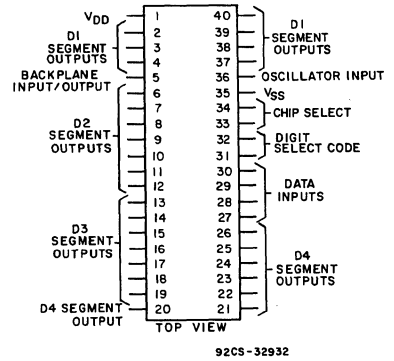
CD22105, CD22105A Terminal Assignment
