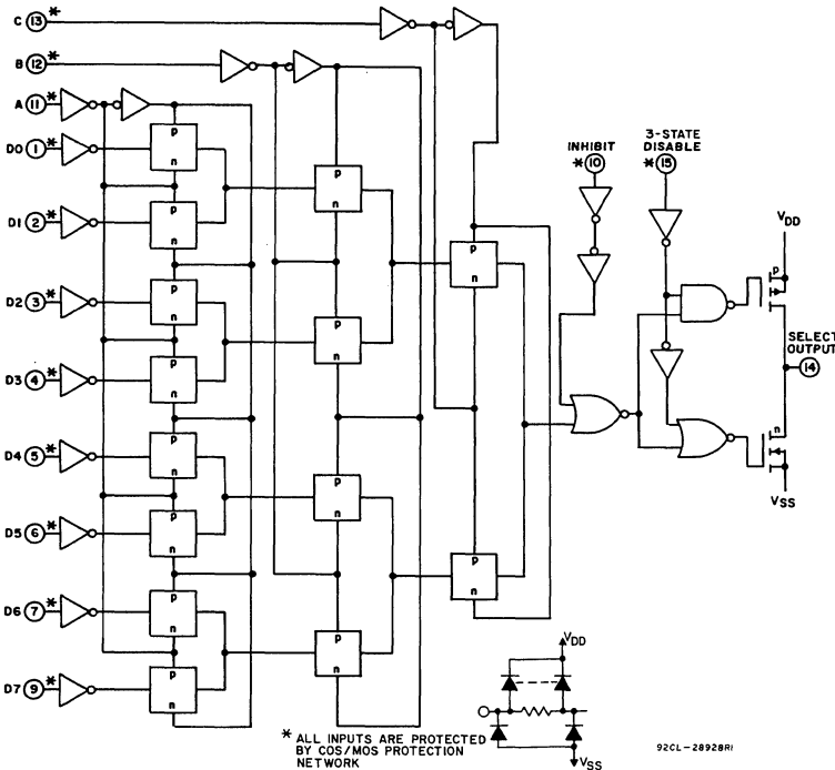
Fig. 1 - Logic diagram.
