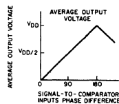
Fig. 4—Phase-comparator I characteristics low-pass filter output.
