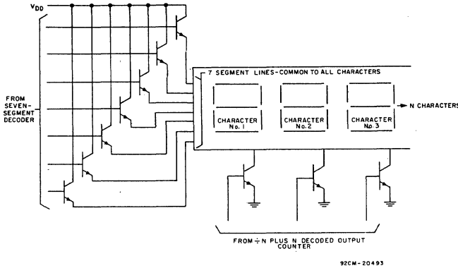
Fig. 16— Multiplexing driving circuit for light-emitting diodes.
