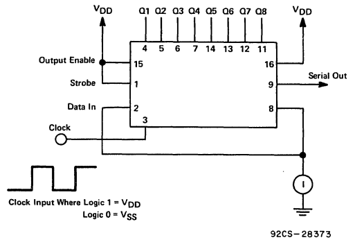
Fig. 15 - Functional-test arrangement for the CD4090.
