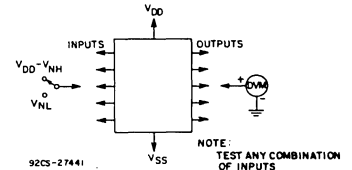
Fig. 10 - Noise-immunity test circuit
