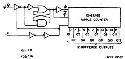
Fig.4 - Functional diagram.
