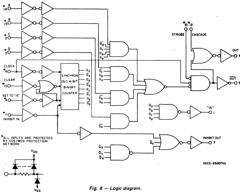
Fig. 4 — Logic diagram.
