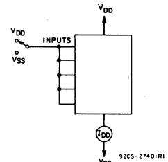
Fig. 11 — Quiescent device current test circuit.
