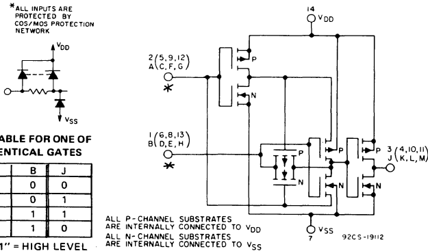
Fig. 1 — Schematic diagram for 1 of 4 identical exclusive-OR gates.
