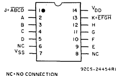
NC=NO CONNECTION TOP VIEW CD4012UB
