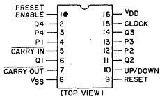
92CS-27015 CD4510B, CD4516B TERMINAL ASSIGNMENT
