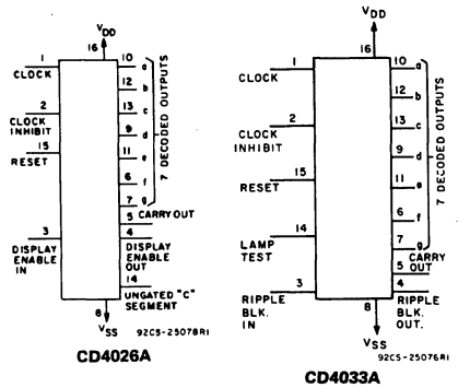
FUNCTIONAL DIAGRAMS
