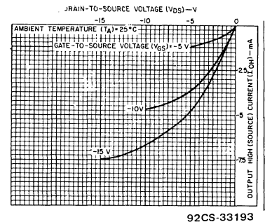
Fig. 13 - Minimum p-channel output high (source) current characteristics.
