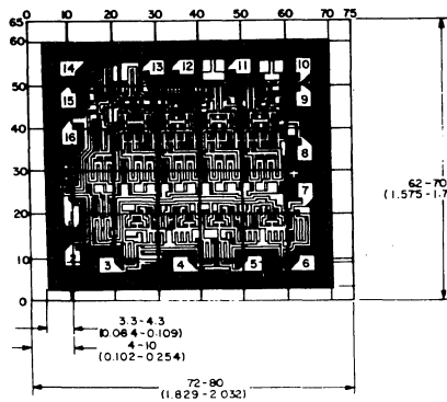
Dimensions and pad layout for CD4054BH.
