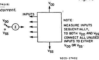
Fig. 11 - Input current.
