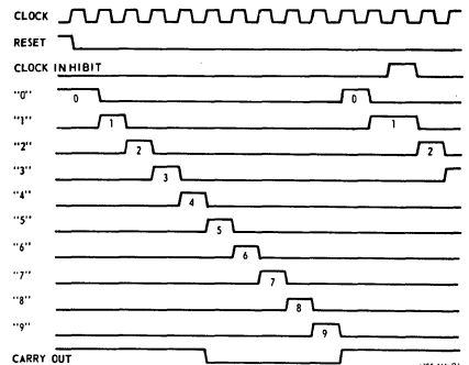
Fig. 2 - Timing diagram.
