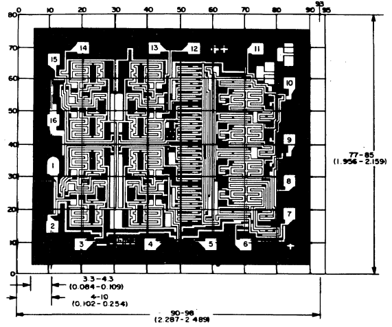
Dimensions and pad layout for CD4051BH. 92CM-27093
