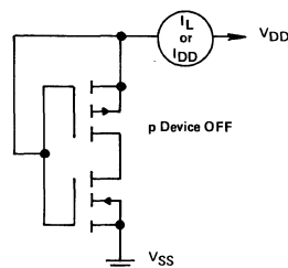
Fig. 8 - Measurement of quiescent leakage current.
