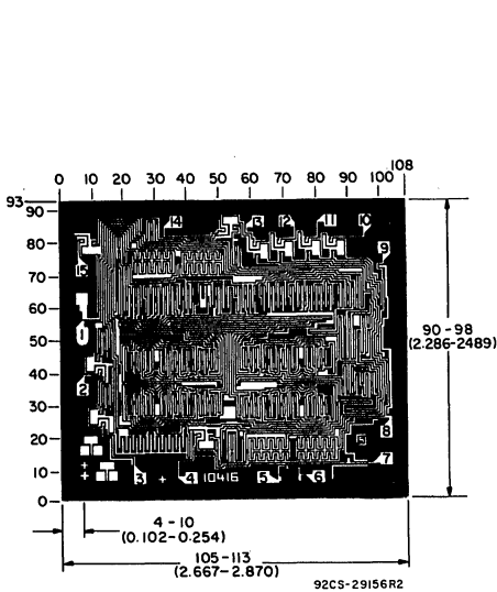
Dimensions and Pad Layout for CD4089BH
