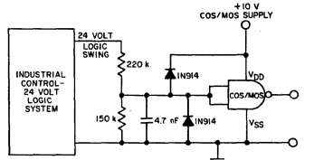
Fig. 12—Industrial control to COS/MOS interface.
