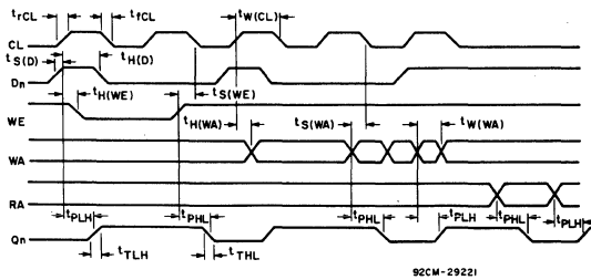
Fig. 3 — Timing diagram.
