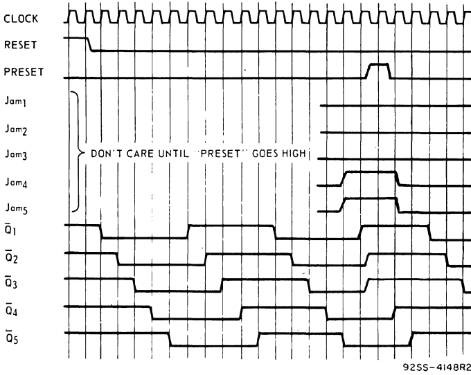
Fig. 15 — Timing diagram.
