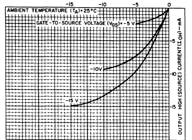
Fig. 5 - Minimum output high (source) current characteristics.
