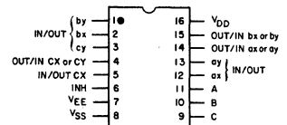
92CS-24484 CD4053B Terminal Assignment
