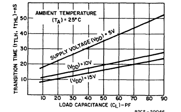
Fig. 12 - Typical transition time vs. C_L - true output.
