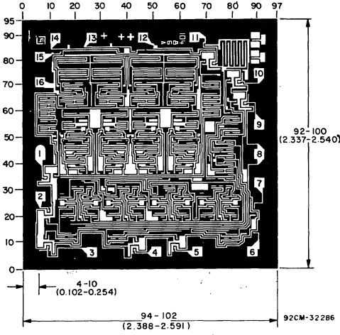
Dimensions and pad layout for CD40104BH
