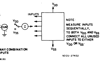
Fig. 11 — Input current test circuit.
