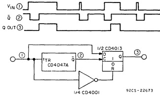
Fig. 23 - Noise-discriminator circuit.
