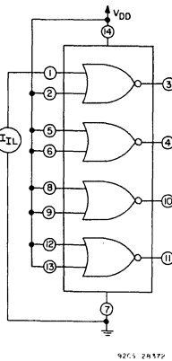
Fig. 14 - Input-current test circuit for the CD4001A, input low ( I_{IL} ).
