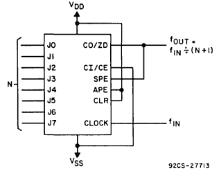
Fig. 18 - Divide-by-"N" counter.
