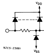
Fig. 1 - Logic diagram - 1 of 4 Schmitt triggers.
