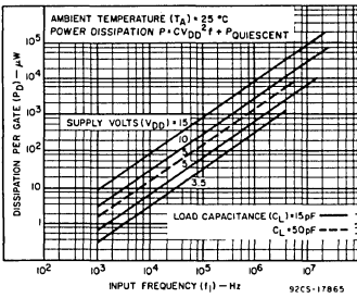
Fig. 14 - Typical power dissipation vs. frequency.
