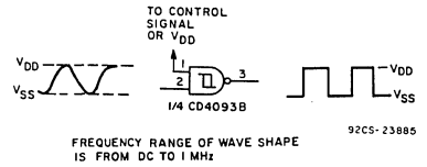
Fig. 16 — Wave shaper.
