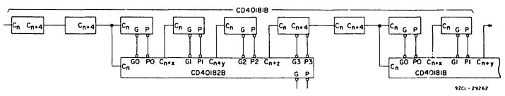
Fig. 15 – Combined two-level look-ahead and ripple-carry ALU.
