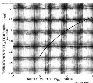
Fig. 12—Variation of normalized output low (sink) current I_{OL} and output high (source) current I_{OH} with supply voltage.
