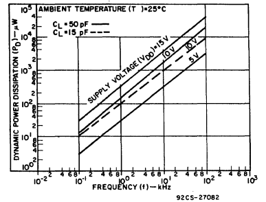
Fig. 7 - Typical dynamic power dissipation characteristics.
