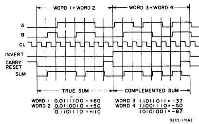
Fig.2 - CD4032B timing diagram.
