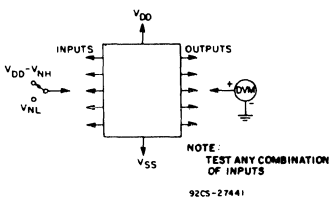
Fig. 15 — Noise-immunity test circuit.
