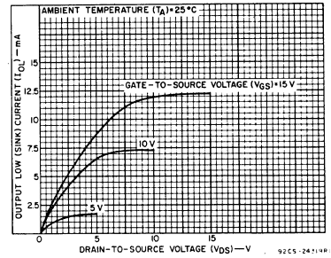
Fig. 5—Minimum n-channel output low (sink) current characteristics.
