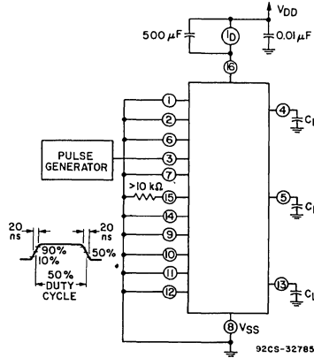
Fig. 20—Dynamic power dissipation test circuit and waveform.
