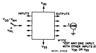
Fig. 12 — Noise immunity test circuit.
