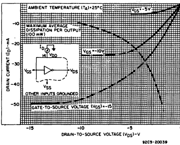
Fig. 5 - Typical output p-channel drain characteristics - complement output.
