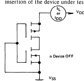
Fig. 8 - Measurement of quiescent leakage current.
