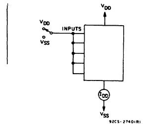
Fig. 9 - Quiescent device current test circuit.
