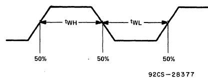
Fig. 26 — Waveform used to define pulse widths.
