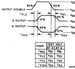
Fig. 14 — Output disable test circuit and waveforms.
