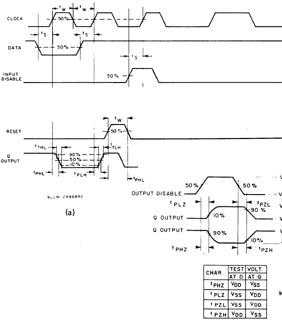
Fig.5 — Functional waveforms for CD4076B.
