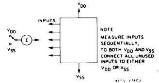
Fig. 19 — Input current test circuit.
