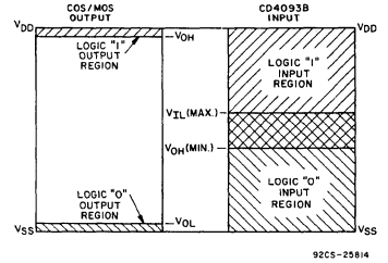
Fig. 4 - Input and output characteristics.
