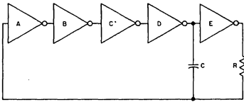
Fig. 8 - CD4047A oscillator section
