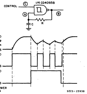
Fig.18 - Gated stable oscillator.
