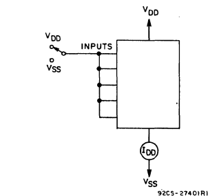
Fig. 10—Quiescent-device-current test circuit.
