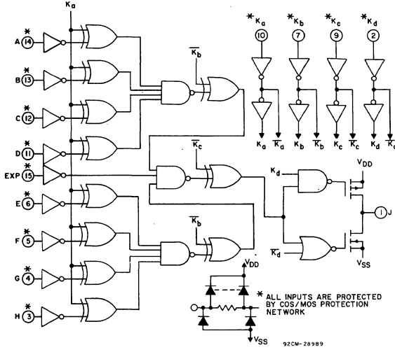
Fig. 2 – Logic diagram.
