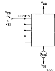
Fig. 17 - Quiescent device current test circuit.
