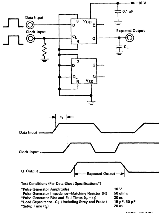
Fig. 25 — Set-up-time test circuit for a CD4013A.
