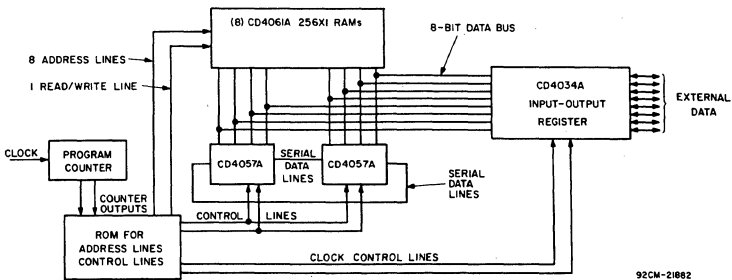
Fig. 18 - Example of computer organization using CD4057A.
