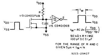
Fig. 17 - Monostable multivibrator.
