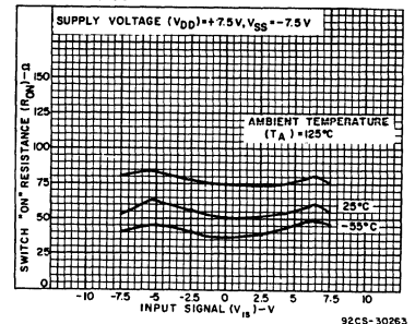
Fig. 4— Typical ON resistance as a function of input signal voltage at V_{DD} = +7.5\text{ V} , V_{SS} = -7.5\text{ V} .
