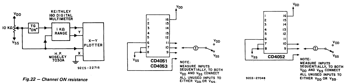
Fig. 23 - Input current.
