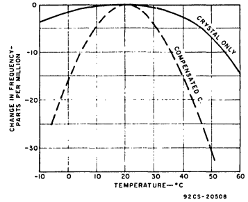
Fig. 7— Effect of temperature on crystal frequency.
