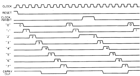
Fig. 4 - Timing diagram for CD4022B.
