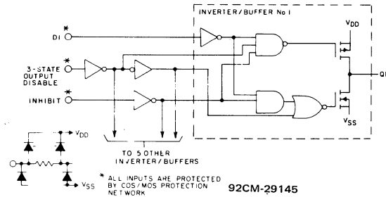
Fig. 1 — Logic diagram of 1 of 6 identical inverter/buffers.
