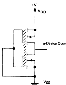
Fig. 6 - Schematic representations of p and n devices when turned off.
