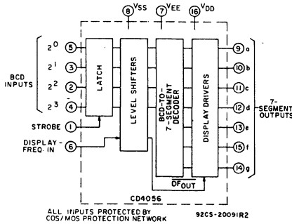
Fig.3 - CD4056B functional diagram.
