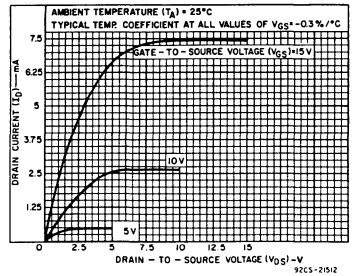
Fig. 2 - Minimum n-channel drain characteristics.
