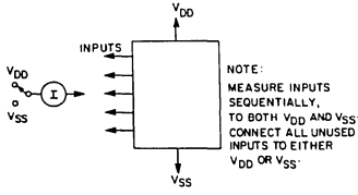
Fig. 15 – Input current test circuit.
