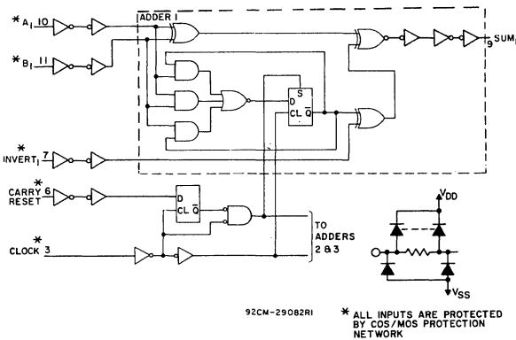
Fig.1 - CD4032B logic diagram of one of three serial adders.
