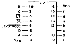
TOP VIEW 92CS-25084R1 CD4511B TERMINAL ASSIGNMENT
