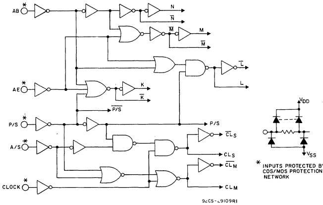
Fig. 1 - Steering logic diagram.
