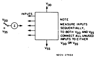
Fig.7 – Input current test circuit.
