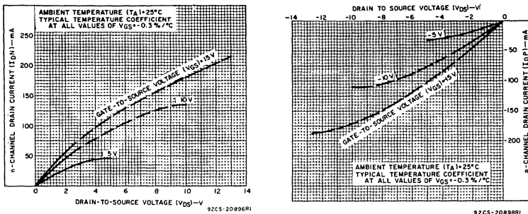
Fig. 2 - Typical output n-channel and p-channel drain characteristics of the CD4045.
