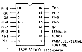
TERMINAL DIAGRAM CD4014B, CD4021B
