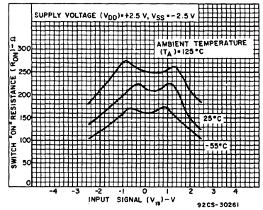
Fig. 2— Typical ON resistance as a function of input signal voltage at V_{DD} = +2.5\text{ V} , V_{SS} = -2.5\text{ V} .
