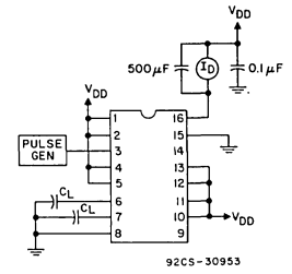
Fig. 9 – Dynamic power dissipation test circuit.
