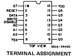
TERMINAL ASSIGNMENT
