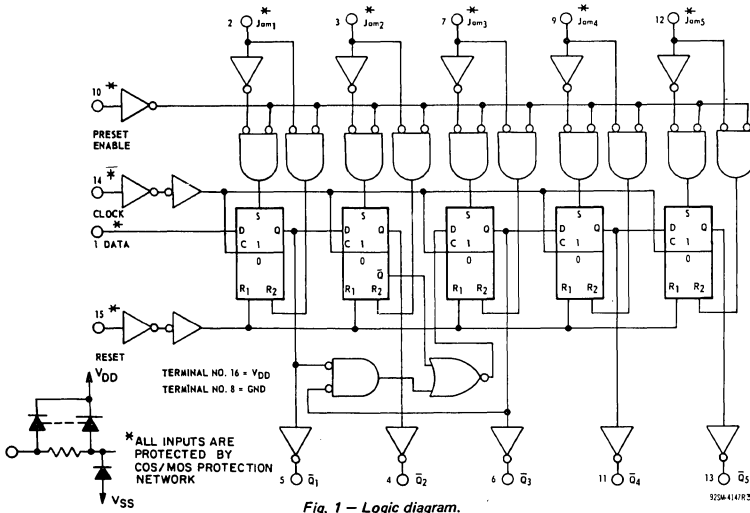
Fig. 1 - Logic diagram.
