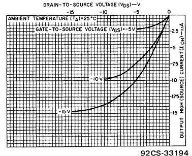
Fig. 10 - Typical p-channel output high (source) current characteristics.
