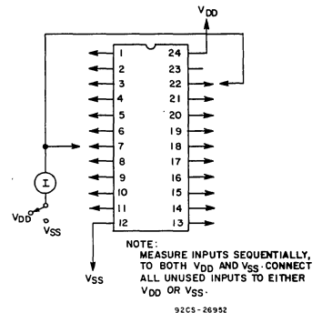
Fig. 20 – Input leakage current test circuit.
