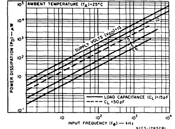
Fig. 5 — Typical dissipation characteristics. (per output).
