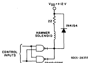
Fig. 9 - Solenoid driver circuit.
