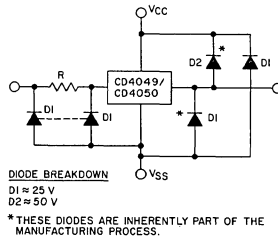
Fig. 3 — Modified protection network.
