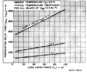
Fig. 4 - Typical propagation delay time vs. load capacitance.
