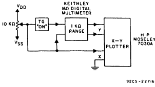
Fig. 13—Channel ON resistance measurement circuit.
