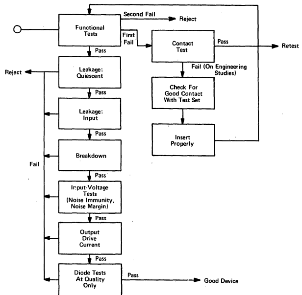
Fig. 2 - A typical COS/MOS IC test sequence.
