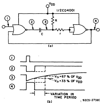
Fig. 11 - Basic one-shot multivibrator circuit: (a) circuit diagram, (b) waveforms.
