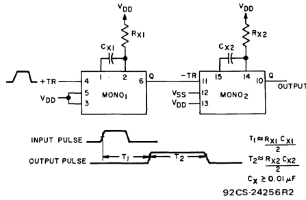
Fig. 15 - Pulse delay.
