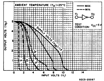
Fig. 3 — Minimum and maximum voltage transfer characteristics—CD4009UB.
