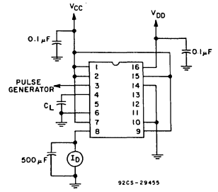
Fig. 16 - Dynamic power dissipation test circuit.
