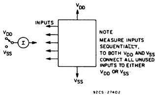
Fig. 14 — Input leakage current test circuit.
