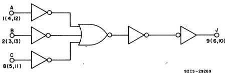
Fig. 13 - Logic diagram for CD4073B (1 of 3 identical gates).
