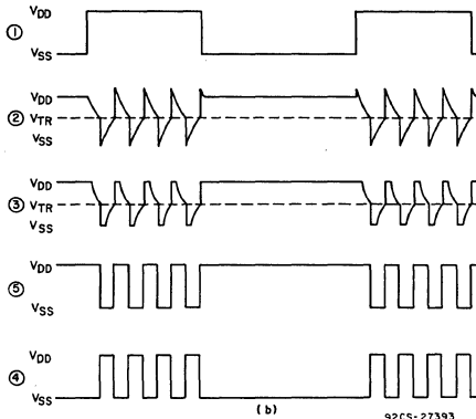
Fig. 24 - (a) Modulator circuit, (b) waveforms.
