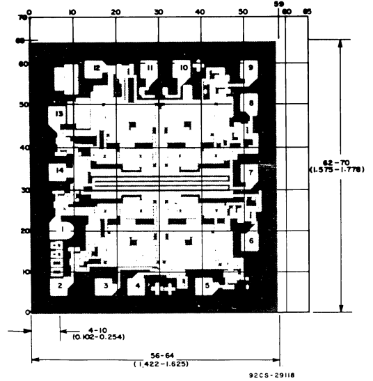
Dimensions and pad layout for CD4071B.
