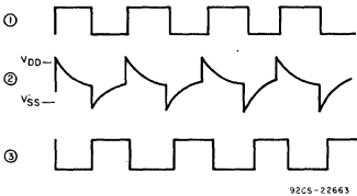
Fig. 2—RC-oscillator operating waveforms.
