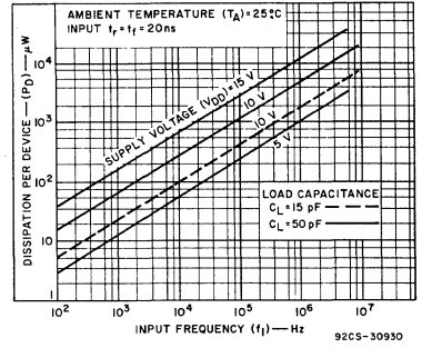
Fig. 9 - Typical power dissipation vs. frequency.
