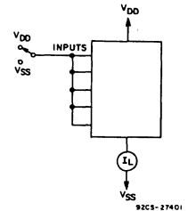
Fig. 6—Quiescent-device-current I test circuit.
