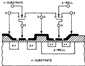
Fig. 1 - Cross-section of COS/MOS transistor.
