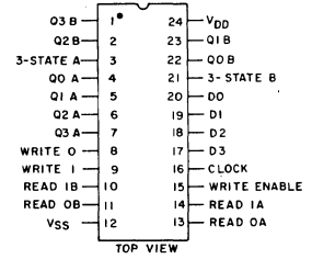
TERMINAL ASSIGNMENT
