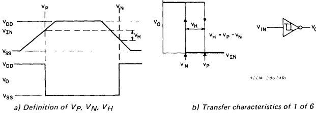
Fig.6 - Hysteresis definition, characteristics, and test set-up.
