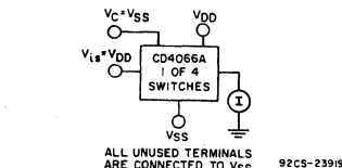
Fig. 7 - OFF switch input or output leakage.
