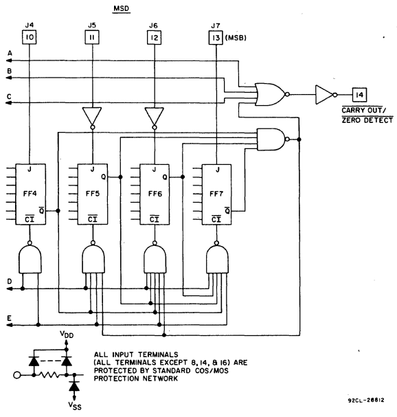
Fig. 12 - Logic diagram for CD40102B.
