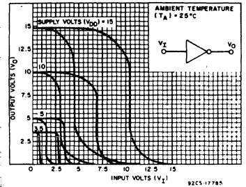
Fig. 1 - Minimum and maximum voltage-transfer characteristics for inverter.
