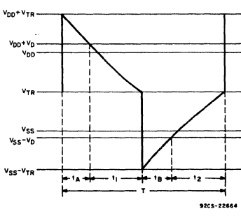
Fig. B-1 - RC waveform for the circuit of Fig. 4.
