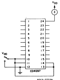
Fig. 10—Quiescent device current.
