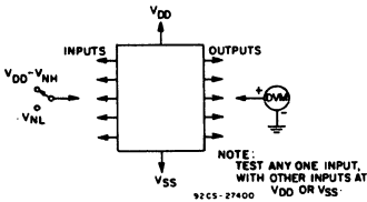
Fig. 11 – Noise-immunity test circuit.
