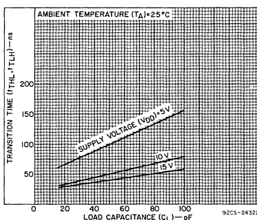
Fig. 15—Variation of transition time ( t_{TLH} , t_{THL} ) with load capacitance.
