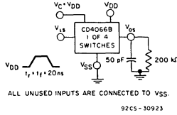
Fig. 12 - Propagation delay time signal input ( V_i ) to signal output ( V_o ).
