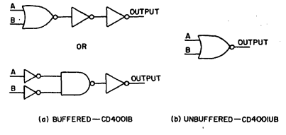
Fig. 1 — Examples of the buffered (CD4001B) and unbuffered (CD4001UB) 2-input NOR gate.
