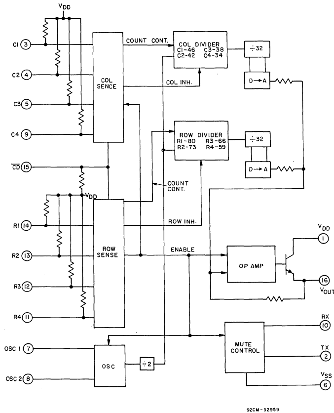
Fig. 2 - Touch-tone generator.
