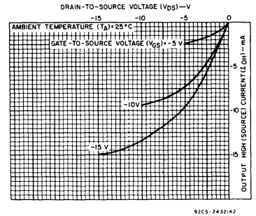
Fig. 11 - Minimum output high (source) current characteristics.
