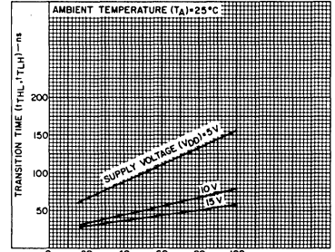
Fig. 5 — Typical transition time as a function of load capacitance.
