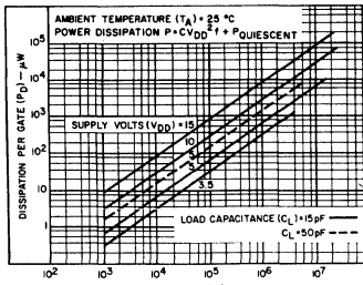
Fig. 18 — Typical dissipation characteristics.
