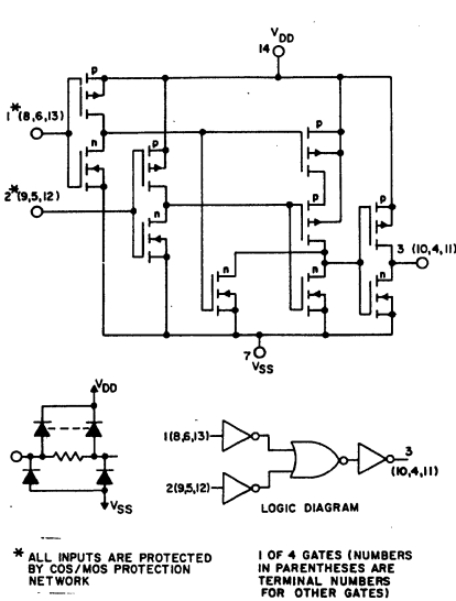
Fig. 7 - Schematic and logic diagrams for CD4011B.
