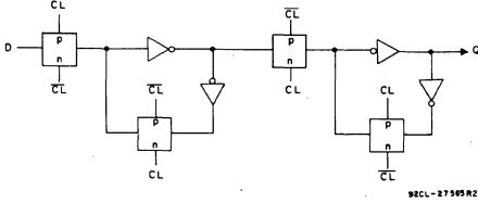
Fig. 3 - Logic diagram.
