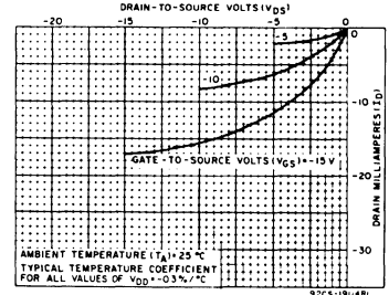
Fig. 2 — Typical output p-channel drain characteristics for Q output.
