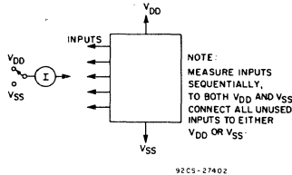
Fig. 9 — Input current test circuit.
