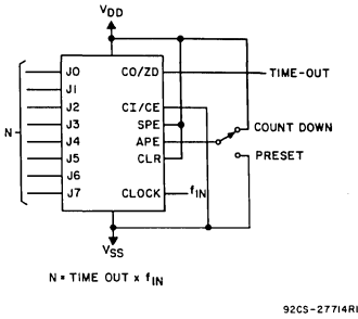
Fig. 19 - Programmable timer.
