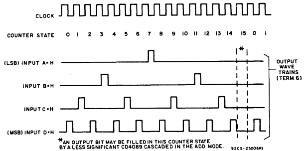
Fig. 15 — Timing diagram.
