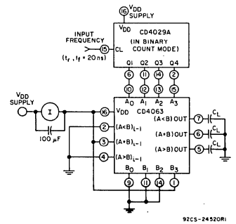
Fig. 12 — Dynamic power dissipation test circuit.
