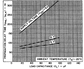
Fig. 8 - Typical propagation delay time vs. load capacitance—clock to \bar{Q}
