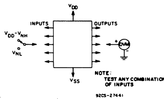
Fig. 13 — Noise immunity test circuit.
