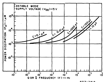
Fig. 32 - Power dissipation vs output frequency ( V_{DD} = 15 V).
