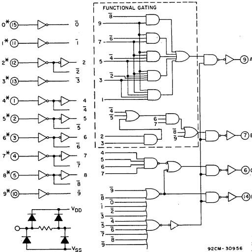
* INPUTS PROTECTED BY COS/MOS PROTECTION NETWORK Fig. 1 — CD40147B logic diagram.
