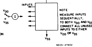
Fig. 11 – Input current.
