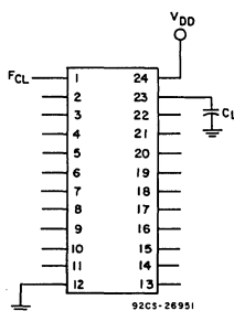
Fig. 19 – Power dissipation test circuit (all ÷ modes).
