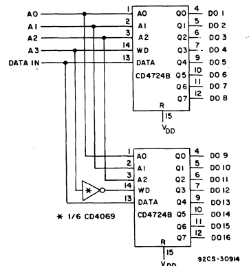
Fig. 14— 1 of 16 decoder/demultiplexer.
