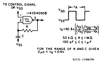
Fig. 18 — Astable multivibrator.
