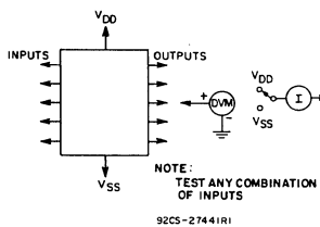
Fig. 14 — Input voltage test circuits.
