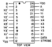
92CS-29839 Top View CD22101 Terminal Diagram
