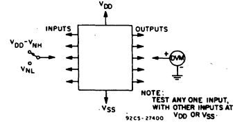
Fig. 11 – Noise-immunity test circuit.
