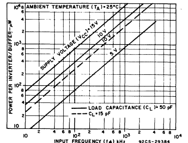
Fig. 10 — Typical power dissipation vs. frequency characteristics.
