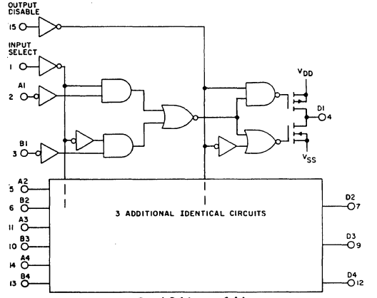
Quad 2-Line-to-1-Line Data Selector/Multiplexer CD40257B (Page 438)
