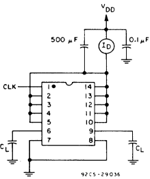
Fig. 9 - Dynamic power dissipation test circuit.
