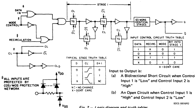
Fig. 7 - Logic diagram and truth tables.
