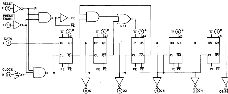
Fig. 1 - Logic diagram.
