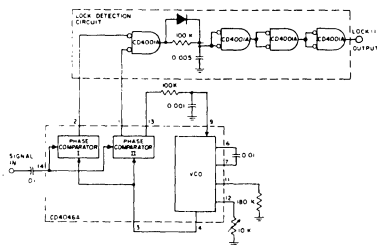
Fig. 15— Lock-detection circuit.
