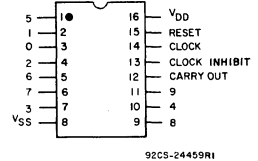
TOP VIEW CD4017B TERMINAL DIAGRAM
