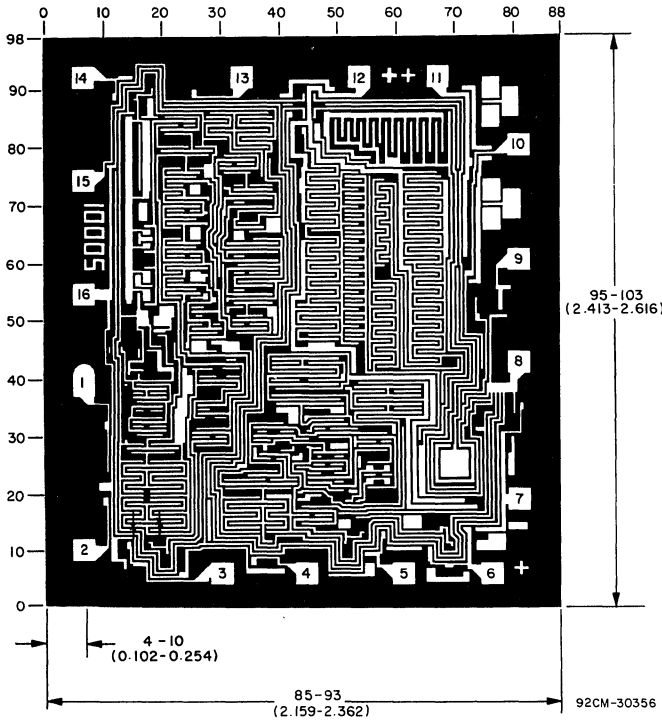
Dimensions and pad layout for CD4046BH.
