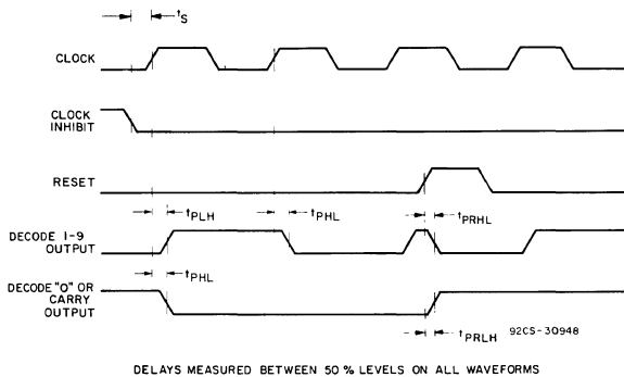
Fig. 9— Propagation delay, setup, and hold time waveforms.
