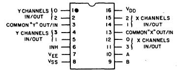
92CS-24483 CD4052B Terminal Assignment
