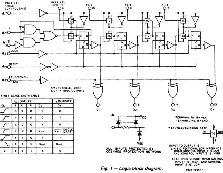
Fig. 1 - Logic block diagram.
