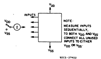
Fig. 11 — Input-leakage-current test circuit.
