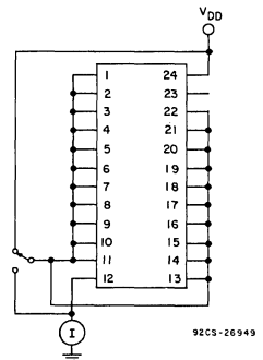
Fig. 17 – Quiescent device current test circuit.
