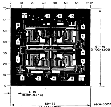
Dimensions and pad layout for CD4030BH.
