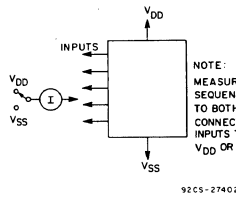
Fig. 11 - Input-leakage current.
