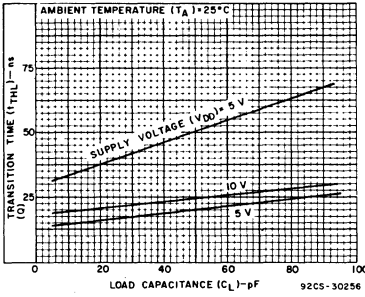
Fig. 9 - Typical transition time as a function of load capacitance ( C_L , t_{THL} ).
