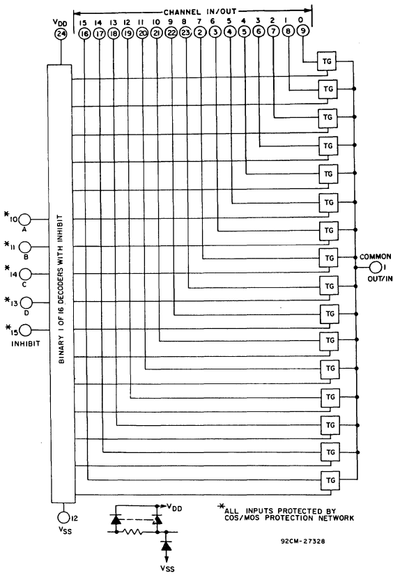
Fig. 16—CD4067 logic diagram.
