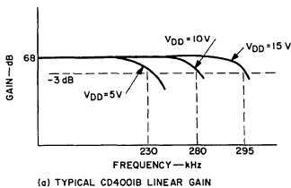
(a) TYPICAL CD4001B LINEAR GAIN
