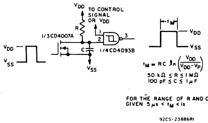
Fig. 17 — Monostable multivibrator.
