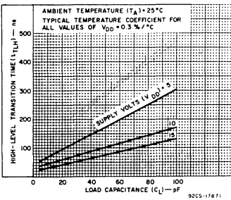
Fig. 16 — Typical low-to-high level transition time vs. C_L .
