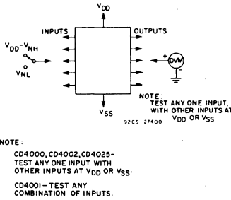
Fig. 13 — Noise immunity test circuit.
