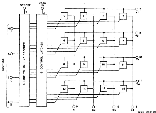
Fig. 1 – Functional diagram.
