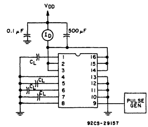
Fig. 11 - Dynamic power dissipation test circuit.
