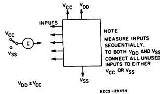
Fig. 15 - Input current.
