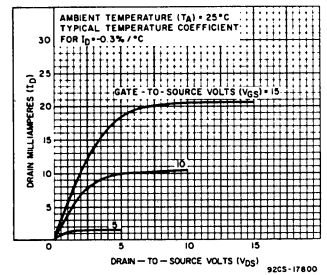
Fig. 2 — Typical n-channel drain characteristics.
