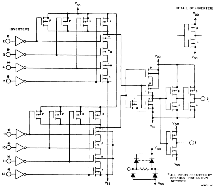
Fig. 8 - Schematic diagram.
