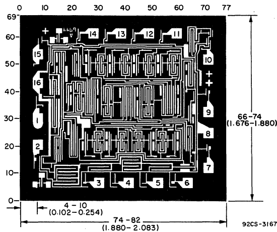
Dimensions and pad layout for CD4048BH.
