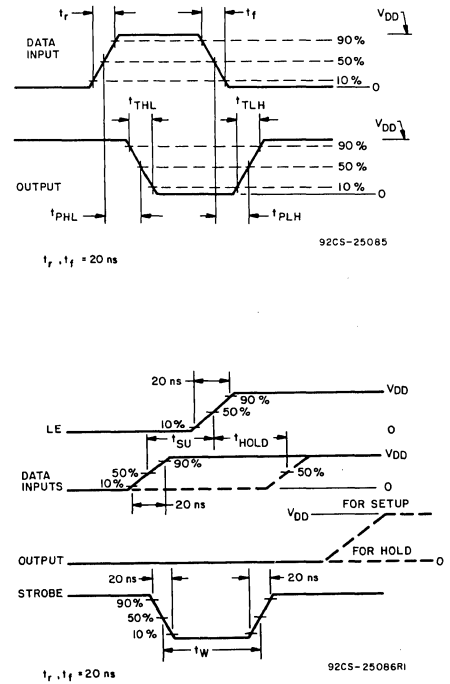
Fig. 14 - Dynamic waveforms.
