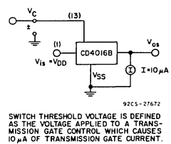
Fig. 23 - Switch threshold voltage.
