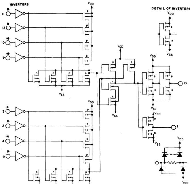
Fig. 7 - Schematic diagram.
