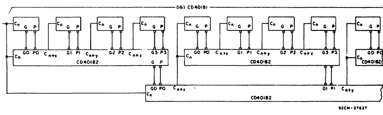
Fig. 14 – 64-Bit full carry look-ahead ALU in 3 levels.
