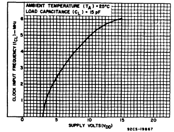
Fig. 7 — Typical clock input frequency vs. supply voltage.
