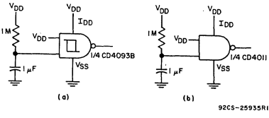
Fig.15 - Reset circuit; a comparison of the CD4093B with the CD4011.
