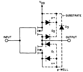
Fig. 4 - Basic inverter showing parasitic diodes.
