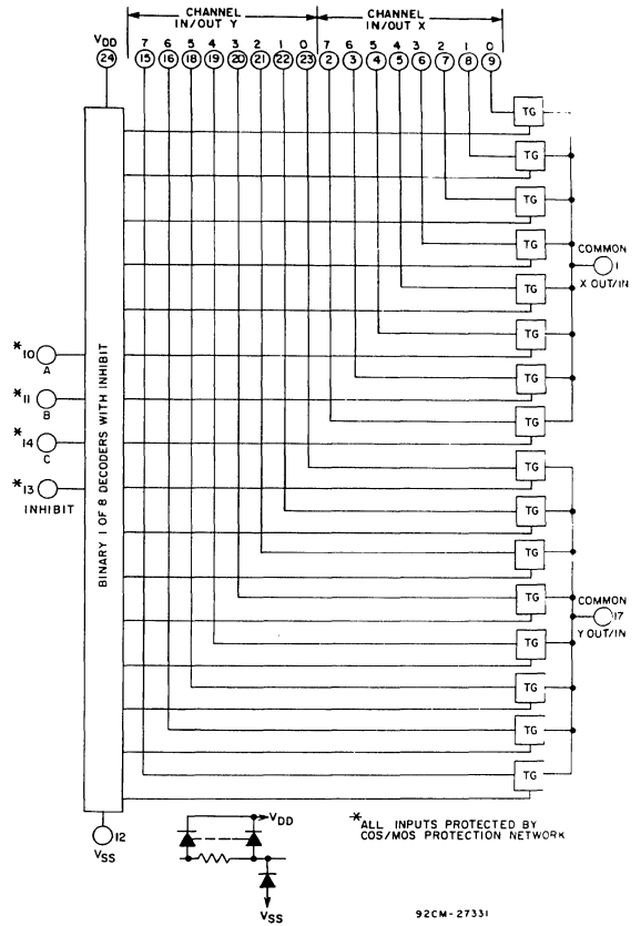
Fig. 17—CD4097 logic diagram.
