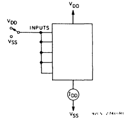
Fig. 12 - Quiescent-current test circuits.
