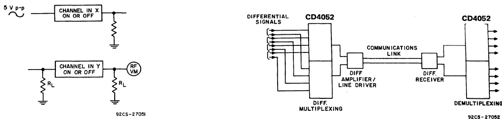
Fig. 26 - Crosstalk between duals or triplets (CD4052B, CD4053B).
