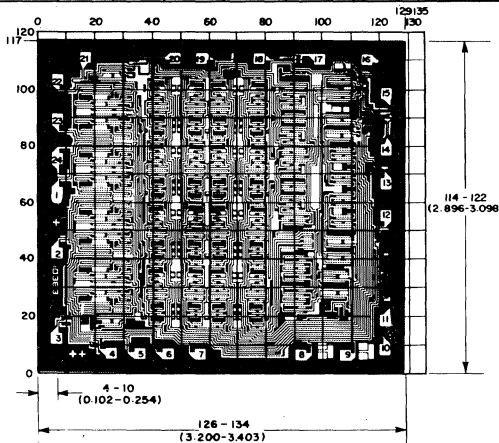
Dimensions and Pad Layout for CD40108BH
