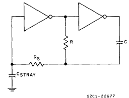
Fig. 7—RC-oscillator circuit with stray capacitance.
