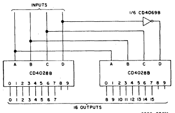
Fig. 13 — Code conversion circuit.
