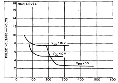
Fig. 5 - Voltage noise immunity of the CD4093B.
