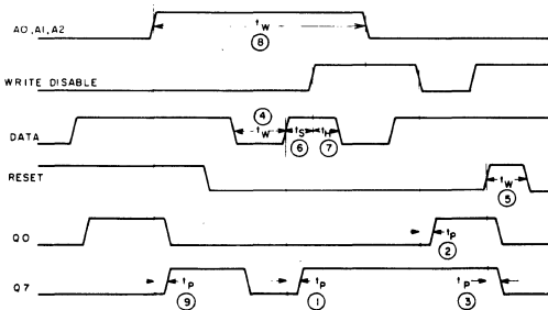
Fig. 15 — Master timing diagram.
