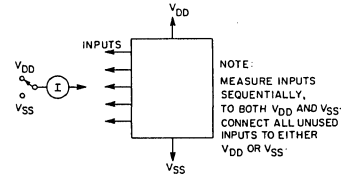
Fig. 16 – Input current.
