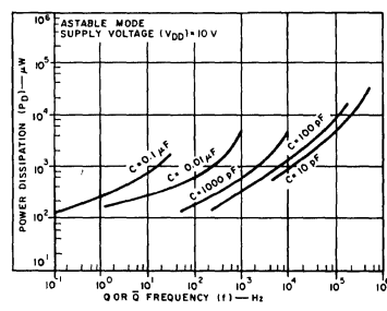
Fig. 31 - Power dissipation vs output frequency ( V_{DD} = 10 V).
