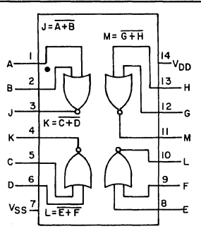
Quad 2-Input NOR Gate
