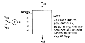
Fig. 11 — Input-current test circuit.
