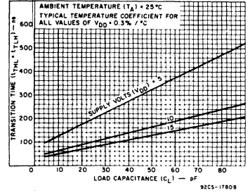
Fig. 3 - Typical transition time vs. load capacitance.
