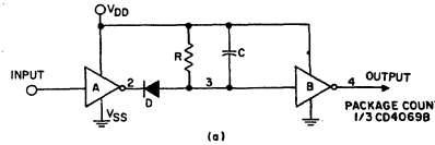
Fig. 24 - (a) Modulator circuit, (b) waveforms.
