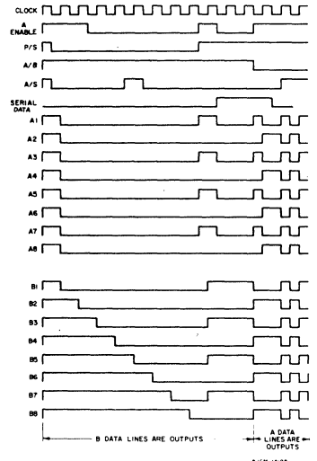
Fig. 3 — Timing diagram.
