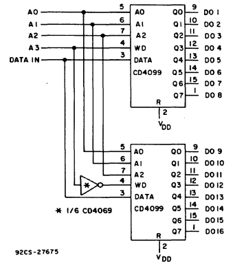
Fig. 14 — 1 of 16 decoder/demultiplexer.
