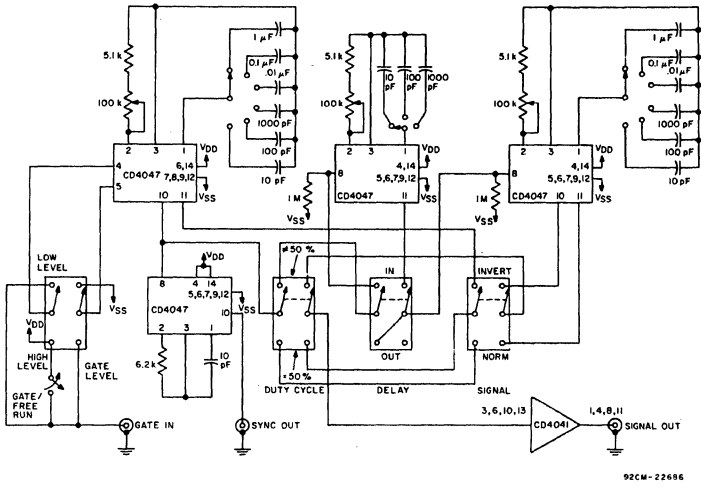
Fig. 34 - Pulse-generator circuit.
