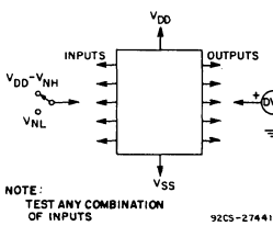
Fig. 6 - Noise-immunity test circuit.
