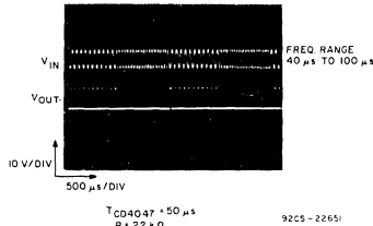
Fig. 28 - Low-pass filter-circuit waveforms.
