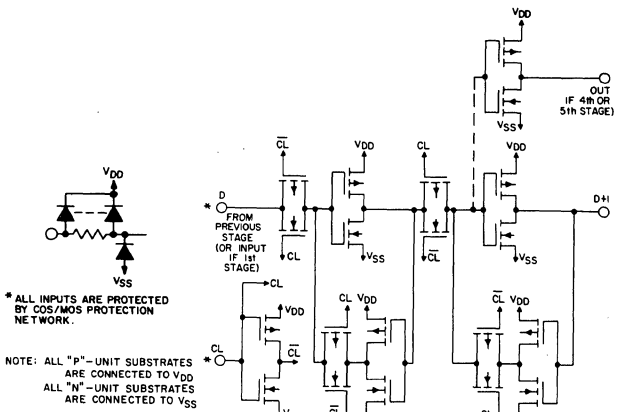
Fig. 4 - Schematic diagram (one register stage).
