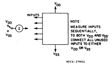
Fig. 15 - Input-leakage current.
