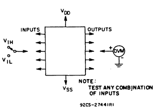
Fig. 10 — Input voltage test circuit.
