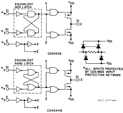
Fig. 1 - Logic diagrams.
