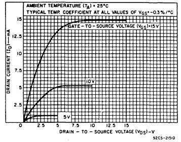
Fig. 1 - Typical n-channel drain characteristics.
