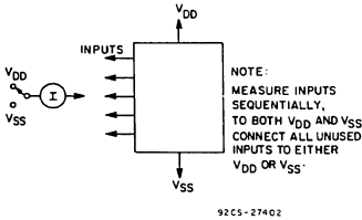
Fig. 16 - Input current test circuit.
