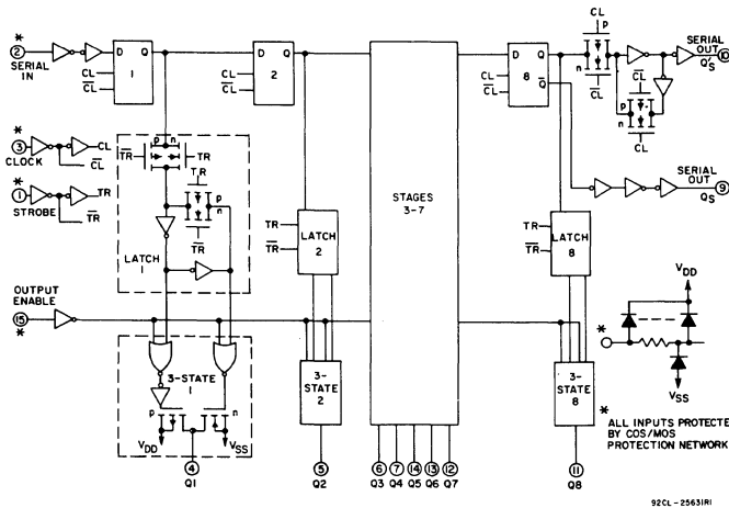
Fig. 2 — CD4094B Logic diagram.
