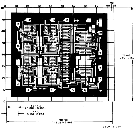
Dimensions and pad layout for CD4052BH.
