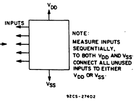
Fig. 12 – Input current test circuit.
