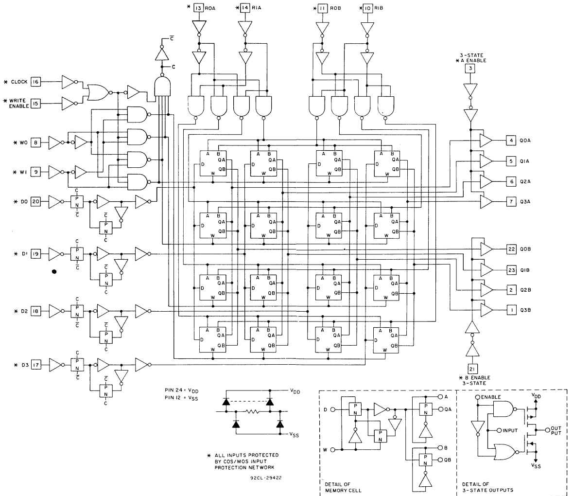
Fig. 13— Schematic diagram
