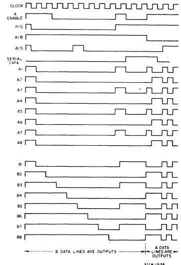
Fig. 4 - Timing diagram.
