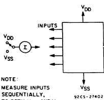
Fig. 22 - Input current test circuit.
