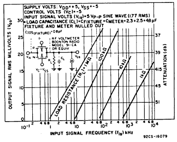
Fig. 8—Typ. feedthru vs. frequency—switch off.
