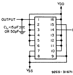
Fig. 17 - Test circuit for t_{PHL} , t_{THL} , and t_{TLH} (AND) measurements.
