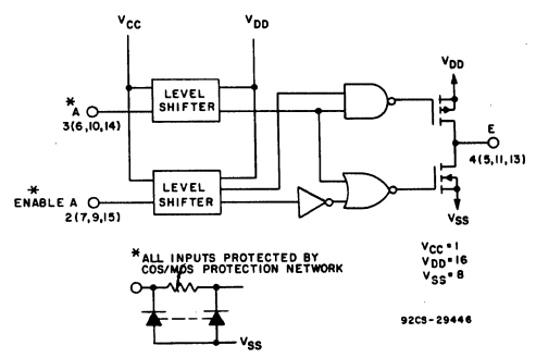
Fig. 1 - CD40109B logic diagram (1 of 4 units).
