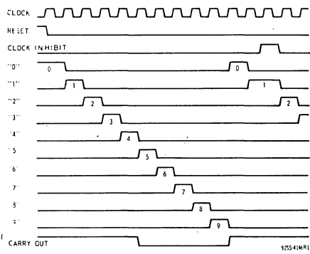
Fig. 2 - Timing diagram for CD4017B.
