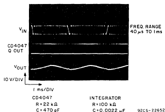
Fig. 26 - Frequency-discriminator-circuit waveforms.
