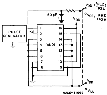
Fig. 20 - Test circuit for t_{PZL} , t_{PZH} , t_{PLZ} , and t_{PHZ} (AND).
