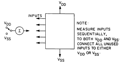
Fig. 31—Input-leakage-current test circuit.
