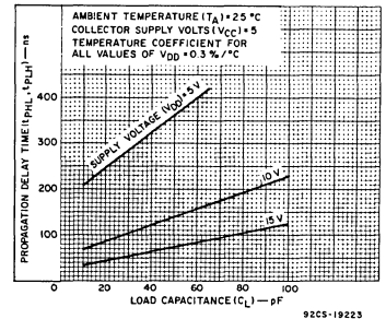
Fig. 5 — Typical propagation delay time vs. load capacitance.
