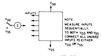
Fig. 11 — Input-leakage-current test circuit.
