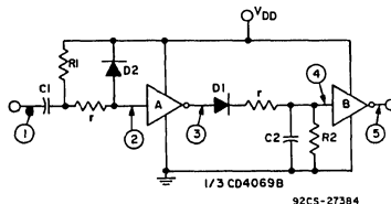
Fig. 12 - Compensated monostable multivibrator circuit.
