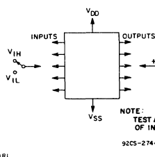
Fig. 10 — Input voltage test circuit.
