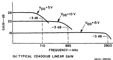
Fig. 8 — Typical linear-mode gain of buffered and unbuffered 2-input NOR gate.
