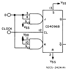
Fig. 17 - CD4096B connected as a "D" type flip-flop.
