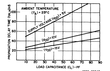
Fig. 15 - Typical low-to-high level propagation delay time vs. C_L - complement output.
