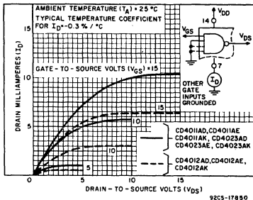
Fig. 2a - Typical n-channel characteristics.
