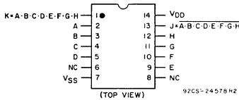
TERMINAL ASSIGNMENT
