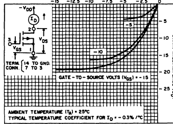
Fig. 6 - Typical output p-channel drain characteristics.
