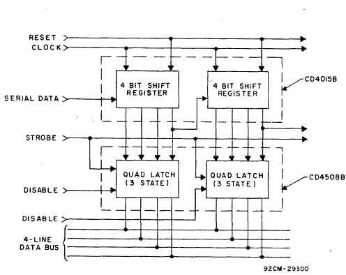
Fig. 15 — Bus register.
