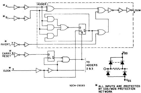
Fig. 3 — CD4038B logic diagram of one of three serial adders.
