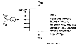
Fig. 8 — Input-leakage-current test circuit.
