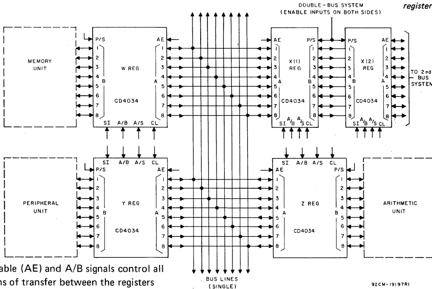
Fig. 19 — Single- and double-bus systems.
