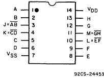
TOP VIEW CD4011UB
