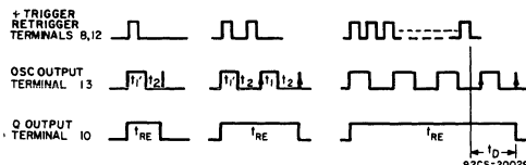
Fig. 29 - Retrigger-mode waveforms.
