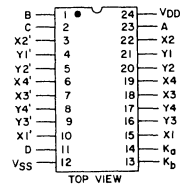
92CS-29840 Top View CD22102 Terminal Diagram
