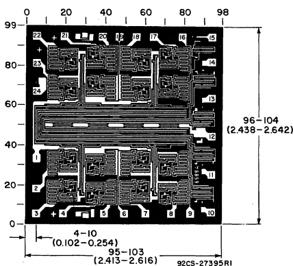
Dimensions and pad layout for CD4067BH.
