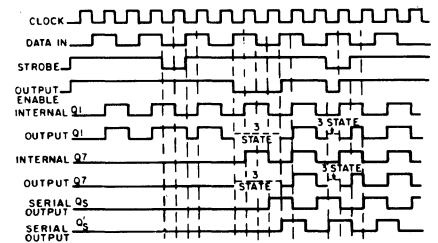
Fig. 3 — Timing diagram.
