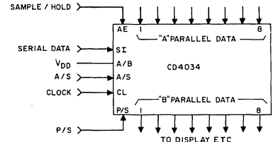
Fig. 22 - Sample and hold register-serial/parallel in-parallel out.
