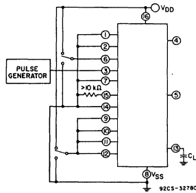
Fig. 21—Switching time test circuit.
