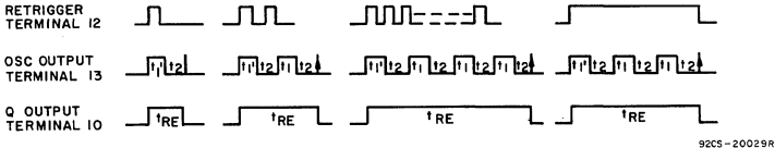
Fig. 34—Retrigger-mode waveforms.
