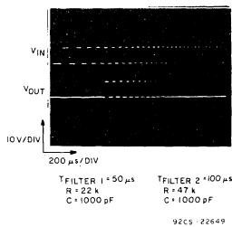
Fig. 31 - Bandpass-filter-circuit waveforms.
