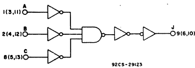
Fig. 13 - Logic diagram for CD4075B (1 of 3 identical gates).
