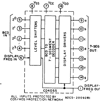
Fig.2 - CD4055B functional diagram.
