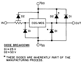
Fig. 1 — Standard protection network.
