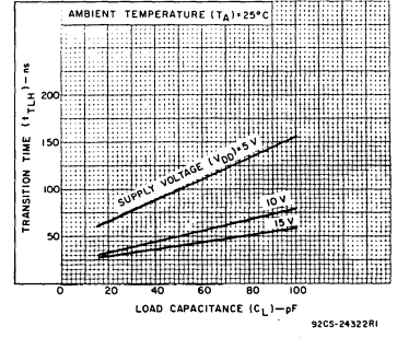
Fig.9 - Typical low-to-high transition time vs. load capacitance.
