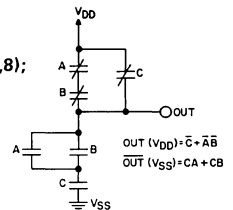
Fig. 2 - Sample COS/MOS logic circuit arrangements using type CD4007UB.
