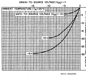
Fig. 10 - Typical output high (source) current characteristics.
