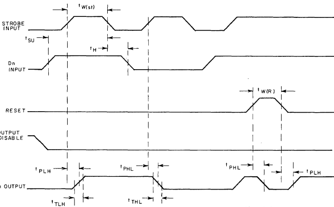
Fig. 12 — Test waveforms.
