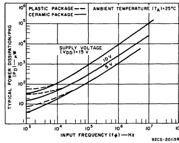
Fig. 6 - Typical dissipation vs input frequency (21 counting stages).
