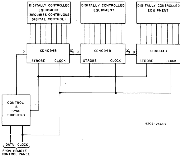
Fig. 14 - Remote control holding register.
