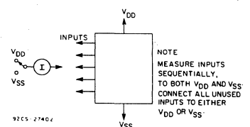
Fig. 14 — Input current test circuit.
