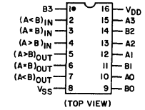
92CS-24523 TERMINAL ASSIGNMENT
