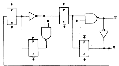
Fig. 2 - Detail of typical flip-flop stage.
