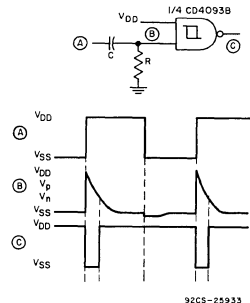
Fig.13 - Rising-edge detector.
