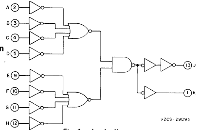
Fig. 1 - Logic diagram.
