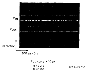
Fig. 29 - Low-pass-circuit waveforms.
