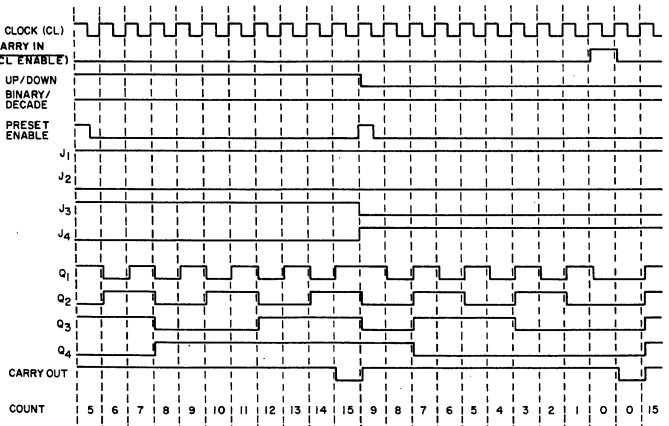
Fig. 10 - Timing diagram-binary mode.
