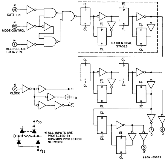
Fig. 1 - Logic diagram.
