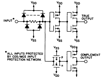
Fig.1 - Schematic diagram 1 of 4 buffers.
