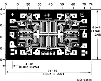
Dimensions and Pad Layout for CD4093BH
