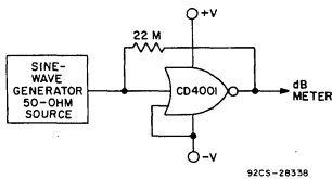
Fig. 7 — Linear-gain test circuit.
