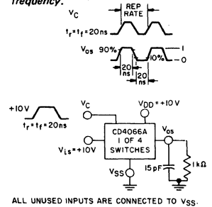
Fig. 10 - Maximum allowable control input repetition rate.
