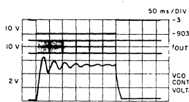
Fig. 13— Frequency-synthesizer waveforms.
