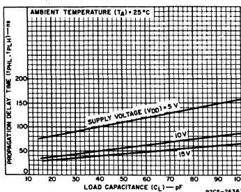
Fig. 6 - Typical propagation delay (E l to G S , E l to E O ) vs. load capacitance.
