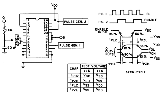
Fig. 14— Output-enable-delay-times test circuit and waveforms.
