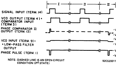
Fig. 10 — Typical waveforms for COS/MOS phase-locked loop employing phase comparator II in locked condition.
