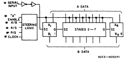
Fig. 1 - Functional diagram.
