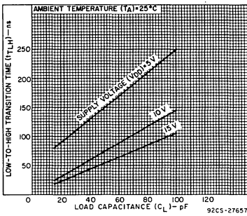
Fig. 17 - Typical low-to-high transition time vs. load capacitance.
