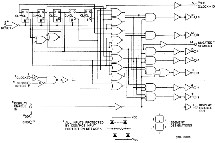
Fig. 1 - CD4026B logic diagram.
