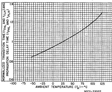
Fig. 13—Variation of low-to-high ( t_{TLH} ) and high-to-low ( t_{THL} ) transition time, and low-to-high ( t_{PLH} ) and high-to-low ( t_{PLH} ) propagation delay time with temperature.
