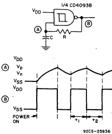
Fig.16 - Astable multivibrator.
