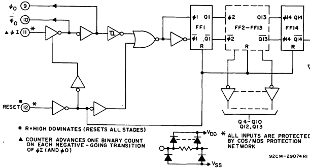
Fig. 1 - Logic diagram.
