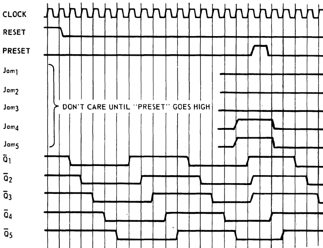
Fig. 2 - Timing diagram.
