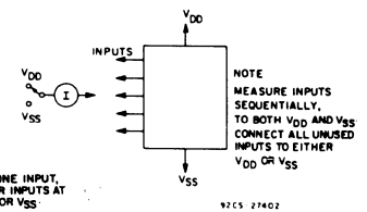
Fig. 21 — Input leakage current test circuit.
