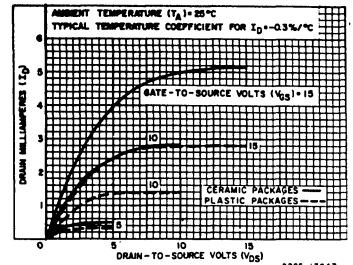
Fig. 8 - Minimum n-channel drain characteristics - CD4011A & CD4023A.
