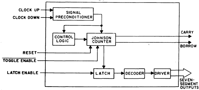
Fig. 1—Functional diagram.
