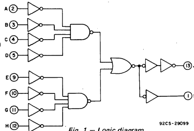
Fig. 1 - Logic diagram.
