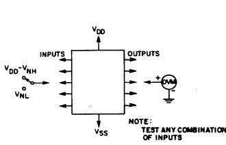
Fig. 14 — Noise immunity test circuit.
