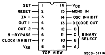
Terminal Assignment
