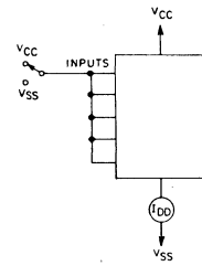
Fig. 13 — Quiescent device current test circuit.
