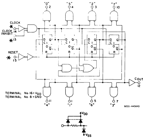
Fig. 1 - Logic diagram.
