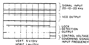
Fig. 16— Lock-detection-circuit waveforms.
