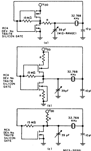
Fig. 9 - Typical COS/MOS crystal-oscillator circuits.
