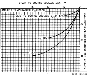
Fig. 7—Minimum p-channel output high (source) current characteristics.
