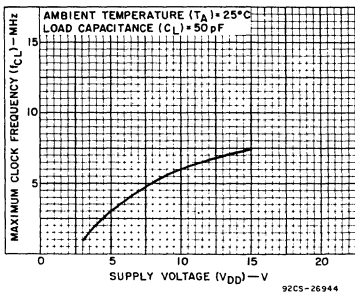
Fig. 11 - Typical max. clock frequency vs. supply voltage.
