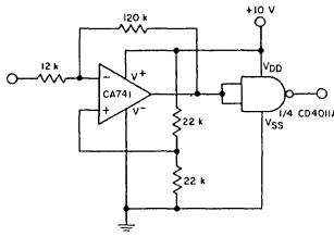
Fig. 21—Interface of op-amp and COS/MOS with common supply rail.
