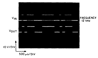
Fig. 33 - Envelope-detector-circuit waveforms.
