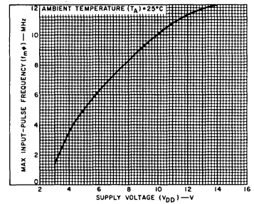
Fig. 10 - Typical maximum input-pulse frequency.
