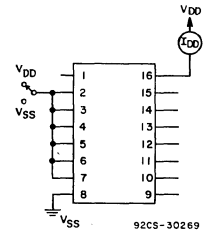
Fig. 11 - Quiescent current test circuit.
