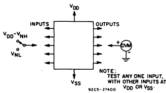
Fig. 10 — Noise immunity test circuit.
