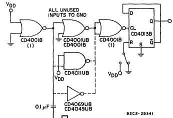
Fig. 6 Test circuit used to evaluate signal-line noise immunity of COS/MOS gates and inverters.
