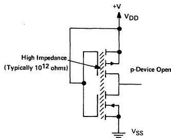
Fig. 6 - Schematic representations of p and n devices when turned off.
