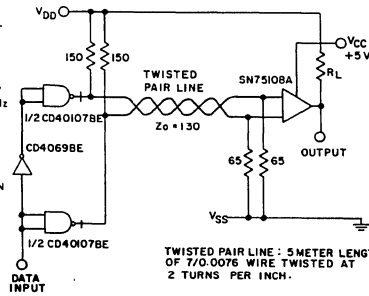
Fig. 14 - Line-driver circuit.
