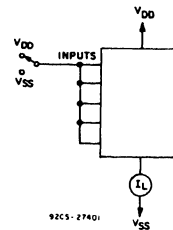
Fig. 11—Quiescent-device-current test circuit.
