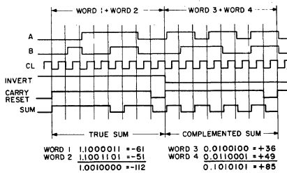
Fig. 4 — CD4038B timing diagram.
