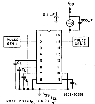
Fig. 11 - Dynamic power dissipation test circuit.
