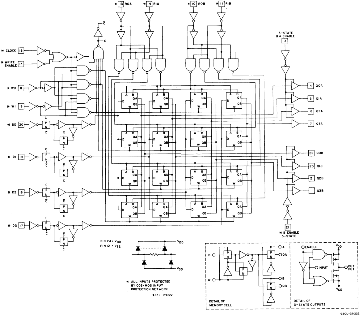
Fig. 2 — Logic diagram.
