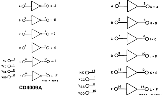
Fig. 1 — Logic diagrams.
