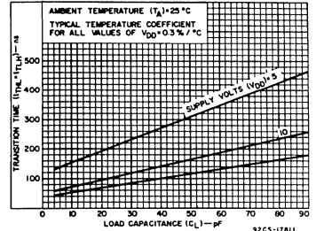
Fig. 9 — Typical transition time vs. C_L .
