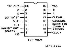
TERMINAL ASSIGNMENT
