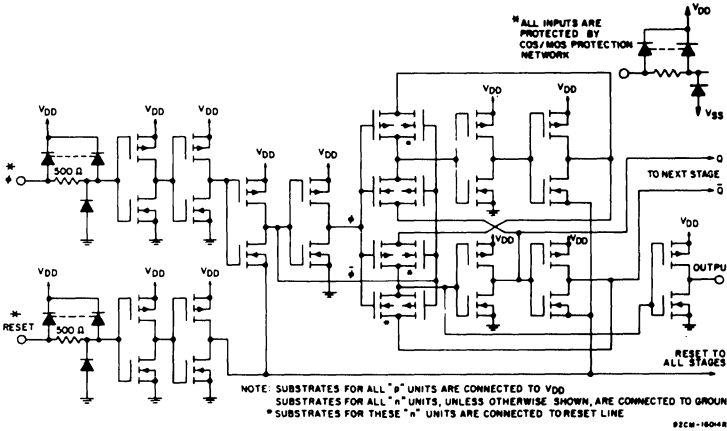
Fig. 2 - Schematic diagram of pulse shapers and 1 of 14 binary stages.
