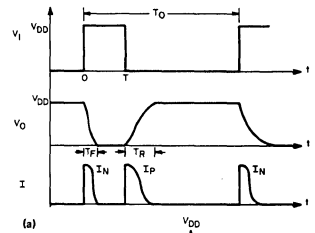
Fig. 6— Typical power dissipation characteristics (a) Basic gate power dissipation characteristics (b) MSI device power dissipation characteristics.
