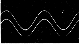
SCALE: X = 0.2 ms/DIV Y = 2.0 V/DIV V_{DD} = V_C = +7.5V, V_{SS} = -7.5V, R_L = 10k\Omega C_L = 15 pF f_{IS} = 1 KHz, V_{IS} = 5V p-p DISTORTION = 0.2 %
