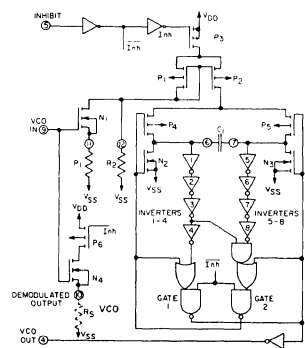
Fig. 8 - Schematic of COS/MOS VCO section.
