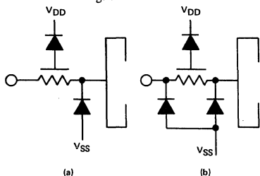
Fig. 7 - (a) Standard and (b) improved protection networks.
