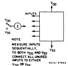
Fig. 8—Input-leakage-current test circuit.
