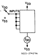
Fig. 15 - Quiescent device current test circuit.
