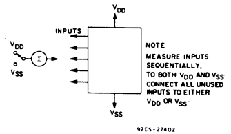
Fig. 12 - Input current.
