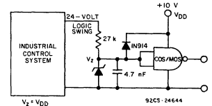
Fig. 13—Zener diode industrial control interface.
