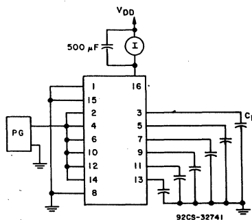
Fig. 9—Dynamic power dissipation test circuit.
