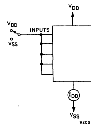
Fig. 14 - Quiescent-device-current test circuit.
