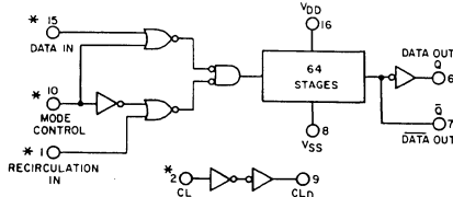
Fig. 12 — Functional diagram.
