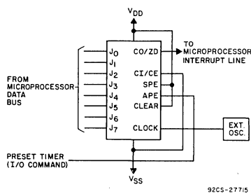
Fig. 20 - Microprocessor interrupt timer.
