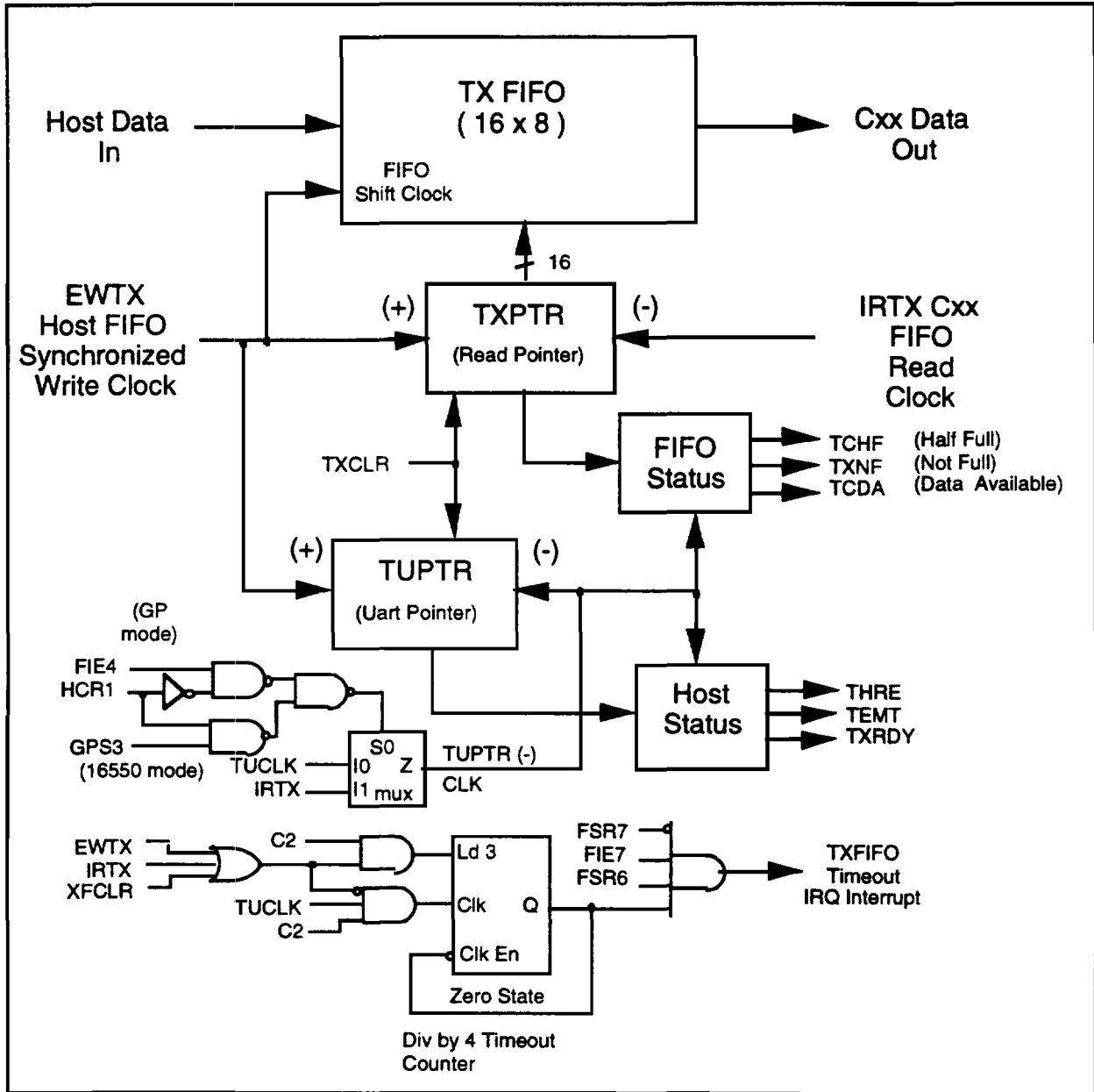
Figure 3-19. TX FIFO Block Diagram
