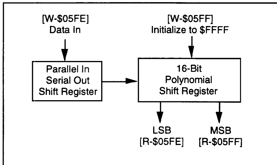
Figure 3-22. CRC Operation
