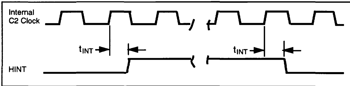
Figure 5-4. Host Bus HINT Waveforms
