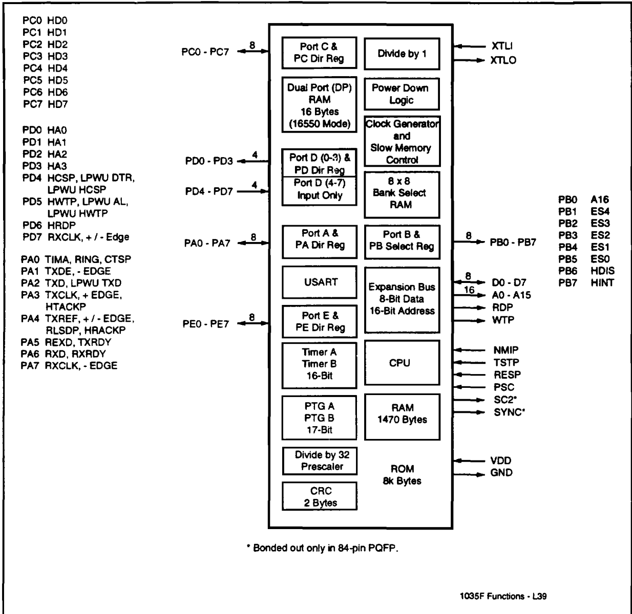
Figure 2-2b. Internal Functions and I/O Signals - L39
