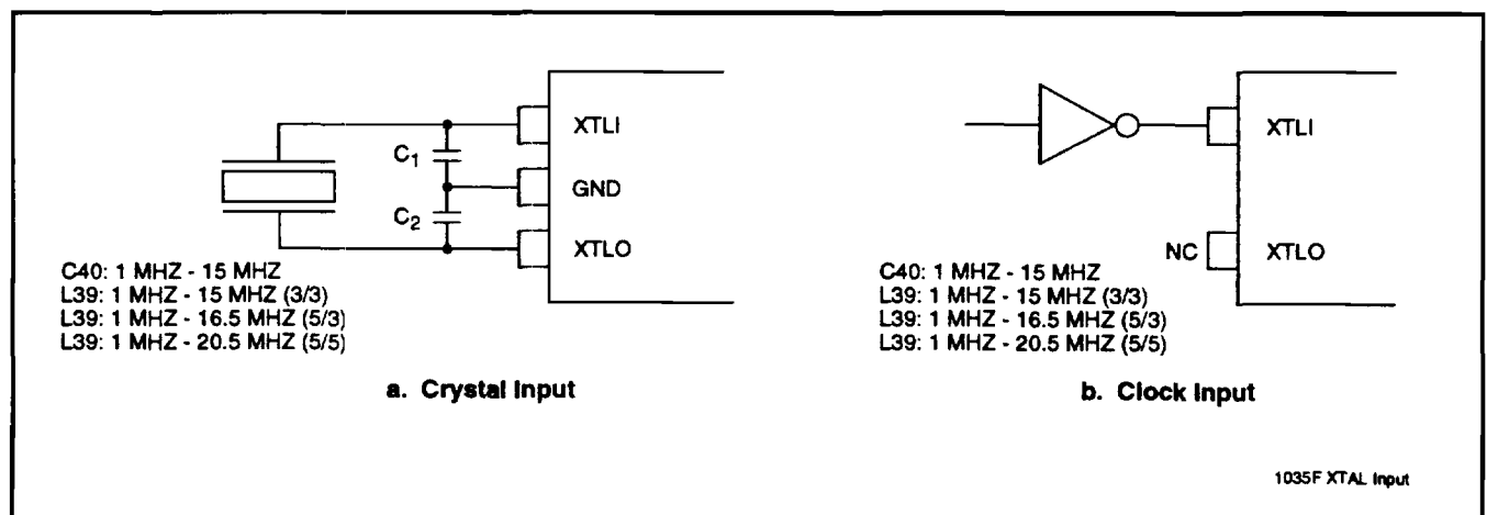
Figure 3-4. MCU Clock Oscillator Input Options
