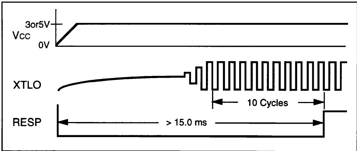
Figure 5-8. Power On RESP Timing
