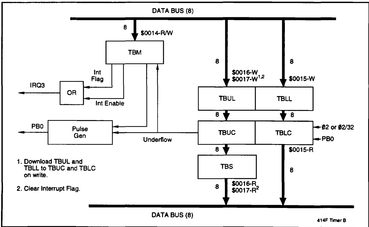
Figure 3-10. Counter/Timer B Block Diagram
