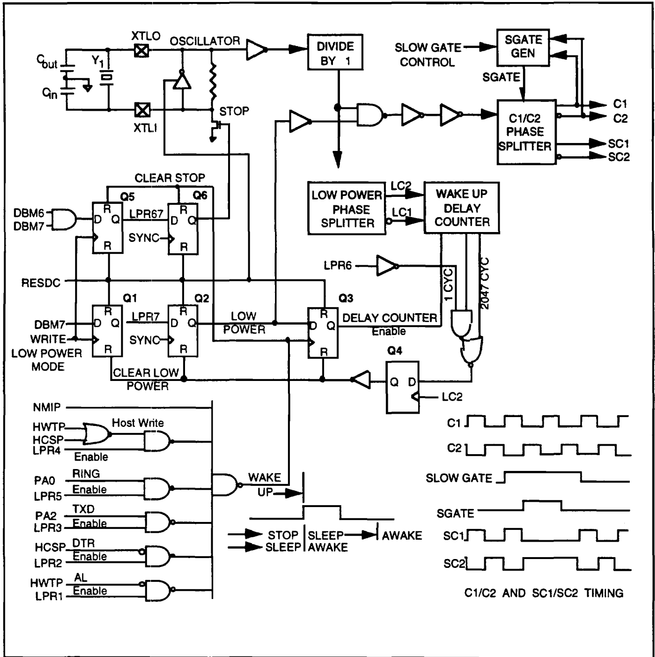
Figure 3-5. Low Power Mode Logic and Timing - L39
