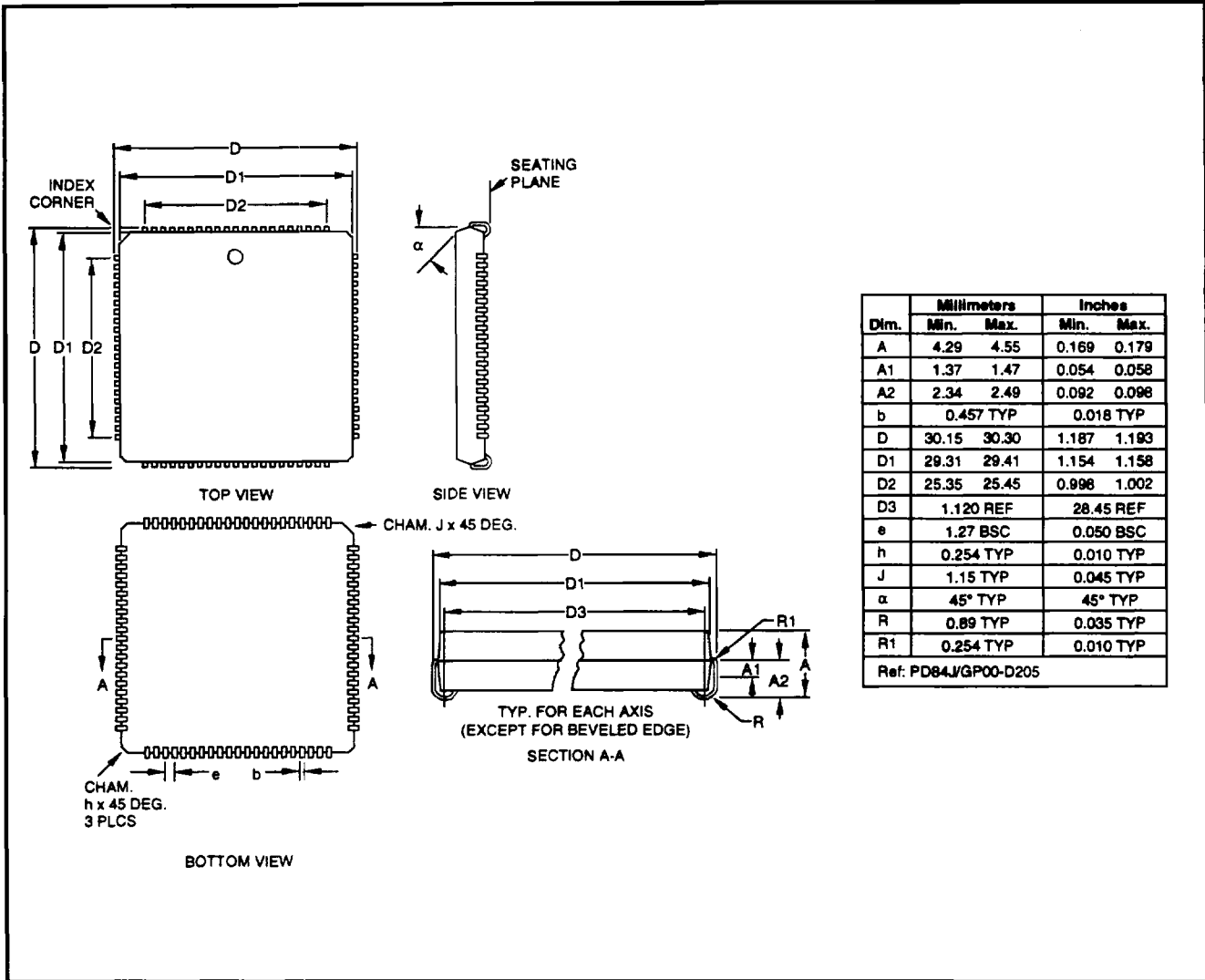
Figure 6-1a. Package Dimensions - 84-Pin PLCC
