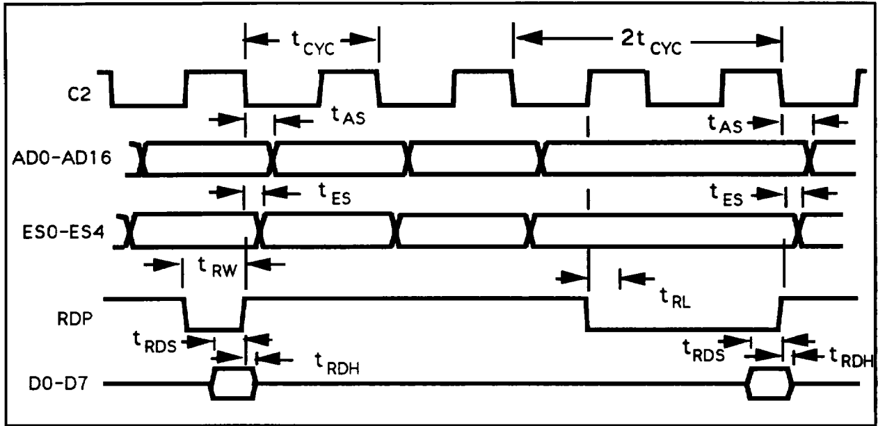
Figure 5-5. Expansion Bus Read Waveforms
