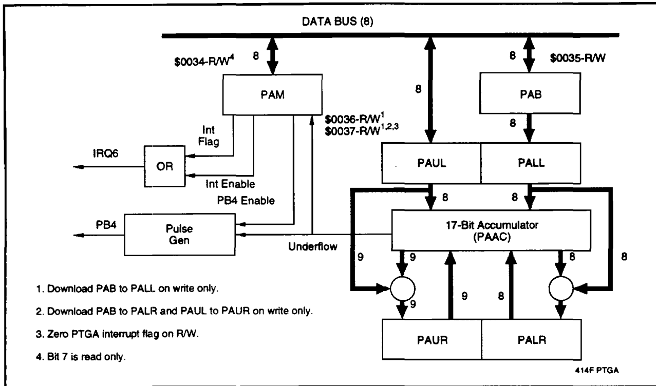
Figure 3-15. Precision Time Generator A Block Diagram
