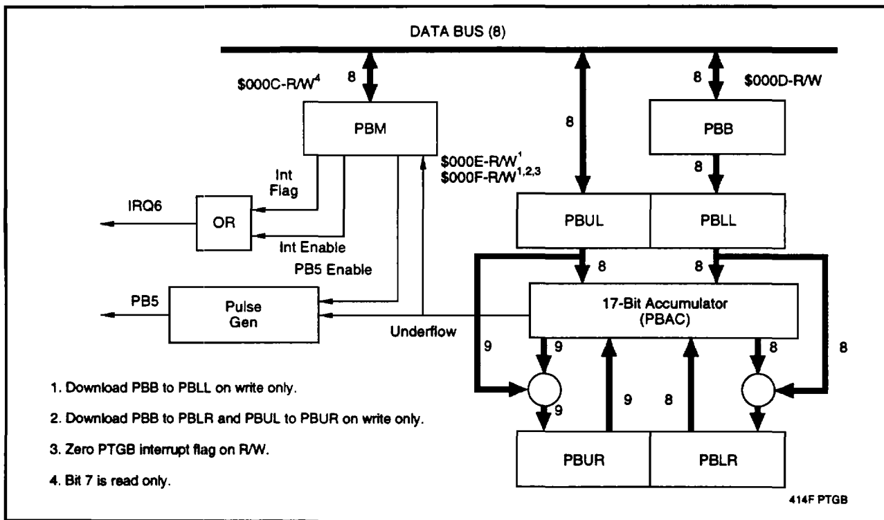
Figure 3-16. Precision Time Generator B Block Diagram
