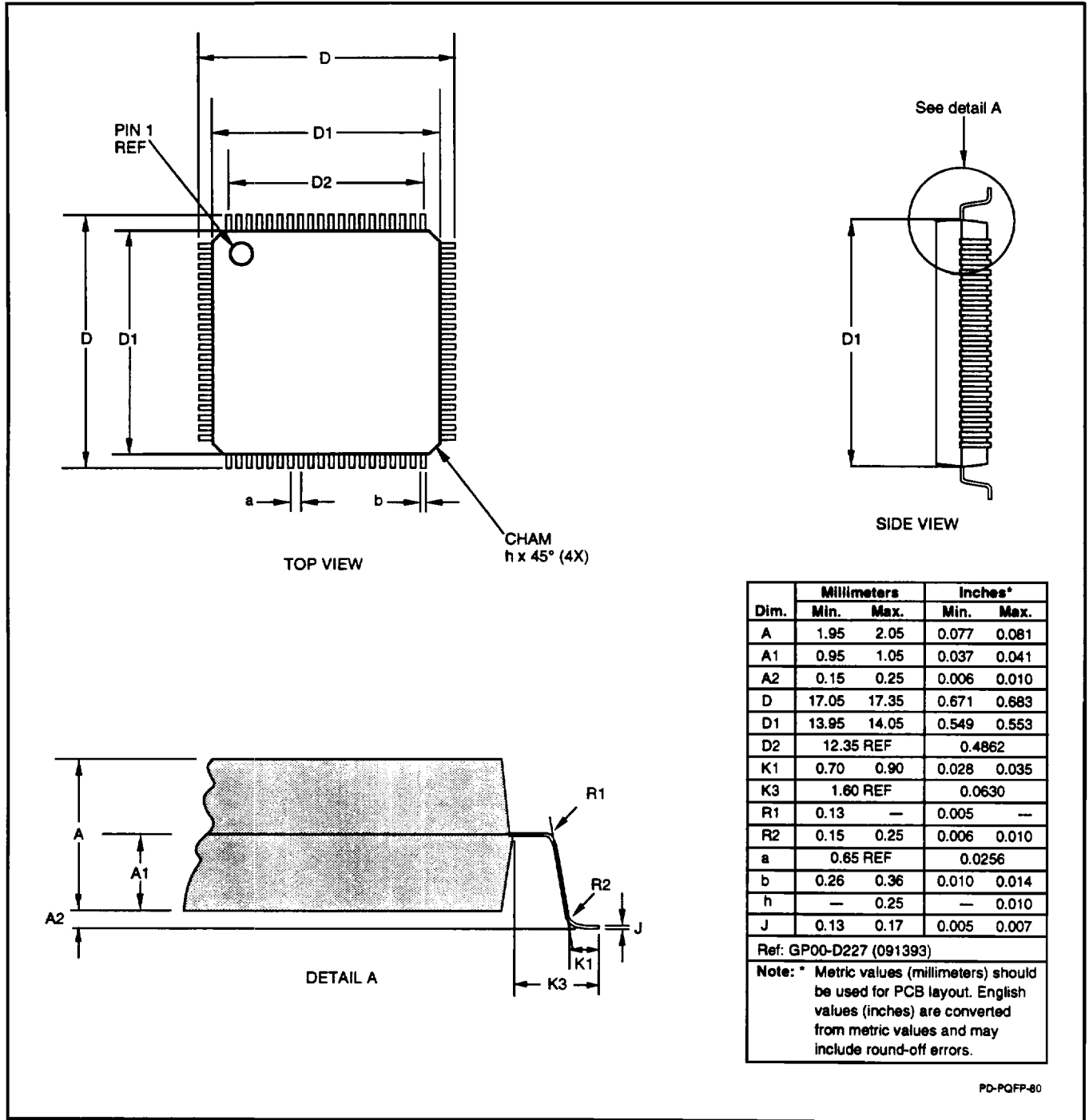
Figure 6-1b. Package Dimensions - 80-Pin PQFP
