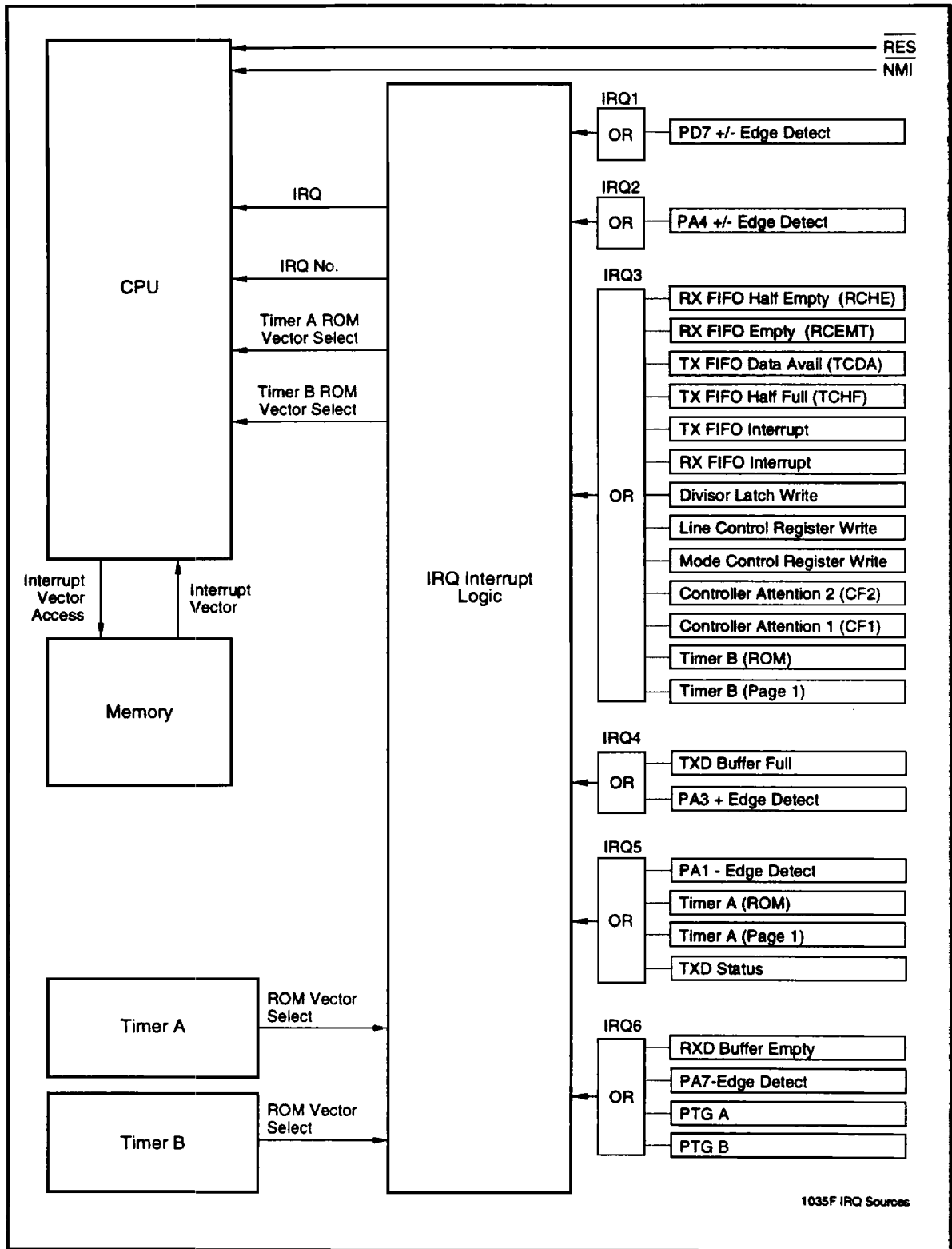
Figure 3-6. IRQ Interrupt Logic Interface
