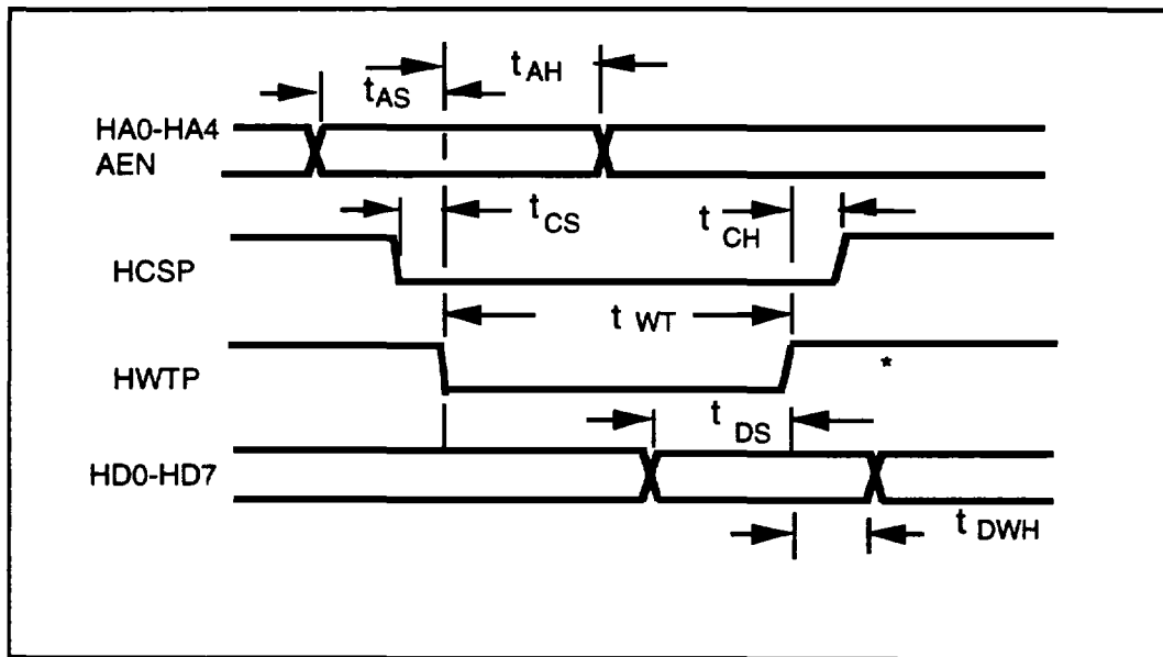
Figure 5-3. Host Bus Write Waveforms
