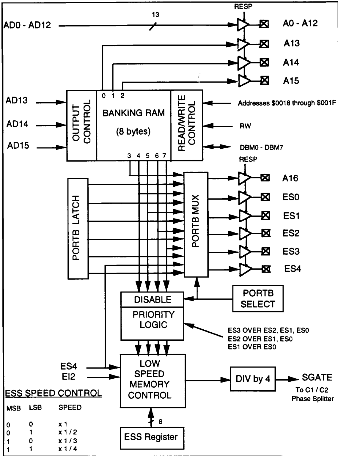
Figure 3-8. Banking Logic
