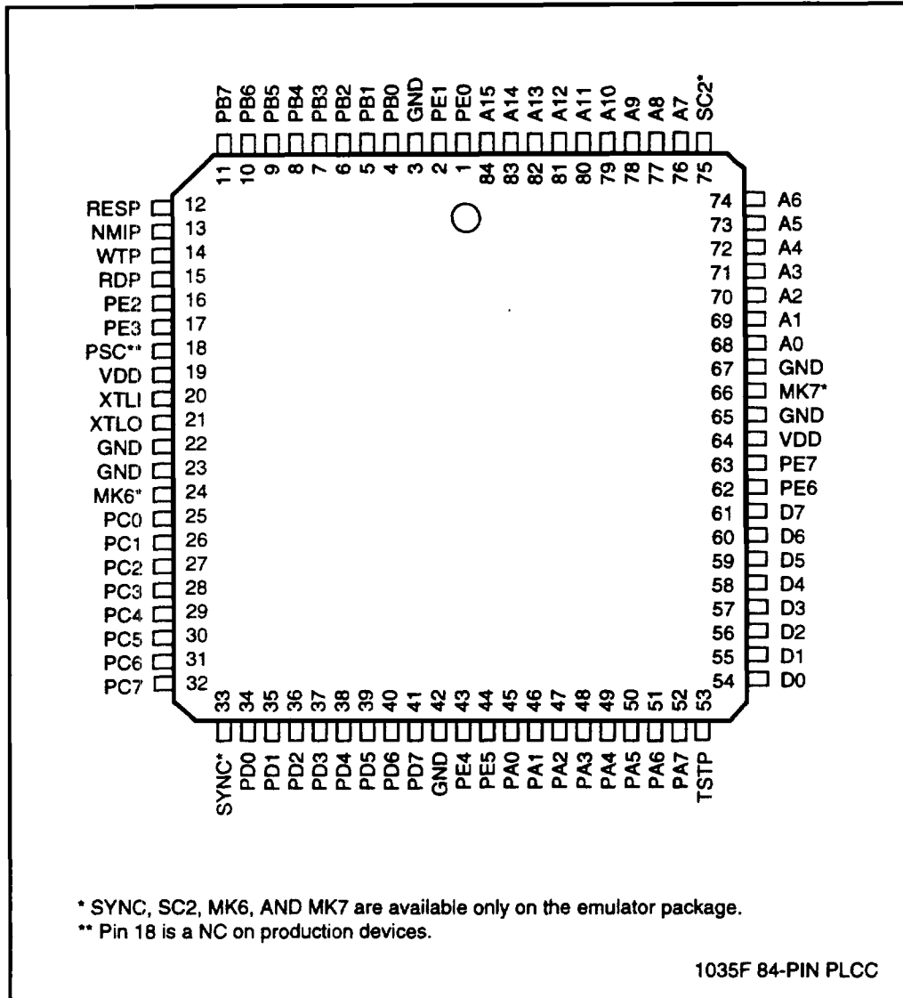
Figure 2-1a. Pin Assignments - 84-Pin PLCC
