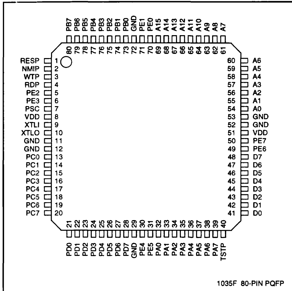
Figure 2-1b. Pin Assignments - 80-Pin PQFP
