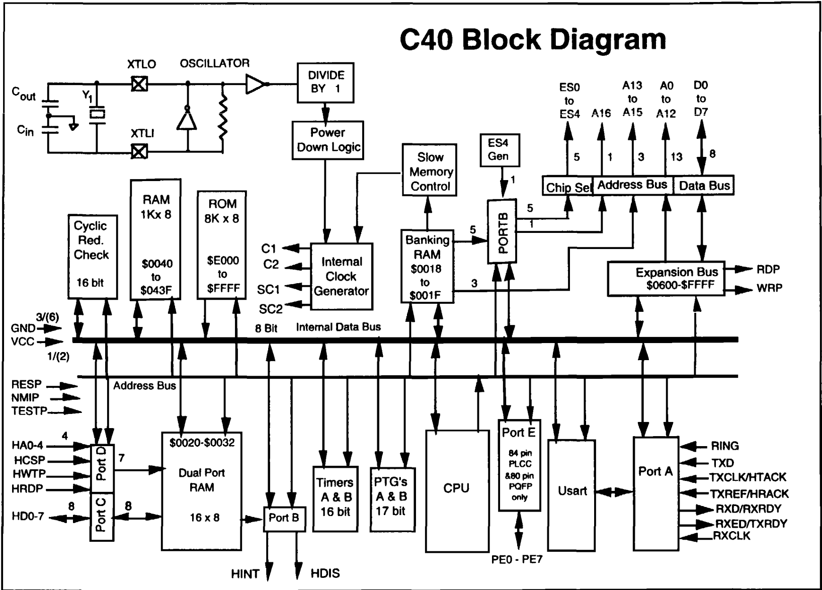
Figure 3-1a. MCU Block Diagram - C40
