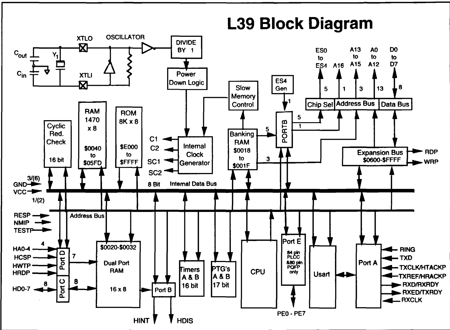
Figure 3-1b. MCU Block Diagram - L39
