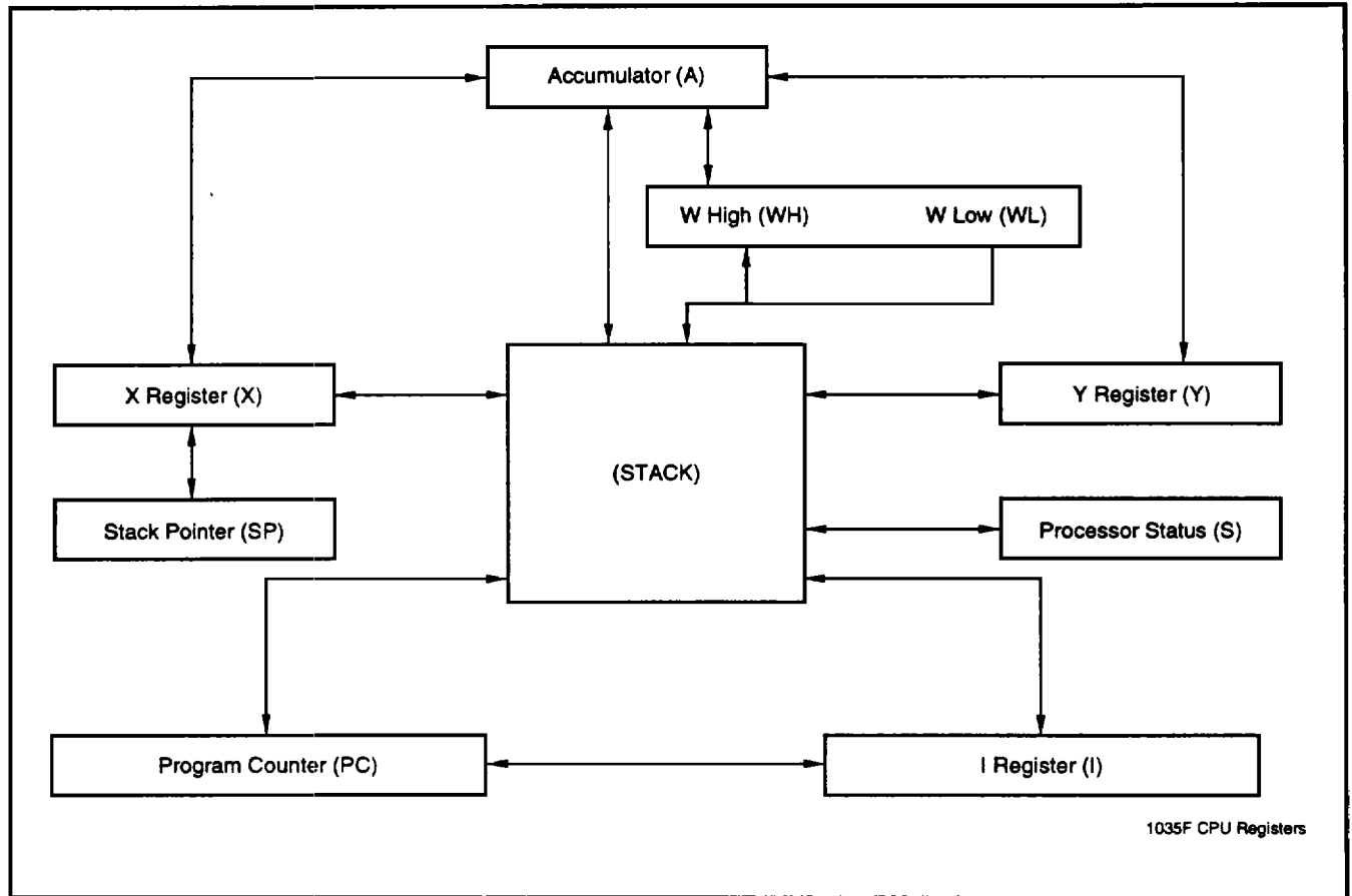
Figure 3-3. CPU Registers and Data Flow
