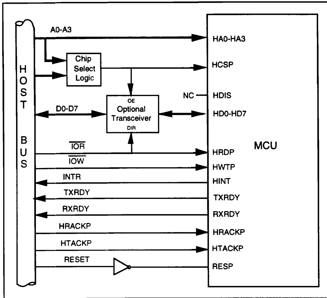
Figure 3-18. MCU/Host Interface
