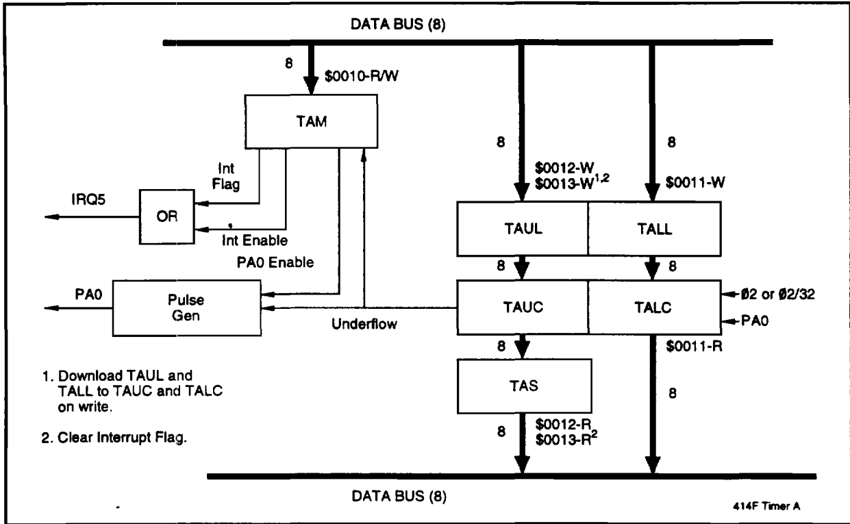
Figure 3-9. Counter/Timer A Block Diagram
