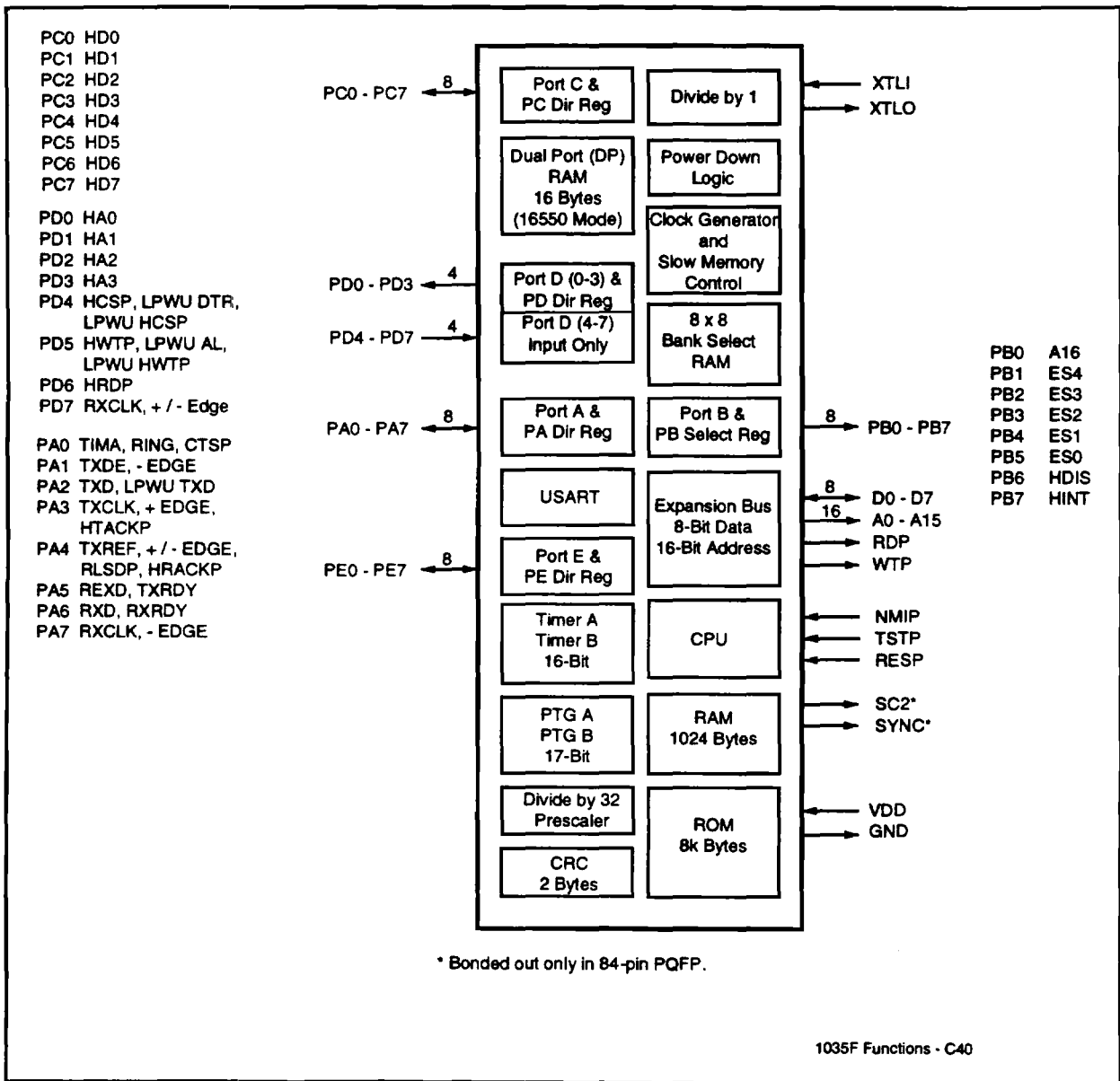
Figure 2-2a. Internal Functions and I/O Signals - C40
