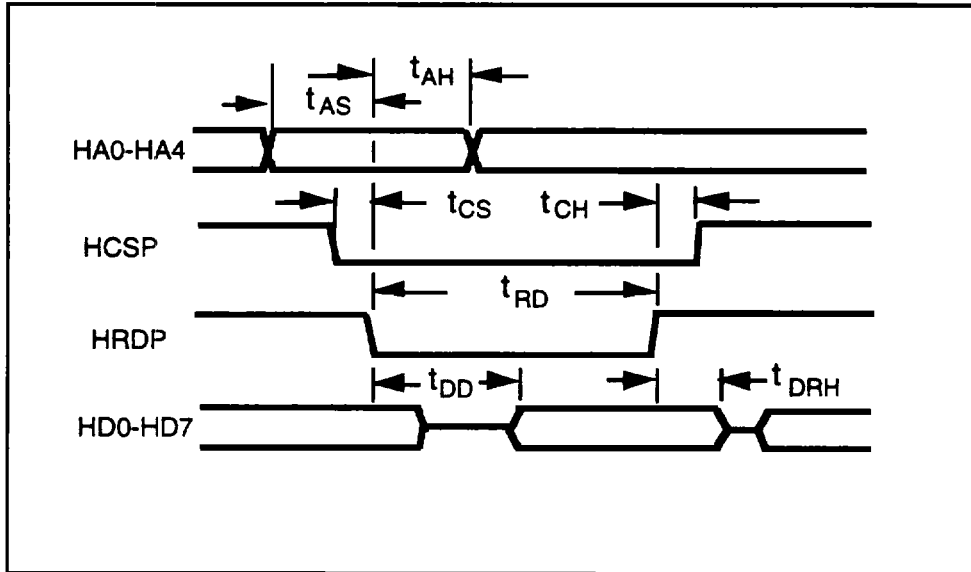
Figure 5-2. Host Bus Read Waveforms
