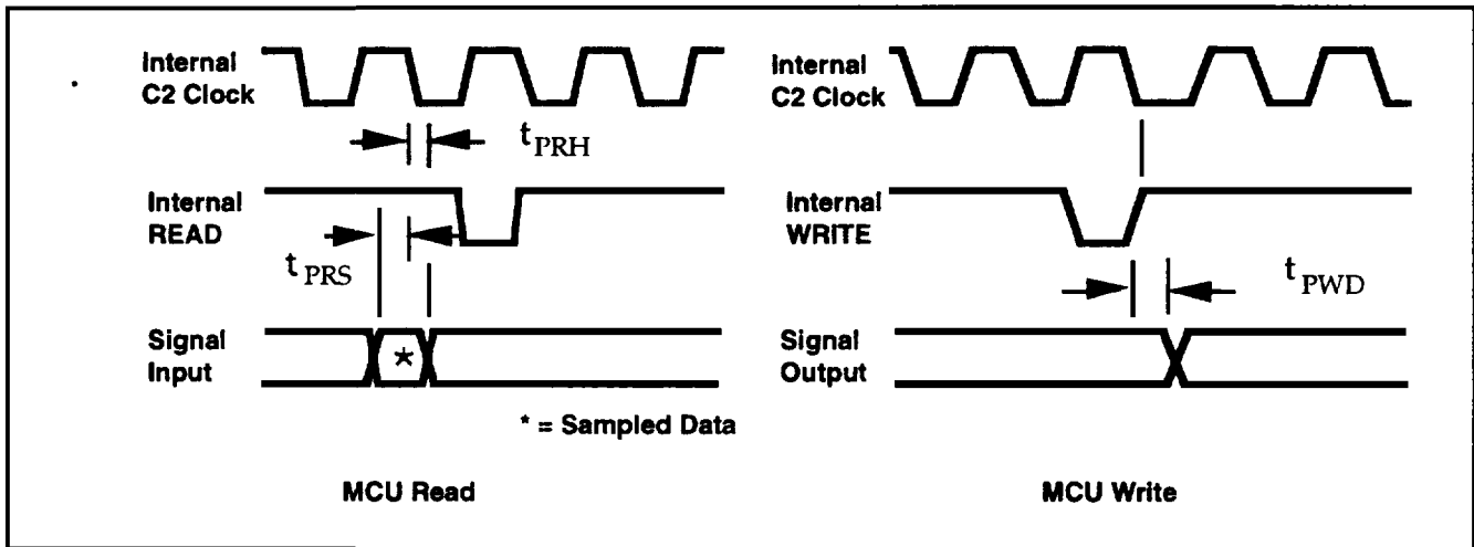
Figure 5-1. Port A, B, C, D, and E Read/Write Waveforms
