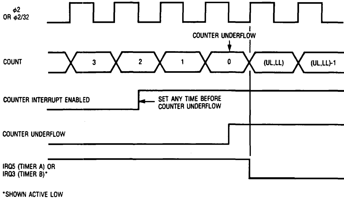
Figure 3-11. Interval Timer (Mode 0) Waveforms
