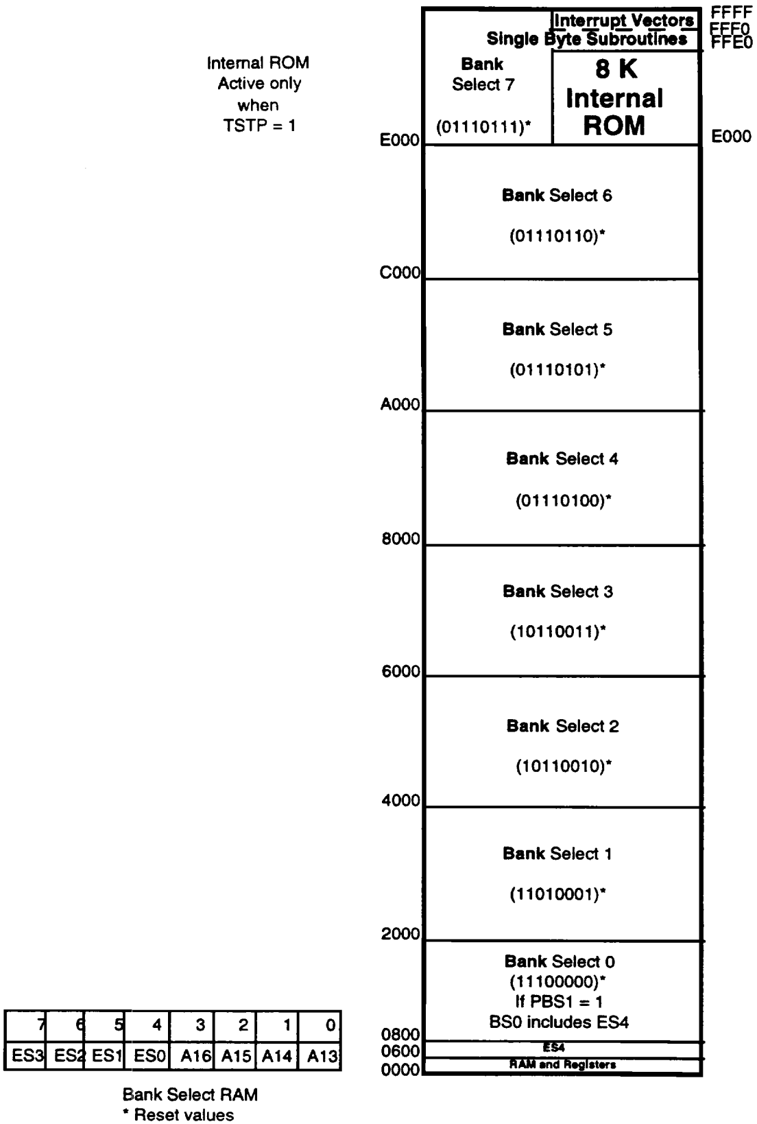
Figure 3-7. Memory Map - RAM Banking
