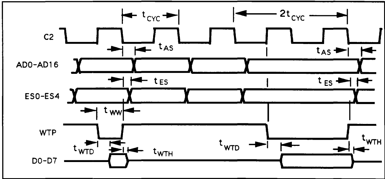
Figure 5-6. Expansion Bus Write Waveforms
