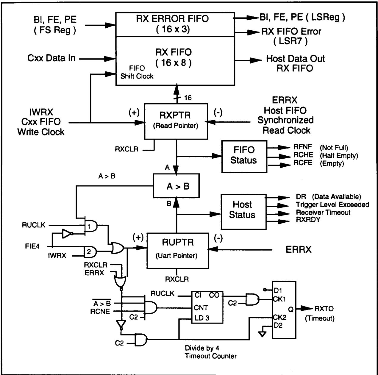
RX FIFO Block Diagram
