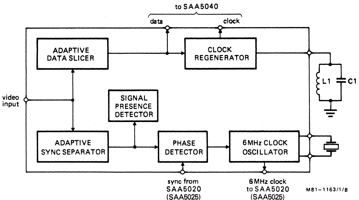
Fig.1 Block diagram
