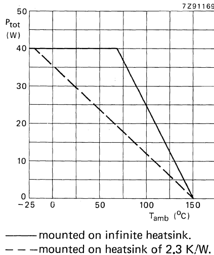
Fig. 2 Power derating curves.
