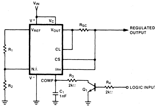
REMOTE SHUTDOWN REGULATOR WITH CURRENT LIMITING ( V_{OUT} = 2 TO 7 VOLTS)
