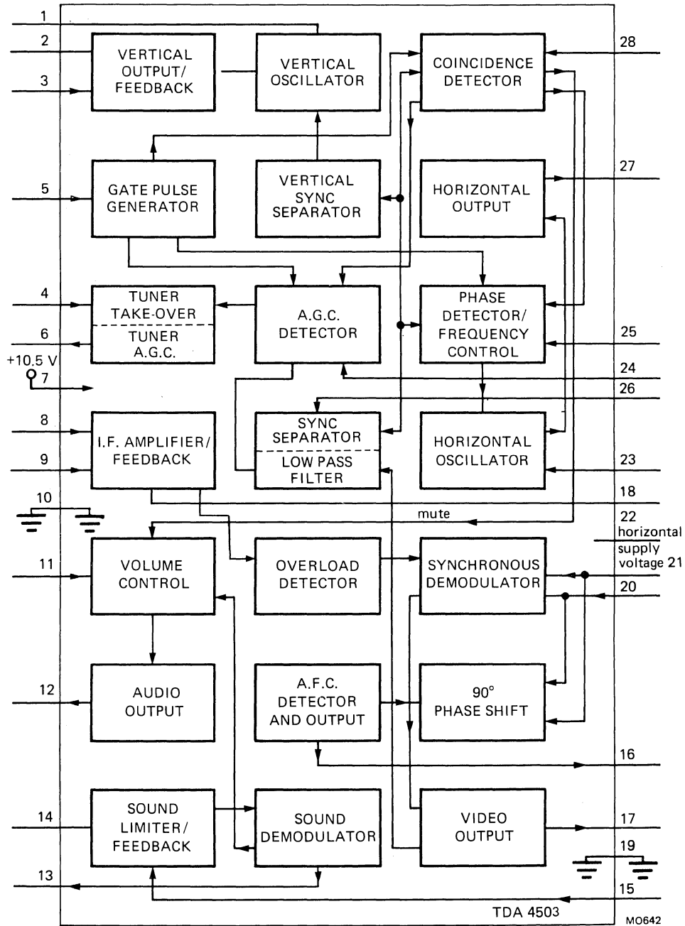
Fig. 1 Block diagram.
