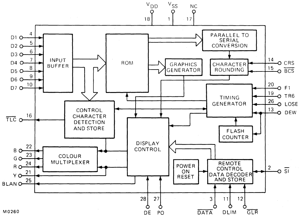
Fig.1 Block diagram
