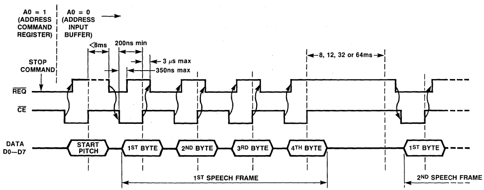
Figure 7. Speech Code Data Write Timing Sequence
