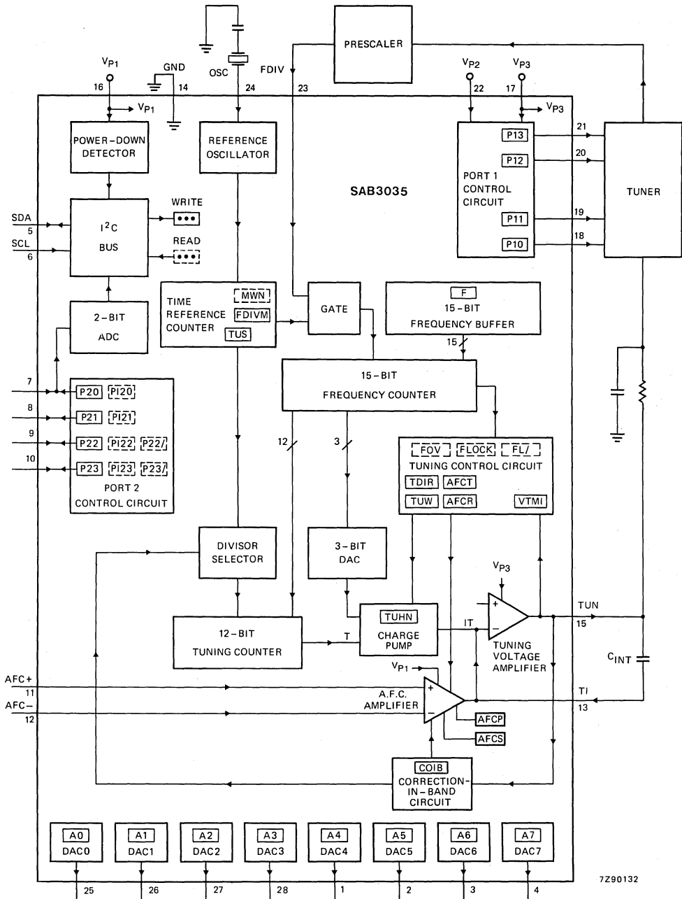
Fig. 1 Block diagram.
