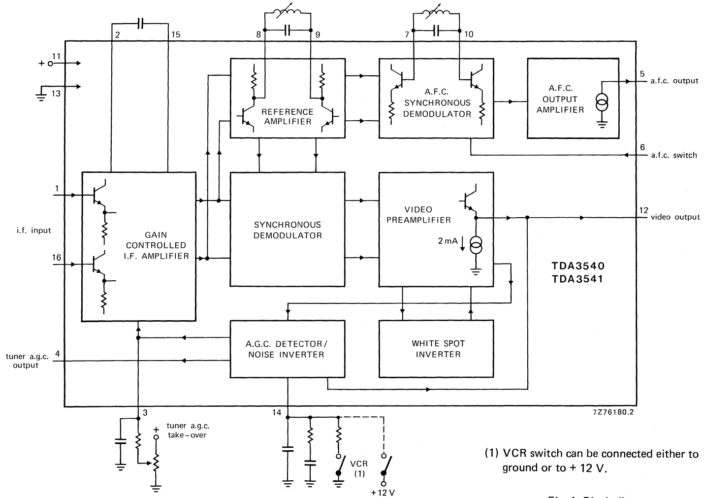
Fig. 1 Block diagram.
