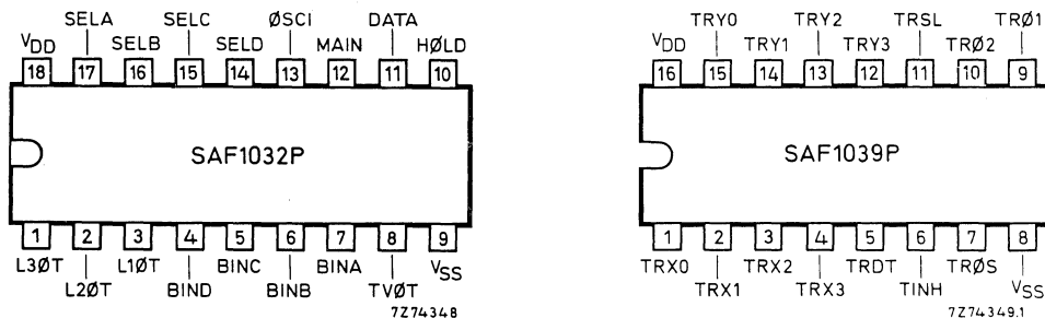
Fig. 1 Pin designations.
