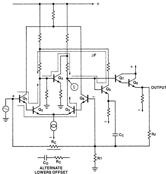
Figure 12B. Pin 12 Compensation Showing Internal Connections — Non-Inverting
