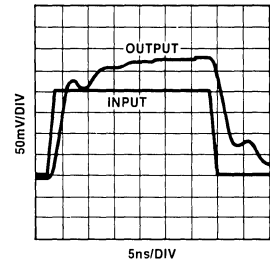
Figure 13F. Closed-Loop Non-Inverting Pulse Response — R_C = 200\Omega , C_C = 3pF , A_V = 3 (Computer Simulation — Overdamped)
