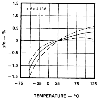
CENTER FREQUENCY TEMPERATURE COEFFICIENT (MEAN AND S.D.)
