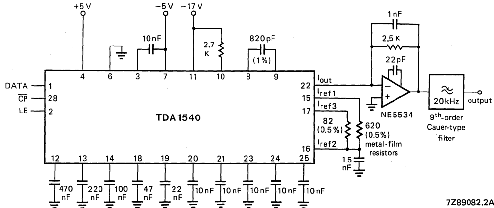
Fig. 4 Application circuit.
