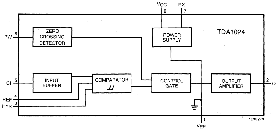
Fig. 1 Block diagram.
