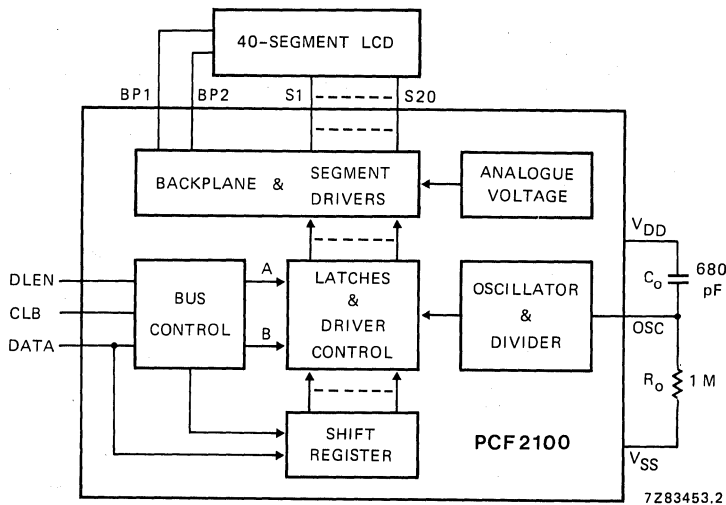
Fig. 1 Block diagram.
