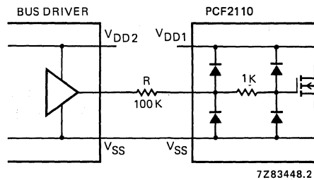
Fig. 10 Input circuitry.
