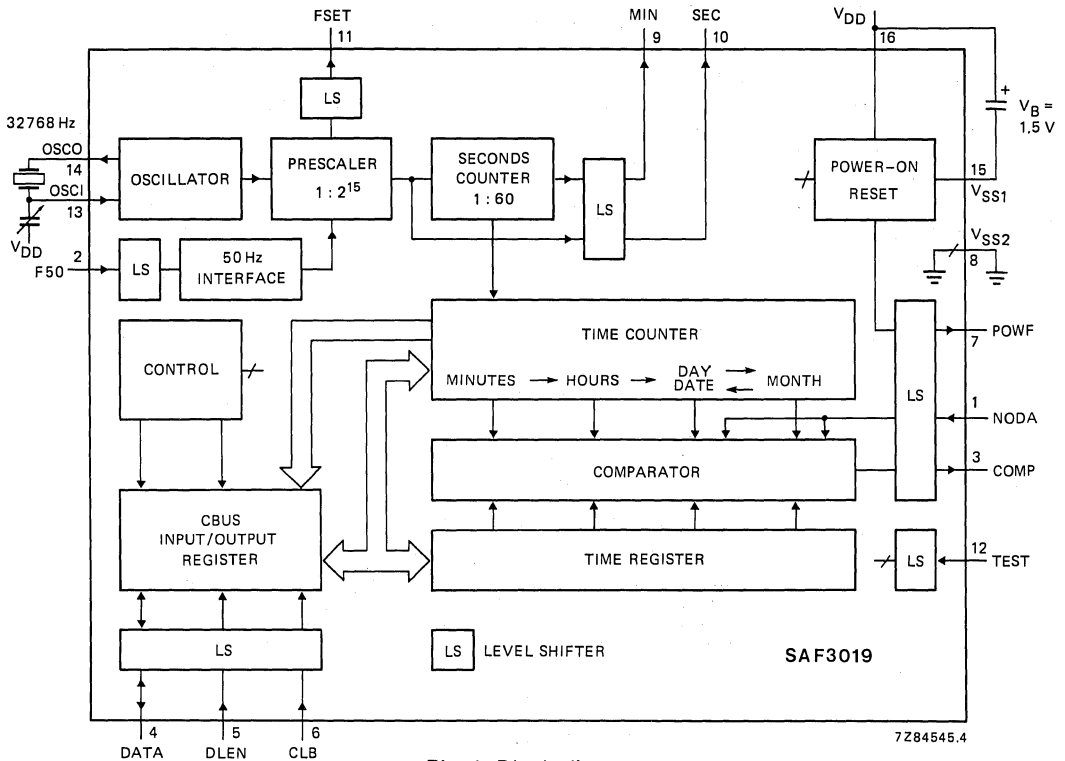
Fig. 1 Block diagram.
