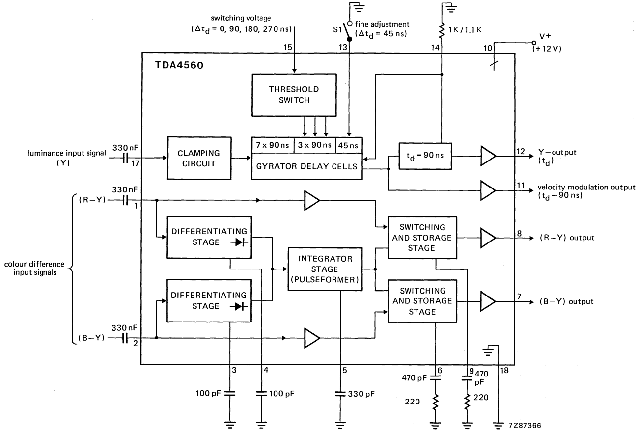
Fig. 1 Block diagram.
