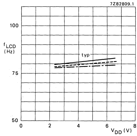
Fig. 5 Display frequency as a function of supply voltage; R_O C_O = 680 \mu\text{s} .
