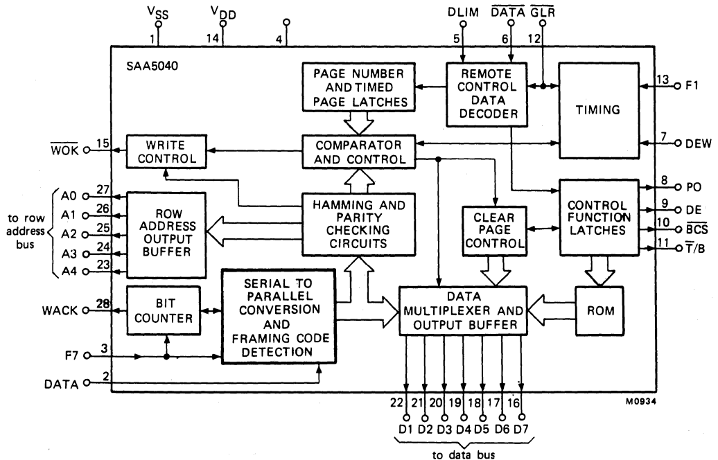
Fig.1 Block diagram.
