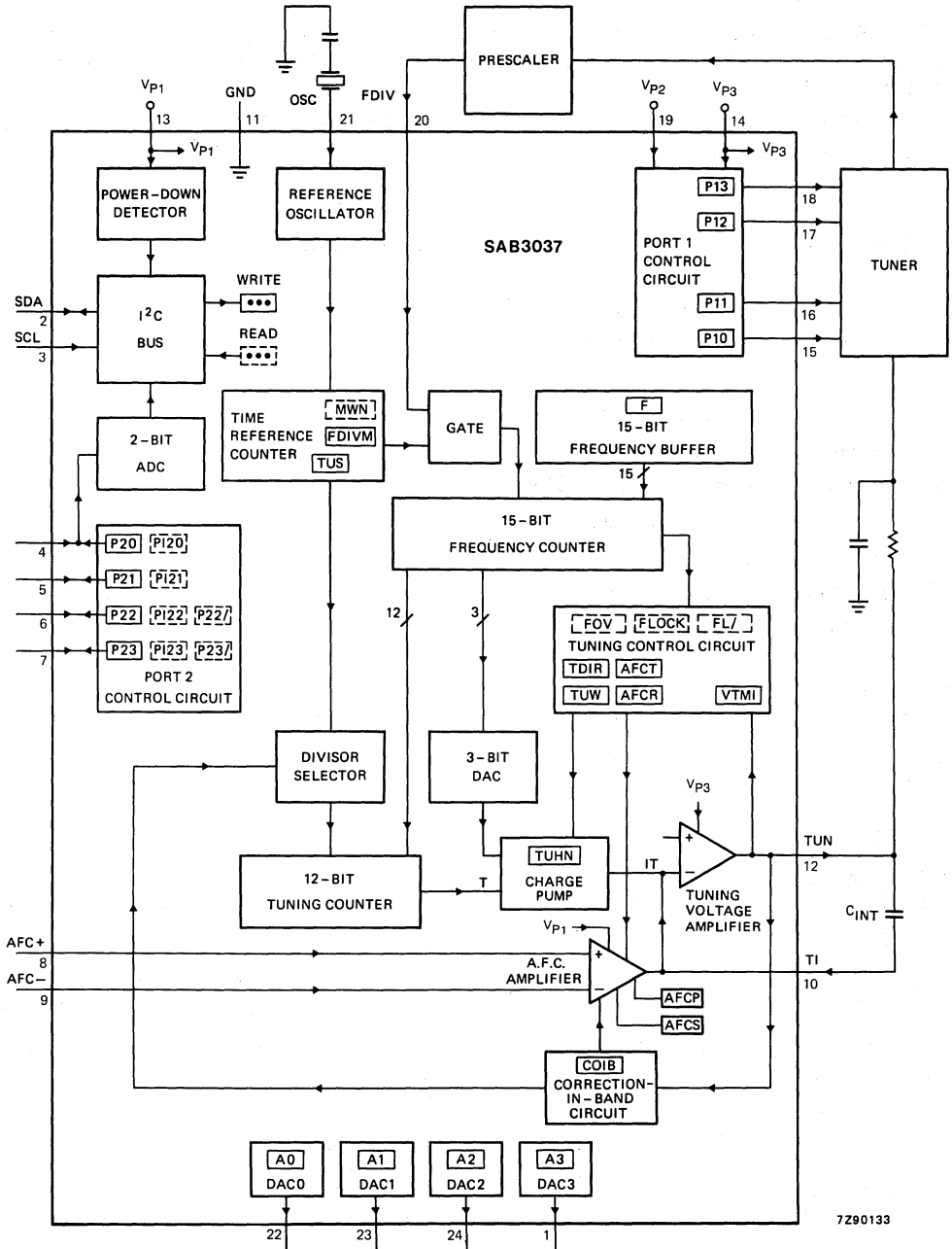
Fig. 1 Block diagram.
