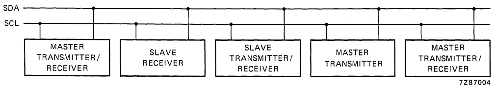
Fig. 5 System configuration.
