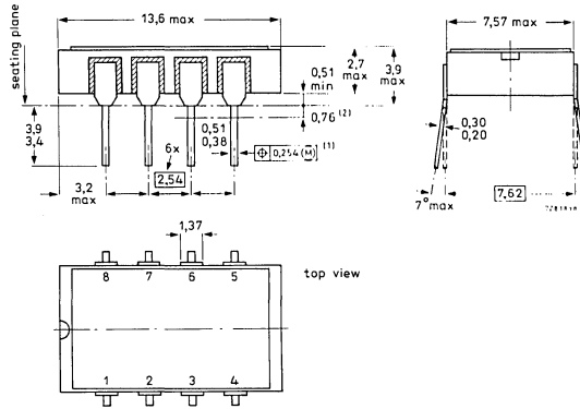
8-LEAD DUAL IN-LINE; METAL CERAMIC (CERDIL) (SOT-153B)
