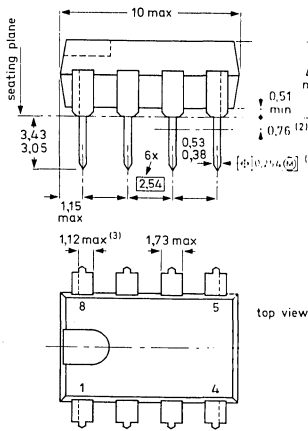
8-LEAD DUAL IN-LINE; PLASTIC (SOT-97A)
