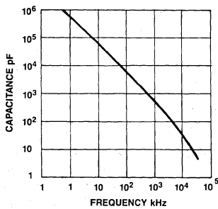
(a) VCO TIMING CAPACITOR VERSUS FREQUENCY
