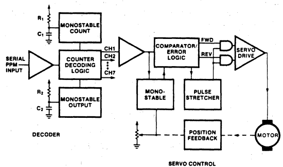
FIGURE 4. Block Diagram of the Serial to Parallel Decoder and of the Servocontrol
