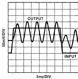
Figure 11B. Closed-Loop Non-Inverting Response — No Compensation (Computer Simulation — Oscillation is Evident)
