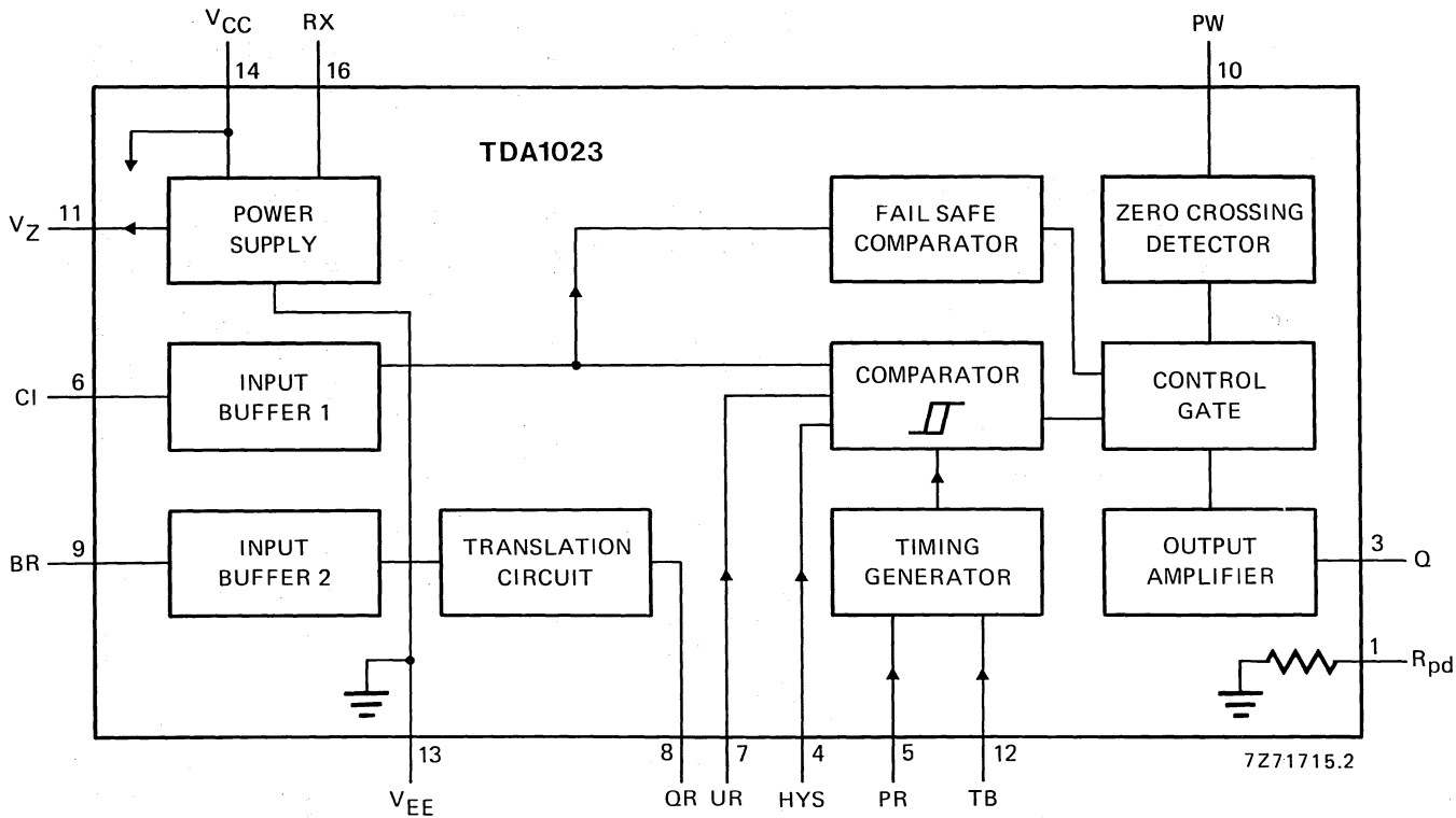
Fig. 1 Block diagram.
