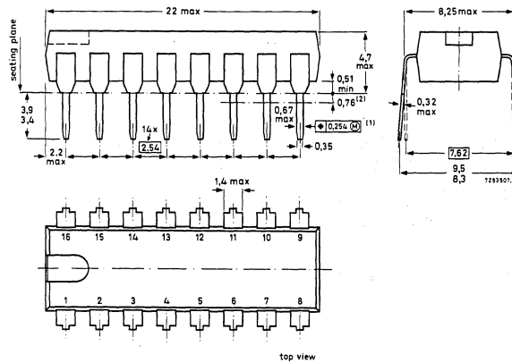
16-LEAD DUAL IN-LINE; PLASTIC (SOT-38A)
