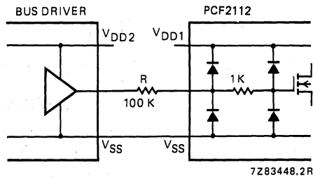
Fig. 8 Input circuitry.
