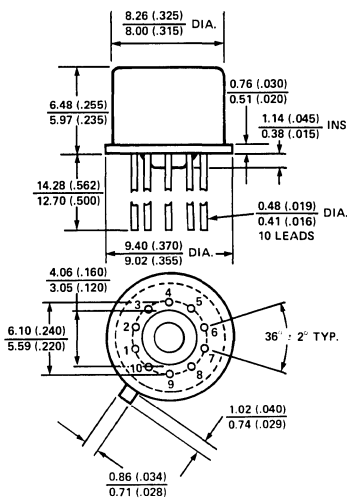
H PACKAGE HERMETIC 10-PIN (TO-5/100 HEADER TALL CAN)
