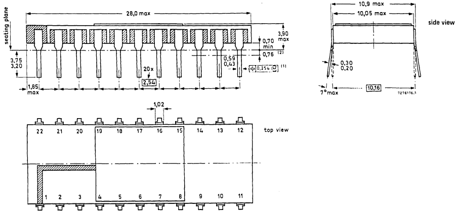
22-LEAD DUAL IN-LINE; METAL CERAMIC (CERDIL) (SOT-118B)
