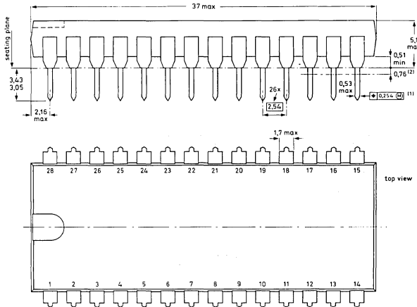
28-LEAD DUAL IN-LINE; PLASTIC (SOT-117D)
