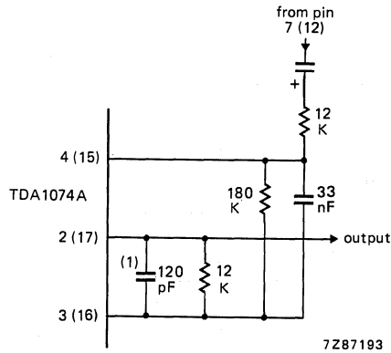
Fig. 13 Circuit diagram for frequency response limiting.
