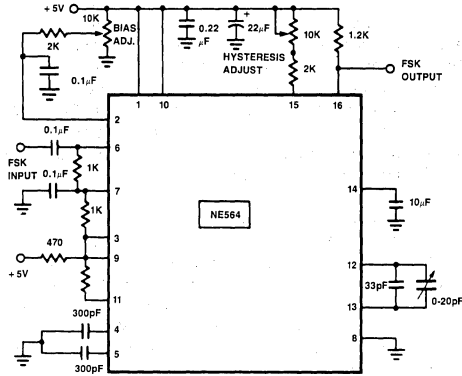
10.8 MHz FSK DECODER USING THE 564
