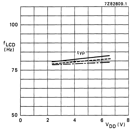
Fig. 5 Display frequency as a function of supply voltage; R_O C_O = 680\ \mu\text{s} . — T_{amb} = -40\text{ }^{\circ}\text{C} ; - - - T_{amb} = +25\text{ }^{\circ}\text{C} ; - · - · T_{amb} = +85\text{ }^{\circ}\text{C} .
