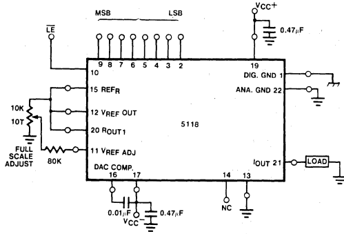
BIPOLAR OUTPUT OPERATION (-1mA TO +1mA)
