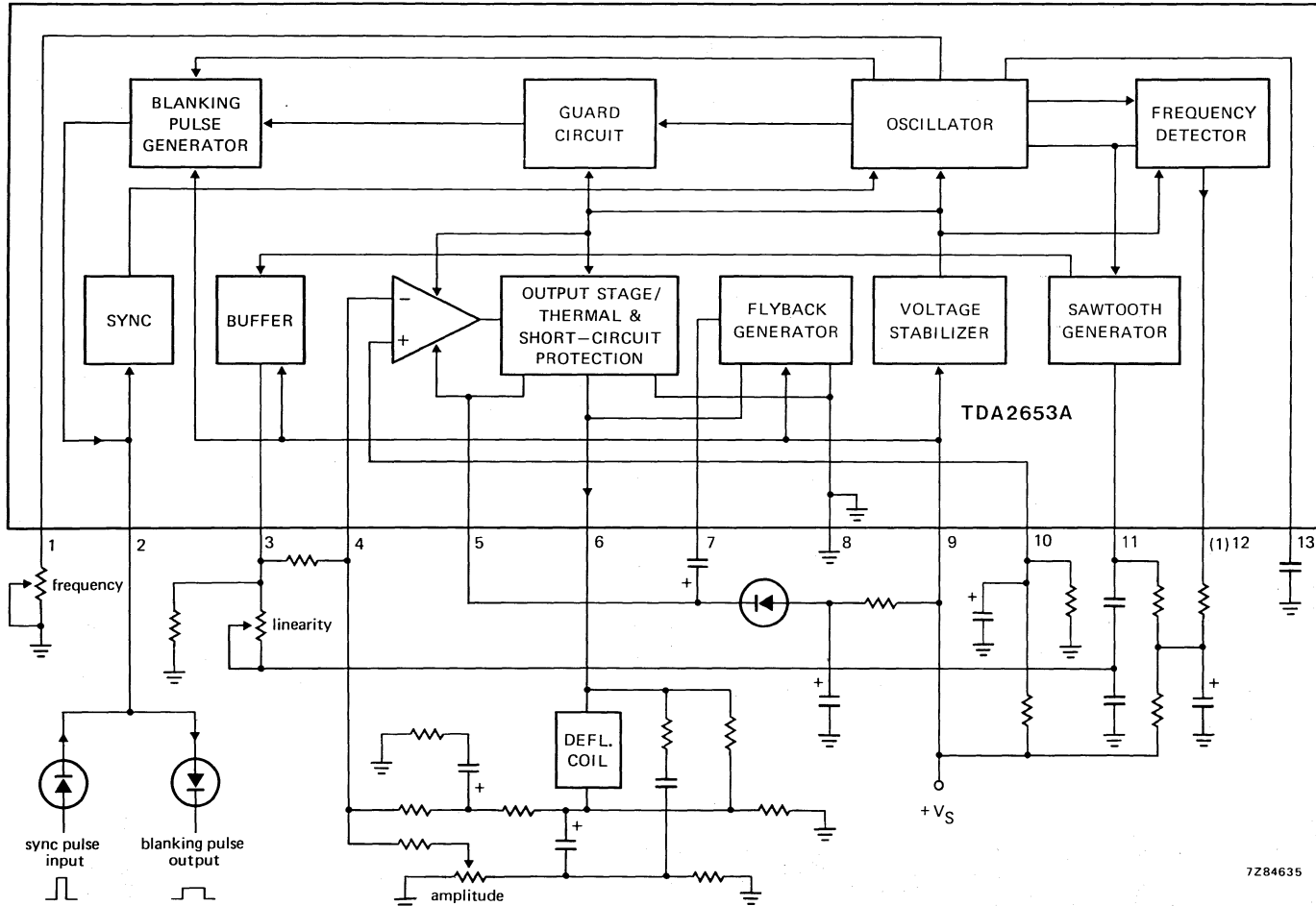
Fig. 1 Block diagram.
