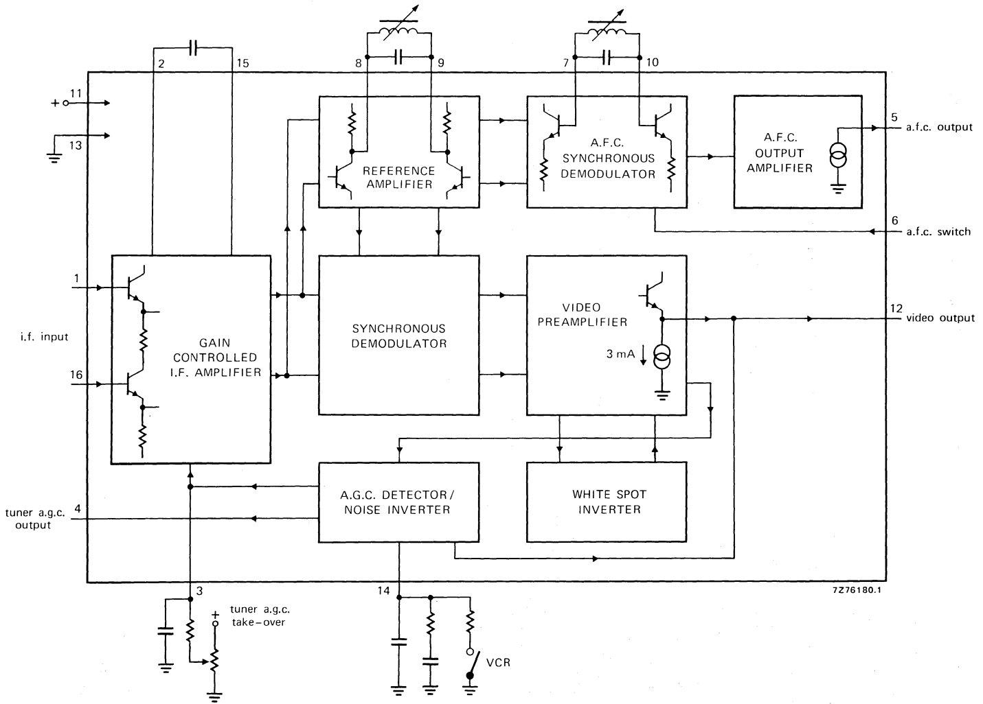
Fig. 1 Block diagram.
