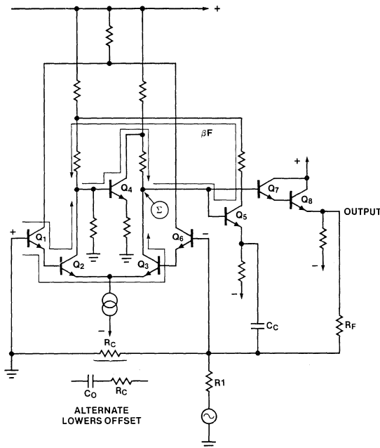
Figure 12A. Pin 12 Compensation Showing Internal Connections — Inverting
