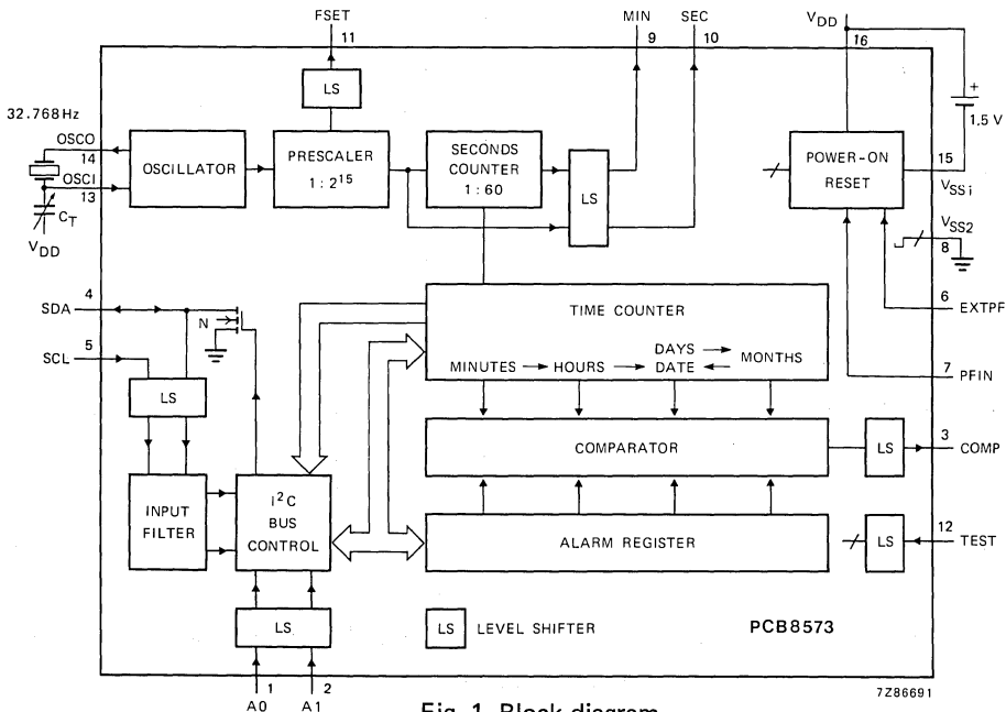
Fig. 1 Block diagram.
