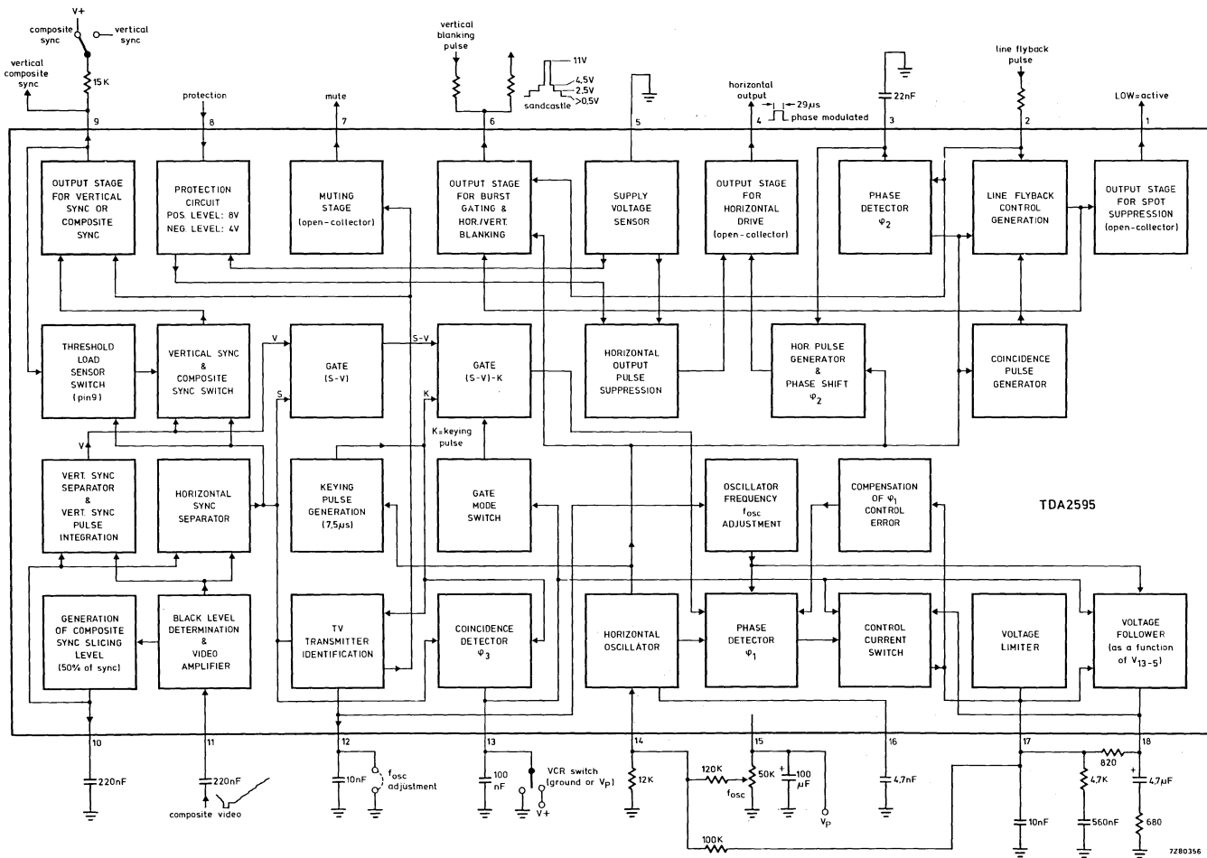
Fig. 1 Block diagram.
