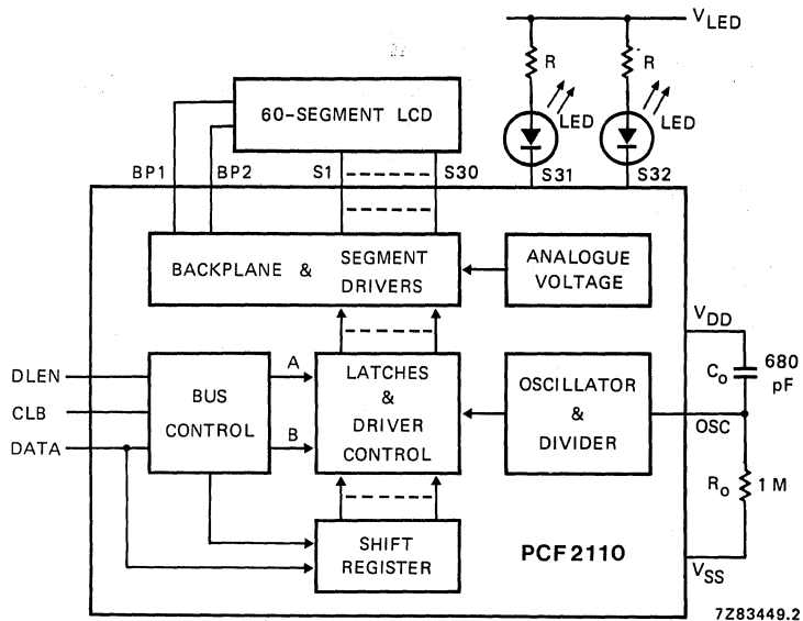
Fig. 1 Block diagram.
