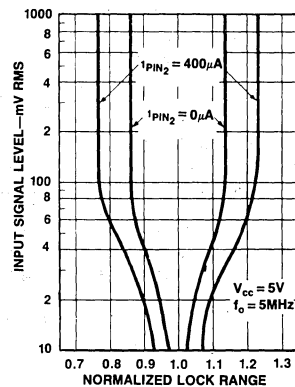
(b) LOCK RANGE VERSUS INPUT SIGNAL LEVEL AND BIAS CURRENT
