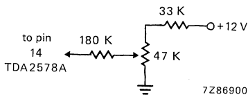
Fig. 6 Circuit configuration at pin 14 for phase adjustment.
