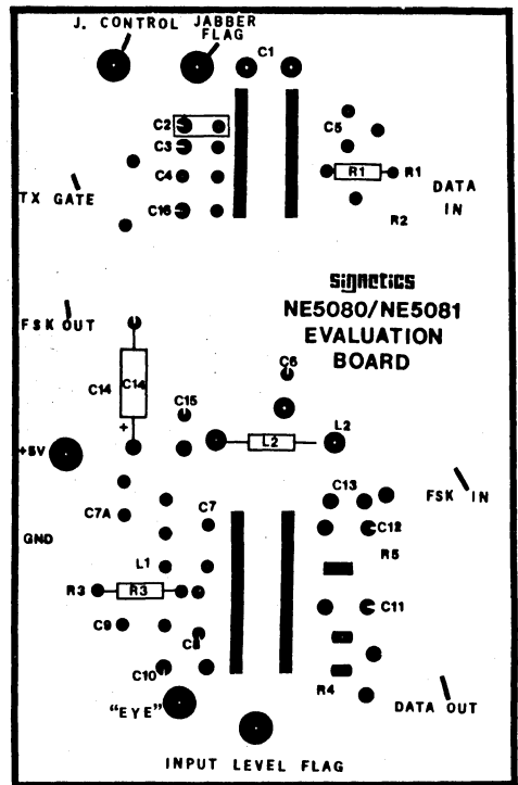
Figure 12. Components and Layout Used for Evaluation Board
