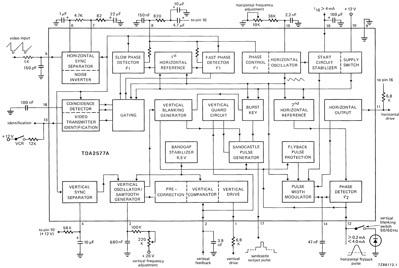
Fig. 1 Block diagram.
