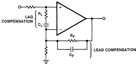
Figure 1. Non-Inverting Configuration
