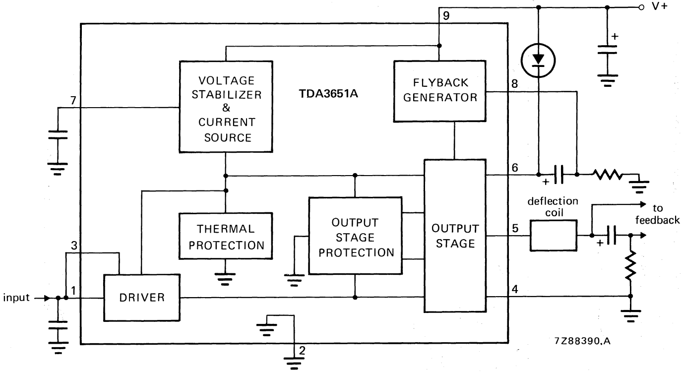
Fig. 1 Block diagram.
