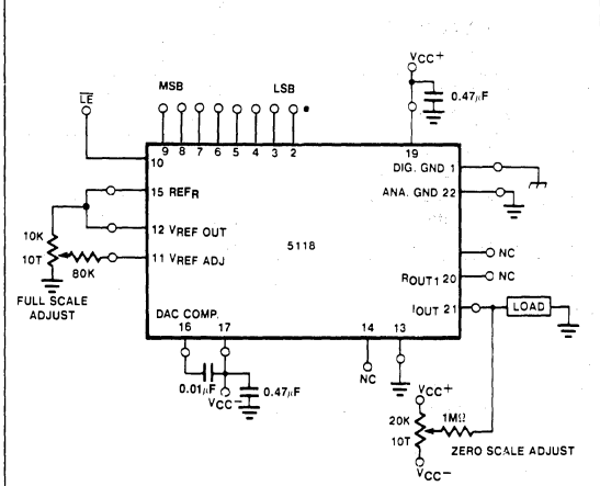
BASIC UNIPOLAR CURRENT OUTPUT (0 → -2mA)
