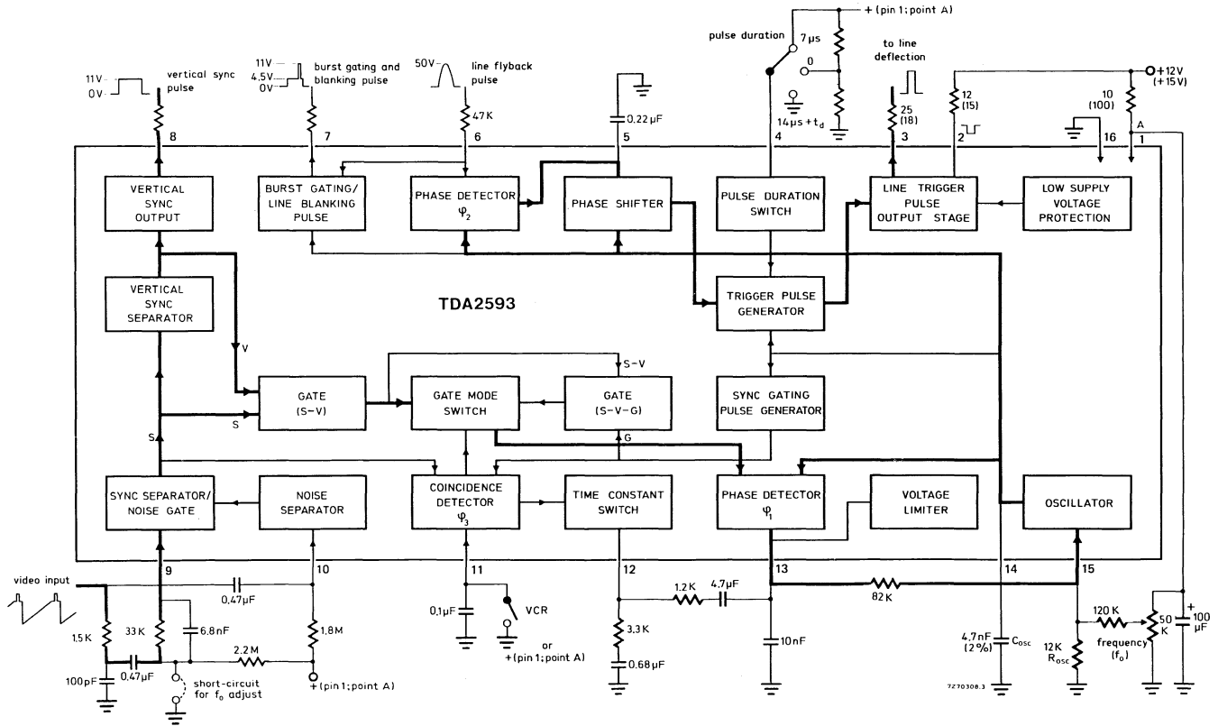
Fig. 1 Block diagram.
