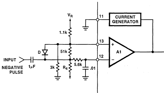
Figure 3. NE5045 Decoder With Neg. Pulse Input
