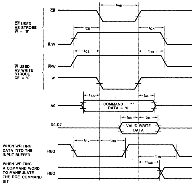
Figure 6. Write Timing
