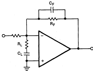
Figure 2. Inverting Configuration
