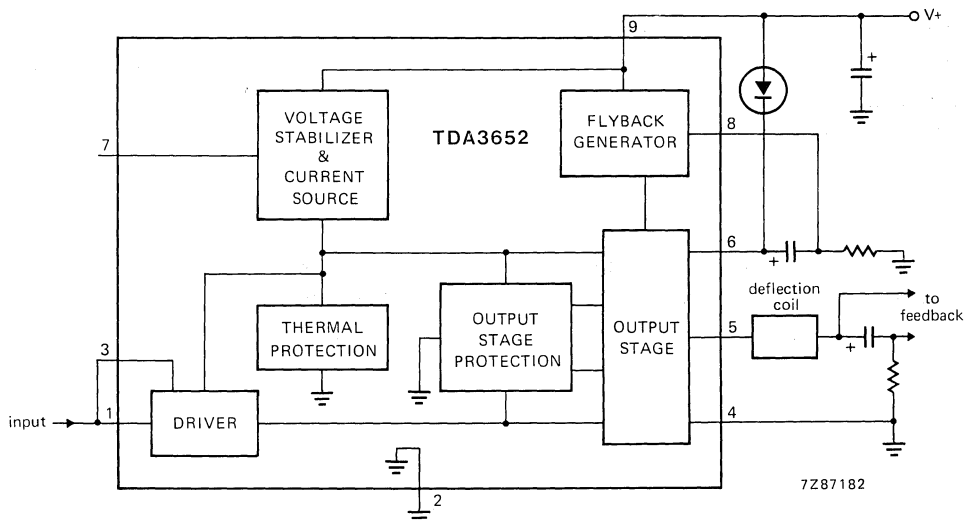
Fig. 1 Block diagram.
