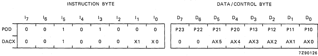
Fig. 5 Control programming.
