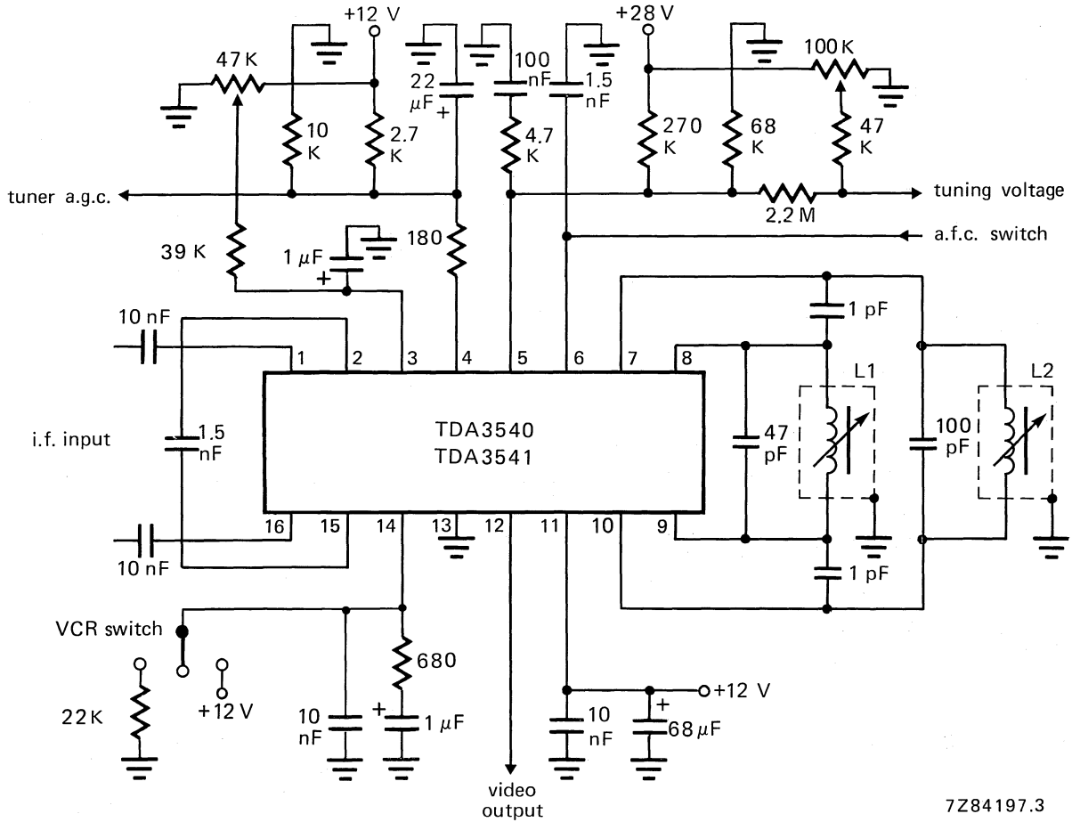
Fig. 8 Typical application circuit diagram; Q of L1 and L2 = 80; f_o = 38.9 MHz.
