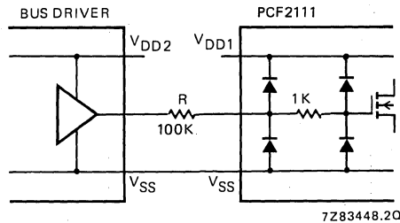
Fig. 9 Input circuitry.
