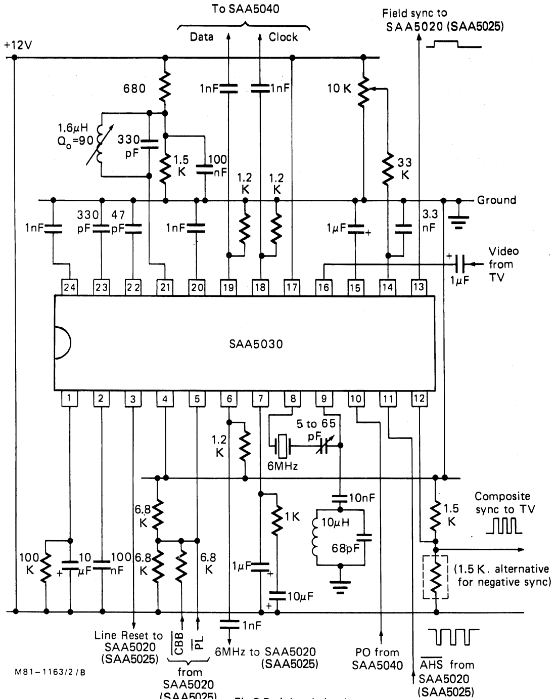
Fig.3 Peripheral circuit
