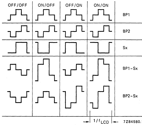
Fig. 8 Timing diagram.
