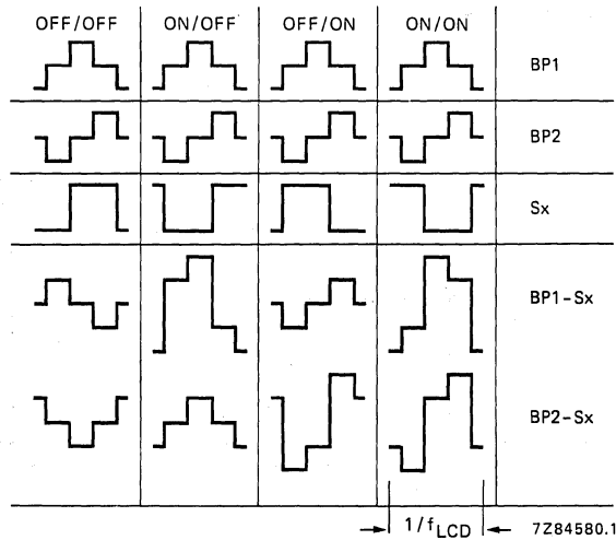
Fig. 9 Timing diagram.
