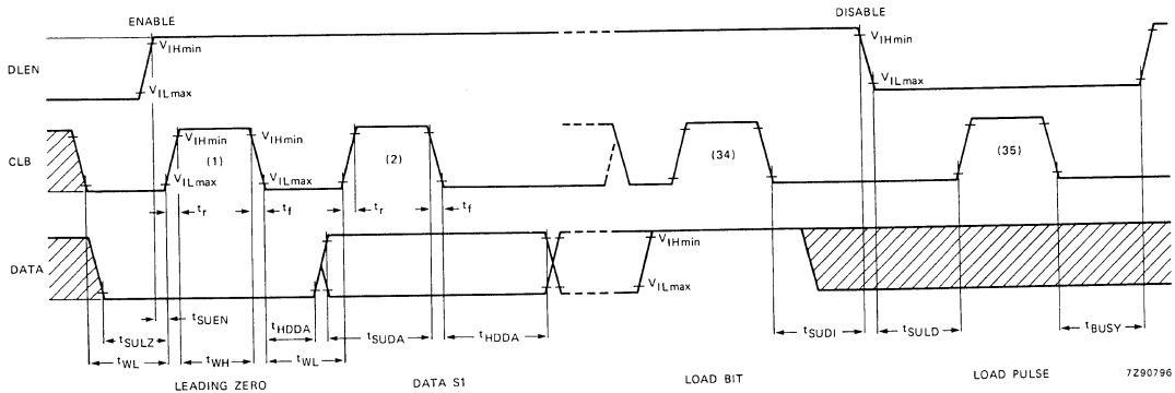
Fig. 2 CBUS timing.
