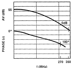
Figure 11A. Open-Loop Gain — No Compensation (Computer Simulation)
