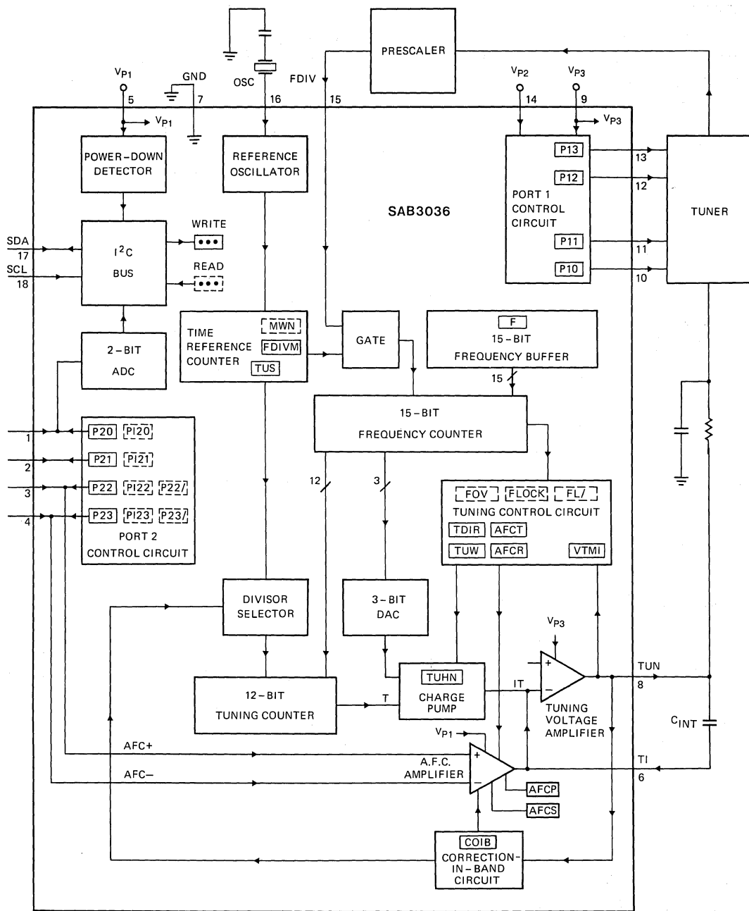
Fig. 1 Block diagram.
