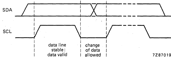
Fig. 3 Bit transfer.
