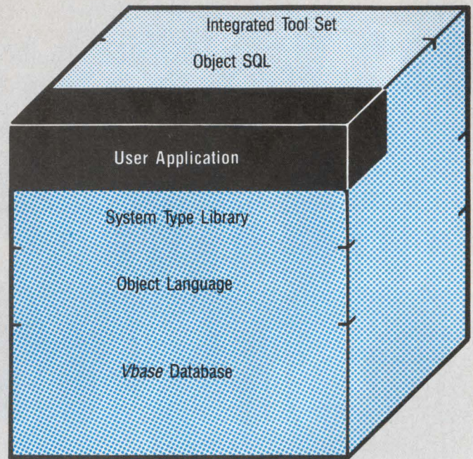
Integration of object databases allows a Vbase application to reference internal and external data and code.
