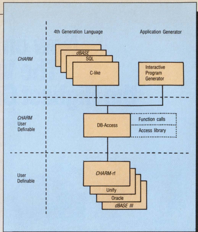
CHARM separates the three aspects of the application into distinct conceptual units.
