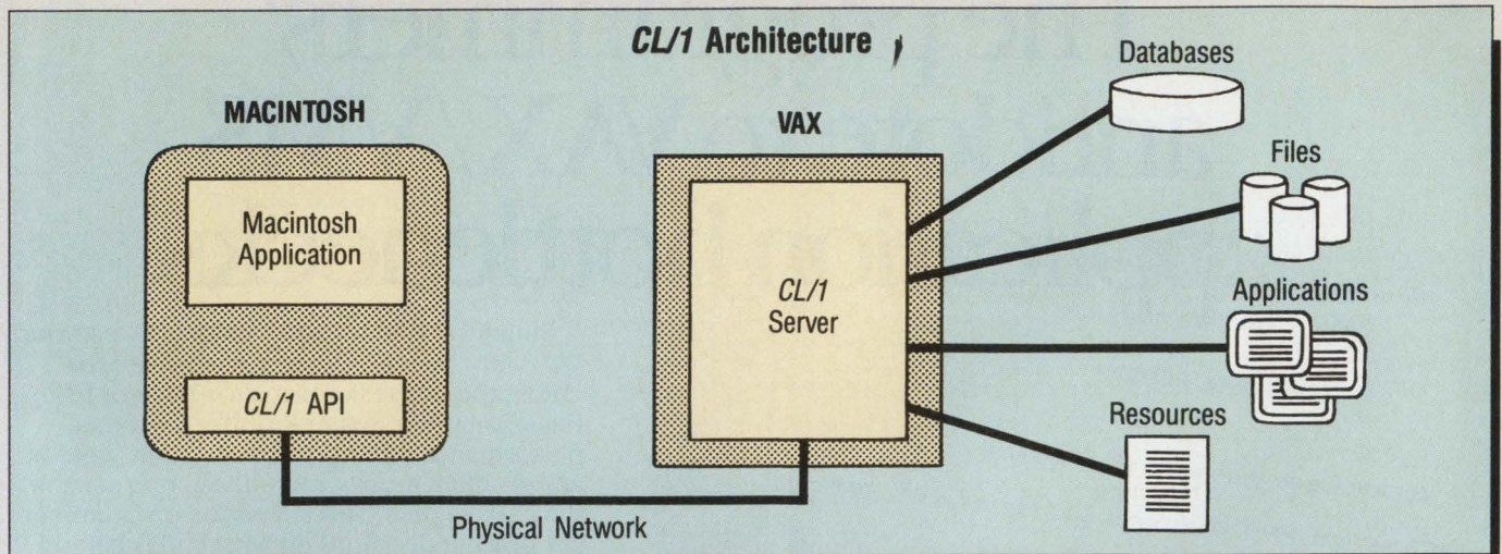
CL/1's Application Program Interface corresponds with a CL/1 server on the VAX over DECNET or Appletalk.
