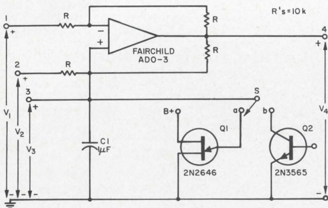
Grounding capacitor C permits use of a standard integrator circuit in a variety of modes determined by electronic switches Q1 and Q2 .
