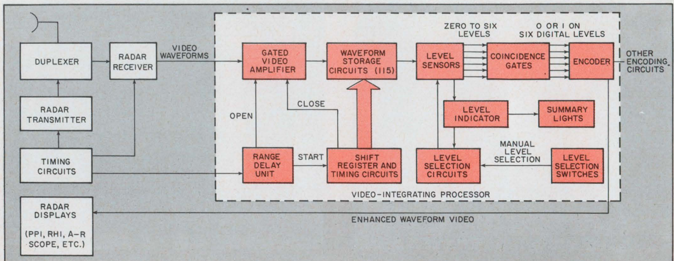
Video-integrating processor contains 115 RC integrators, each corresponding to 1-mile range storage bins.
