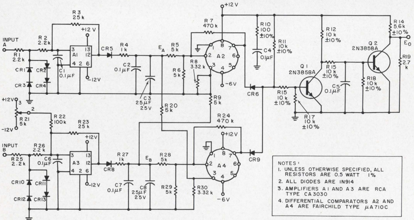
Amplitudes of two sinusoidal signals are compared with the simple circuit above. Output signal, E_o , is obtained
