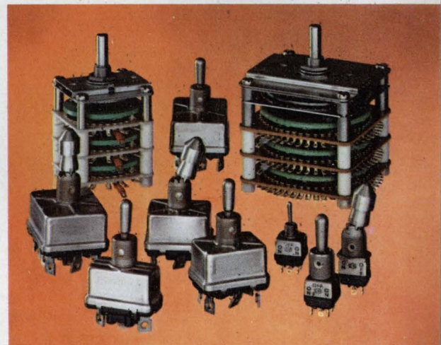
A few of the thousands of military switches available from Cutler-Hammer: miniature, and standard-size positive-action toggle switches (MIL-S-8834), Shallcross rotary switches (MIL-S-3786).
