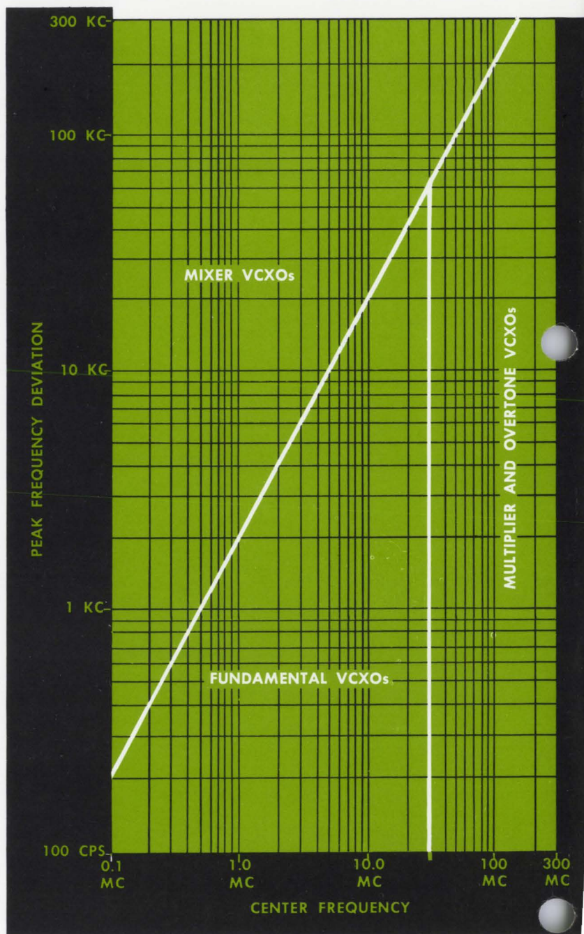
Figure 4 — Characteristic Graph: Peak Frequency Deviation vs. Center Frequency
