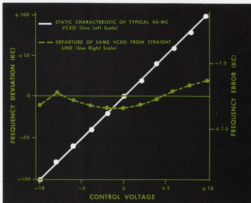
Figure 3 — Typical VCXO Linearity Plot
