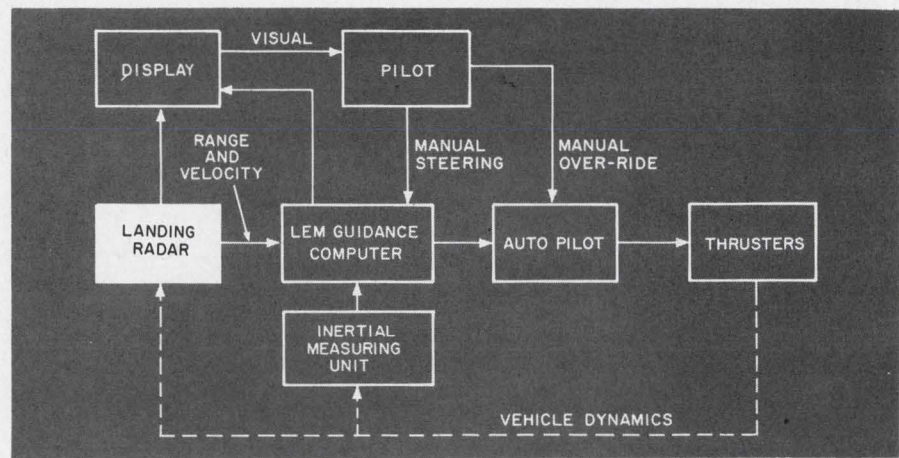
LEM computer controls spacecraft descent with data input from inertial guidance unit above 40,000 feet, and from landing radar at lower altitudes.
