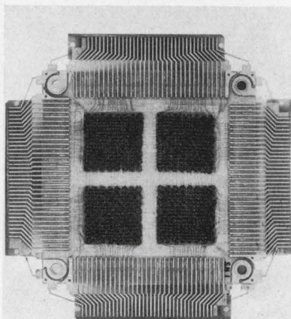
Array detail of 256 \times 8 transfluxor array for first DRO/alterable NDRO core memory stack.
