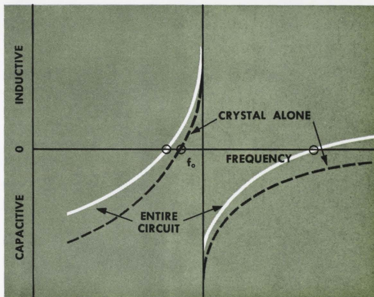
Figure 2 — Reactance-Frequency Plot for Typical Damon VCXO
