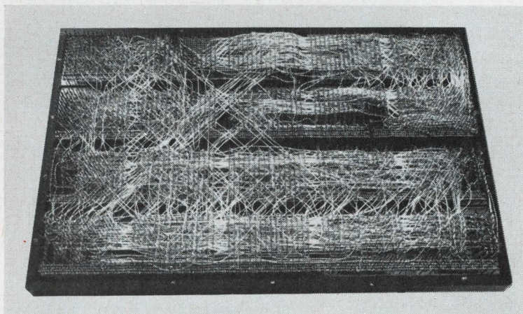
Panels pre-wired at AMP's Harrisburg facilities give you the benefits of automated production without requiring capital investment.
