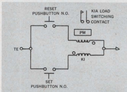
1. 'Moebius' counter will not lock up in subsequence.
