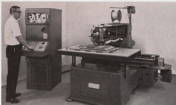
Tape-programmed TERMI-POINT Automatic Wiring Machine routes and fully terminates a 10" lead in less than four seconds.
