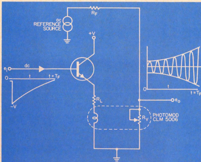
1. Photomod produces ac output ramp that is controlled by the dc input ramp. The emitter-follower stage provides isolation and current gain.
