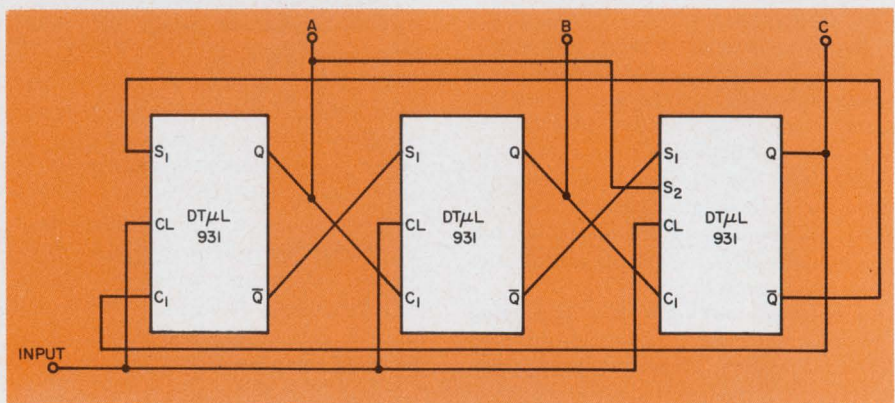
2. Twisted-ring counter also escapes unused states.
