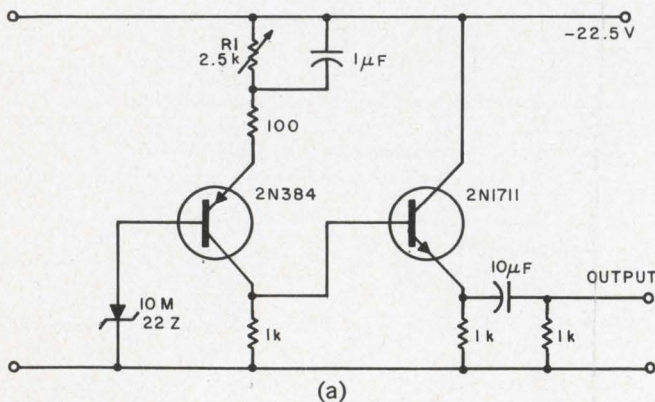
Random-signal generator (a) uses Zener diode as a "noise" source. The time base is 5 ms/cm in (b) and 0.1 ms/cm in (c). Output voltage can be set anywhere between 4 and 10 V peak-to-peak.
