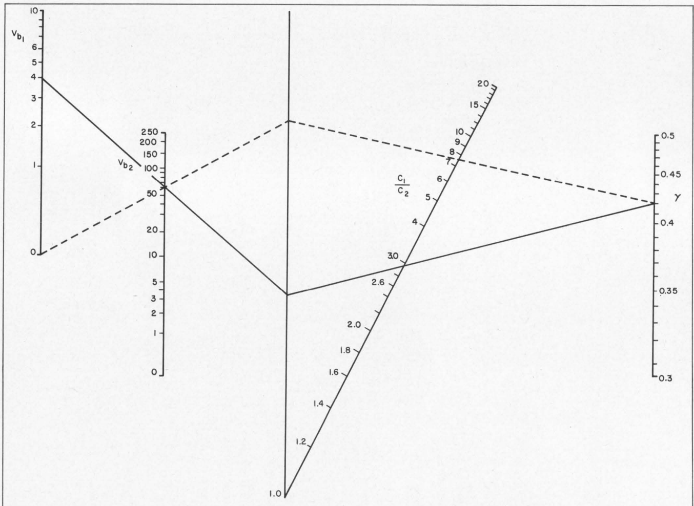
1. Changes in the ratio of capacitances with changes in the bias voltages are found with this nomogram. It also helps to find \gamma , the exponent in Eq. 1, that characterizes
