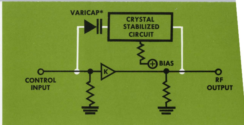
Figure 1 — Simplified Damon VCXO Schematic Diagram
