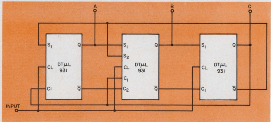
1. 'Moebius' counter will not lock up in subsequence.
