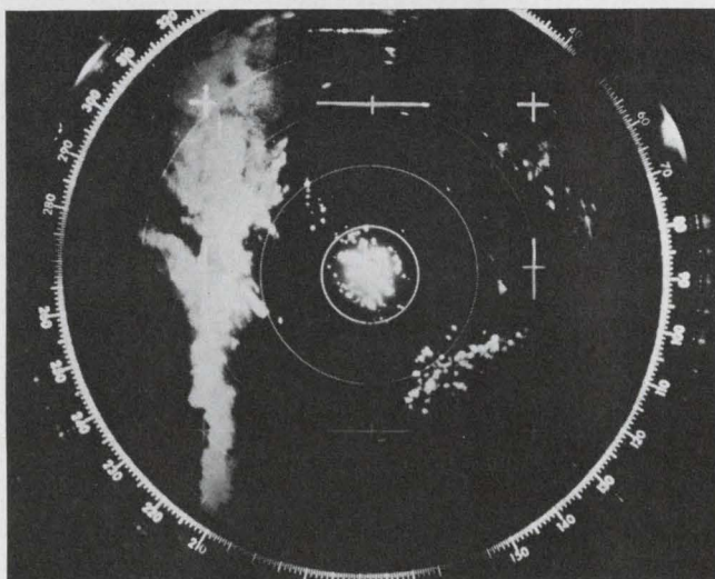
Integrating weather radar video signals produces the improved display shown at right. Use of three analog
