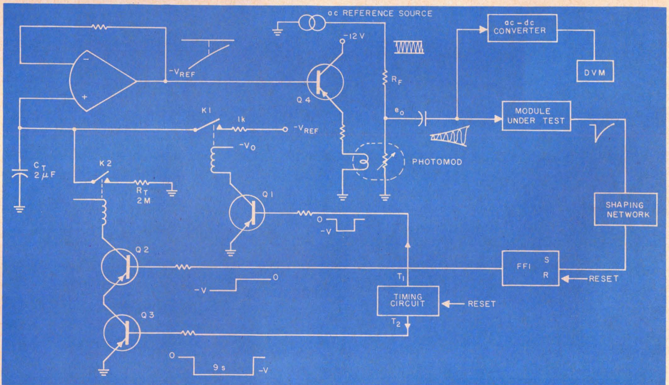
3. Thyatron firing is detected automatically by the system, and the input level at which firing occurs is read
