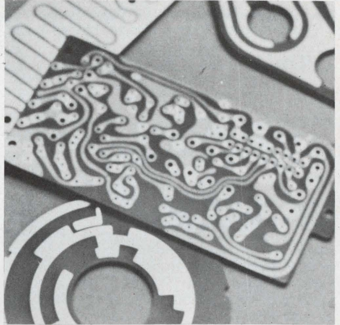
PC boards use 7-ounce beveled edge copper to increase load-handling capacity. Page 128
