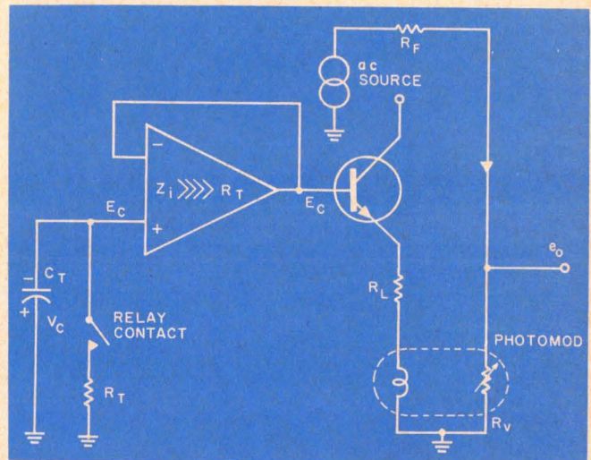
2. Dc ramp is generated when capacitor C_T discharges through resistor R_T . The high-gain dc amplifier couples the ramp to the base of the emitter-follower.
