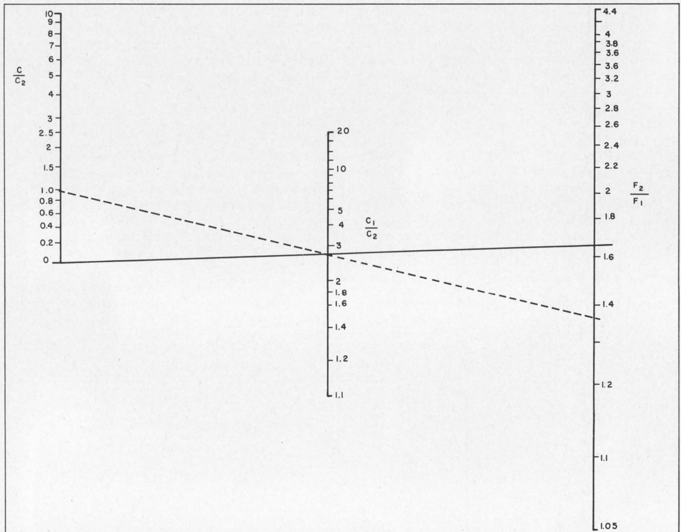
3. Circuit capacitances related to frequency range through the diode's capacitances are shown in this nomogram.
