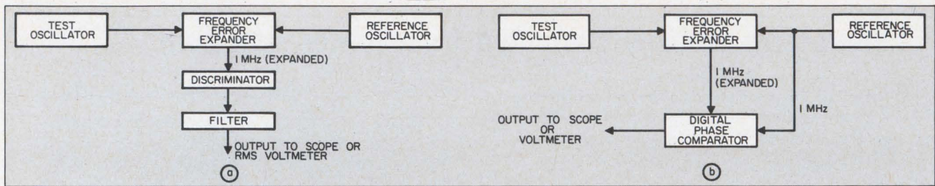
7. Error expander can measure short-term frequency stability (a) or phase stability (b). It accepts the input (between 250 kHz and 5 MHz), converts it to 1 MHz and
