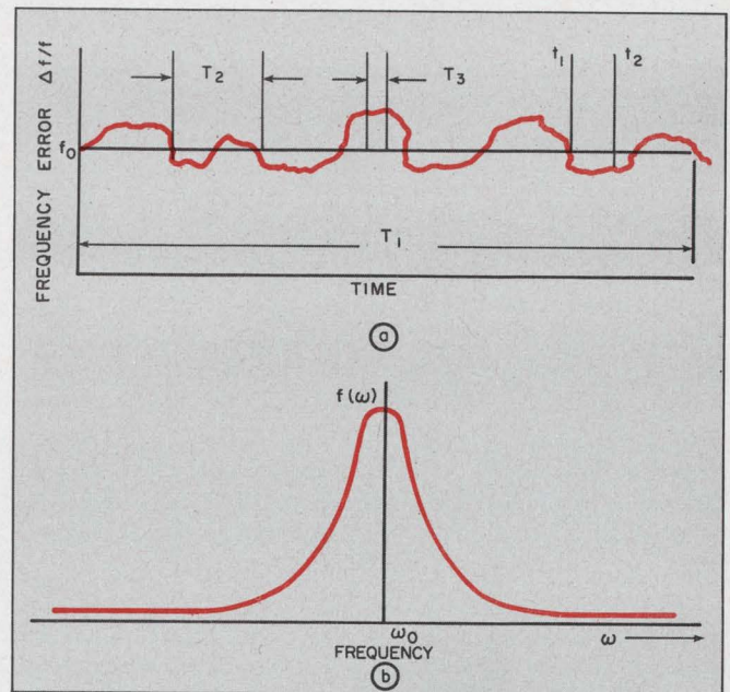
1. Random plot of frequency error variation with time (a) shows dependence of the averaged frequency error, \Delta f/t , on the observation intervals T_1, T_2, T_3 . In the frequency domain, a spectral density curve (b) must be constructed. The frequency perturbations give rise to sidebands.
