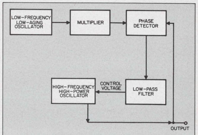
3. Complex frequency-correction scheme uses a high-power oscillator, the phase of which is controlled by a low-frequency, very stable oscillator.
