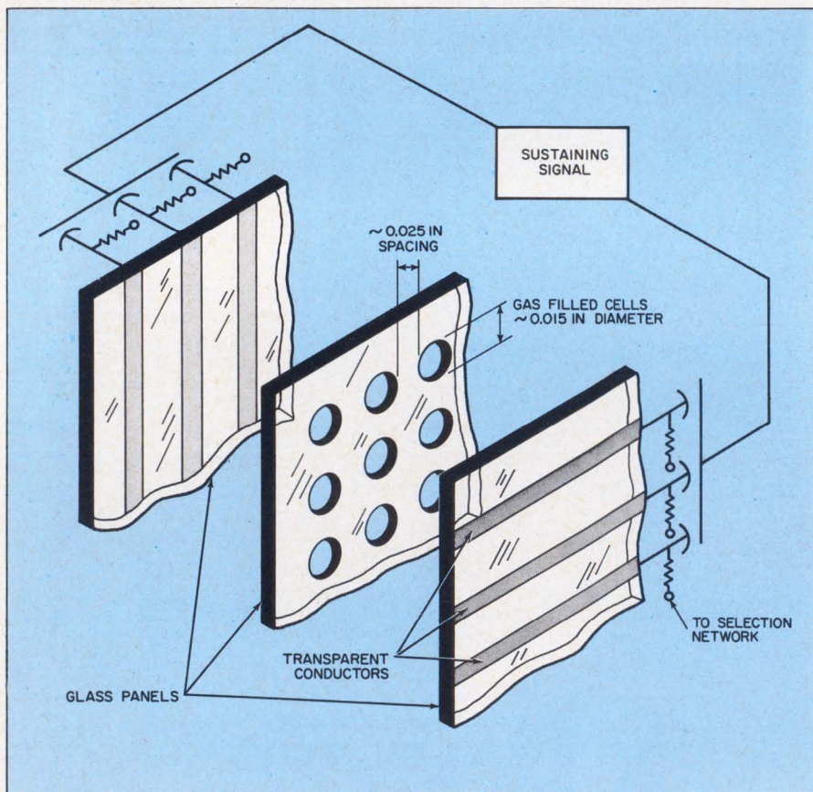
The plasma display panel (shown exploded) is a possible substitute for the CRT in computer displays. Signals directly from the computer combine with the sustaining signal to fire gas cells and form characters.
