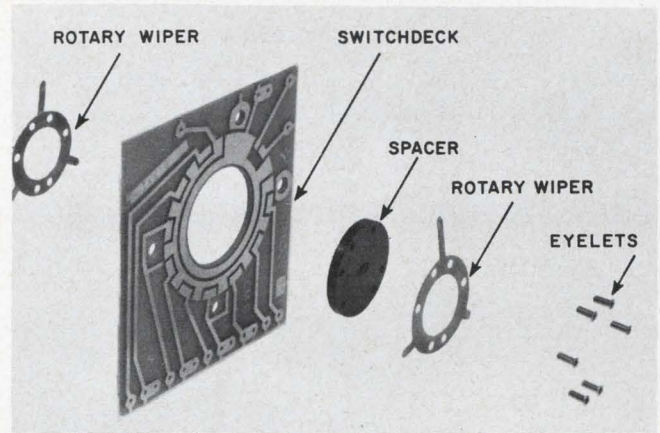
2. Exploded view shows relationship of printed-circuit rotary switch parts.
