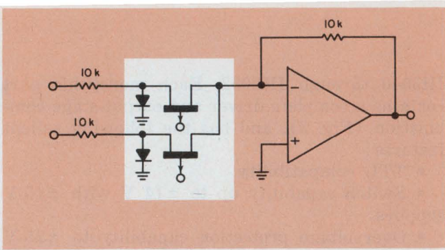
4. Virtual-ground switches provide an economical alternative for switching low-level signals, such as the inverting input of an op amp. Two channels of a 5009 series are shown. The family can be driven from TTL levels.
