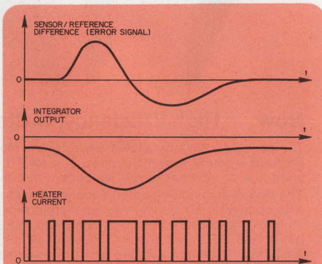
2. Heater current settles to a sustaining level as the error signal returns to zero after a change in temperature.
