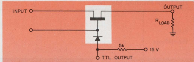
6. A positive-signal switch does not require an op amp, as with virtual-ground switches. One channel of an IH 5025 is shown. This switch family can handle signal levels as high as 30 V.
