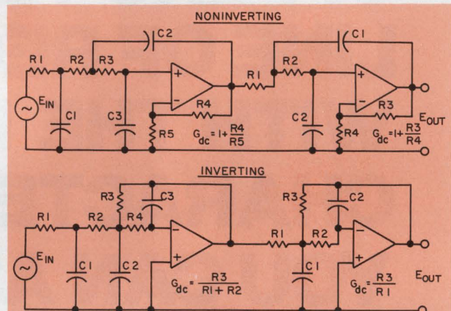
1. Multipole low-pass filters are designed and analyzed by the program. The user can choose noninverting or inverting gain stages. Filters containing up to 10 poles are designed from these four basic stages. Each op amp forms a two or three-pole section whose input is at R_1 .
