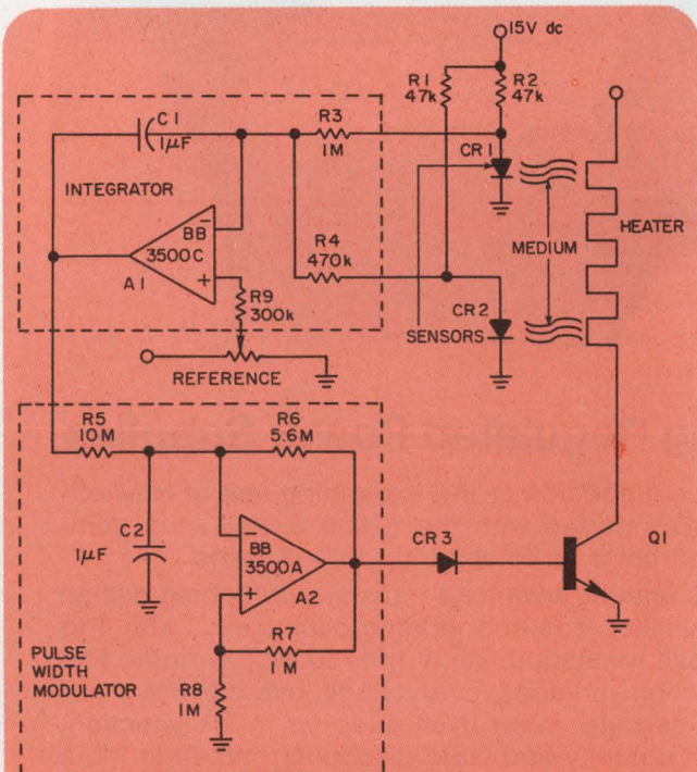
1. Proportional controller varies the heater-current pulse width to maintain equilibrium.
