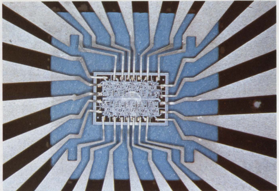
Lead frames used in the TAB process are etched from a metallized plastic film. Devices with up to 72 pins have been fabricated.
