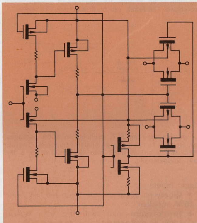
3. CMOS switches feature microwatt dissipation, switching capability up to 1 V of the power supply voltage and low ON resistances over wide signal voltages. Shown here, the monolithic IH 5042.
