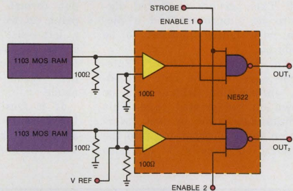
NE522 COMPARATOR USED AS MOS RAM SENSE AMPLIFIER
