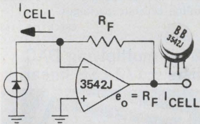
PHOTOCELL AMPLIFIER
