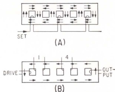
FIG. 2—Multiaperture square-loop ferrite logic combines set windings (A), and drive and four hold windings (B)
