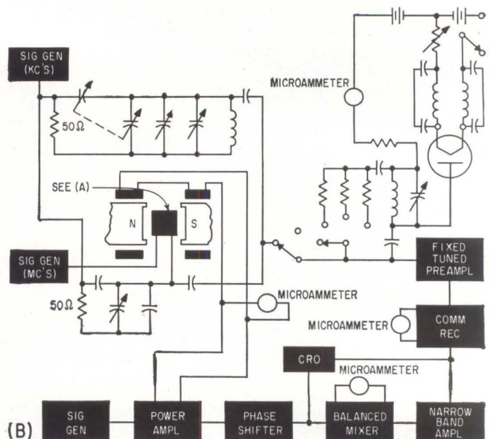
Simplified schematic of Overhauser method (A) and nuclear magnetic resonance circuits (B) being explored by Arma's basic research department
