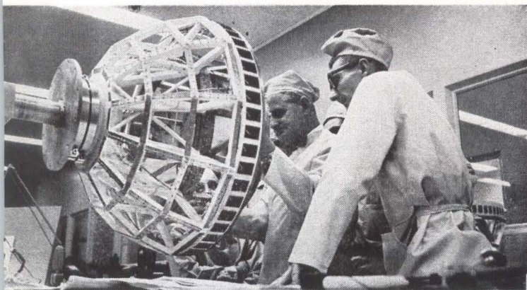
Canister containing electronic systems will be suspended in center of magnesium frame by shock-absorbing nylon cords
