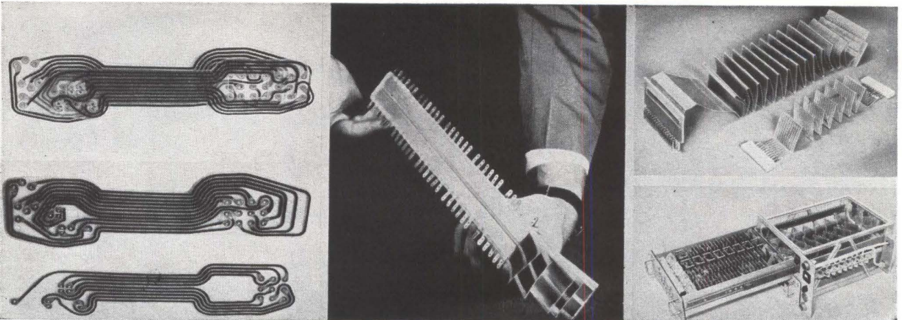
Two flat etched cables, superimposed (left, top), permit significant size reduction where space is a premium. Multi-layered power distribution cable (center) has exactly reproducible electrical characteristics. Flat accordion-fold cable (right) has a permanent heat-set spring for stretch-retract situation.
