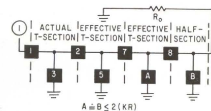
FIG. 2—Reduction of binary output commutator to actual and effective T-sections
