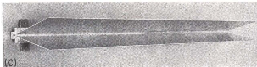
FIG. 2—Dielectric-loaded antenna (A) and effect of frequency on its beam position (B). Dielectric-loaded antenna of (C) operates in the X-band
