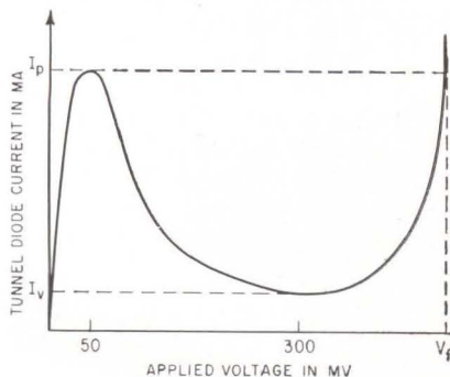
FIG. 1—Typical negative resistance characteristic of a single tunnel diode showing peak and valley currents and final voltage
