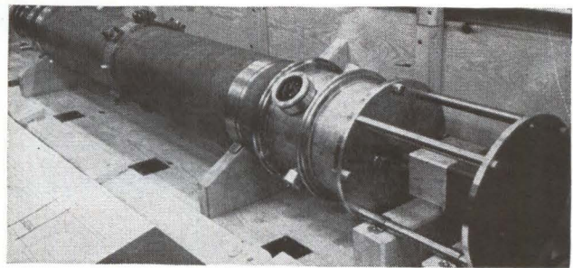
FIG. 5—400-Mc traveling-wave tube produces 100 Kw
