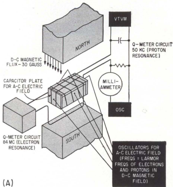
Simplified schematic of Overhauser method (A) and nuclear magnetic resonance circuits (B) being explored by Arma's basic research department
