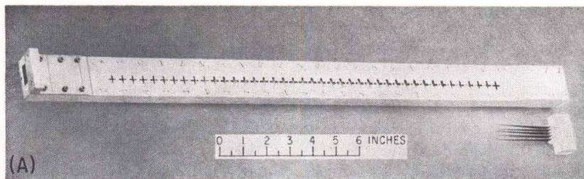
FIG. 3—Antenna (A) consists of an array of waveguides that radiate through their slots. Curves in (B), (C) and (D) at right, on next page, show effect of frequency on characteristics of the antenna's main beam
