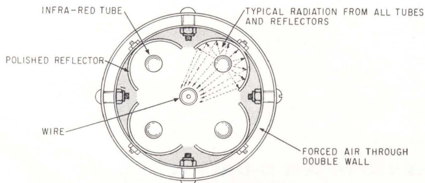
Teflon wire passing through the center of the oven is heated enough to make a permanent fusion between insulation and Teflon markers
