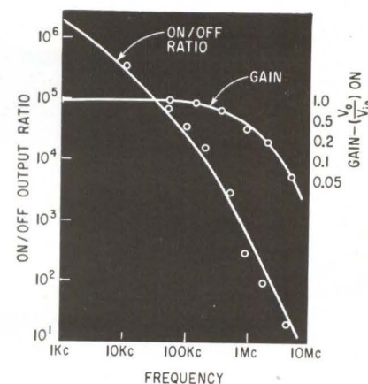
FIG. 3—Gain and on-off ratio for an eight-channel binary output commutator plotted against frequency
