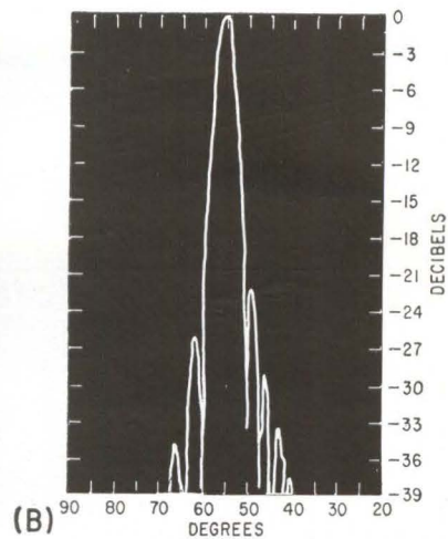
FIG. 1—Cylindrically contoured leaky-wave antenna (A) and its experimental H-plane pattern (B), measured at 11.42 Gc
