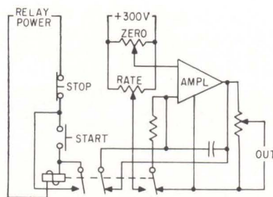
FIG. 2—Ramp function generator for testing indicator uses dual-input operational amplifier connected as integrator
