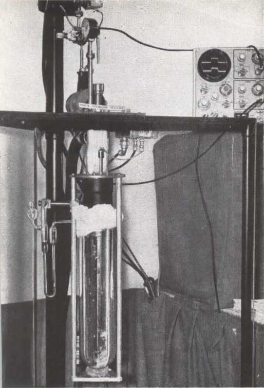
FIG. 1—Crystal detector for millimeter wavelengths is cooled to 1.5 K
