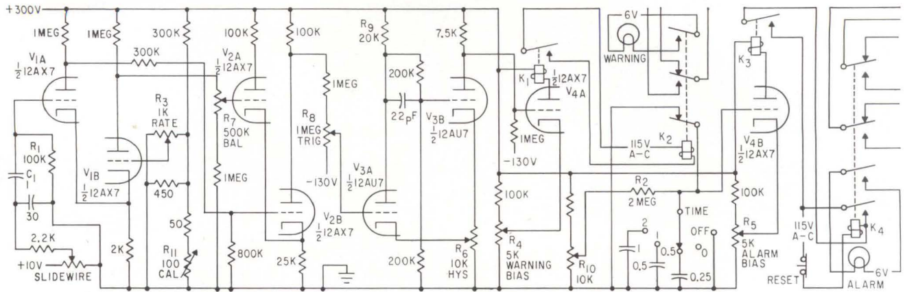
FIG. 1—Circuit lights warning lamp if rise rate exceeds preset limit and alarm lamp if excessive rise rate persists beyond preselected time delay
