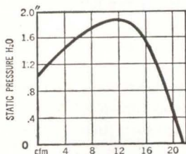
Typical performance at 22,500 rpm
