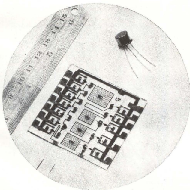
DIODE-SWITCHED tuner developed at General Instrument applied research laboratory covers range of 50 to 200 Mc—Fig. 5
