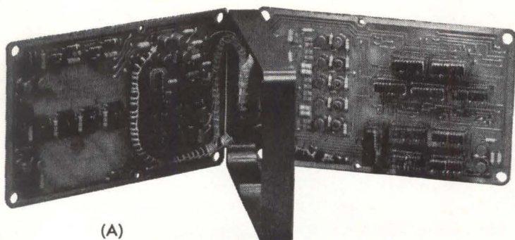
ONE OF FOUR standard wafers that comprise the logic in Arma's 20-lb space computer
