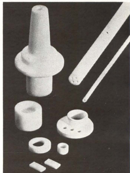
Typical Beryllium Oxide Ceramic Shapes Being Produced by Coors—.026" to .375" OD rods; lengths to 24", in larger diameters.
