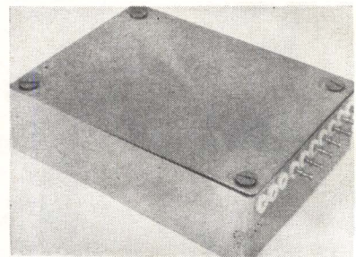
HEAT SINK for module is completed with mounting of metal covers, which also protect encapsulating gel
