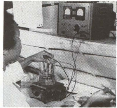
FOUR microinches of 24-karat gold coating is deposited in less than one minute in plating silicon disks
