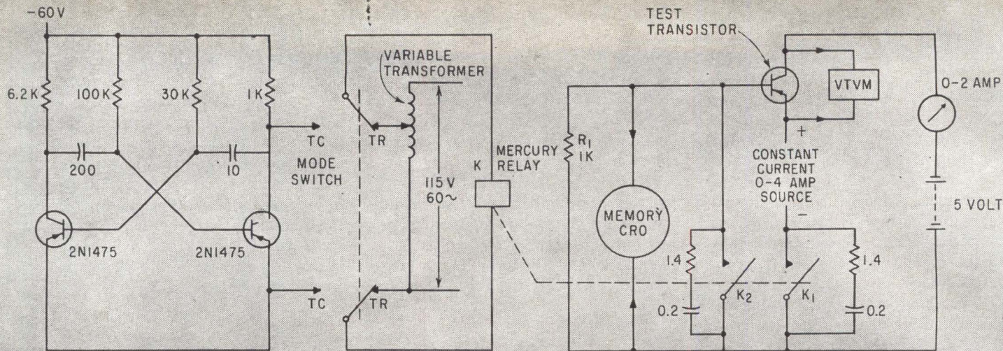
MULTIVIBRATOR pulses relay K during time-constant determination; 60-cycle supply drives relay for thermal resistance testing—Fig. 1
