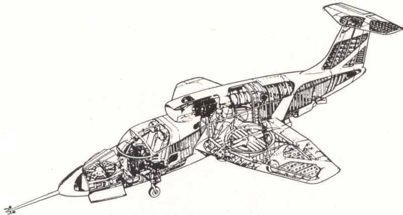
ARMY RESEARCH VTOL aircraft uses GE jet engines in Ryan-built airplane. Jet streams are diverted to turbine edges of lift fans in wings and nose for vertical take-off and landing
