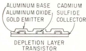
TRUE INTEGRATED thin-film circuits could result if research on these active thin-film devices is successful—Fig. 12
