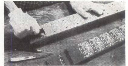
SCRAP COPPER is easily peeled from stamped phenolic strips
