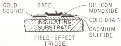
TRUE INTEGRATED thin-film circuits could result if research on these active thin-film devices is successful—Fig. 12
