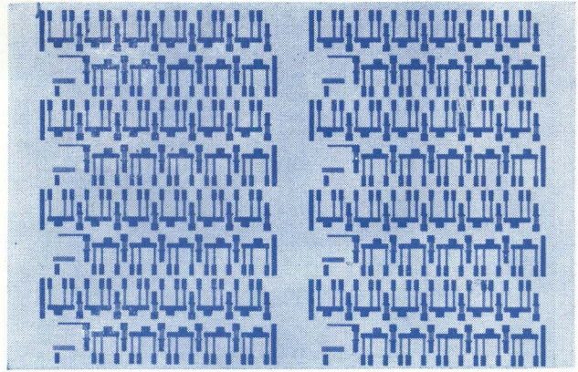
(2) Resistor Lands, Some Cu Interconnections
