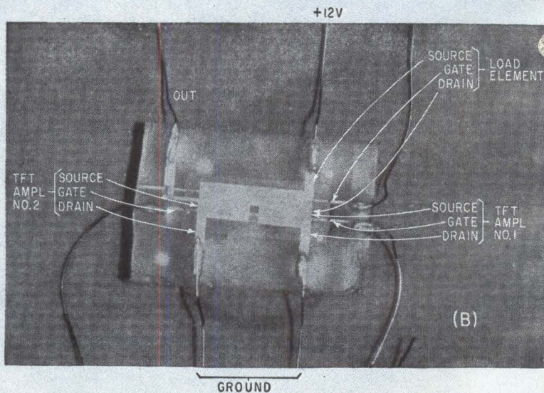
TWO RCA TFT's with typical characteristics as shown in (A) are used with a common load resistor in NOR gate (B); a 5-v pulse applied to input of either TFT gate (C) causes output to drop by 3 v (D). Two-stage audio amplifier (E) has circuit (F) which is not yet fully operative but has first stage waveform shown for 10-Kc input in (G)—Fig. 13
