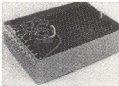
END-CONNECTION terminals and test points are brought out of the wired module to be soldered, wire-wrapped or welded
