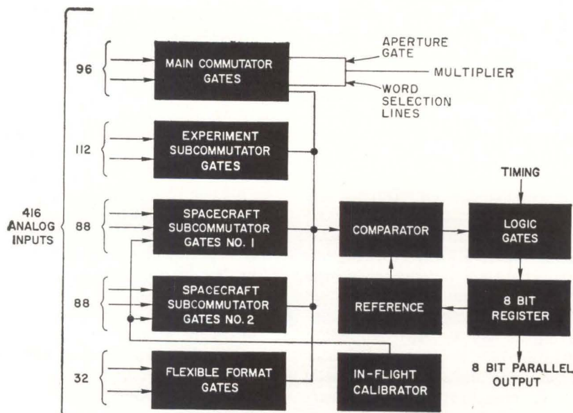
ANALOG data handling assembly contains gates for the main commutator, experimental subcommutator, two spacecraft commutators and an analog flexible format gate—Fig. 3
