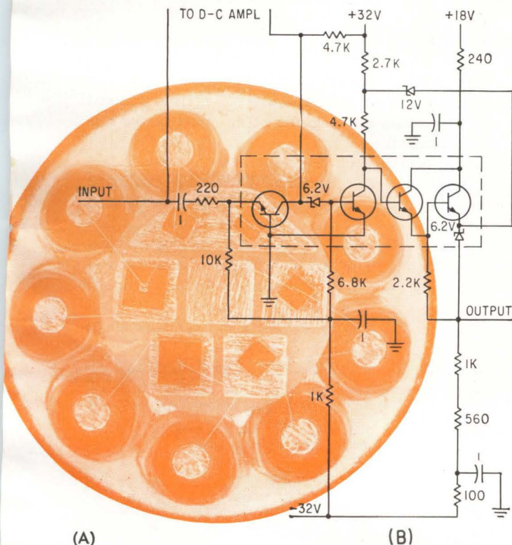
INTEGRATED CIRCUIT package (A) for Bell Labs high-frequency operational amplifier module (B) contains two experimental 2-Gc planar epitaxial transistors and two silicon zener diodes. External d-c stabilizing circuits and feedback loops are not shown—Fig. 2
