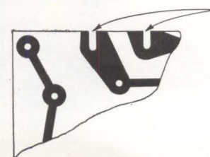
OVERSIZED PADS are located in areas of especially high component density to reduce mechanical stresses during assembly—Fig. 3
