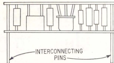
COMPONENT location technique drastically increases heat conduction to protect parts against overheating—Fig. 2
