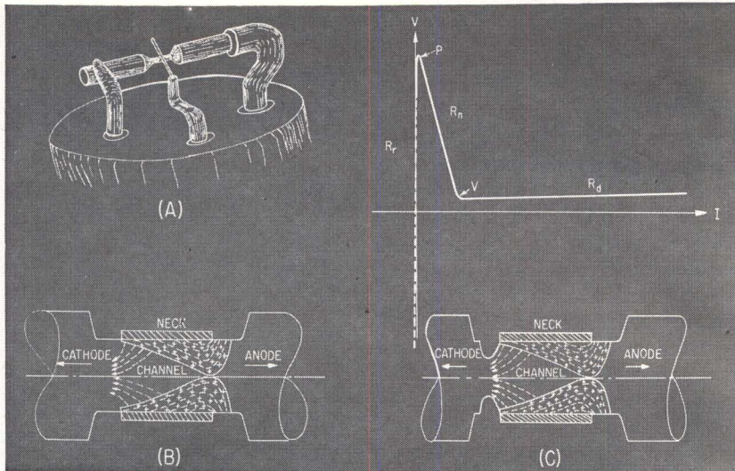
FIELDTRON (Tecnatron) field effect transistor. Grooved active assembly is shown in mounting position in (A). Electron flow at neckdown section is indicated in (B). Electron flow at the subgroove section of the bistable switching type and I-V plot are diagrammed in (C)
