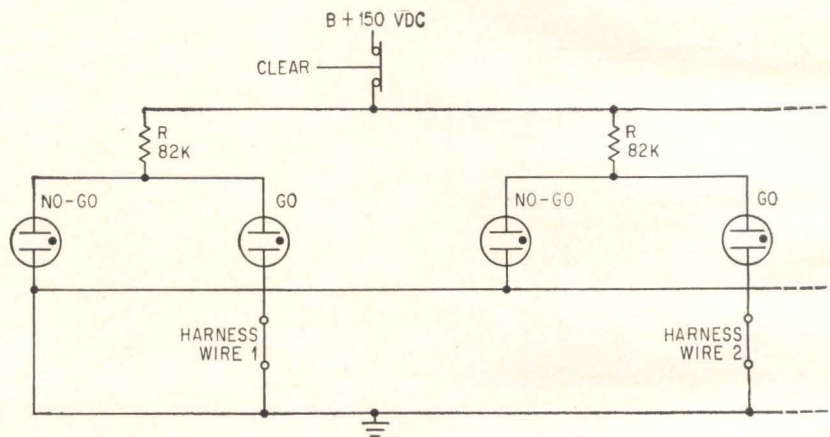
HARNES TESTER uses two neon lamps per conductor to indicate conditions during test. Momentary fault turns on NO-GO lamp until CLEAR switch is used
