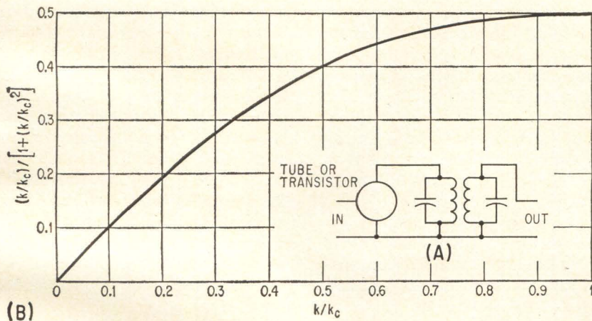
TUNED vacuum-tube or transistor amplifier (A); plot of (k/k_c)/[1+(k/k_c)^2] versus k/k_c (B)—Fig. 3
