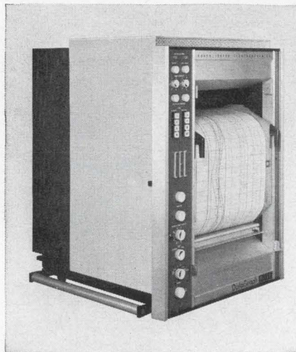
BENCHMOUNT CONFIGURATION
