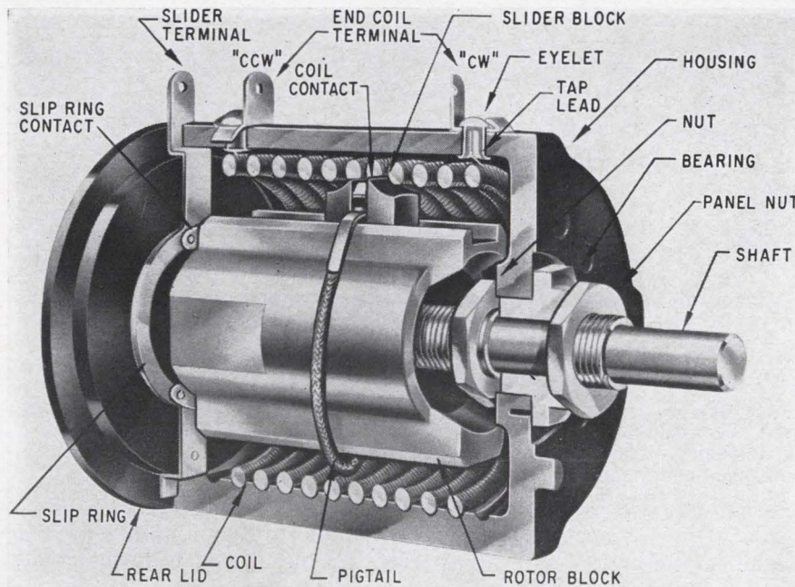
Multiturn wirewound potentiometer, shown in cutaway view, has been greatly improved by using more uniform wire and better coil-encapsulation techniques; new oils and greases lubricate wire paths, inhibit oxidation and entrap wear debris away from the contact path.
