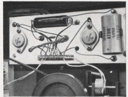
Ten-position Junction Block, accepting TERMI-POINT terminals, connects various components in the rear tape deck section.
