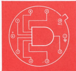
LU305 AND GATE
