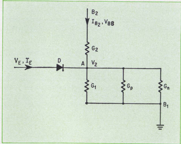
Equivalent circuit for a unijunction transistor. G_p and G_n represent the excess hole and electron conductivities between the emitter and base one. G_1 and G_2 are the conductivities corresponding to R_{B1} and R_{B2} .
