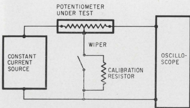
Noise-test circuit, established to measure potentiometer quality, may give false picture of noise performance.
