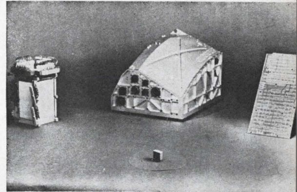
Gemini computer (center) shown with its memory element (left). In foreground is example of microcircuit used; these are interconnected with printed wiring plane similar to that shown at right.
