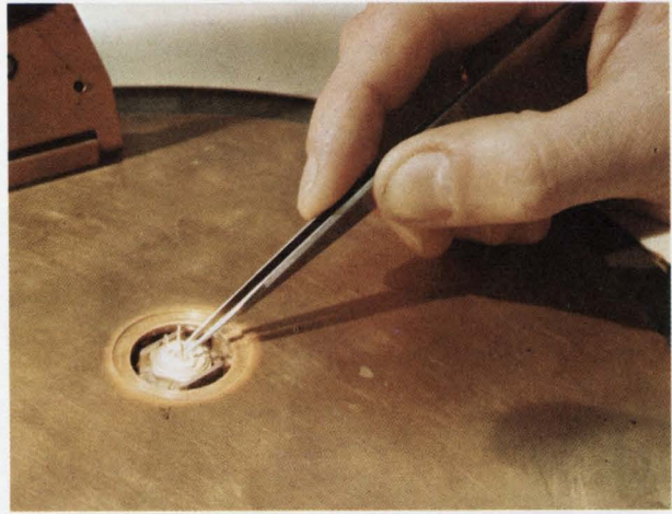
Pellet-mounting process. Here, the header is being inserted into a heating chamber. After a 30-second warm-up period, the pellet is placed on the header and connected to it with a gold-silicon alloy.
