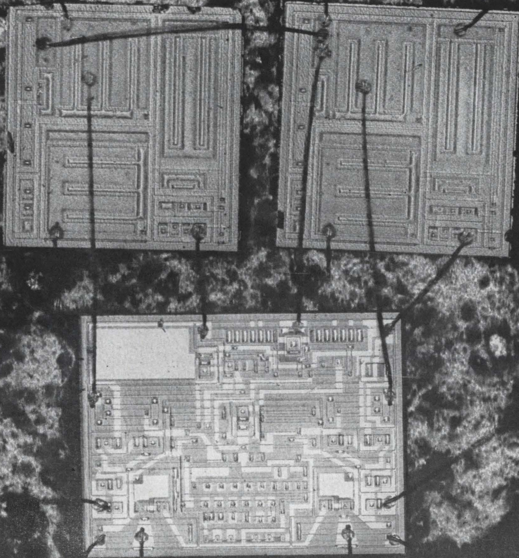
Forty-watt servo amplifier is made with three silicon chips, two carrying high-power transistors and one for control circuitry. Leads are aluminum wire; chips are aluminum-bonded to molybdenum.
