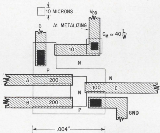
Mask layout to realize the function diagramed in the preceding illustration. The series connection on the left required twice the width for each transistor so that the total resistance of the series branch equals that of the parallel branch on the right.
