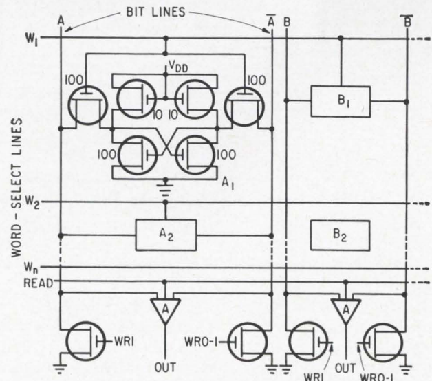
Nondestructive word-select memory laid out in MOS transistors. Each block represents a flip-flop which stores a single bit; one such flip-flop is shown in detail at the upper left.
