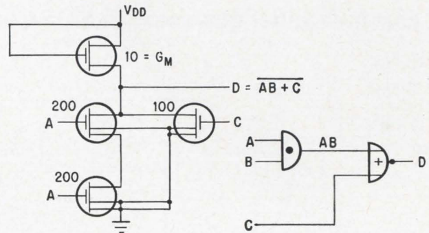
Simple logic function implemented in MOS devices. Note the series connection of two transistors, possible only because of the high input impedance and, therefore, negligible base current found with these devices.
