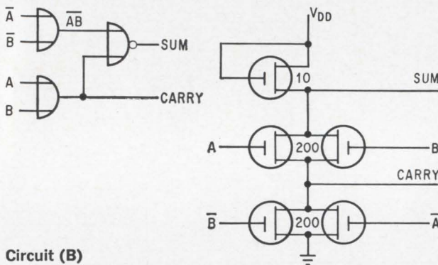
Circuit (B)
