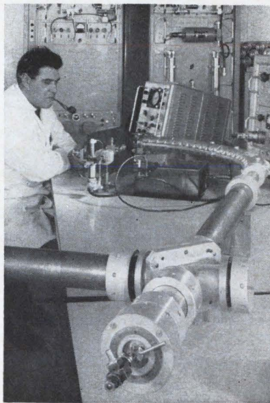
Experimental waveguide being tested at CGE research center in Marcoussis.
