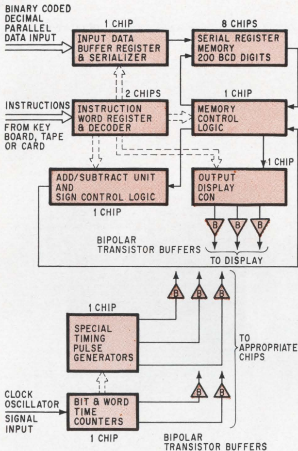
Typical serial computer in block diagram form. By using MOS integrated circuits instead of double-diffused, epitaxial integrated circuits, the number of IC's required is only 16. If conventional IC's had been used, nearly 1,000 would have been needed.
