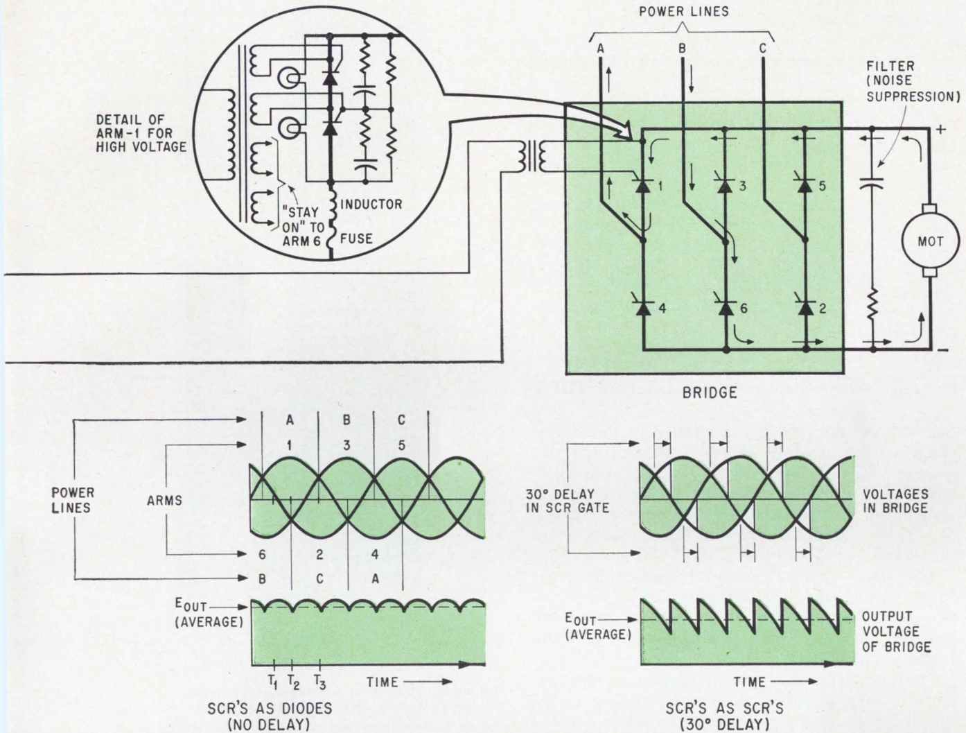
The three-phase scr bridge above is the basic building block of the 10-megawatt amplifier. Two scr's are used per arm, as shown in the insert, to make the bridge able to handle 700 volts with available scr's. The wave forms below the bridge show how the three-phase input is converted by the scr's into variable-voltage d-c output. At zero triggering delay ( V_i=20 volts), the bridge is at 100% output. At about 30° triggering delay ( V_i \approx 17 volts), the bridge is at 80% output.
