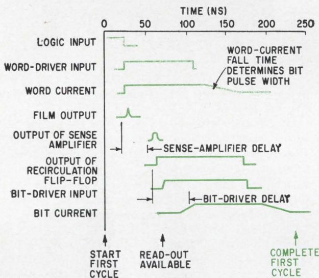
Memory cycle timing diagram. Times to perform each of the memory's read and write operations are measured in nanoseconds. The complete cycle takes 250 nanoseconds.
