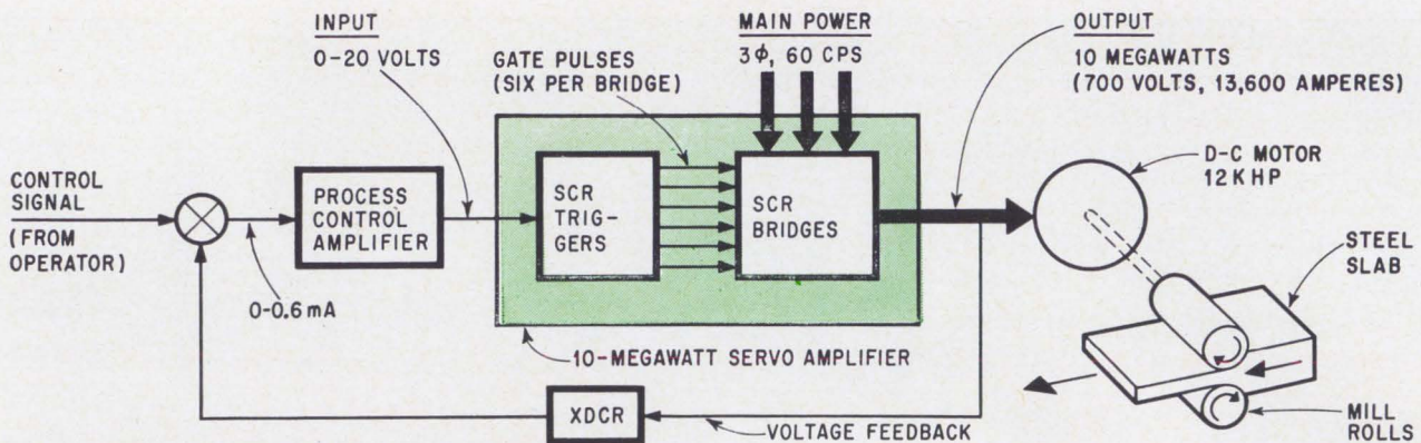
The servo loop in which the 10-megawatt servo amplifier operates. The amplifier is composed of scr bridges and the scr triggering circuits. Together, these circuits must take a 0-20 volt input signal and produce 0-700 volts output. (For simplicity, the identical bridge needed to drive the motor in the opposite direction is not shown).
