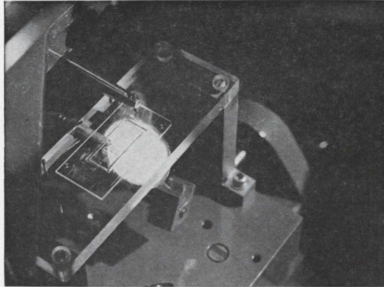
Ultrasonic bonder is set up to weld integrated-circuit chip to glass substrate. The operator peers through a microscope to align the bond points. Although this looks like a fussy, time-consuming operation, it is far faster than conventional circuit-assembly methods because all contact points are welded simultaneously. The substrate is seen in the closeup.
