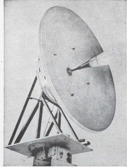
The Dielguide , a polystyrene cone that funnels electromagnetic waves between feed and reflector. In the photo of a Cassegrain antenna, right, the Dielguide juts out in front of the main reflector. Above, in the photo of a prime focus antenna, it covers the entire face of the reflector.
