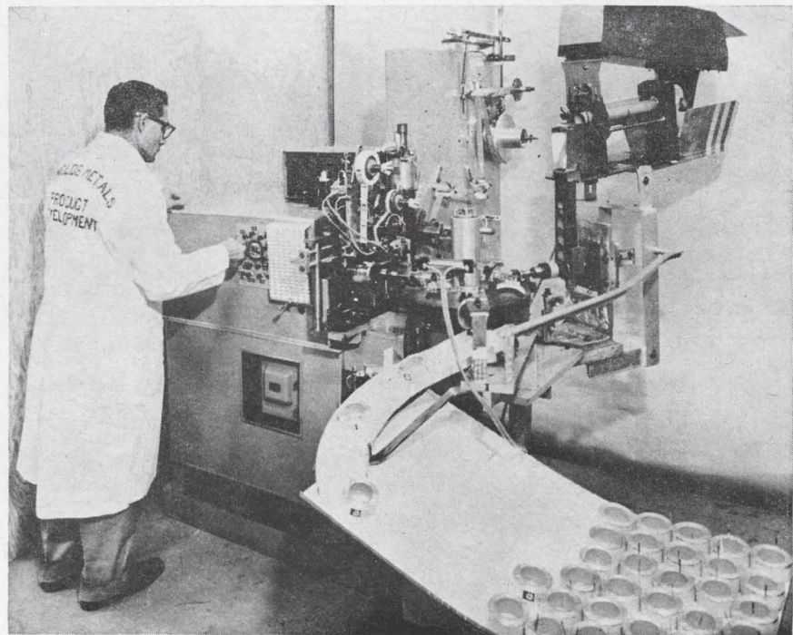
Automatic aluminum foil winding machine introduced by Reynolds. Up to 120 coils an hour can be wound with the machine, and one operator can tend several machines.
