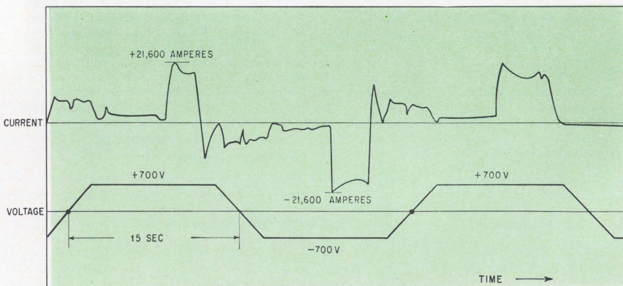
Currents and voltage for driving a 12,000 horsepower motor are immense. These traces taken from data obtained during the operation of the Burns Harbor rolling mill show that while the voltage varied from minus to plus 700-volts (d-c), the current went as high as 21,600 amperes.
