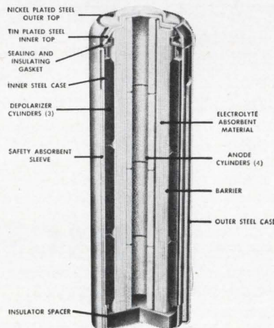
Internal construction of cylindrical Mallory Mercury Cell.
