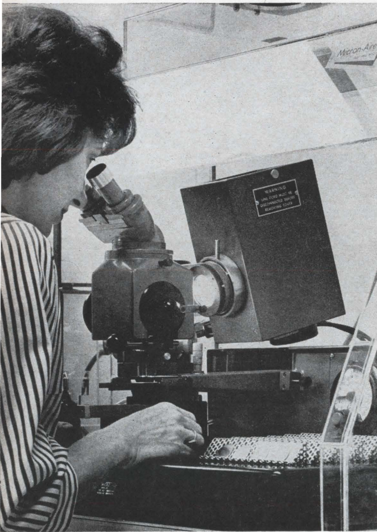
Operator aligns working plate with silicon wafer for exposure of photoresist with ultraviolet source.
