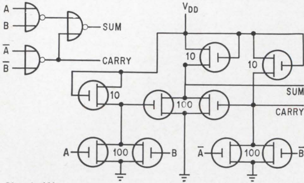
Circuit (A)
