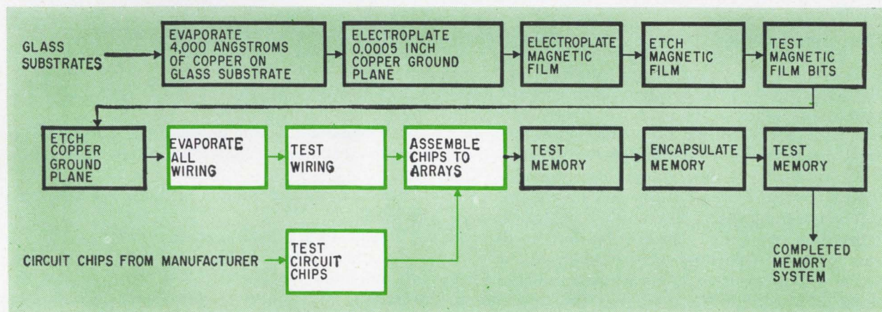
How to build a tiny memory: vacuum-deposit (evaporate) and plate the memory plane conductors, evaporate and etch the magnetic film, evaporate several layers of thin-film interconnection wiring for circuitry connections, add chips and test. Only the steps in color are needed for face bonding.
