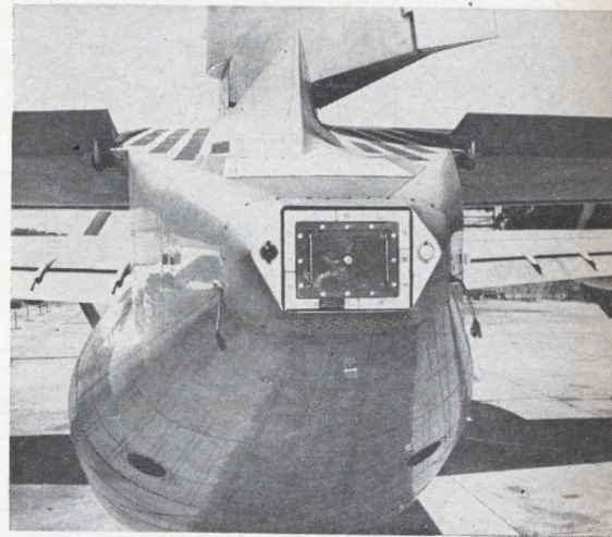
Crash recorder attached to tail of Cargomaster picks up information from 86 transducers and four voice channels.
