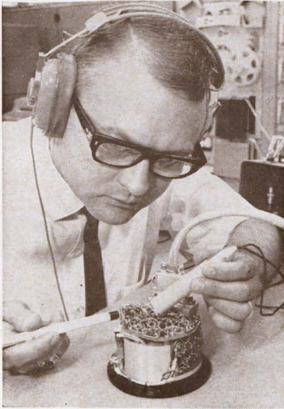
Listening for r-f noise in a micro-electronic assembly is Richard T. Stevens, senior systems development engineer at Honeywell.
