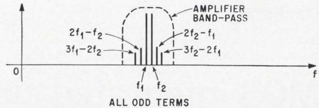
Two signals, close together, are used in the narrow band method of distortion analysis. The amplifier under test has a narrow pass-band, and the intermodulation terms measured are restricted to this band. As shown in the diagram above, these terms are all odd.
