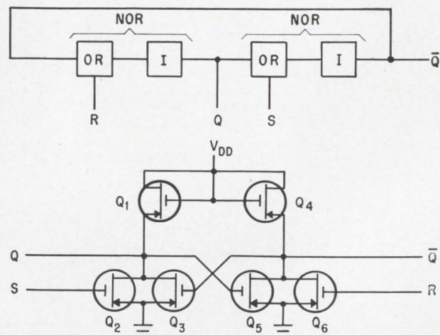
A set-reset flip-flop formed by a pair of NOR gates. The circuit stores one bit of information. The flip-flop state is permanent until the circuit is reset (or set). This circuit is a basic building block for complex counters and shift registers.
