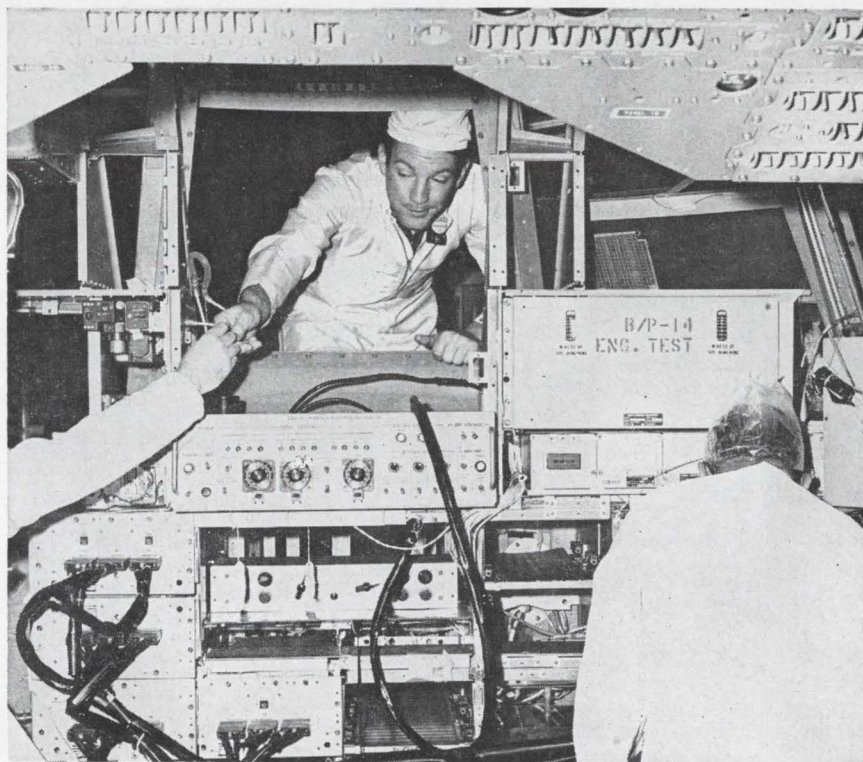
Block I communication and data subsystem, which will fly the first Apollo earth orbital missions, is being tested at North American Aviation, Inc. Many of the front connectors have been removed from the Block II version.
