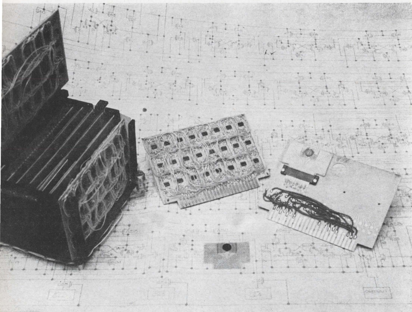
Breadboard system of small serial computer is at the left. Next to it is a typical logic card with 48 MOS integrated circuits: device count: 864 MOS transistors. A substitution logic card with single complex integrated circuit representing the 96 circuits is at the right. Miniature card with complex MOS integrated circuit is at bottom, center.
