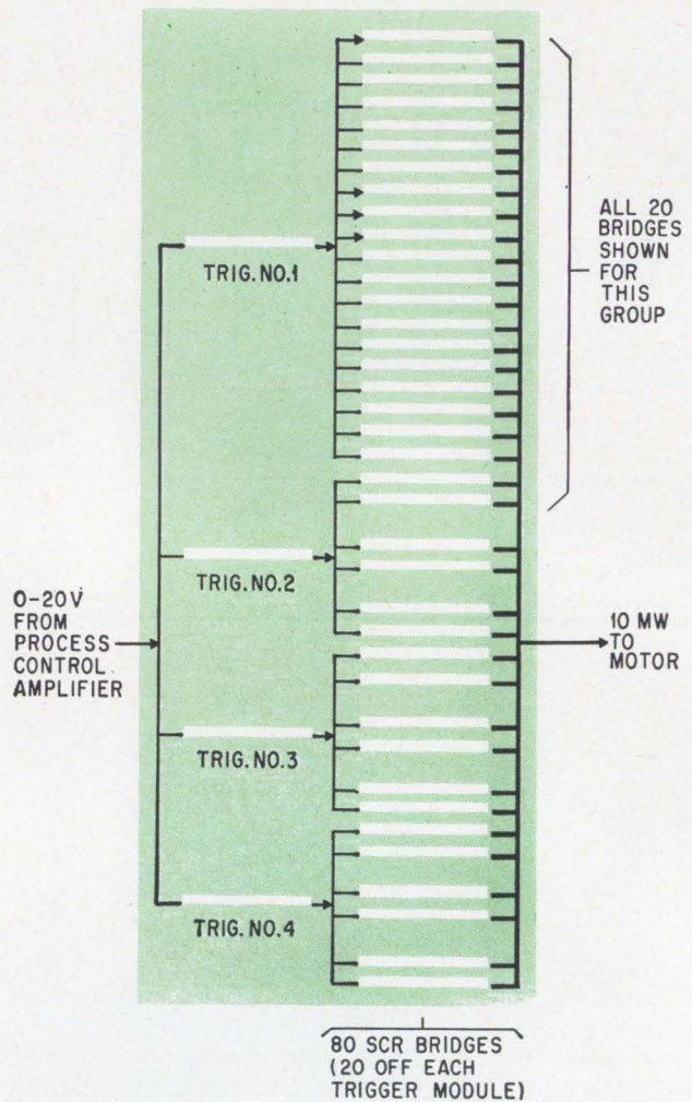
The fan-out needed to achieve 10-megawatts with present scr's. The single 0- to 20-volt control signal drives four scr trigger modules. These modules each drive 20 scr bridges.
