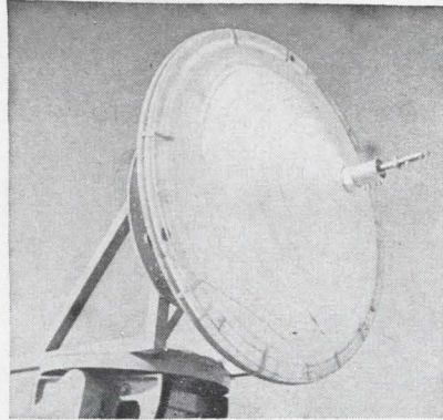
The Dielguide , a polystyrene cone that funnels electromagnetic waves between feed and reflector. In the photo of a Cassegrain antenna, right, the Dielguide juts out in front of the main reflector. Above, in the photo of a prime focus antenna, it covers the entire face of the reflector.
