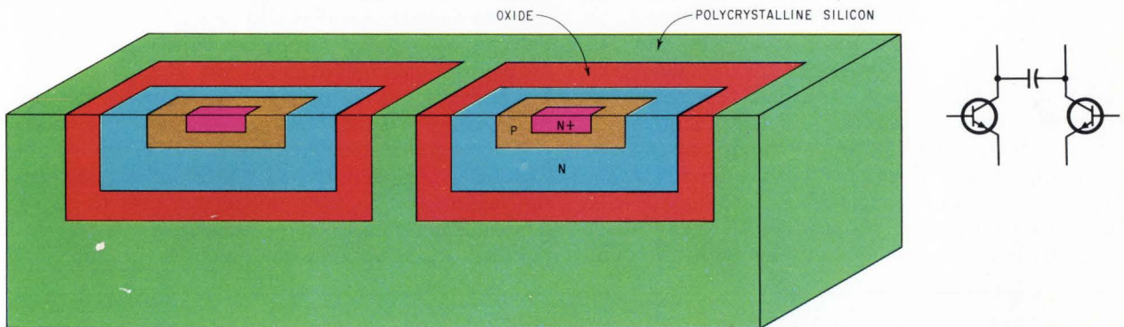
Twin pair of npn transistors in a dielectrically isolated IC are modeled by two npn transistors and a capacitor between their collectors. The model requires a capacitor between dielectrically coupled elements.
