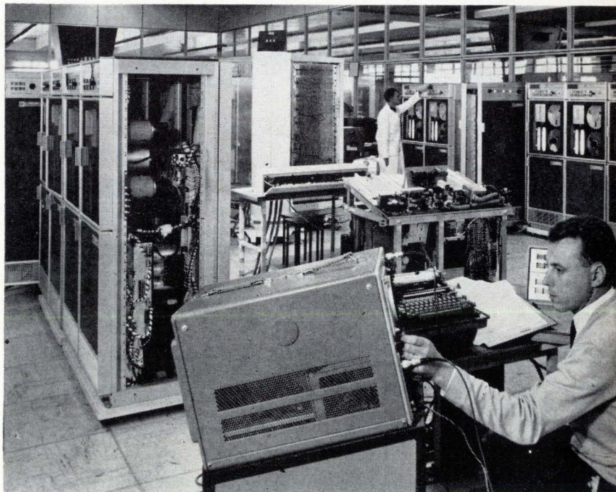
Bull-GE computer undergoes test in production area of French plant. General Electric is seeking a $30 million increase in the firm's capitalization.
