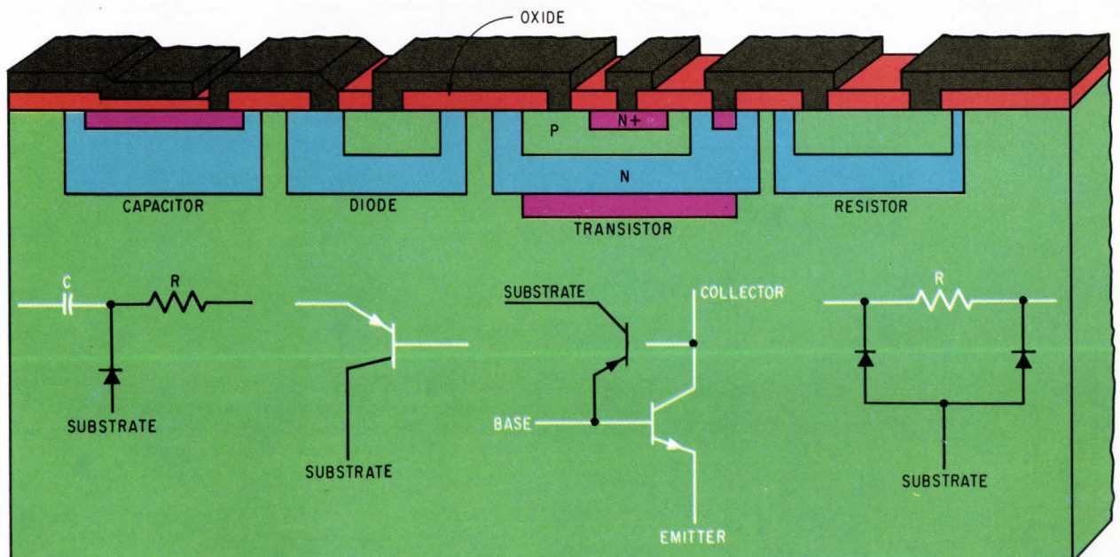
Each element in IC structure above is modeled by a corresponding element below. In each case, the intrinsic element (in white) is connected to a parasitic component (in black) that represents the interacting regions.
