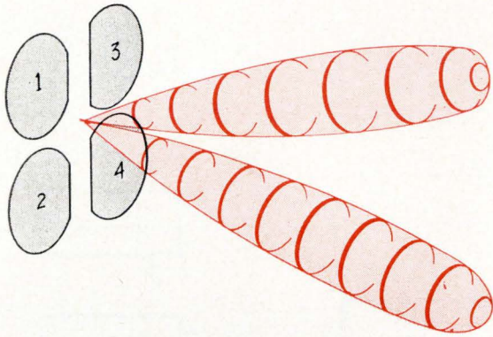
Difference beam for C-axis error signal is produced by subtracting the sum of beam 2 and 4 from the sum of 1 and 3.
