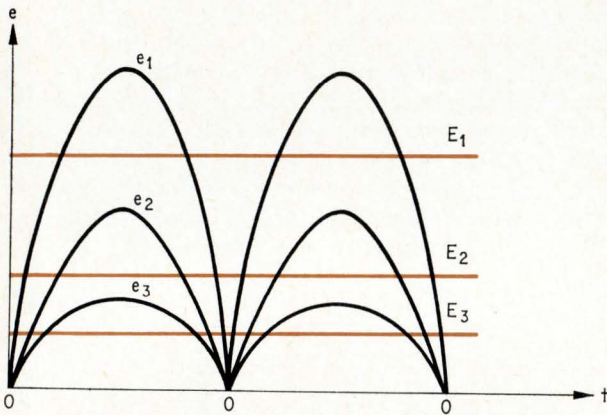
e_1, e_2 AND e_3 = RECTIFIED A-C E_1, E_2 AND E_3 = FILTERED D-C
