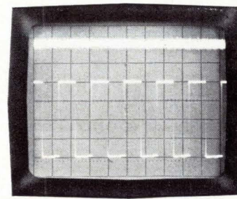
Measure frequency of signal in noise up to 560 kHz by using square wave output, hp as a counter preamplifier.
