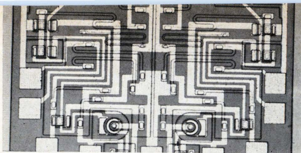
Twoifers. Dual operational amplifiers on a single chip represent the latest step in the evolution of linear IC's. The halves of this Motorola device can be operated independently or in parallel; they have only power-supply connections in common. Price is about 50% more than that of a single-unit chip.
