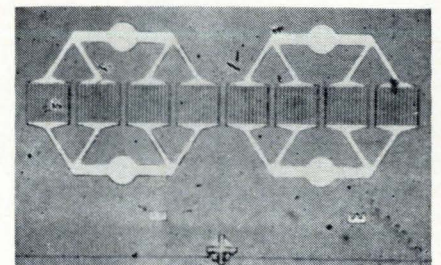
50 watts at 500 Mhz. Interdigitated transistor contains eight cells on each of two chips.
