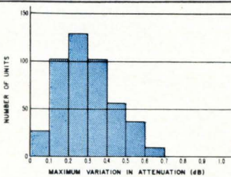
MAXIMUM VARIATION IN ATTENUATION—DC to 12.4 GHz for 463 production-run 8491A Attenuators (263 10-dB units, 200 20-dB units)
