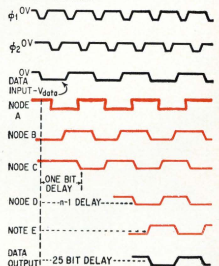
TIMING DIAGRAM
