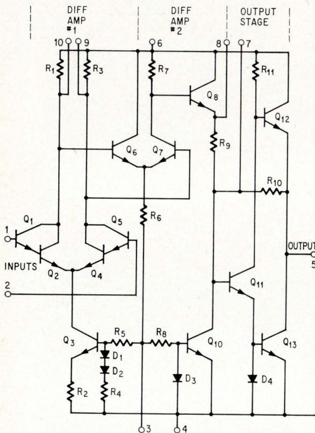
Operational amplifier. Two differential amplifier stages and an output stage make up this early off-the-shelf operational amplifier fabricated in a single chip.
