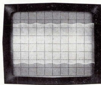
Measure 10 mV, 5 Hz amplitude modulating 1 V, 400 Hz.
