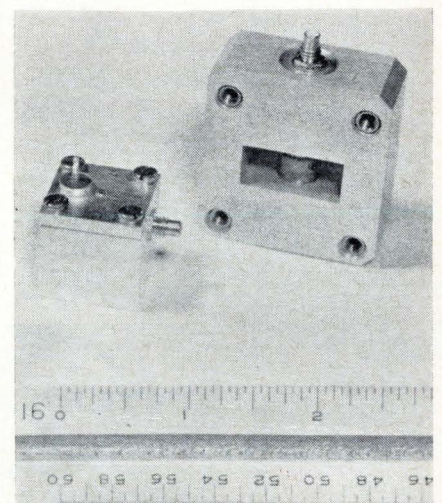
Shhh. Oscillator fits in low-power radar.
