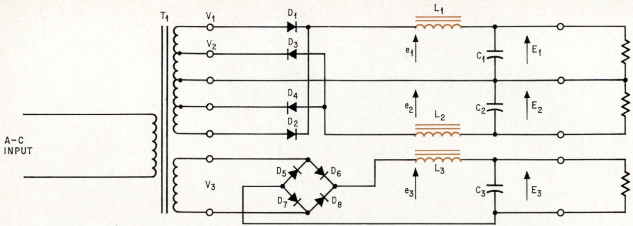
Power supply. Rectified outputs e_1 through e_3 are filtered by individual choke-input filters L_1 - C_1 through L_3 - C_3 . Essentially pure d-c voltages, E_1 through E_3 , are present at the load.
