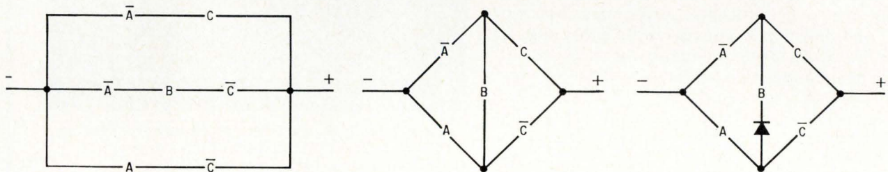
Example 1. Series-parallel configuration (left) is reduced to a bridge circuit arrangement (center). Diode is placed in the shunt leg (right) to keep path ABC open.
