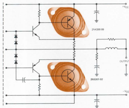
Complementary silicon power-pairs obviate “totem pole” output stages, complex bias adjustments and circuitry.
