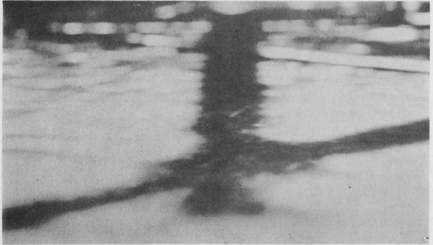
On target. Terminal landing radar for VTOL craft will present the pilot with a head-up display projected from a radar scope. Shown are the runways at Mercer County Airport, Trenton, N.J., as they appear on the scope.
