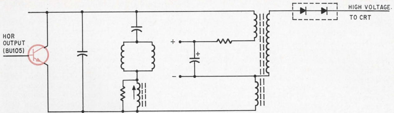
Built-in protection. The output stage can be effectively protected from picture-tube flashovers by a resistor in series with the power supply and primary of the flyback transformer. For circuits using the BU105, a resistance value of 27 ohms is adequate. The resistor should not be decoupled, however.
