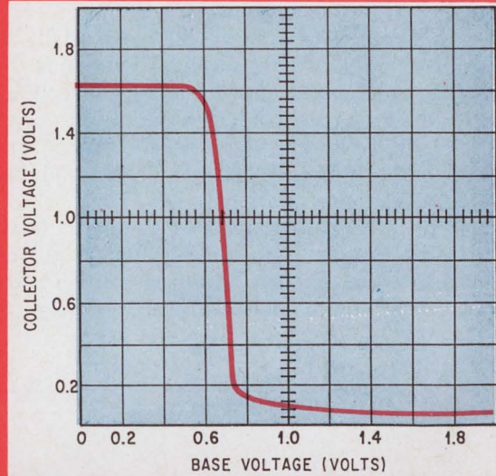
Caught in the act. Input and output signals synchronize the curve tracer into a stable display of the logic circuit's switching.
