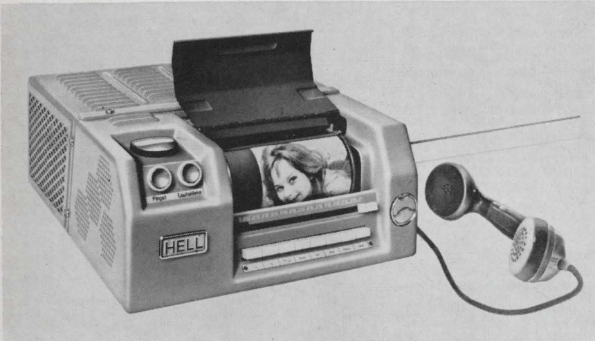
New for newsmen. Portable facsimile transmitter helps press photographers meet deadlines by speeding pictures back to their editors.
