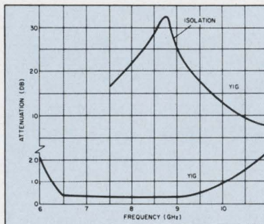
BANDWIDTH CURVE
