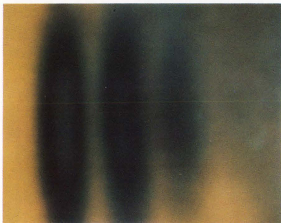
Scattering rod. Polaroid film depicts the electric field scattered by a metal cylinder 17 millimeters in diameter.
