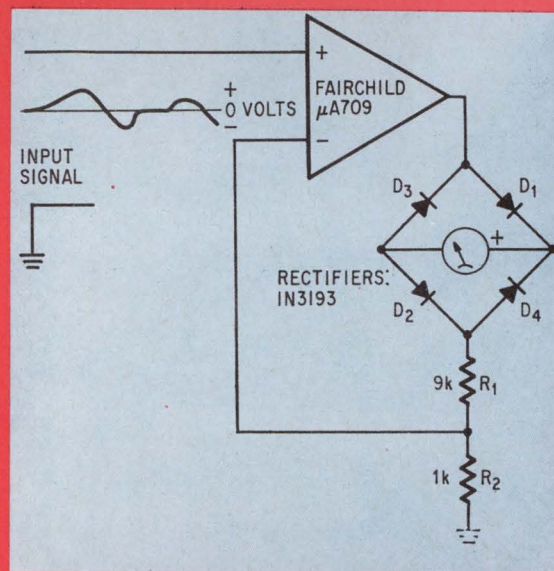
Accurate both ways. Variations in a voltage level are given meter-driving capability by the operational amplifier.
