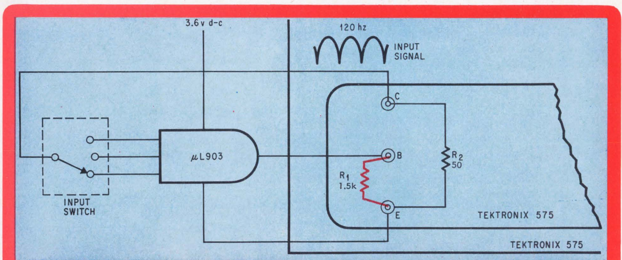
Internal diagnosis. Any flaws in the logic circuit will be displayed on the curve tracer as either high saturation voltage, low cutoff collector voltage, or low gain in the active region. The collector voltage in the integrated circuit appears on the vertical axis of the scope face.
