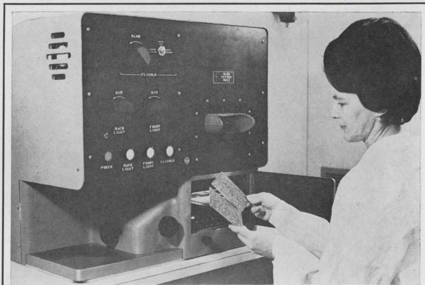
Done with mirrors. RCA's new printed-circuit board tester borrows a technique used by astronomers to chart the movement of stars. Stationary and rotating mirrors superimpose the image of a new board upon the image of a board of known quality; a defect in the new board appears as a flicker. The device can inspect every part of the board—holes, wiring, and components—at each production stage. Used for checking the number and alignment of holes, the prototype has reduced the time for this operation by 50%.
