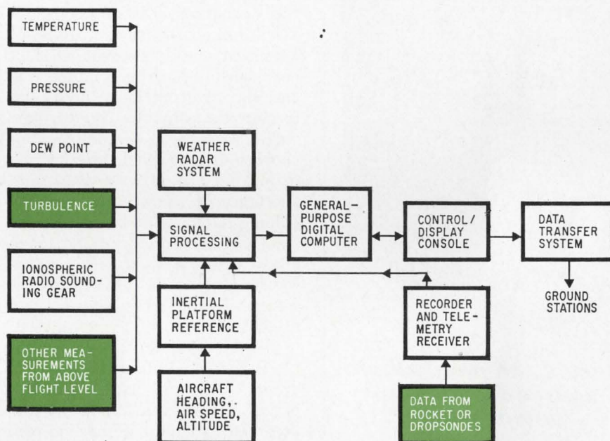
Best guess. Preliminary block diagram of airborne weather reconnaissance system shows potential growth items in color. Improved sensor techniques will permit system to monitor twice as many parameters as present gear.
