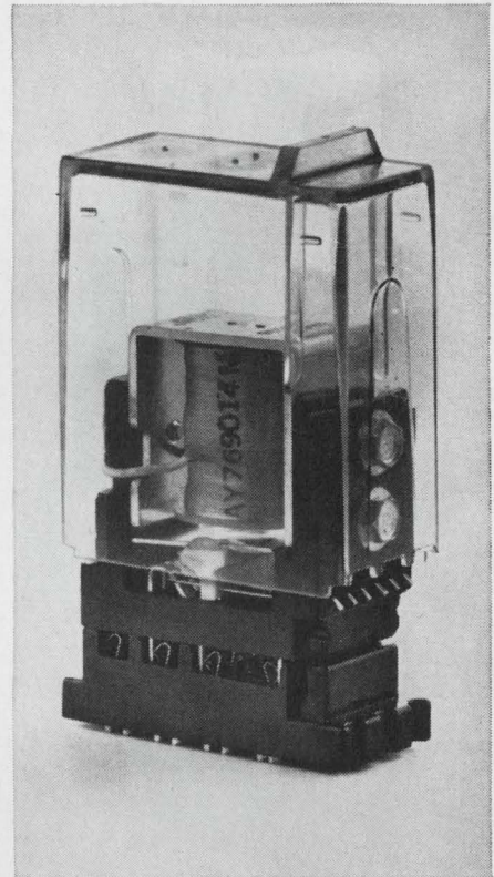
Dust covers are available for various types of IBM wire contact relays. The six-pole model above is shown with cover partially removed.
