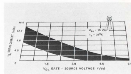
This curve for the 2N5270 illustrates the tight 2-to-1 I_{DSS} ratio offered by the new 2N5265-70 JFET series.
