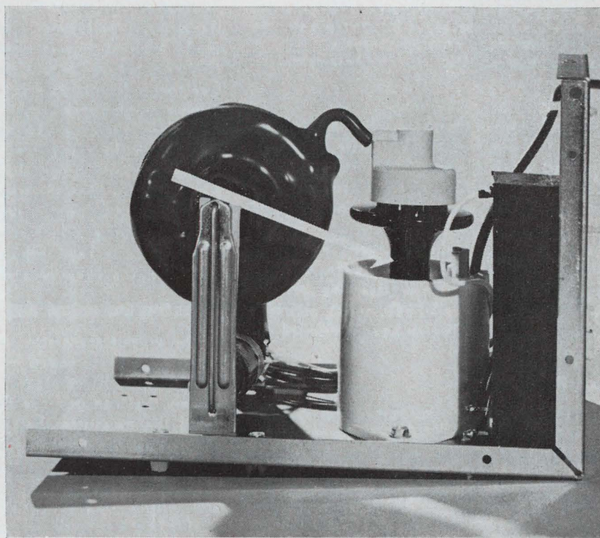
High-voltage module. Motorola's solid state high-voltage module replaces vacuum-tube rectifier with a silicon unit that's shown mounted in position.
