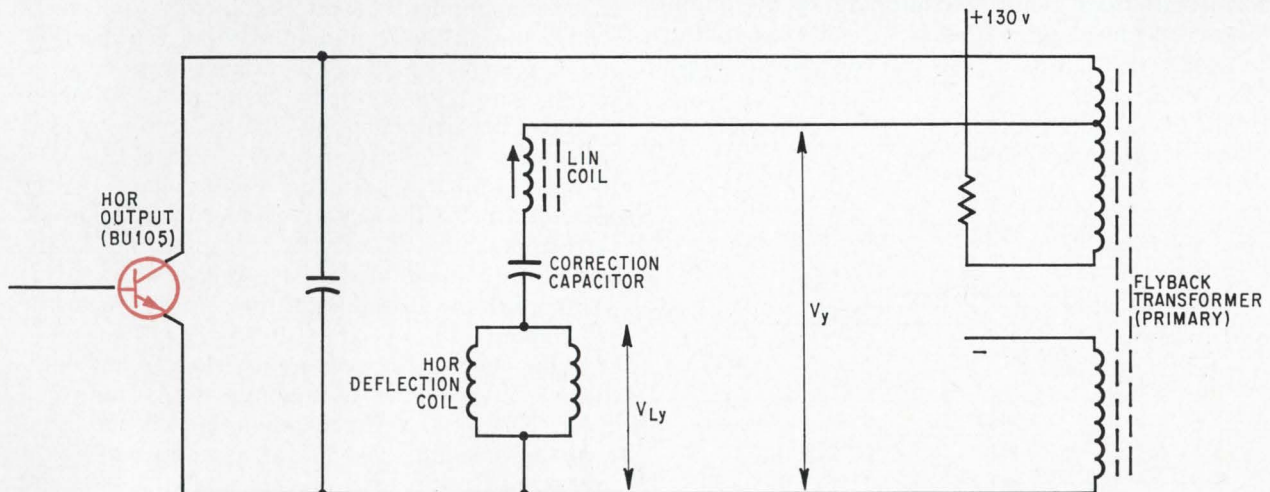
Horizontal output stage. The deflection coil and horizontal linearity correction circuitry are hooked up to a tap on the primary of the flyback transformer. The coil compensates for linearity errors, while the capacitor provides tangent (S) correction. Supply voltage is applied between the primary split terminals.
