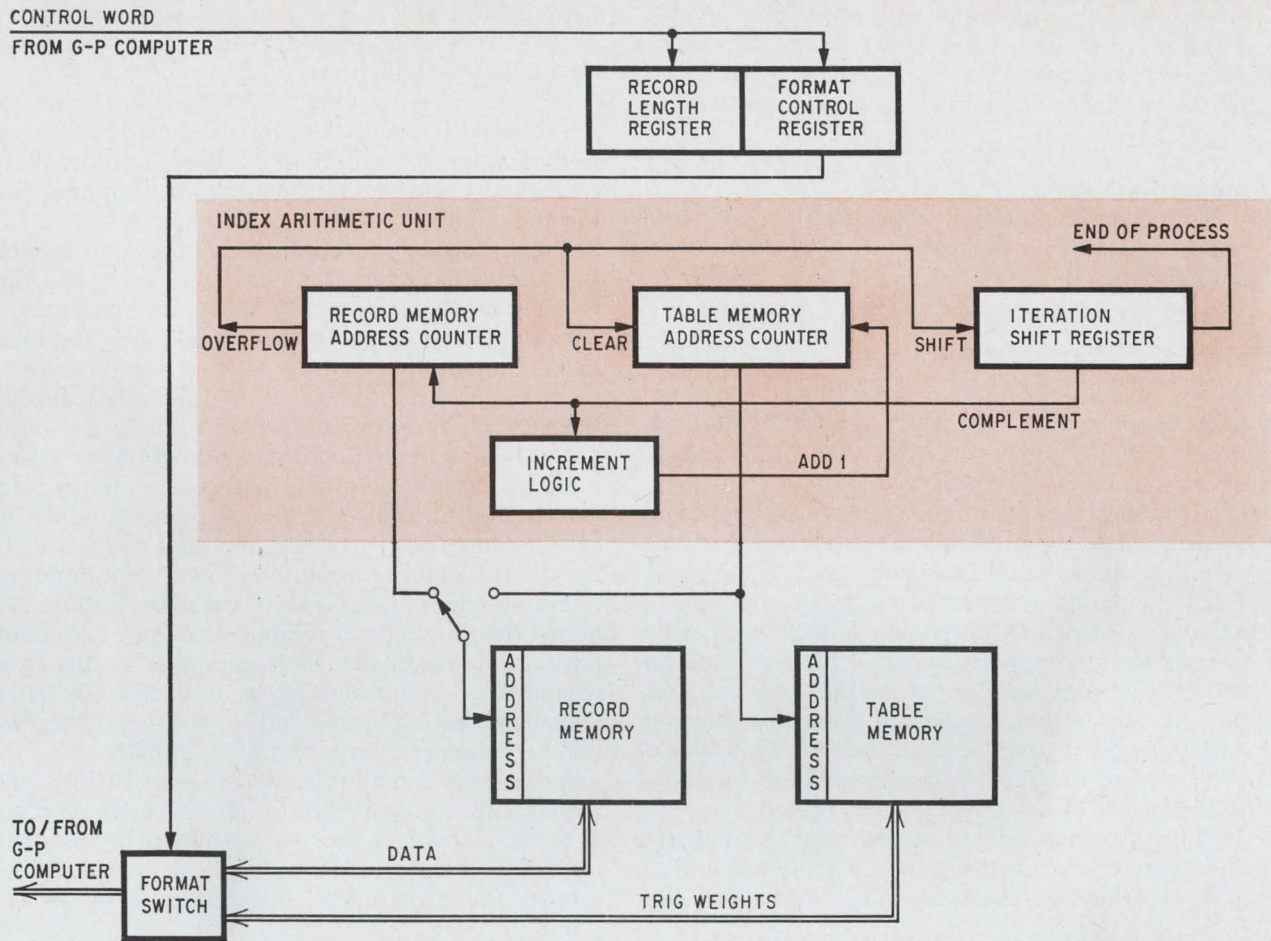
Computational key. Without the indexing unit, which controls the sequence of memory addresses, the fast Fourier transform processor would be much more complicated.
