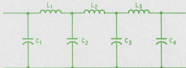
SEVEN-ELEMENT FILTER
