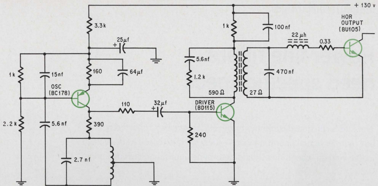
Oscillator and drive stages. The values shown for the circuit components are suited to the transistor types employed in this deflection system. The use of transistors with different characteristics might require some changes in these values, therefore. The oscillator must include provisions for frequency adjustment.
