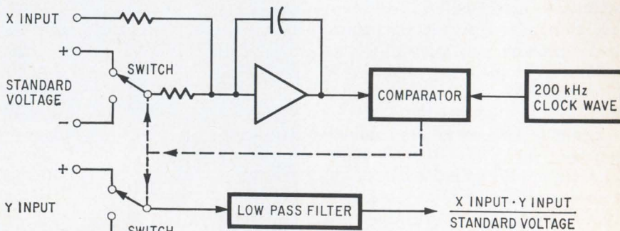
Power is the product. Analog multiplier is the key to the highly accurate power measurements made by Yokogawa's watt converter.
