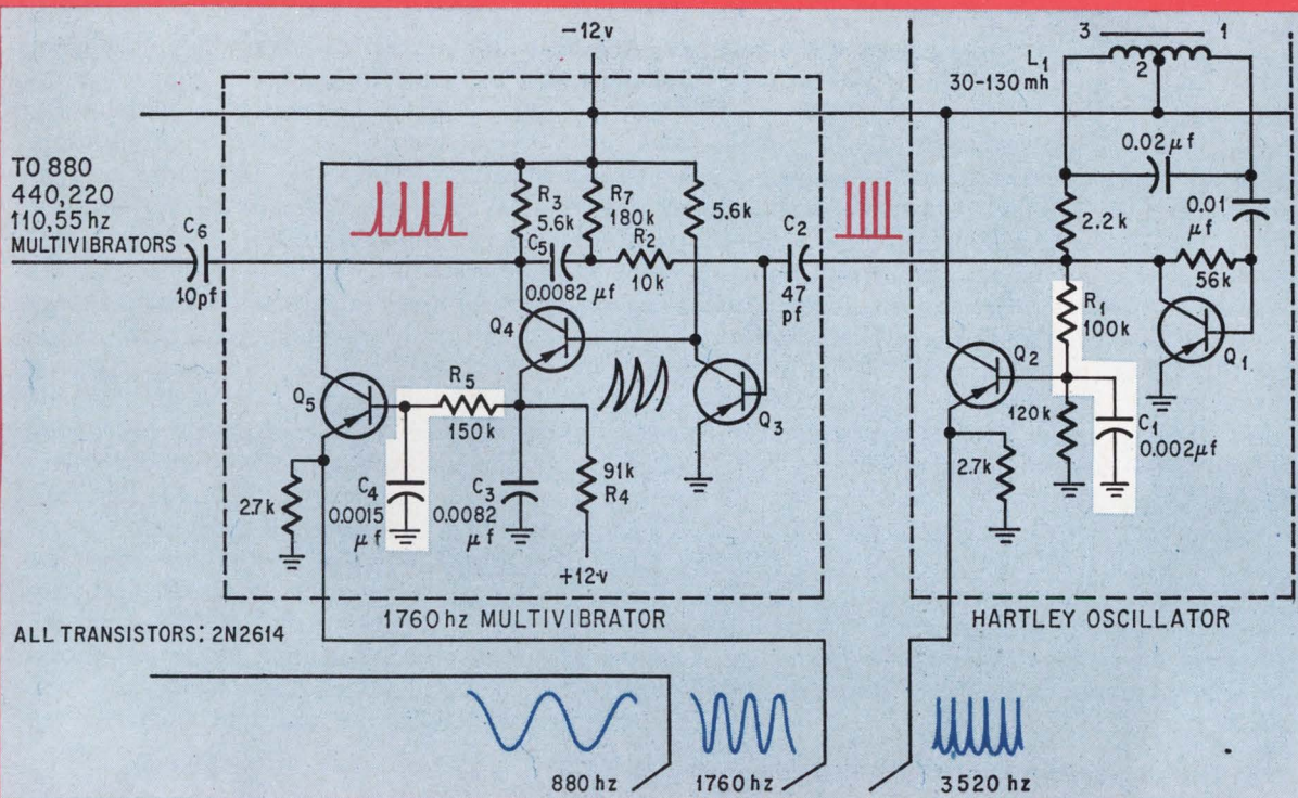
Music maker. The Hartley oscillator generates a very stable audio frequency that is used as both a note for the electronic organ and a synchronizing signal.
