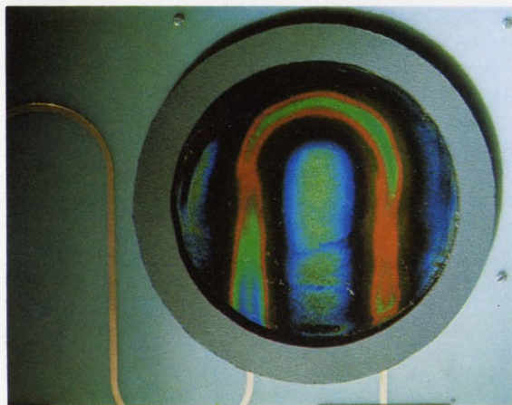
Balancing act. Liquid crystals delineate standing waves along a transmission line. Real-time display enables line's load to be adjusted for proper match. The standing wave smoothes out as the load is balanced.
