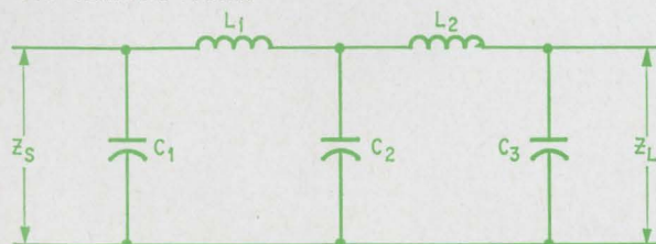
FIVE-ELEMENT FILTER
