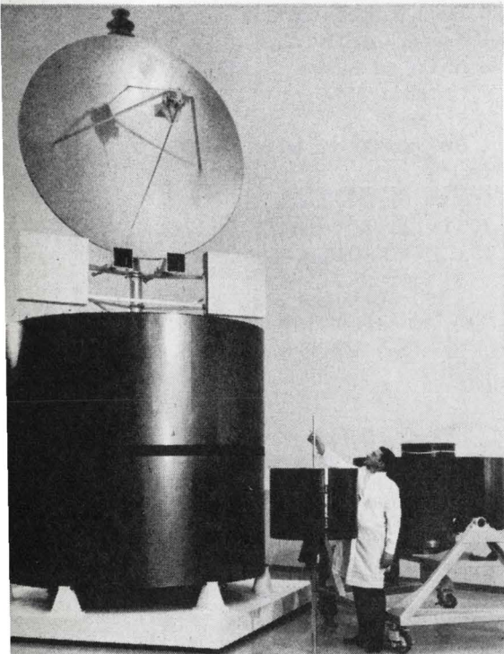
Big brother. Hughes' proposed version of Intelsat 4 towers over Early Bird and Intelsat 2; dish can transmit two spotlight beams to heavy-traffic areas.
