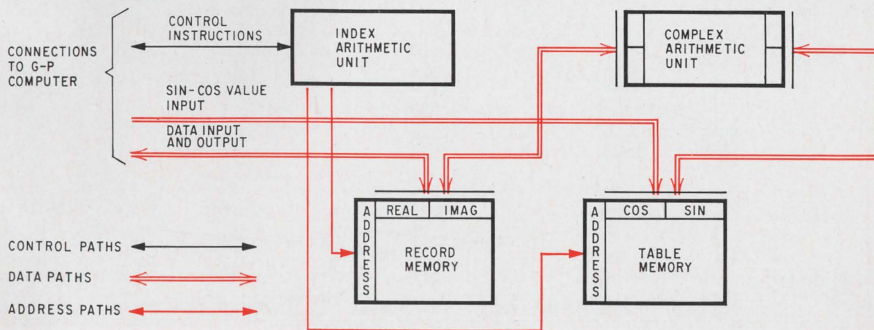
Computer components. Sample records are stored in the record memory, coefficients in the table memory. Indexing unit generates memory addresses, and the arithmetic unit computes the coefficients.
