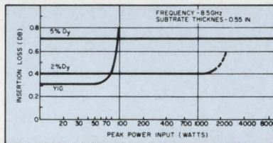
POWER CURVE
