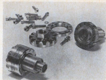
Cleanup. The 404 can be taken apart for cleaning. No recalibration is needed.
