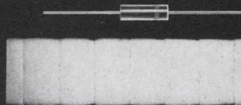
Enlargement of “Ministac” with solid internal construction using high temperature bond
