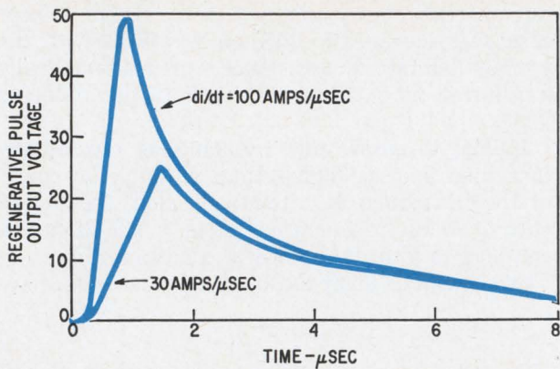
Output. The regenerative pulse output is a voltage spike that hits its peak in 2 μsec.
