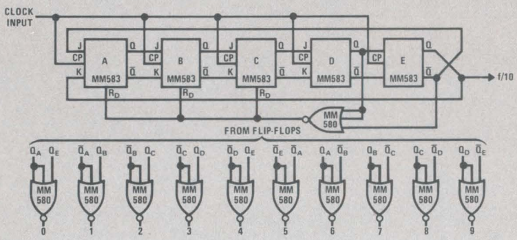
FIGURE 3. Counter/Decoder
