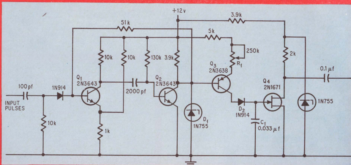
Dividing. Input pulses trigger a multivibrator whose output charges a capacitor. When the charge reaches a preset level, unijunction Q_4 is triggered, producing one pulse. The number of pulses from the multivibrator needed to charge C_1 is determined by the setting of R_1 , a 10-turn potentiometer.
