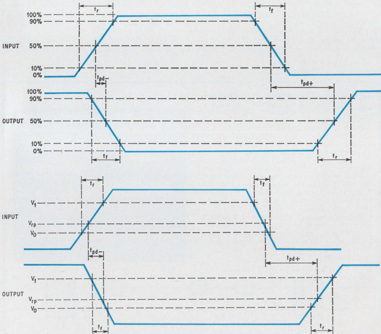
Two ways. Propagation delay can be defined in terms of percentages (top) or voltage levels (bottom).
