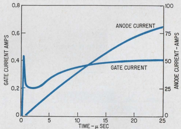
Slow ascent. Gate current remains positive with a slow-rising anode current, and device is kept under control.
