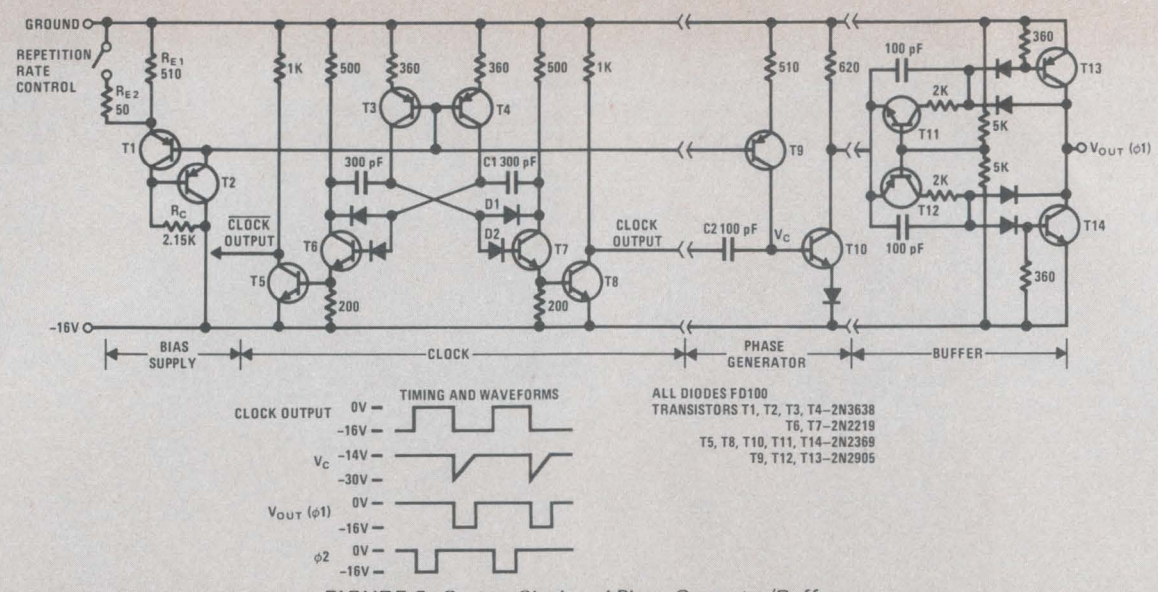
FIGURE 2. System Clock and Phase Generator/Buffer
