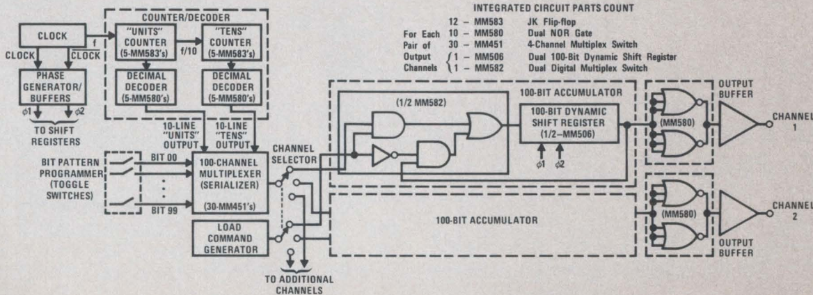
FIGURE 1. Programmable MOS 100-Bit Word Generator
