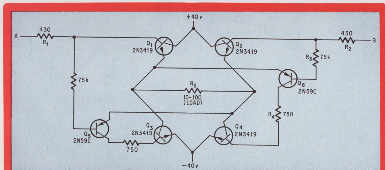
Amplifier with class. Bridge amplifier, which operates class B, is used when isolation is needed between the input and output. When point A is positive with respect to point B, Q_1 turns on, and Q_6 turns on Q_4 . When B is positive, Q_2 conducts, and Q_5 is turned on by Q_5 . The amplifier isn't dependent on the load resistance.
