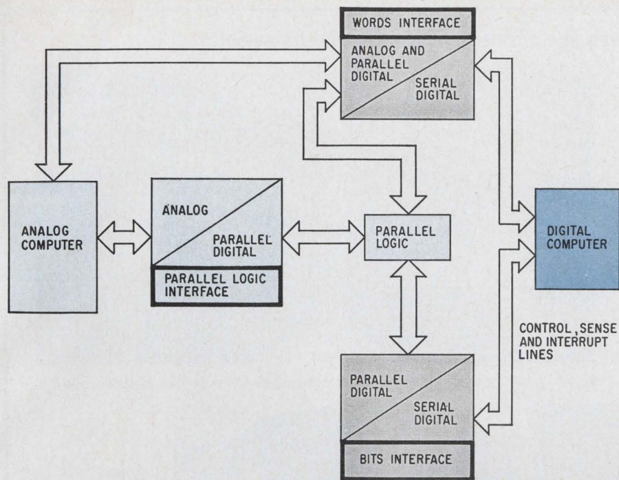
Traffic managers. Interface equipment and cables keep bits and words moving between the analog and digital computers.
