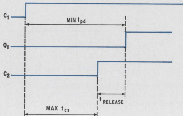
Askew. The time separation between clock edges at two adjacent flip-flops should not be greater than the propagation delay minus the release time.
