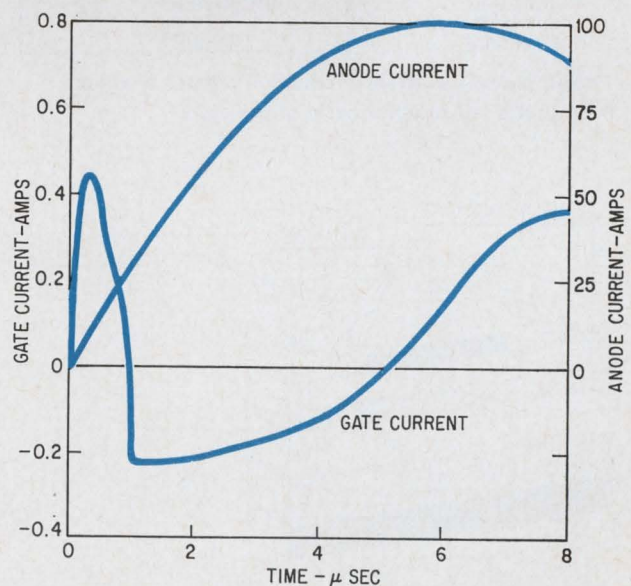
Fast climb. A fast-rising anode current causes negative gate current after about 1 \mu\text{sec} , slowing conduction.
