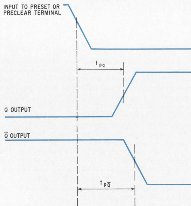
Preset and preclear. The propagation delays from PS to Q, PS to \bar{Q} , PC to Q, and PC to \bar{Q} are measured independently.
