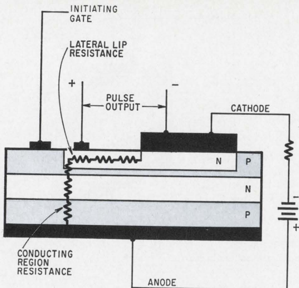
Lossy path. Conduction follows lateral lip resistance before passing down through the chip.
