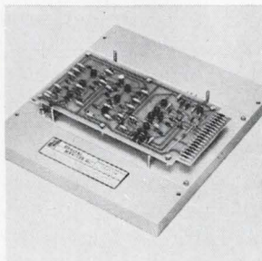
Magnetostriuctive delay line 613E-1015 has a storage capacity of 30,000 bits. Cost per bit is around one cent, in small quantities. The unit provides a 15,000 \mu sec delay and a 2 Mhz data rate over the temperature range 60° to 90°F. Applications include crt displays, digital tv displays, and communications terminals. Digital Devices, 200 Michael Drive, Syosset, N.Y. 11791. [425]
