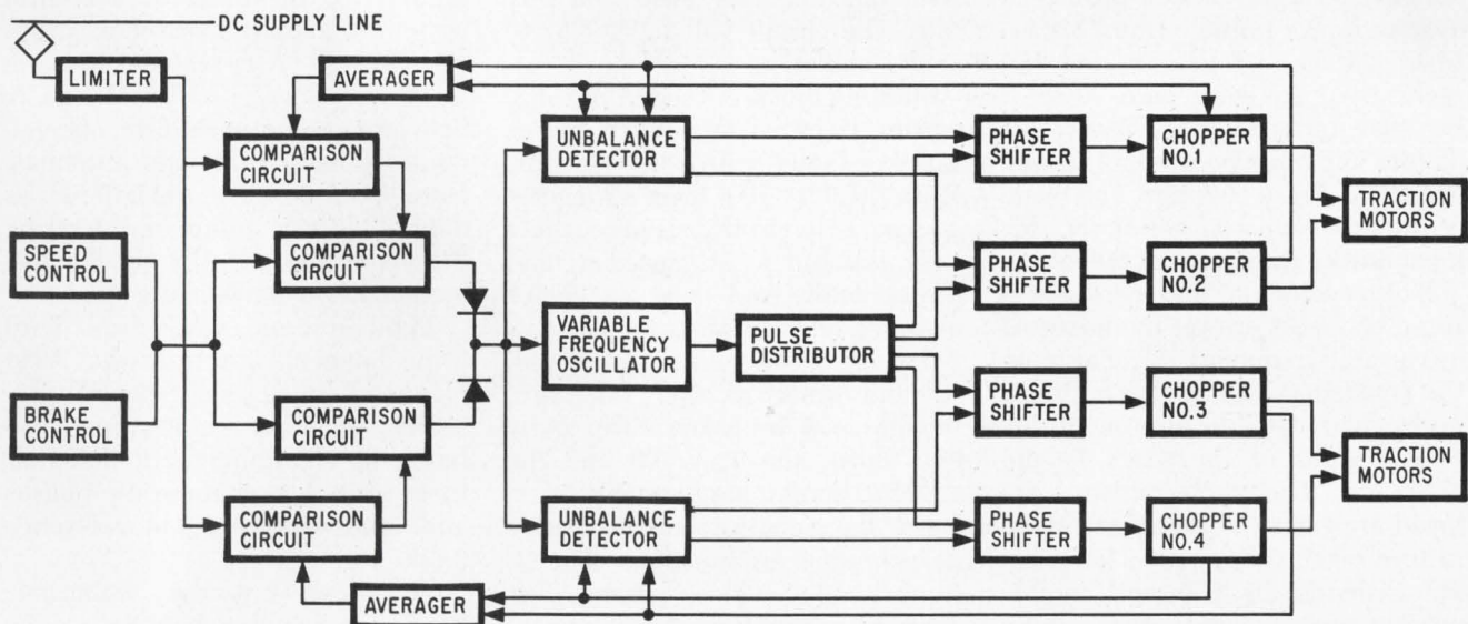
Stepping out. Continuously variable duty cycle of choppers controls speed and regenerative braking of prototype subway cars. Turn-on pulses pass through phase shifter and thus become turn-off pulses too.
