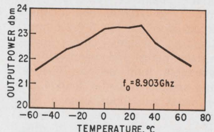
Summit. Power of the Hughes 44010H peaks at room temperature and falls off at high and low readings.
