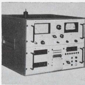
Particle analyzer/counter/printer CI-201/207 features an elliptical mirror optical sensor to detect airborne particles by the "forward light-scattering" technique. It counts, displays, and records airborne particle concentration in two size ranges (normally 0.5 micron and larger, and 5 microns and larger). Climet Instruments Inc., Birchwood Dr., Sunnyvale, Calif. 94086. [361]
