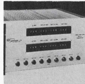
High-speed digital comparators series 6000 are for component sorting applications. They feature go-no/go decisions as short as 10 \mu sec, providing both visual front panel indications and contact closures, for direct interface with BCD instruments. They come in 3 basic configurations: 3-, 4-, and 9-decision models. Micro Instrument Co., 12901 Crenshaw Blvd., Hawthorne, Calif. [368]
