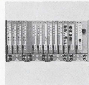
PCM wideband data terminal B313 provides accurate high speed data (0 to 256 kilobits per sec) and voice transmission over exchange type telephone cables at less cost than conventional microwave or frequency division multiplex systems. It transmits signals from digital computers and other data processing equipment. Lynch Communication Systems, 695 Bryant St., San Francisco. [428]
