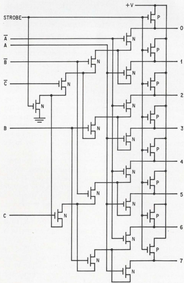
Decoder. Complementary pair at output can generate larger currents to charge circuit capacitance, thus can operate faster than single-channel circuit.
