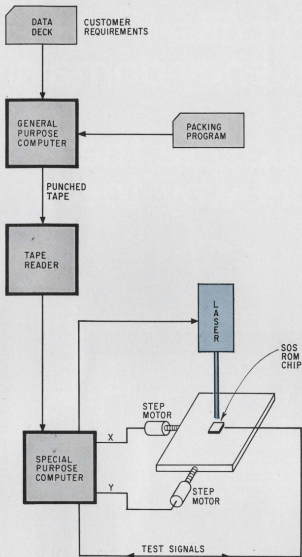
Zap machine. A laser machine tool encodes data in diode array by burning out unwanted connections.
