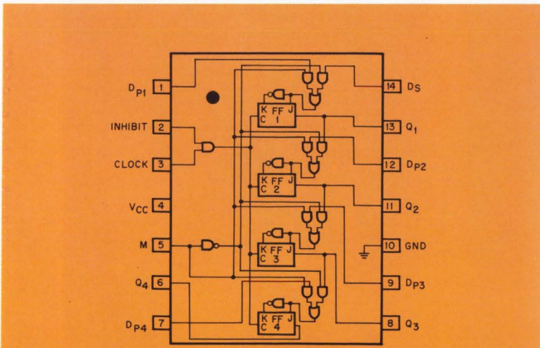
Fig. 1. Logic diagram of SM-110 4-bit shift register.
