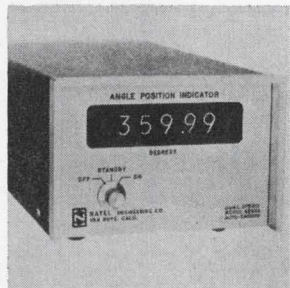
Dual-speed, automatic-ranging angle position indicator model 4062A can handle 1:36 and 1:10 two-speed synchro inputs. It offers several automatic features including 60 and 400 hz operation, 26 v and 115 v reference (rotor) amplitudes, and 11.8, 90, or 115 v rms line to line stator voltages, all available in one package. Natel Engineering Co., 7129 Gerald Ave., Van Nuys, Calif. [366]
