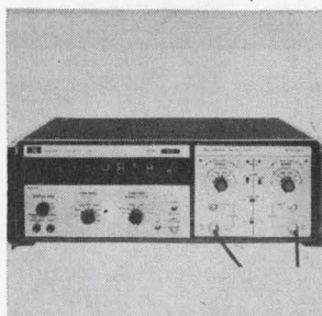
Electronic counter model 1515A has a frequency range of d-c to 70 Mhz and can totalize to 10^9 counts. Frequency ratio is 10^{-6} to 10^6 and sensitivity is 100 mv. Crystal aging rate is 1 part in 10^7 per day. Internal time base output scaled from 0.1 hz to 10 Mhz in decade steps is available at rear panel. Monsanto Electronic Instruments, 620 Passaic Ave., West Caldwell, N.J. [365]
