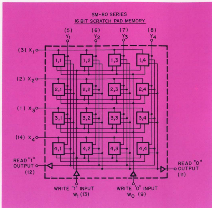
Fig. 1. Logic layout of SM-80 16-bit scratchpad memory.
