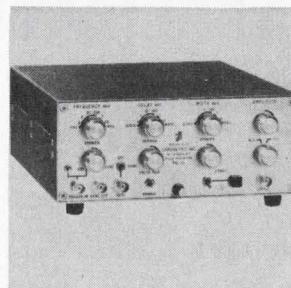
Pulse generator PG-11 provides single or double pulses, pulse pairs, pulse bursts or one-shot output. It operates over a repetition rate range from 10 hz to 20 Mhz in the double pulse mode and to 10 Mhz in the single pulse mode. Rise and fall times are 5 nsec max. at full \pm 15 v output amplitude. Price is $375. Chronetics Inc., 500 Nuber Ave., Mt. Vernon, N. Y. 10550. [367]
