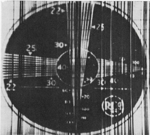
Crude proof. Although resolution and sensitivity are poor, RCA's early efforts with solid state image sensors proved the feasibility of a tubeless television camera.
