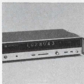
Automatic counter model 5323A has a range of 0.125 hz to 20 Mhz. It can measure the carrier frequencies of pulsed r-f or tone bursts, even those that are but a few microseconds in duration, without the use of a transfer oscillator. The unit is priced at $2,150. Deliveries are scheduled to begin in March. Hewlett-Packard Co., 1501 Page Mill Road, Palo Alto, Calif. [363]
