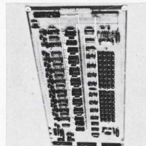
Instant memory system ECOM-S comes on a single 7.50 x 16.70 p-c board. It is for volume applications as a refresh memory for displays, a block buffer in key-to-tape, and as a small memory in process control computers. It operates in either the \frac{1}{2} cycle mode at 2 \mu sec or the full cycle mode at 4 \mu sec. Standard Memories Inc., Ventura Blvd., Sherman Oaks, Calif. [427]
