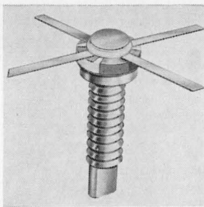
Microwave transistor PT6821 provides 20 w c-w power at 1 Ghz. It has 5 db gain, 55% efficiency operating from a 28-v source. The hermetic devices can be incorporated into microstripline amplifiers for design simplicity and economical construction. Common emitter configuration provides circuit stability. TRW Semiconductors Inc., 14520 Aviation Blvd., Lawndale, Calif. 90260. [438]
