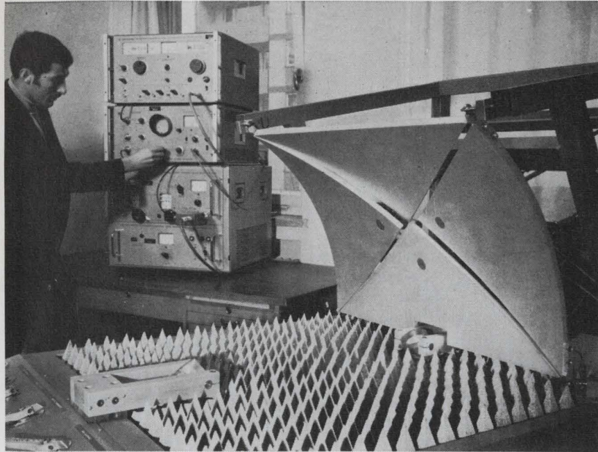
Horning in. Alignment of the four segments of this parabolic mirror can be checked to within 0.3 mm with new West German technique. Horn just below mirror and second one opposite it radiate interference patterns that are picked up by probes (dark spots) on moveable segments.
