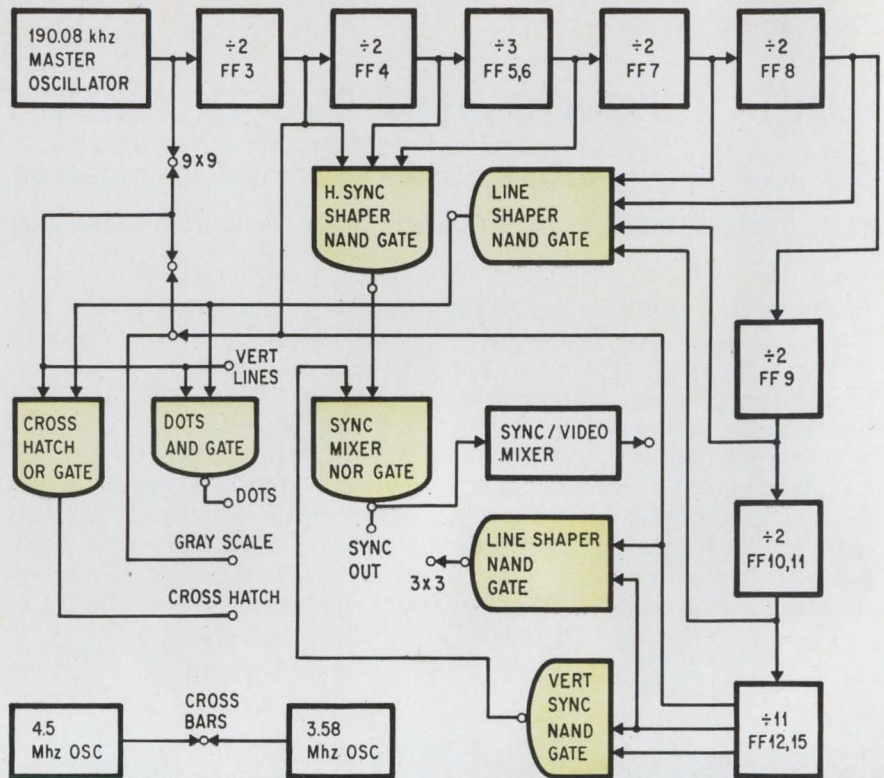
Logic flow. Thirteen test patterns are generated from a crystal-controlled oscillator countdown with frequencies selected by OR, NOR, AND and NAND gates, above, in Heath's IG-28 color-bar and dot generator, at right.
