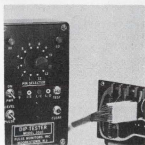
DIP tester 2010 can check dual-in-line IC's without removing them from their circuit boards. Using an integrated circuit clip, the unit selects an active pin and a red or green light indicates the level or polarity of pulses at that point. The tester obtains its nominal 5 v, 75 ma power directly from the power leads of the DIP under test. Pulse Monitors Inc., Moorestown, N.J. [362]
