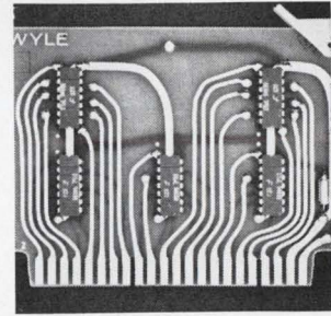
RS flip-flop card MSF-10 provides a ten set-reset or storage capability. Designed for many storage and general-purpose logic applications, the card provides for frequency, d-c to 5 Mhz, and input loading of one unit load each input. Output drive capability is 7 unit loads, and power required is +5 \pm 0.5 v at 75 ma, max. Wyle Laboratories, 128 Maryland St., El Segundo, Calif. [424]
