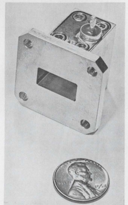
Powerpoint. Diode atop waveguide is source for Varian's Ku-band oscillator.
