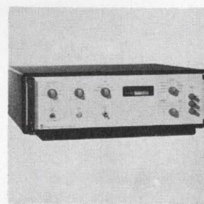
Digital voltmeter calibrator type 1822 checks out a DVM by stepping it through a programmed test sequence. It checks whether DVM readings are affected by circuit loading, by a-c superimposed on the measured d-c signal, and by common-mode a-c or d-c signals. Price is $2,800 for the bench model; $2,775 for the rack mounting unit. General Radio Co., West Concord, Mass. 01781. [364]
