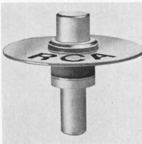
Silicon overlay transistor TA7403 is for power oscillator applications in receivers and power sources that operate in the L- and S-band ranges. A typical unit operated at 21 v can provide 0.6 w of power at 2 Ghz with 25% efficiency; and provide 100 mw at 3 Ghz. Production quantities will be available after April. RCA/Electronic Components, 415 S. 5th St., Harrison, N.J. [442]
