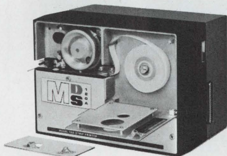
With cover panels removed, the miniaturization of the mini-baby can easily be seen.
