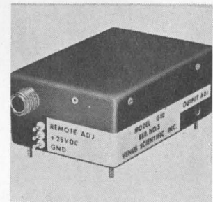
Crt power supply G10 is less than 15 cu. in. in volume and weighs 1 1/4 lbs. A screwdriver adjustment allows the output voltage to be set at any value between 8,500 and 10,500 v d-c. Both line and load regulation are \pm 0.1\% . Output ripple is 0.15% peak-to-peak at full load (500 \mu\text{a} ) and less than 0.1% at 350 \mu\text{a} . Venus Scientific Inc., 399 Smith St., Farmingdale, N.Y. [384]
