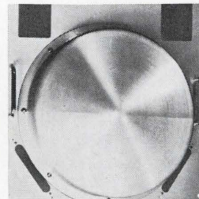
Ten-inch rotating drum memory system CLC-1 can store up to 1.2 million bits of data and has an average access time of 8.5 msec. It features four multiple pole-piece head assemblies, each containing eight write/read heads on 32 data tracks, operating at 3,600 rpm. The drum unit comes complete with digital interface. Bryant Computer Products, Ladd Road, Walled Lake, Mich. [426]
