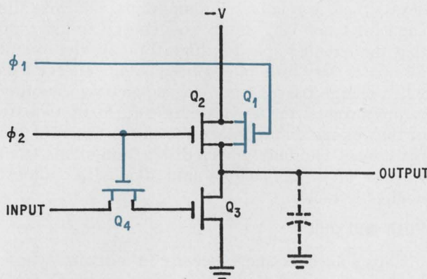
Precharge. Two alternating clock pulses set up the stage before its logic state is acquired, for further speed improvement.
