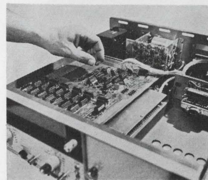
Quick change. Any of the more than 70 IC's in the counter-timer can be replaced without soldering.
