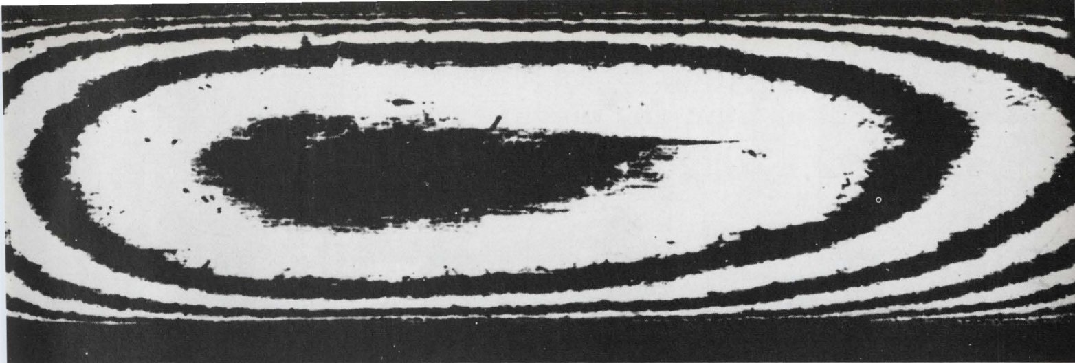
Interference photomicrograph of a gage block surface. Fringes give a clear picture of a surface dropping toward the edges.
