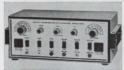
Logic flow. Thirteen test patterns are generated from a crystal-controlled oscillator countdown with frequencies selected by OR, NOR, AND and NAND gates, above, in Heath's IG-28 color-bar and dot generator, at right.
