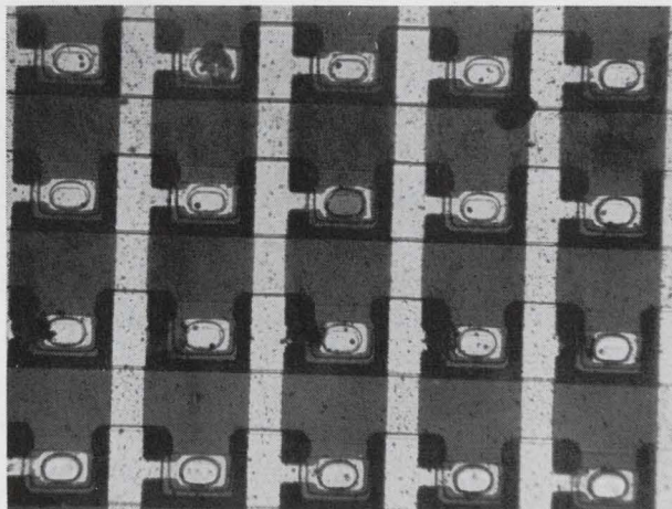
Encoder array. The laser has burned out all the diode connections in one horizontal row, where the light-colored connection is missing.
