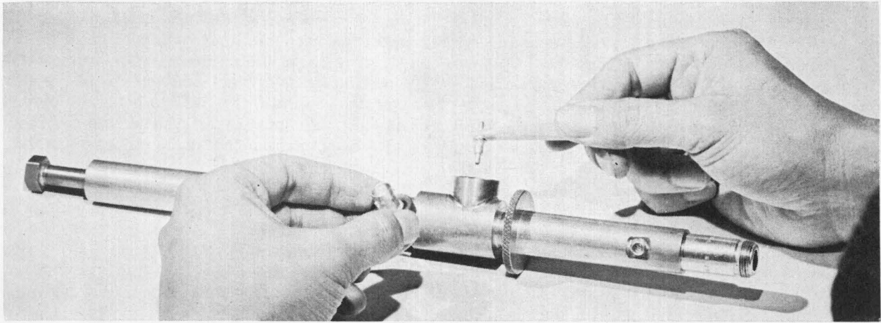
Powerful. RCA's Trapatt, or anomalous mode diode delivers hundreds of watts at 0.1% duty cycle. Here, it's being placed in a tuning circuit.
