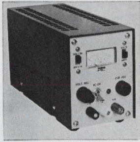
Constant voltage, constant current lab power supply QAD50-1 has 0.01% regulation. It is designed for applications such as computer controlled lab testing requiring programing either up or down at a rate of 10 mv/ \mu sec. Ripple is less than 0.5 mv rms or 2 mv peak-to-peak with excellent stability. Price is $99. Todd Products Corp., 28 Laurel St., Hicksville, N.Y. 11801. [382]
