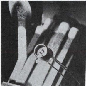
Photo-SCR'S series RTPC0501 are for operation over the military temperature range ( -55^{\circ} to +125^{\circ} C). They feature light sensitivity of 20 footcandles typical without need for a focusing lens. Five types are offered with peak off-state voltages ranging from 15 to 200 v. All handle up to 300 ma of d-c current. Transitor Electronic Corp., 168 Albion St., Wakefield, Mass. [436]
