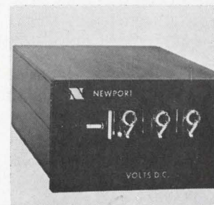
Digital panel meters 200, 210, 220 and 230 measure d-c voltage, d-c current, a-c voltage and a-c current, respectively, with full-scale display of 1,999 counts. Currents are measured from 1 na to 200 ma, and voltages from 10 \mu v to 200 v. Thirty-one different models and 13 options permit a variety of applications. Newport Laboratories Inc., 630 E. Young St., Santa Ana, Calif. [368]
