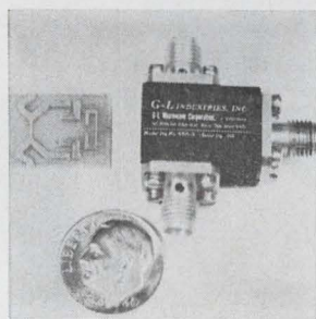
Ultraminiature balanced mixer model MI8010-5 covers a frequency range of 8.4 to 9.7 Ghz. Noise figure is 7.5 db max. Vswr is 1.75 max. Local oscillator-signal isolation is 15 db minimum. Package measures 1/2 x 3/4 x 1/2 inch. Price in 1-9 lots is $250 each. Delivery of prototypes is 2-3 weeks. G-L Microwave Corp., 825 Black Oak Ridge Rd., Wayne, N.J. 07470. [402]
