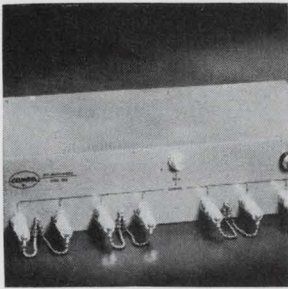
Antenna couplers series CRM-108 are for coupling the signal from one antenna to one to eight receiver outputs. The solid state devices feature a constant gain of 4 db with a \pm 1 db frequency deviation over the entire operating range of 1.5 to 50 Mhz. Maximum noise figure is 6 db; typical dynamic range 130 db. Price is $2,125. Comdel Inc., Beverly Airport, Beverly, Mass. 01915. [381]
