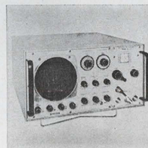
Microwave spectrum analyzer model SPA-100 offers full 100 Mhz dispersion throughout its 10 Mhz to 40 Ghz range. It has built-in i-f marker for self-calibration, and provides calibrated 60-db on-screen log display with 1 Mhz bandwidth for maximum dynamic range. Singer Co., 915 Pembroke range. Price is in the $6,000 range. Singer Co., 915 Pembroke St., Bridgeport, Conn. [404]
