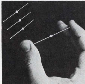
Microminiature, 3-amp, fast recovery rectifiers, designated types 1N5185, -6, -7, and -8, are available in peak reverse working voltages of 50, 100, 200, and 400 v. Features include reverse current of less than 5 \mu a and recovery time of less than 300 nsec. Price is $2.50 each at the 999 piece order level. Centralab Semiconductor, 4501 North Arden Dr., El Monte, Calif. 91734. [440]
