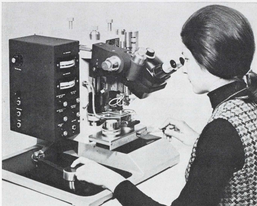
Leading off. Automatic bonders for beam-lead circuits, like this one from Kulicke & Soffa, are just now becoming commercially available.
