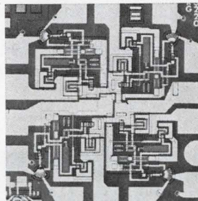
Transistor-transistor-logic IC's known as RAYIII come in 19 basic circuit types including NAND gates, AND gates, AND-OR-INVERT gates, a hex inverter, and single and dual flip-flops. Maximum propagation delay for NAND gates is 5.5 nsec and power dissipation is typically 22 mw per gate. Logic levels are typically 3.5 and 0.3 v. Raytheon Co., 350 Ellis St., Mtn. View, Calif. [442]
