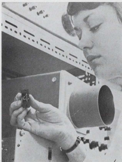
Number's up. Gallium phosphide diodes in SERL array glow with a brightness of 500 foot-lamberts. The array measures \frac{1}{2} by \frac{3}{4} inch.
