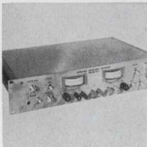
Inverter model MT-1 is for testing and evaluation of fractional h-p, instrumentation motors, and has provisions for driving center-tapped or full winding motor loads. By taking the product of the two front panel meter readings, the a-c power delivered to the load is given without requiring the usual corrections for power factor. Kintron Co., 29 S. Pasadena Ave., Pasadena, Calif. [385]
