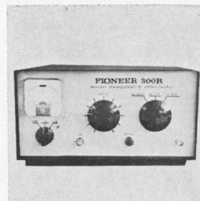
Secondary frequency standard 300R can be used in the receive mode for calibrating oscillators directly without the use of an oscilloscope or other indicating device. Stability is 0.005% (5 hz at 10 khz, 0.01 hz at 200 hz). A switch selects up to 3 standard frequencies. Price is $169.50; availability, 4 weeks. Pioneer Electronics, 738 Pacific St., San Luis Obispo, Calif. [367]
