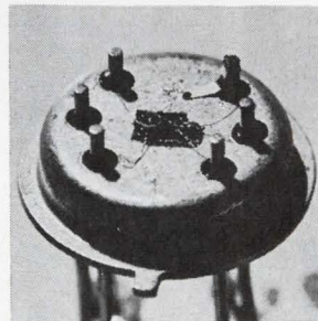
Optically coupled isolators XL102 and 103 can replace low-power relays and transformers. They provide electrical isolation of \pm 100 v, internal resistance greater than 10^{12} ohms, and a capacitance of 4 pf, all enhancing signal-to-noise performance. Typical over-all current gains are 0.6 for the 102 and 1.4 for the 103. Texas Instruments, P.O. Box 5012, Dallas 75222. [441]
