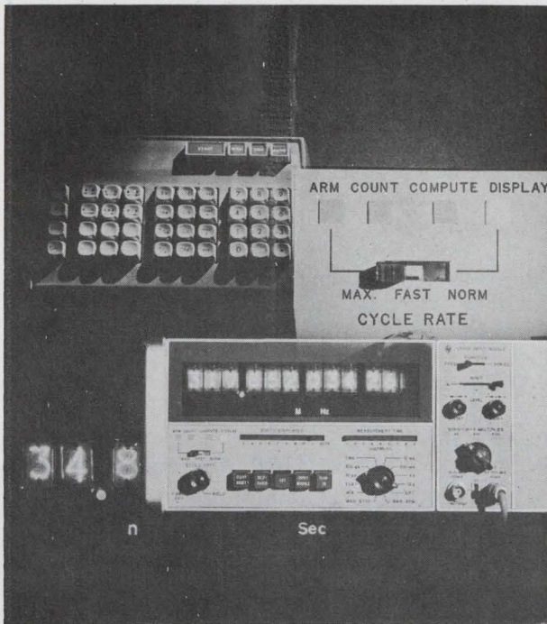
It counts; it figures. Hewlett-Packard's newest entrant in the counter timer race is the 5360A which, is both a fast and accurate counter and a calculator.
