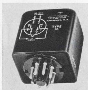
A-c null sensing relays combine solid state input circuitry with dry reed load contacts. The hybrid modules can often replace more complicated, costly components commonly used for transducer sensing, servo positioning, or sensing and regulating motion displacement in control systems. Price (1-24) is from $21.75. Sensitak Instrument Corp., 531 Front St., Manchester, N.H. [347]
