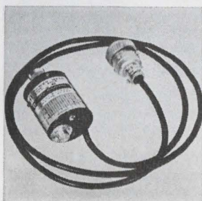
Coaxial, thin-film thermoelectric power heads models N420C, -21C, -22C and -23 operate from 2 Mhz to 12.4 Ghz. Vswr is a maximum of 1.5 over the entire operating range. They can be used with all the manufacturer's power meters. Each meter is capable of direct-reading power measurements from 30 nw to 3 w. General Microwave Corp., 155 Marine St., Farmingdale, N.Y. [405]
