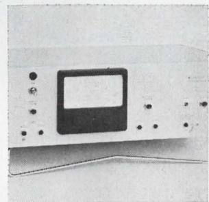
Transmission test set model 9271 checks telephone lines that will be used for digital transmissions or for facsimile work. It also tests and aligns equalizers. Group delay errors and circuit noise effects on the test signal are measured as the reduction in peak-to-average ratio of the received test signal. Wiltron Co., 930 East Meadow Drive, Palo Alto, Calif. 94303. [364]
