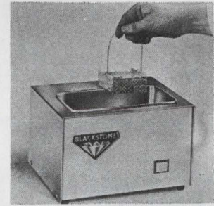
Portable ultrasonic cleaner model SP-100 measures 10 5/8 x 8 1/2 x 6 3/4 in. and incorporates a stainless steel tank with a capacity of 1 3/8 quarts. Its 100-watt average output results in high intensity uniform action and efficient cleaning in the removal of grease or contaminants. The unit's only control is an off-on switch. Blackstone Ultrasonics Inc., Sheffield, Pa. 16347. [424]
