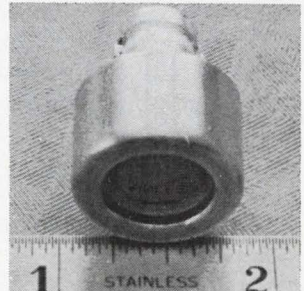
Silicon Schottky barrier photo-diodes models QD80, -80A, -20, and -20A are for near infrared applications. Key features include: highest detectivity at 0.85 \mu of 9 \times 10^{12} cm hz ^{1/2} /w; fast rise-times of 5 \times 10^{-9} sec; active diameters up to 10 mm; dark currents as low as 5 \times 10^{-7} amps. Prices range from $30 to $95. Nuclear Diodes Inc., P.O. Box 135, Prairie View, Ill. 60069. [443]
