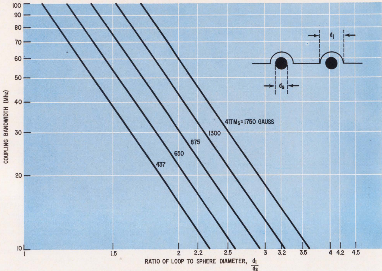
Semiloop coupling. The coupling-loop diameter depends on the coupling bandwidth and saturation magnetization.
