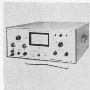
A-c/d-c transfer standard model ATS converts rms to d-c at 0.01% accuracy in 15 seconds. It converts a d-c digital voltmeter, potentiometer, or any d-c measuring system to a true rms measuring system. Its rated accuracy covers the range of 0.25 to 1,000 v and 5 khz to 20 khz. Price is $3,500; availability, from stock. Singer Co., 915 Pembroke St., Bridgeport, Conn. 06608. [366]
