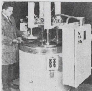
Free-abrasive machinery tool is for semiautomatic controlled-temperature polishing of memory disks used in the computer field. Designed to polish 4 disks simultaneously, the machine features automatic timing, a vacuum system that holds the memory disk to the chuck, and a continuously rotating polishing wheel. Speed-Fam Corp., 509 N. Third Ave., Des Plaines, Ill. 60016. [425]
