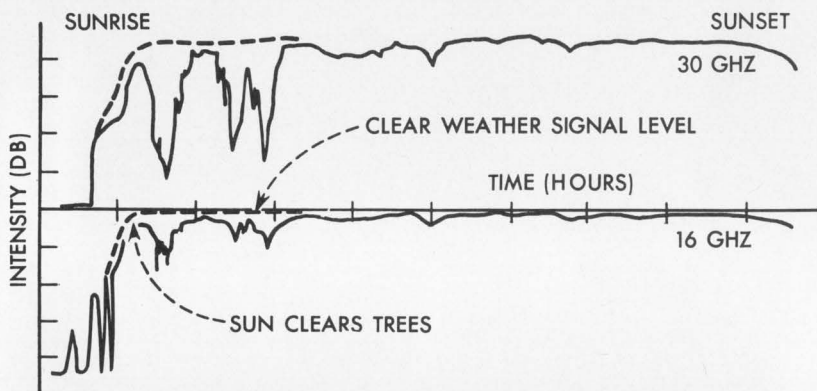
Intensity of solar radiation at two frequencies, recently observed at Bell Laboratories' installation at Holmdel, N. J. Graphs show one 9-hour period out of months of study. Note attenuation due to rain early in the day.
