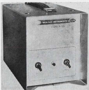
Scope pack model P-TEK improves the performance of oscilloscopes and crt devices. It provides 50 db filtering to 1 Mhz and 0.25% regulation. Scope problems such as pretriggering, jumping off scale, false signals, jitter, and erroneous readings caused by line disturbances are virtually eliminated. Price is $325. Wanlass Instruments, 1540 E. Edinger Ave., Santa Ana, Calif. [361]
