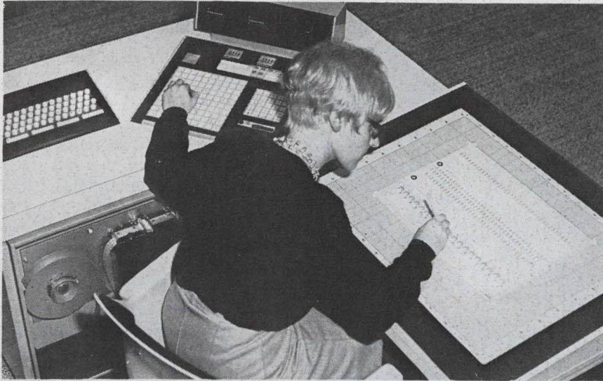
Quick on the draw. Telefunken's graphics-input terminal converts sketches to digital data that a computer can process. An ordinary ballpoint pen or sharp pencil will work on the 18-by-24-inch input pad.
