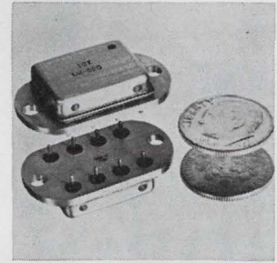
Voltage regulator model LM500 has a peak input voltage of 40 v and peak current of 4 amps. Load regulation with an input voltage of 12 v is typically better than 0.01% from no load to 3 amps full load. Dimensions are 1.2 x 0.65 x 0.25 in. Price for quantities of 100 to 999 is $49 each. International Circuit Technology Corp., 18225 Euclid St., Fountain Valley, Calif. [384]
