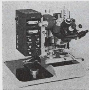
Semiconductor output is boosted by precision beam lead bonder model 573. Bonding is achieved by a thermocompression wobble tool and is readily adaptable to semi-automatic setups. A reflex optical system gives the operator a clear view of the device pattern superimposed directly on the workpiece pattern. Kulicke and Soffa Industries Inc., Fort Washington, Pa. 19034. [427]
