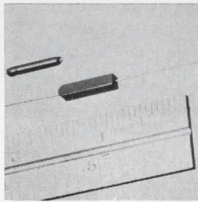
High-voltage, fast recovery, silicon rectifiers series FR are hermetically sealed devices that have a recovery time of 300 nsec and are rated at 3 ma continuous current at voltages from 7,500 to 50,000 v. They are for voltage multiplier assemblies, crt and electrostatic power supply use. Atlantic Semiconductor, Div. of Aerological Research, Mattison Ave., Asbury Park, N.J. 07712. [438]
