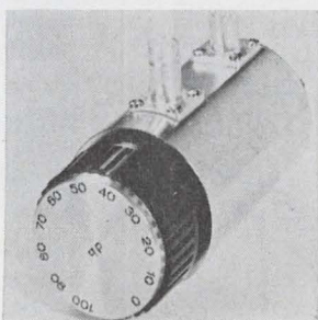
Rotary attenuator RA-100 covers 0 to 100 db in 10-db steps. It covers the frequency range of d-c to 1.2 Ghz with a 1.2:1 maximum vswr at 1 Ghz, with impedance of 50 ohms. The unit measures 1 7/8 x 2 1/8 in. Connectors available include the BNC, TNC, type N and STM. Price is $140 each with delivery in 2 weeks. Texscan Corp., 2446 Shadeland Ave., Indianapolis 46219. [406]
