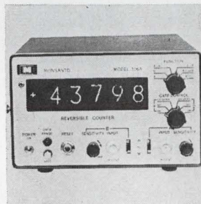
Reversible 2-channel counter model 106A has a 5 hz to 5 Mhz counting rate for each channel. Versatility is provided by the rapid counting rate, combined with averaging capability as well as measuring sum and differences. The unit measures 4\frac{1}{4} \times 7\frac{1}{2} \times 9 in., weighs 5.6 lbs. Price is $895; delivery, 4 weeks. Monsanto Electronic Instruments, 620 Passaic Ave., West Caldwell, N.J. [363]
