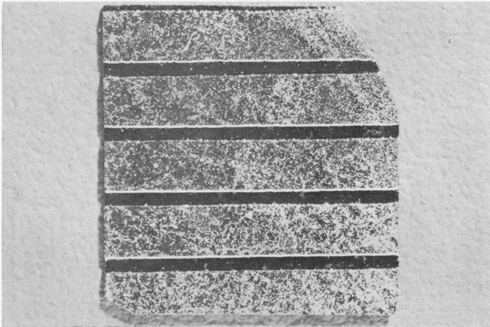
Etching. Black stripes are semi-insulating substrate, showing through where p-type material (gray) has been etched away to isolate the columns in a memory array about \frac{1}{4} -inch square. Continuous gray material connects the anodes of a column of diodes. The bottom photograph shows the reverse side of a \frac{1}{2} -by-1 inch wafer that, except for size, is similar to the one above. Each white dot is a spot of n-type material. A memory array would be made from this wafer by evaporating a thin-film resistor beside each dot, then connecting the resistors in rows perpendicular to the columns, as shown on page 116.
