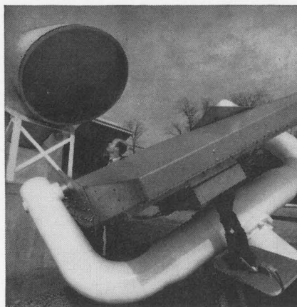
Bell Laboratories' station for studying atmospheric effects on solar radio energy. The flat mirror has two axes. One is parallel to the earth's polar axis—for daily rotation. The other is perpendicular—for seasonal variation. Experiment designer R. W. Wilson checks the horn antenna into which signals are reflected.
