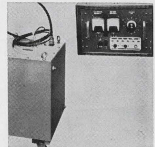
High-voltage d-c power supplies series H come in 55 models with voltmeter and ammeter hand calibrated to \pm 2\% . Units have voltage outputs up to 250 kv and are air or oil insulated. Other features include a load regulation of 7.5 to 15-25%, and capability of withstanding a continuous ambient temperature range from 0 to 40°C. NJE Corp., 20 Boright Ave., Kenilworth, N.J. [388]
