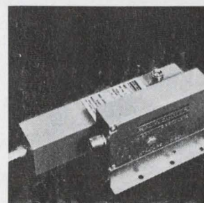
Phase-locked fundamental oscillator MO (L)-100XE is for use in tropospheric scatter or line-of-sight radio relay use. It operates at 685 to 1,055 Mhz with a minimum power out of 80 mw over a temperature range of -30 to +60° C. F-m noise is 6 hz in a 3 khz bandwidth. Price (1-9) is $535 each. Fairchild Microwave Products, 2513 Charleston Rd., Mtn. View, Calif. [408]
