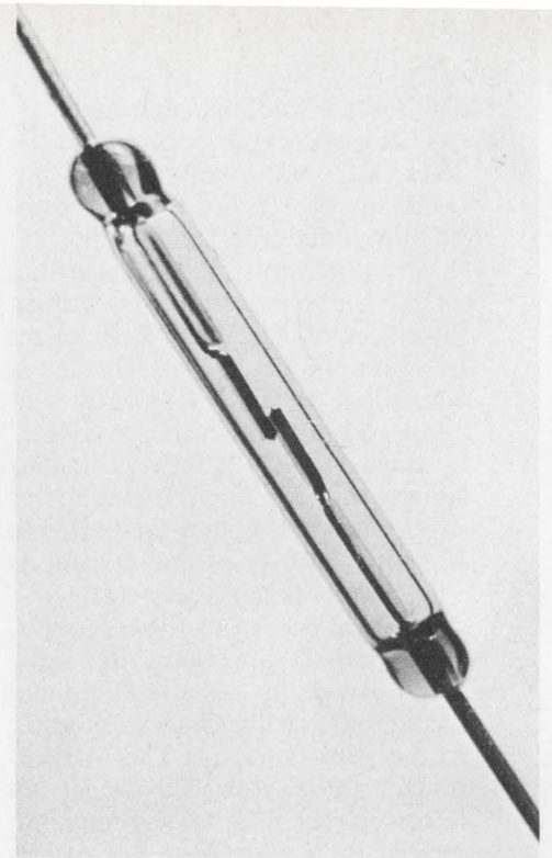
Slider. Twisted reeds slide along each other, keep contacts clean.
