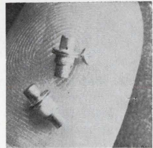
Gallium arsenide varactor diodes offer a 400 Ghz cut-off. Operating at all frequencies from uhf through Ku band, the units provide high gain bandwidth and low noise figures. Minimum reverse breakdown voltage is 6 v. Maximum power dissipation is 250 mw. Operating temperature is +10^{\circ} K to +175^{\circ} C. Varian Solid State Operation, Salem Road, Beverly, Mass. 01915. [439]
