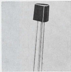
Epoxy encapsulated transistors designated GET'S come in a package with TO-18 lead configuration. They are for use in switching and amplifier applications and are of the npn and pnp types. Features include these reliability characteristics: 85^{\circ} C at 85% relative humidity; thermal shock of -65^{\circ} to +150^{\circ} C. General Electric Co., 1 River Road, Schenectady, N.Y. 12305. [437]
