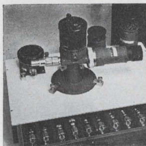
Standing wave detector type 2219K measures vswr and angle of reflection coefficient over a frequency range of 10 to 2,300 Mhz at a sensitivity of 5 mw. It eliminates heavy slotted sections and features adapters to all standard coaxial transmission lines. Detector components are now available in a kit form. PRD Electronics Inc., 1200 Prospect Ave., Westbury, N.Y. [401]
