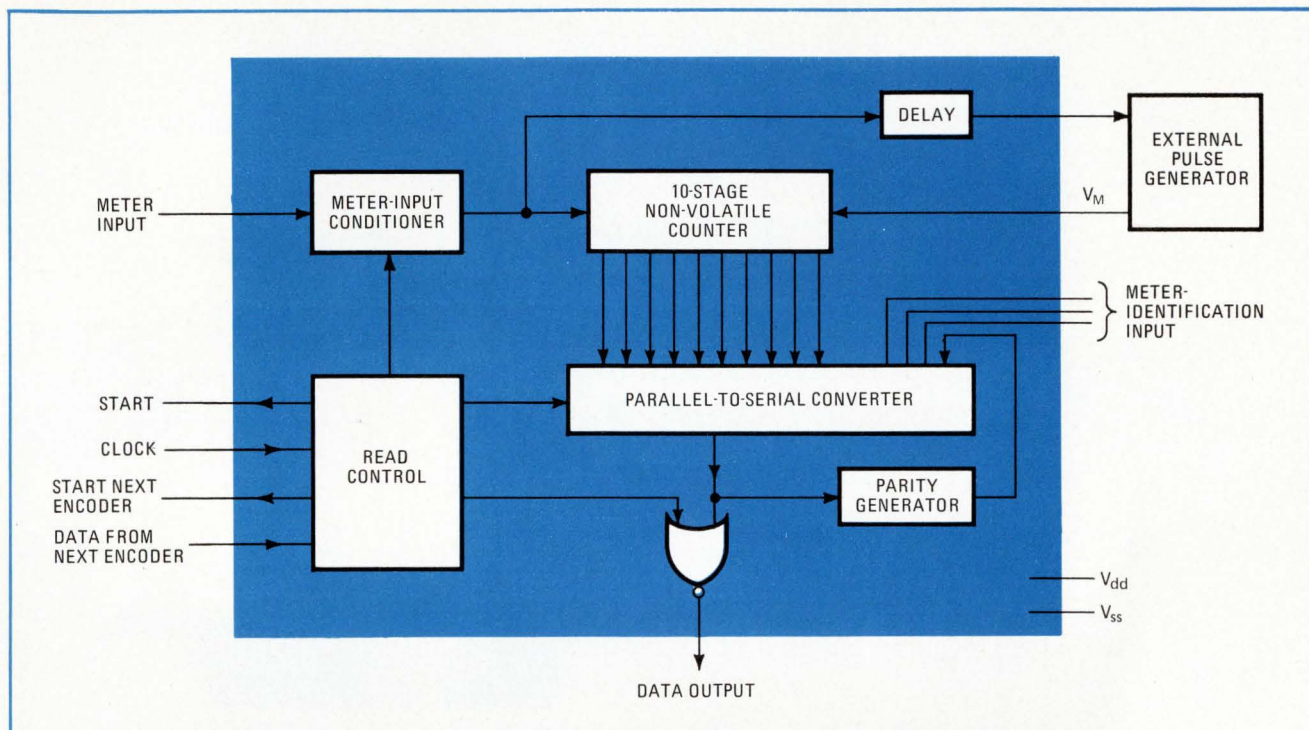
6. Meter encoder. After the 10-stage counter stores the meter pulses, a delay circuit allows the binary counter to "settle" before an external pulse generator provides a +25-V pulse to the V_M line of the counter that sets the memory transistors to a threshold of -2 V. Return of this line to its quiescent state of -25 V shifts the threshold of the proper memory transistor to -10 V, thus ensuring retention of metered count.
