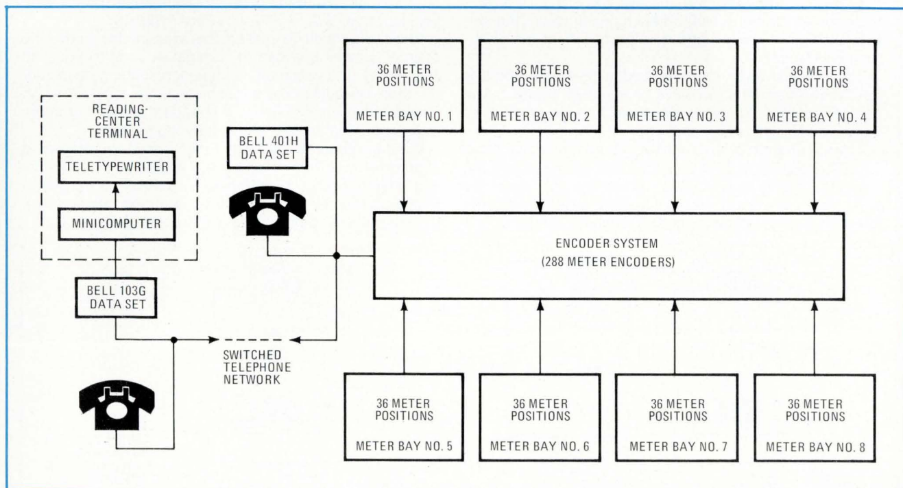
1. Remote readers. The electronic meter-reading system for utilities links meter bays to the encoder system, as shown in this block diagram of the Raleigh, N.C., installation, which in turn is linked to a central terminal minicomputer by telephone.
