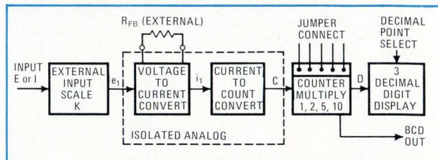
1. Flexible scaling. Arbitrary engineering units are easily accommodated by properly selecting external network (K), external range resistor ( R_{FB} ), and counter multiplier (M). K and R_{FB} set the full-scale range, while M determines the size of the counting increments.
