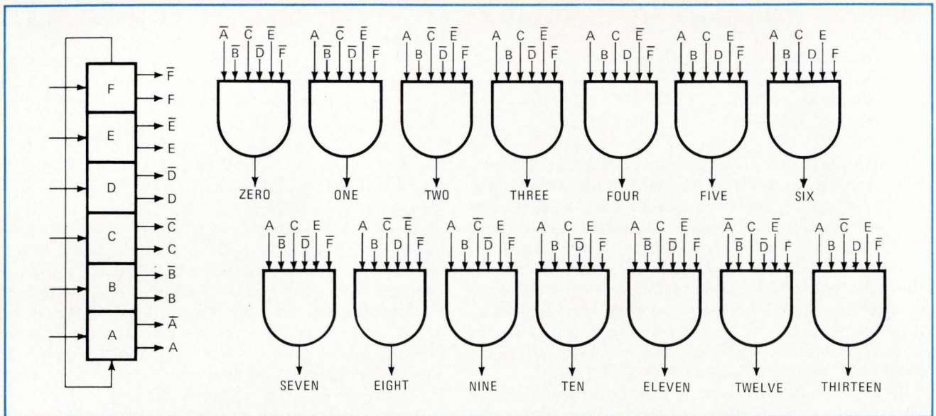
3. Rotation. After the six-bit ring counter is loaded, its contents are shifted five times so the decoding gates can determine if a given surround is present, regardless of its field orientation.
