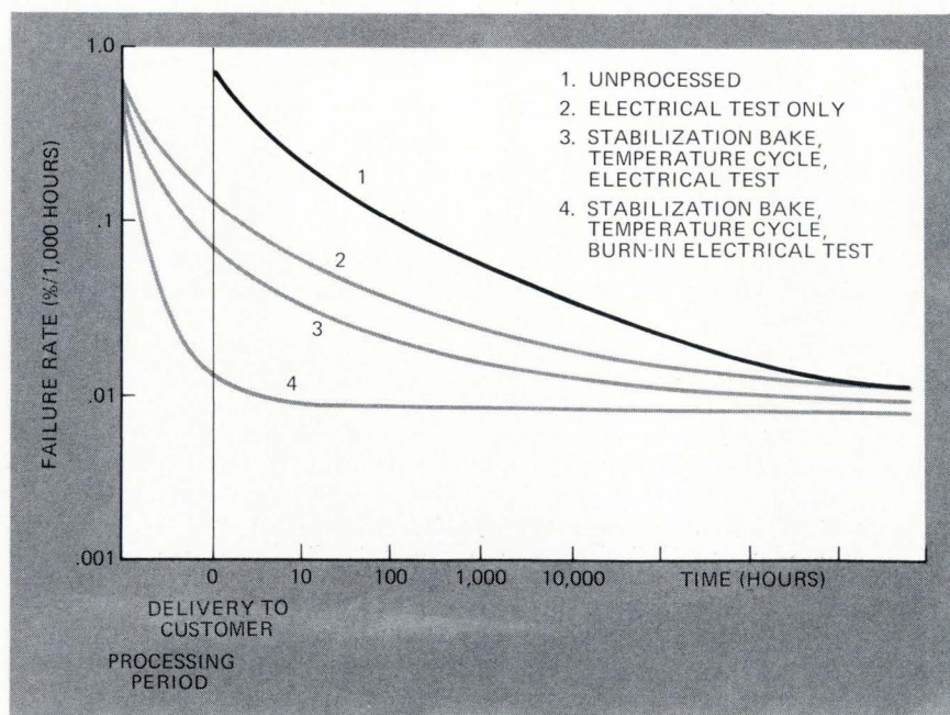
Data Curve. Reliability Inc. data is based on input from six customers on 1 million ics.
