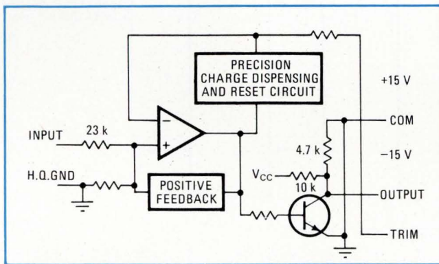
1. Converter. Frequency-to-voltage module follows charge-dispersing design approach. Output is buffered and TTL-compatible.
