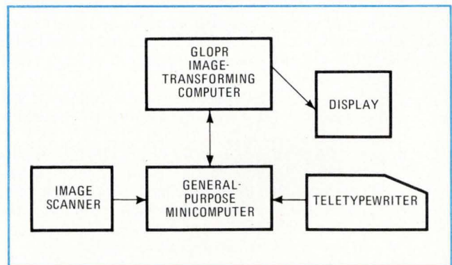
1. Interaction. Processing consists of transferring binary images into and out of GLOPR. Operator observes results of image transformations on CRT and acts on system through teletypewriter.
