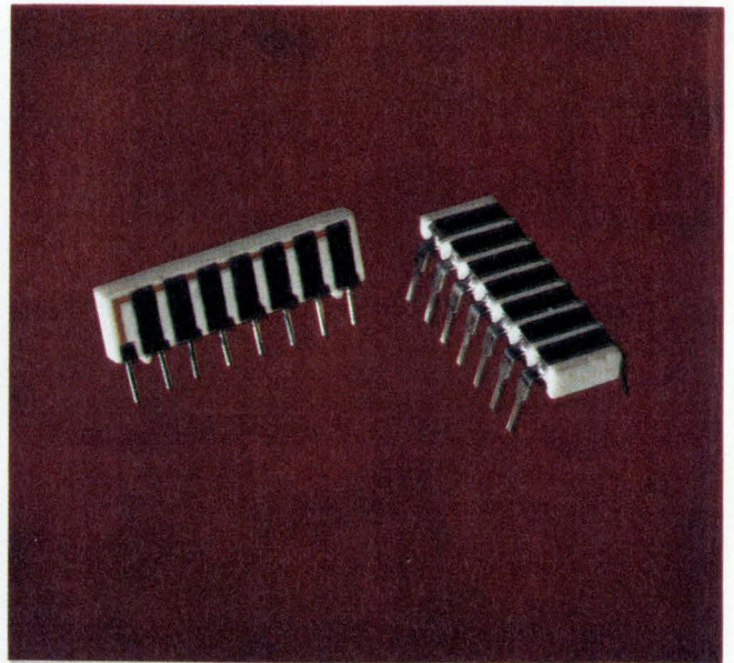
12. SIPs and DIPs for nets. Identical resistor networks are shown in DIP and SIP configurations. The SIP uses less board area but the DIP is more compatible with automatic insertion equipment.
