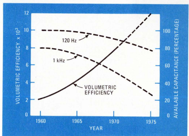
5. Tantalum in progress. Reduction in particle size and control of tantalum powder have decreased the potential loss of capacitance at higher frequencies, increased the capacitance per unit volume, and increased the upper frequency.
