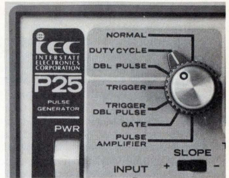
A single control selects all 7 modes.
