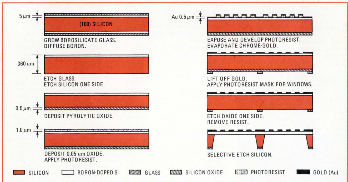
X-ray mask fabrication. Gold-on-silicon masks for X-ray exposure are made much like conventional silicon wafers. The mask is written with electron-beam techniques, however, and must be etched to a thickness of a few micrometers.
