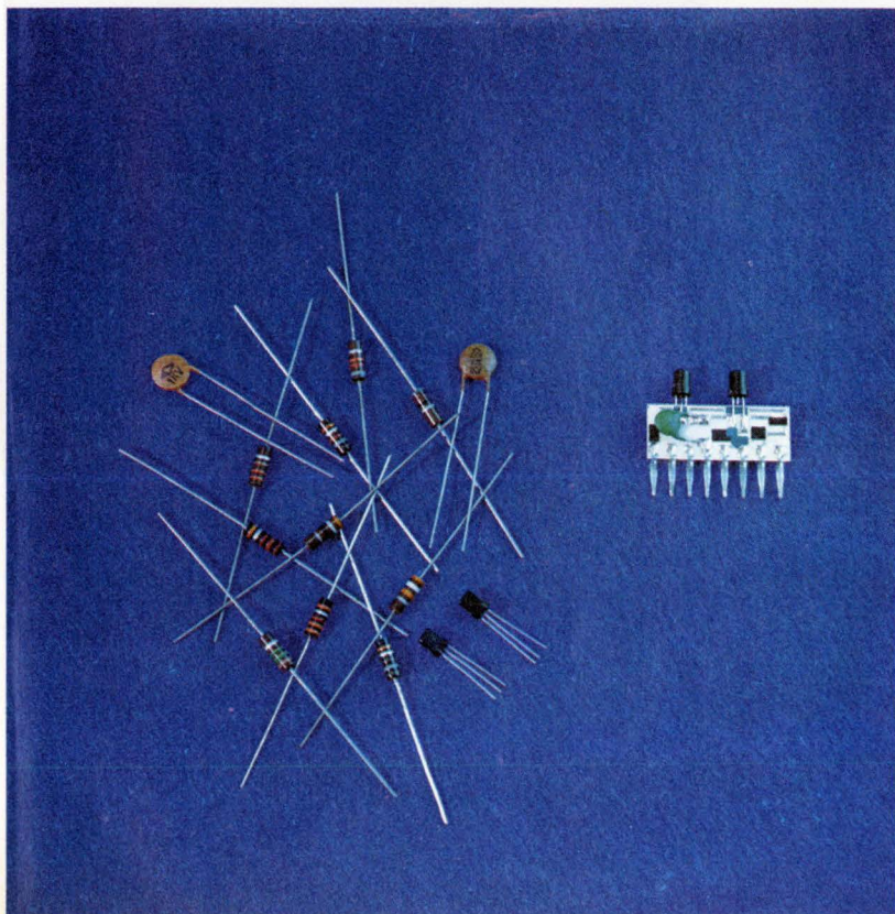
11. In the nets. This collection of discrete components (left) can all be incorporated in the network shown at the right. It is often cheaper to use networks for volume applications. Also, device-to-device tracking and tolerances are often tighter.
