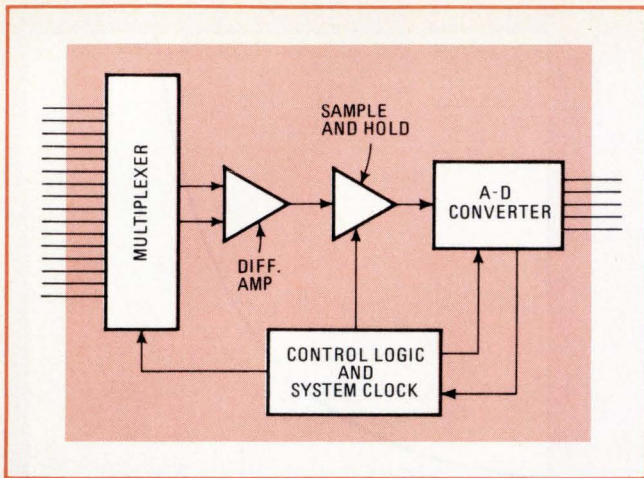
2. Internal peripheral. Data-acquisition front end includes expandable multiplexer, sample-and-hold circuitry, and a-d converter. Entire unit can be built into a package small enough to be mounted inside a minicomputer. Provisions for external control are not shown.
