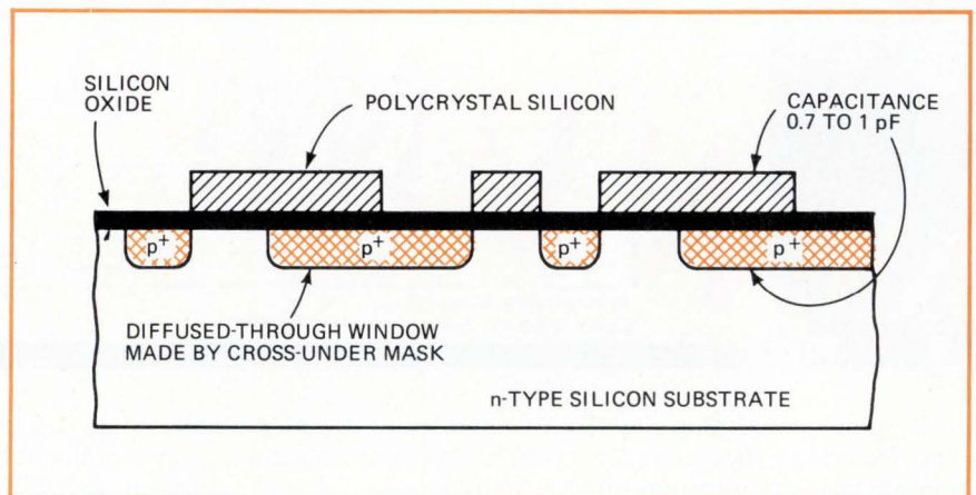
Bucket-brigade key. Single region of polycrystal silicon serves as both gate and electrode of capacitor. Note overlapping cross-under and self-aligned diffusions.
