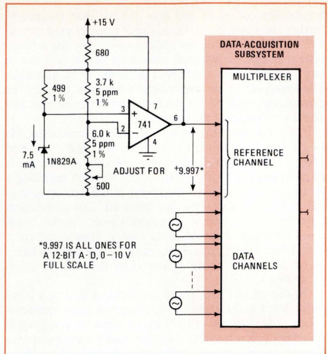
3. Self test. Stable reference source hard-wired to one channel of multiplexer can be used to test accuracy of entire system. A precision ramp generator might also be added to check linearity.
