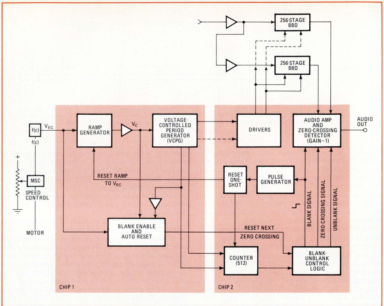
4. Tape chips. Functional block diagram of the two-chip Variable Speech Control shows how speed control is linked to the signal-processing circuitry. Ramp generator controls bucket-brigade switching rate via the VCPG to effect compression or expansion.
