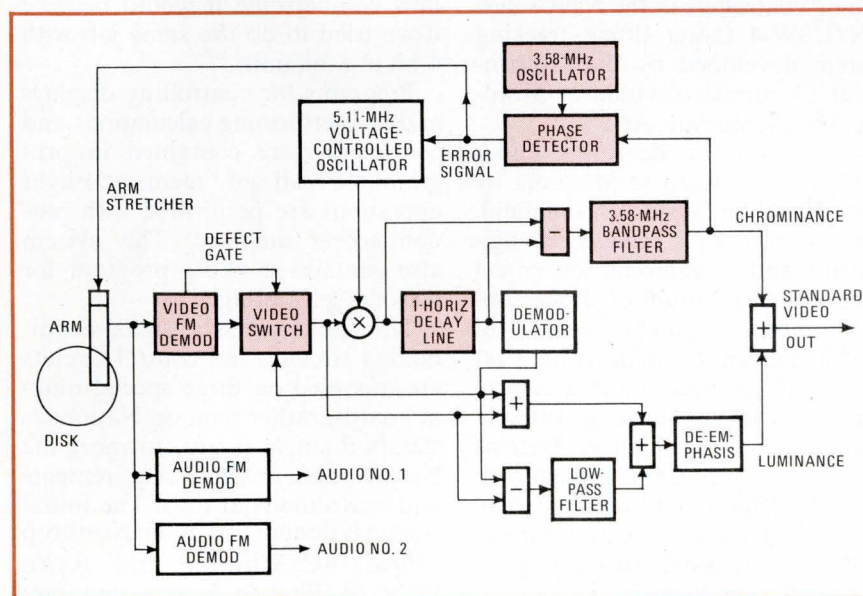
Loop. The only mechanical servo loop in RCA's VideoDisc player controls the "arm stretcher" which positions the stylus along the axis of the grooves in the disk.
