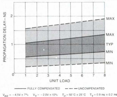
FULLY-COMPENSATED ECL vs. UNCOMPENSATED ECL
