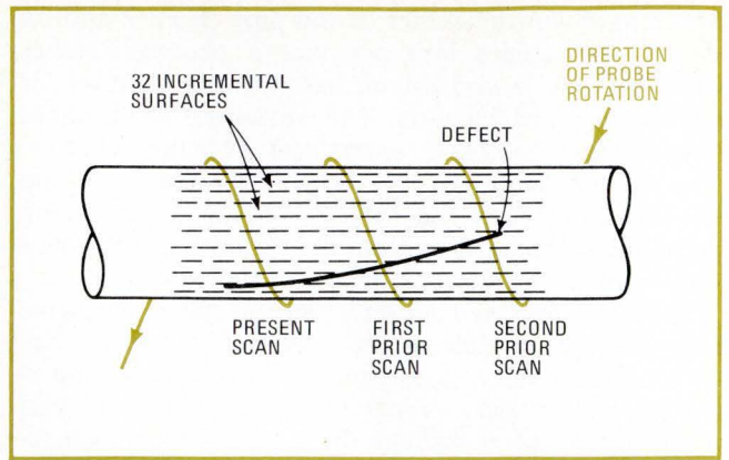
6. Locating the probe. As eddy-current probe rotates around an advancing bar, an encoder divides bar circumference into 32 increments. When defect signal is delivered by the pulse-width discriminator, the increment and scan number are stored, and the circuits correlate the present defect signal with signals for the same position in a preselected number of previous scans.
