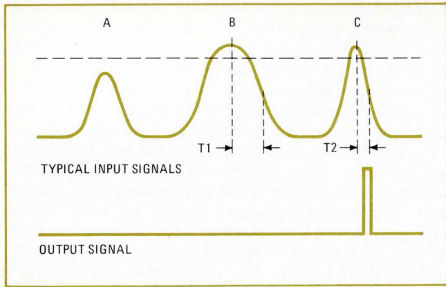
5. Pulse-width discriminator. In eddy-current testing, signal A, generated by shallow surface scratches in bars does not exceed a preset amplitude. Signal B, which is characteristic of loose surface scale, exceeds the amplitude, but does not decay fast enough. Signal C from a typical surface defect, exceeds preset limit and also falls off to half the peak value in less than the preset period.
