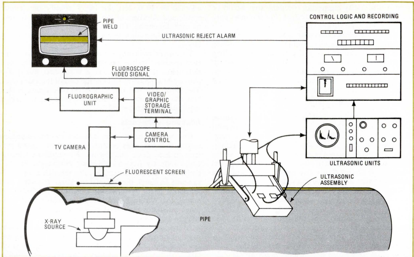
2. Tandem Inspection. After a flaw in the pipe weld is detected by the ultrasonic transducers, the rejection signal is stored in a shift-register memory until the rejected area is in view of the fluoroscope. At that point, the signal triggers an alarm on the TV screen, and simultaneously, a cursor appears on the screen to call the operator's attention to the defect. Inconsequential weld variations will not trigger an alarm.
