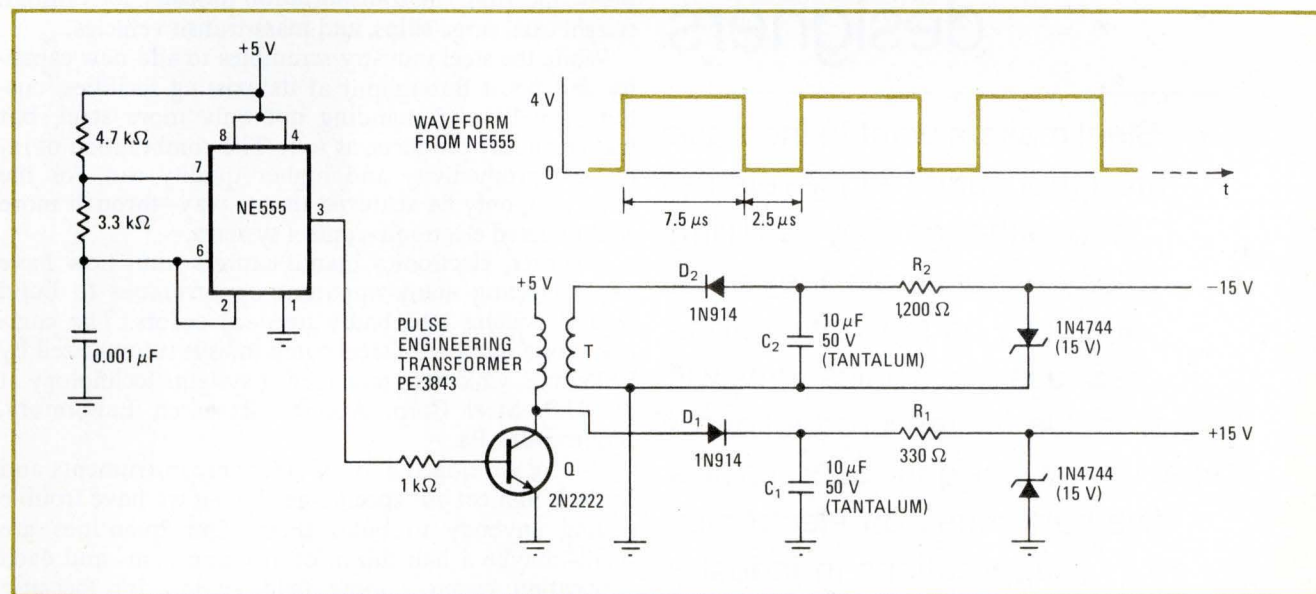
Space saver. Bipolar dc-to-dc converter operates from 5 volts and produces ±15 volts to supply op amps. Major advantage over conventional supply is small size, allowing assembly right on circuit board with other elements of system that it serves.
