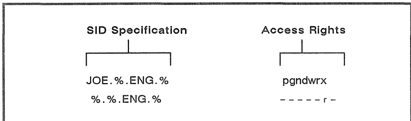
Figure 8-2. Sample ACL Entries
