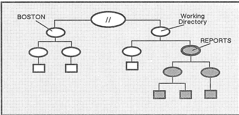
Figure 7-10. Deleting a Directory Tree
