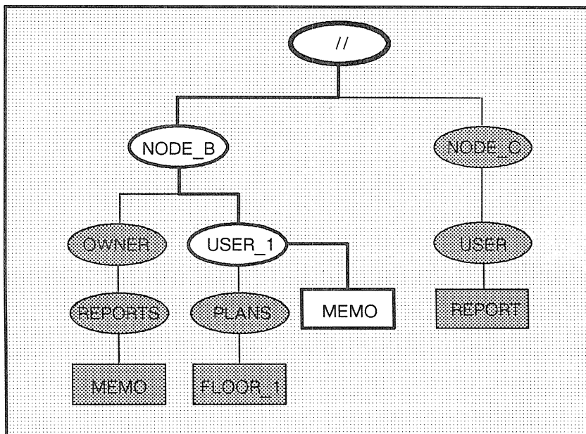
Figure 1-3. A Sample Path Through the Naming Tree
