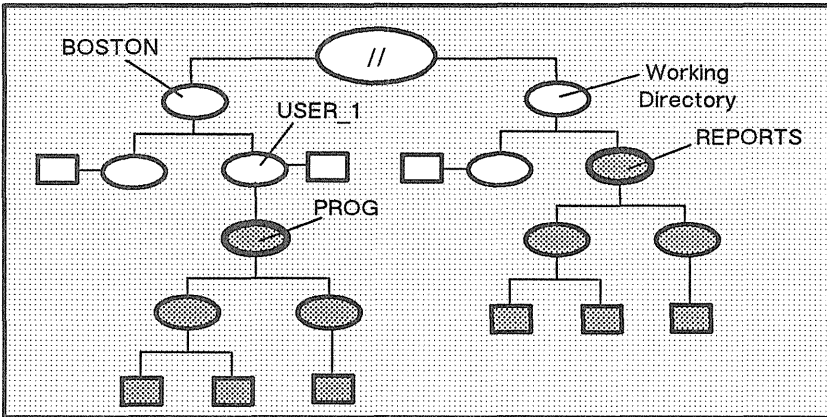
Figure 7-6. Copying a Directory Tree
