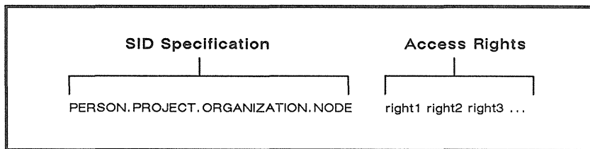
Figure 8–1. Structure of an ACL Entry
