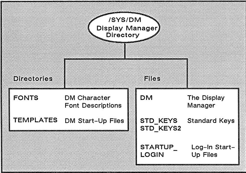
Figure A-3. The Display Manager Directory (ISYS/DM)
