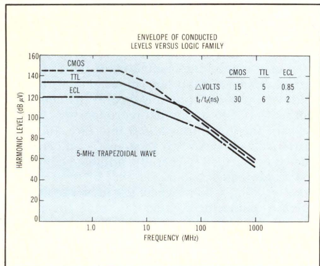
Fig 3 Fourier analysis of major logic families—CMOS, TTL, and ECL—yields the spectrum envelopes illustrated. All three logic types generate significant harmonics to the gigahertz region.
