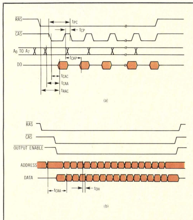
Fig 2 Addresses flow through the DRAM while column address strobe (CAS) is high, so data access actually begins from valid column addresses ( t_{CAA} ), not from CAS (a). Eliminating the CAS clock from the critical path of the DRAM makes short cycle times easier to use. In the static column mode (b), one clock period is eliminated, providing simpler system design. In this mode, the DRAM acts like a fast static device.
