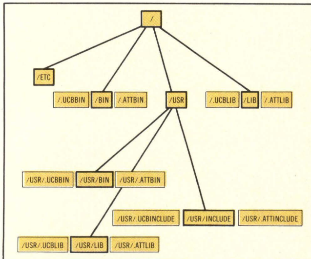
Fig 2 The dual-universe directory structure underlies the normal transparent directory structure perceived by the user and/or the programs. Bold lines indicate what the user sees; lighter boxes reveal underlying directories with universe-indicating attribute fields.
