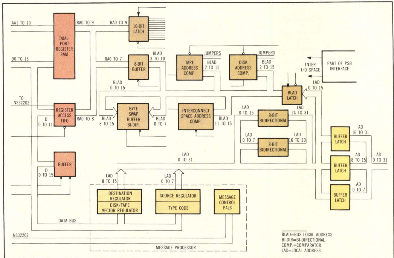
Fig 4 In this example of an SCP message processor and disk/tape registers, byte swapping for correct alignment occurs on the local bus. It is placed in easily accessed locations in the dual-port RAM during the transfer operation.
