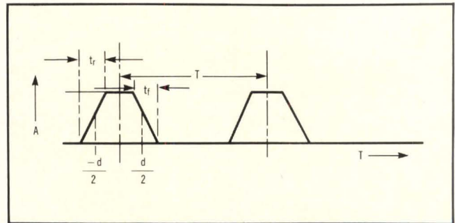
Fig 1 Trapezoidal waveforms approximate signals. Controlling emi is difficult due to the large resource of harmonics found in digital control signals because of fast rise times and high frequencies.
