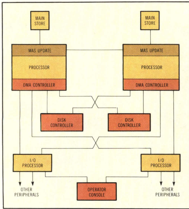
Fig 1 The 3B20D minicomputer hardware architecture is designed for fault tolerance. It features duplicated hardware for critical components. Applications for the computer system designer or integrator include transaction processing, process control, and aerospace.
