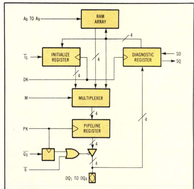
The Advanced Micro Devices Am9151 static RAM contains three internal registers that enable the designer to monitor internal states of combinational logic blocks for diagnostic operations.
