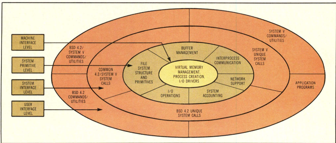
Fig 4 In OSx, the differences between System V and 4.2 BSD are handled in the outer three levels. Many user interface conventions are the same; some unique commands and utilities have been added. Both operating systems' call handling functions exist at the system call level.
