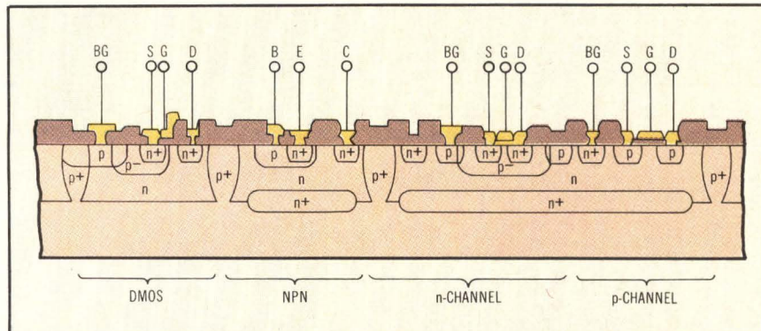
CMOS logic devices (right) may share the same substrate space with high current DMOS transistors (left). Siliconix has used this process to build a controller IC with exclusive-OR logic to switch 12-A peak currents at 120 V and at 200-kHz rates. The process can handle 150-V potentials and 20-A peak currents.
