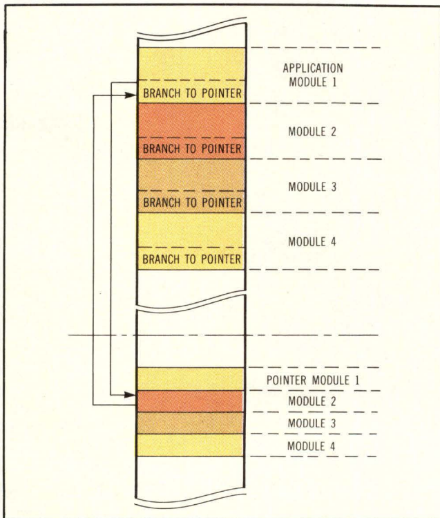
Fig 3 A simple way to change software remotely is to store code in modules, then change pointers and implemented code. Here, the end of application module 1 branches to a pointer register, which directs the processor to application module 2. Changing the pointer to application module 4 via modem link changes system operation.
