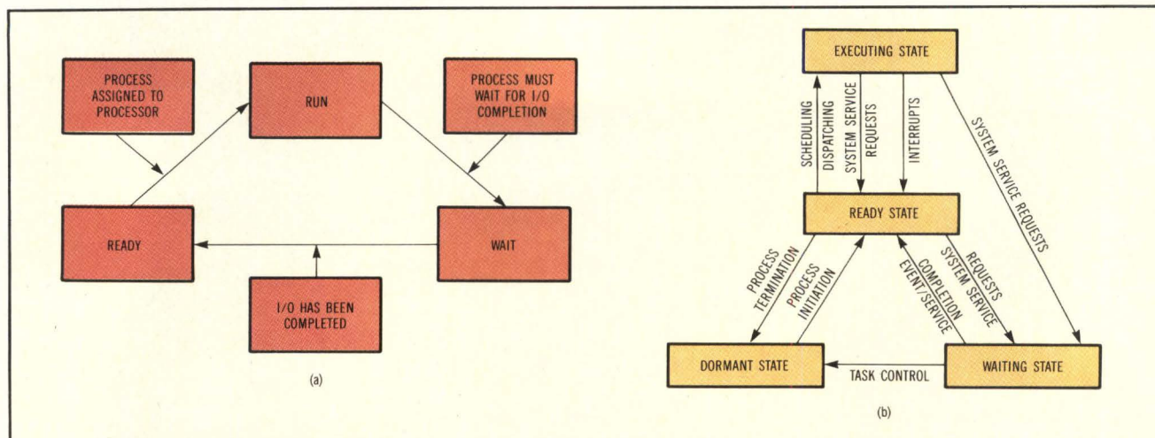
Fig 2 Processes can have simple states (a) or a more complicated set of state transitions (b). Realtime minicomputer designers should look for the simplest set for a really fast system and, for example, avoid wait states with memory, file, device, and other wait subdivisions.
