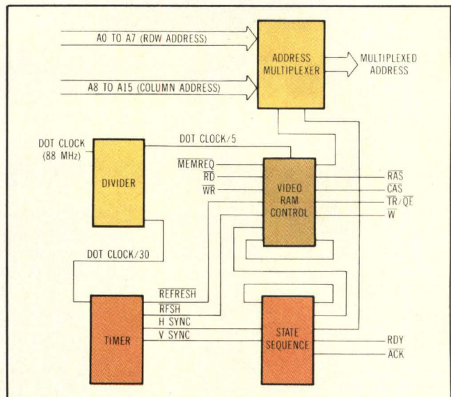
Fig 5 RAM and video control logic for a unified design can be implemented with programmable logic arrays and MSI circuits. A gate array or custom device could integrate the entire function in a high volume application.
