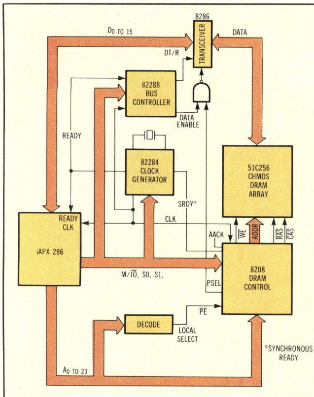
Fig 6 Fast cycle times and relaxed timing margins within the cycles are useful in high performance and high density memory systems.
