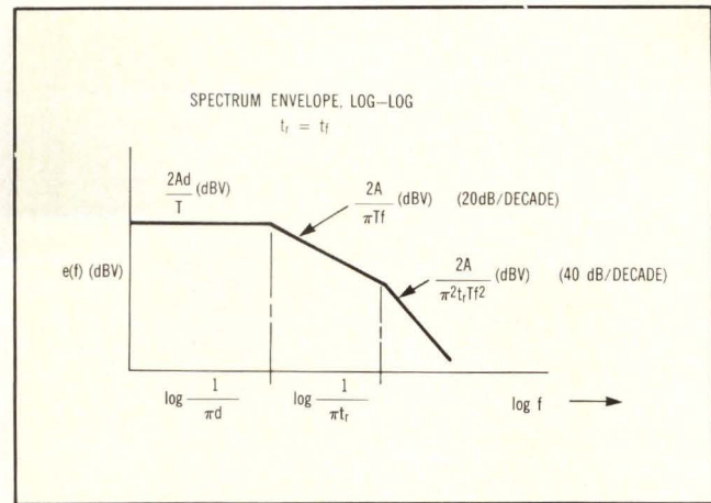
Fig 2 The spectrum envelope shown is developed from a Fourier analysis of the waveform in Fig 1. Here, the signal's rise and fall times are assumed to be equal.
