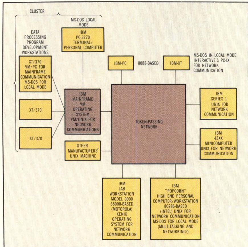
The communication link hooking all the departments in the corporate environment will feature a Unix-based communication system that links IBM and other vendors' machines, regardless of type. Both local and remote machine operation will be possible. Each machine will be able to access data or programs from the others and will perform either general purpose or dedicated functions.
