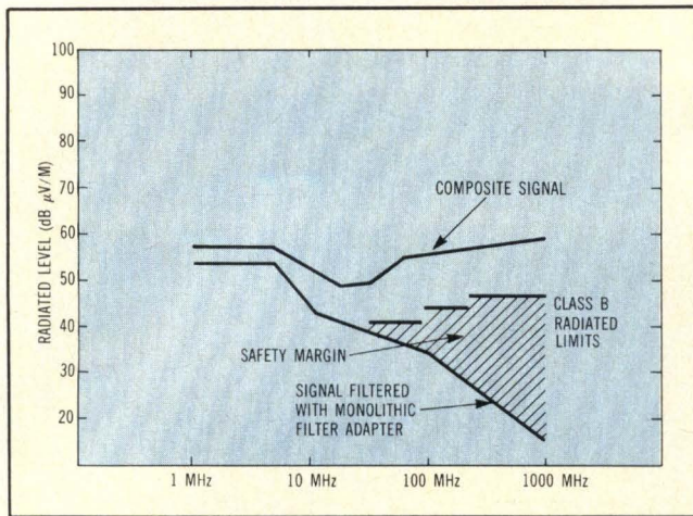
Fig 6 The addition of a filtered connector to the antenna model analyzed in Fig 4 brings radiation well within FCC specifications.
