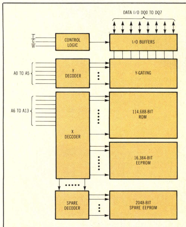
In addition to 16 Kbits of EEPROM in the memory map, a spare 2-K can be mapped into the memory space of Motorola's MCM683616 combination ROM/EEPROM by the decode circuitry.
