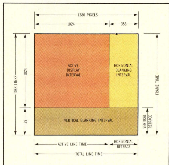
Fig 3 In a high resolution video display, the total frame time is the sum of active display time, and horizontal and vertical blanking intervals.
