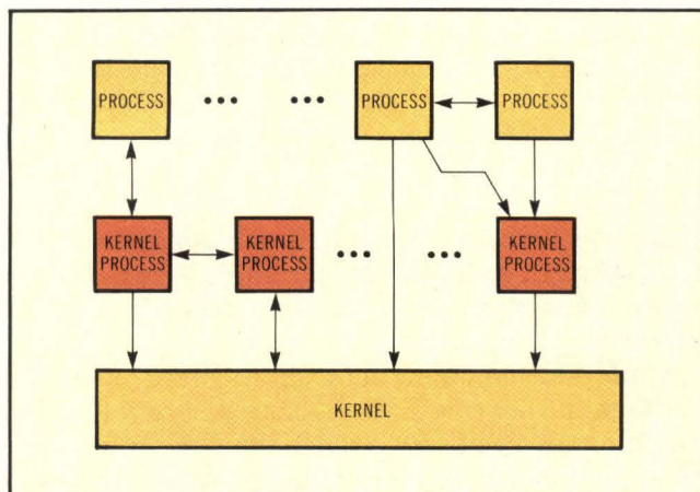
Fig 2 The software architecture of the Unix RTR realtime operating system in the 3B20D minicomputer is comprised of three layers: process, kernel, and kernel process. The kernel process is new and is not used in standard Unix. Processes and kernel processes can communicate with each other as shown.
