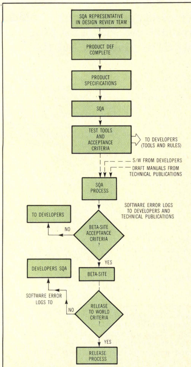
Fig 1 In product definition, the software quality assurance (SQA) group advises the development team about potential problems that can arise during testing, defines the acceptance criteria, and learns about the product in advance of final testing during the release stage. Once the software has passed SQA criteria, it is released to beta-sites, and if all tests are passed, it is released to manufacturing.
