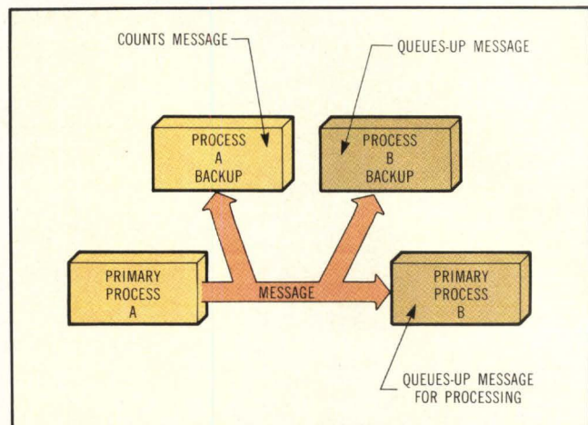
Fig 2 When a message is sent by a primary process to its next process, the primary's backup receives a copy, as does the backup for the next process. If one message fails to arrive, the system bus ensures that none arrive, so the queue-and-count software does not fail.
