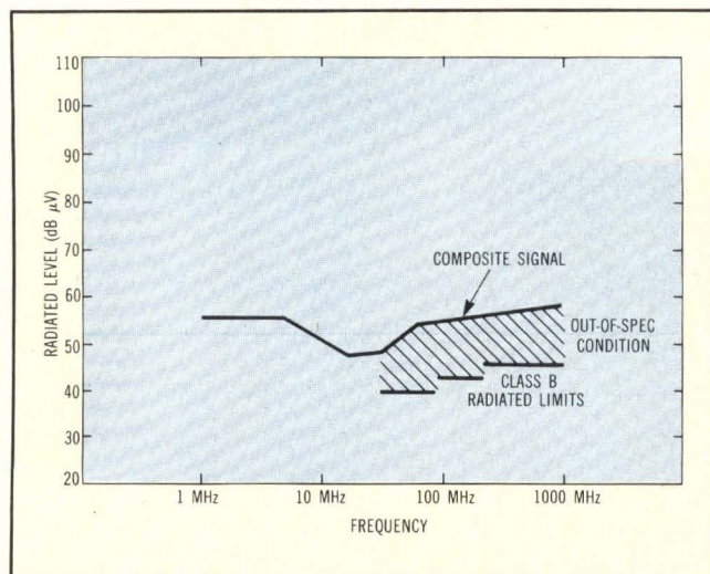
Fig 4 Maxwell field equations applied to a digital circuit antenna model yield a composite signal in excess of the FCC limits.
