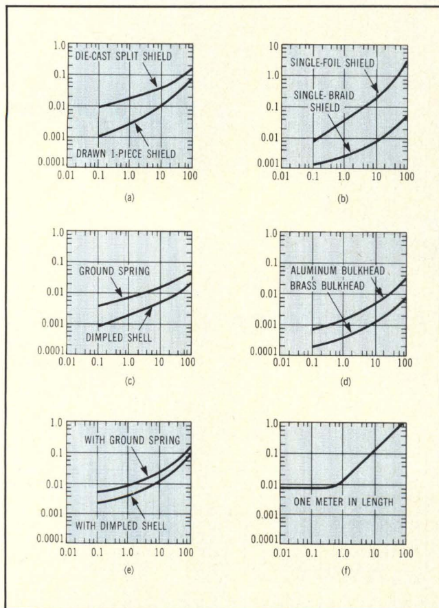
Fig 5 Pictured are the transfer impedances (ohms/ y axis) versus frequency (MHz/ x axis) between, for example, shielded backshell and connector backshell (a); between shielded backshell and cable shield, including 0.5 in. of cable shield (b); between plug and receptacle shells (c); and between receptacle and bulkhead (d). Also pictured are the total of all contributions from aluminum bulkhead through to shield crimp (e); and the typical braid shielded cable (f), which is 0.3 in. in diameter.
