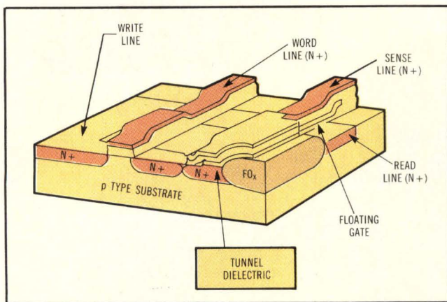
Fig 1 Advanced fabrication technology (Oxinitride) and a memory cell circuit design technique (Q-cell) increase EEROM speeds and endurance.
