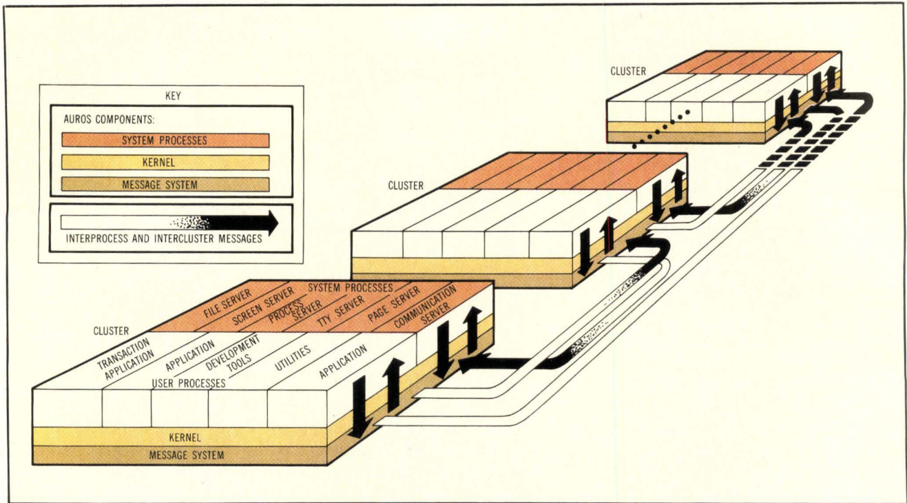
Fig 3 All processes and clusters send and receive messages via the kernel-based message system. Division of the cluster processes into user and system processes allows the kernel to handle local operations while the servers handle global ones.
