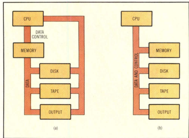
Fig 1 Most minicomputer architectures sport a central memory to connect a CPU and its peripherals (a). With some exceptions, the minicomputer operating system must be designed around this approach. DEC's PDP-11 features a central bus for data and control (b).
