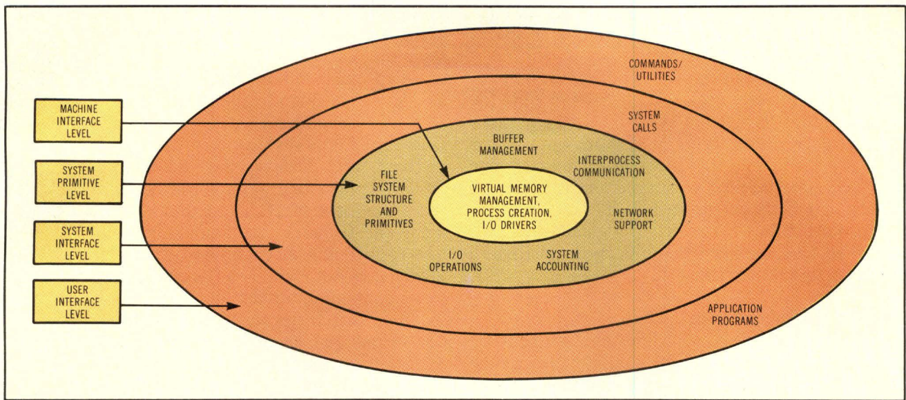
Fig 3 Unix is divided into levels that separately handle user, system, services, and machine interface functions. Calling conventions and software structures isolate levels from one another and allow modular software changes to meet new needs.
