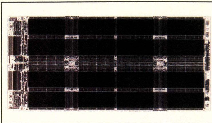
The Intel 51C256 dynamic RAM is representative of the new generation of 256-Kbit DRAMs. Implemented in the company's CHMOS process, the chip features Ripplemode for extremely fast access to successive bits.
