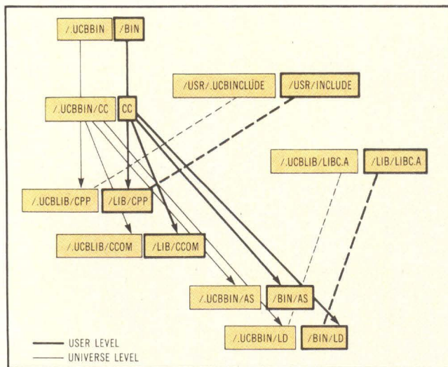
Fig 5 Because programmers can access both universes, it is important that application programs be fixed to one environment for compatibility. A program execution environment is established by linking compiler, libraries, and header files during compilation/linking.
