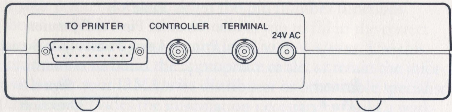
Figure 3-1 IRMAprint Rear Panel
