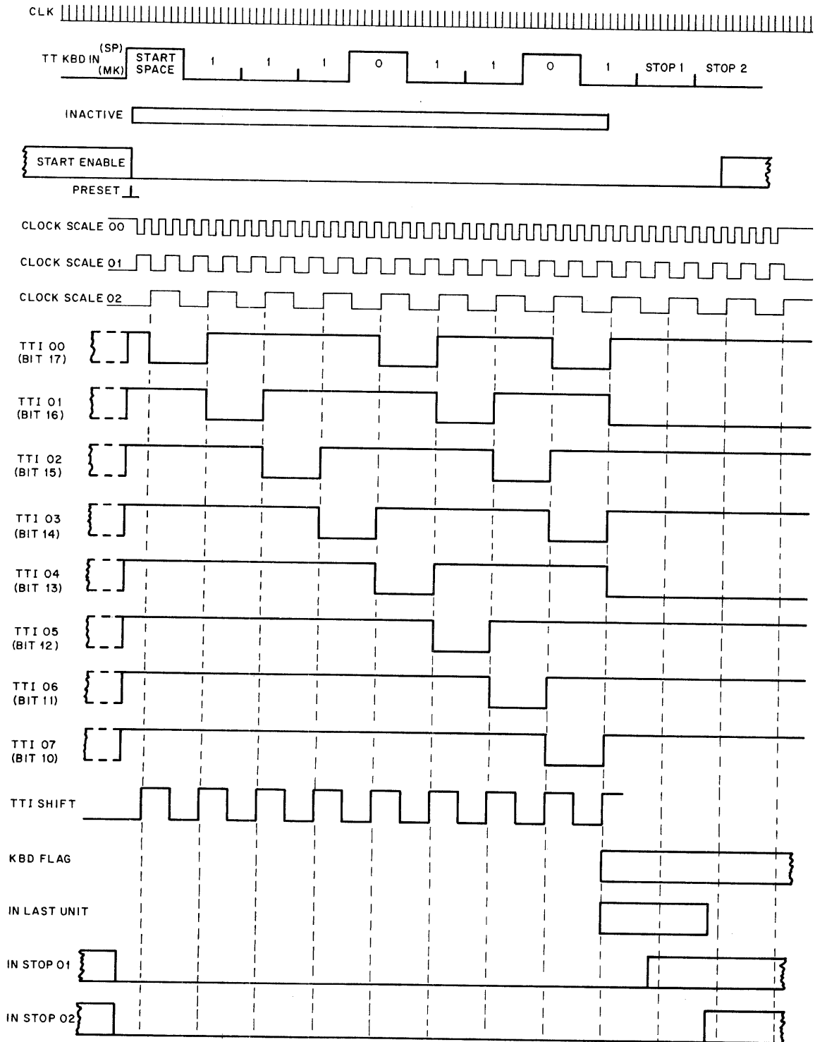
Figure 6-17 Teletype Receiver (Keyboard) Timing
