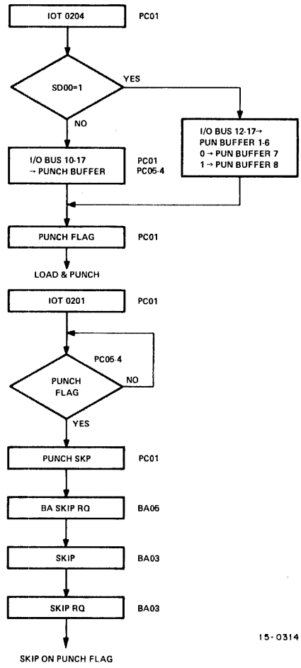
Figure 6-16 High-Speed Punch Operation, Flow Diagram
