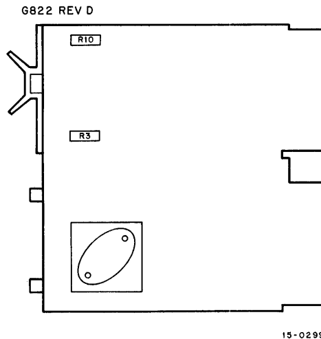
Figure 7-4 G822 Module Adjustment Locations
