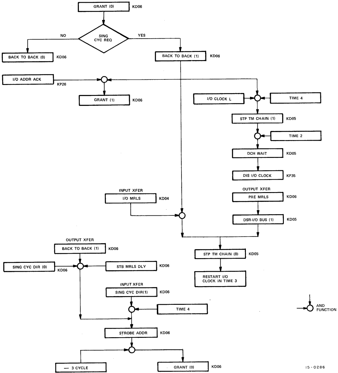
Figure 4-11 Single Cycle Back-To-Back Transfer, Detailed Flow Chart
