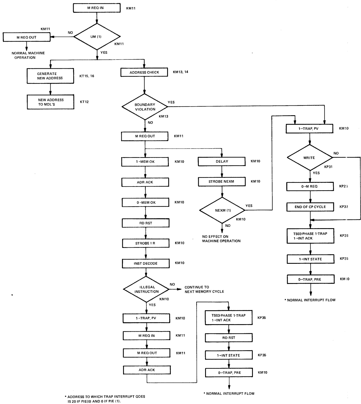
Figure 6-12 KT15 Memory Protect/Relocate Flow Diagram
