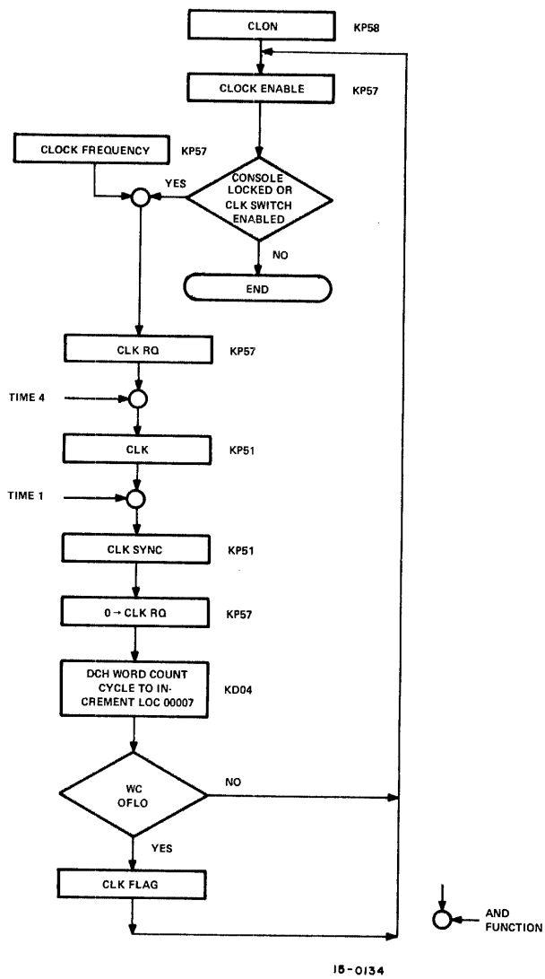
Figure 6-4 Real-Time Clock, General Flow Diagram
