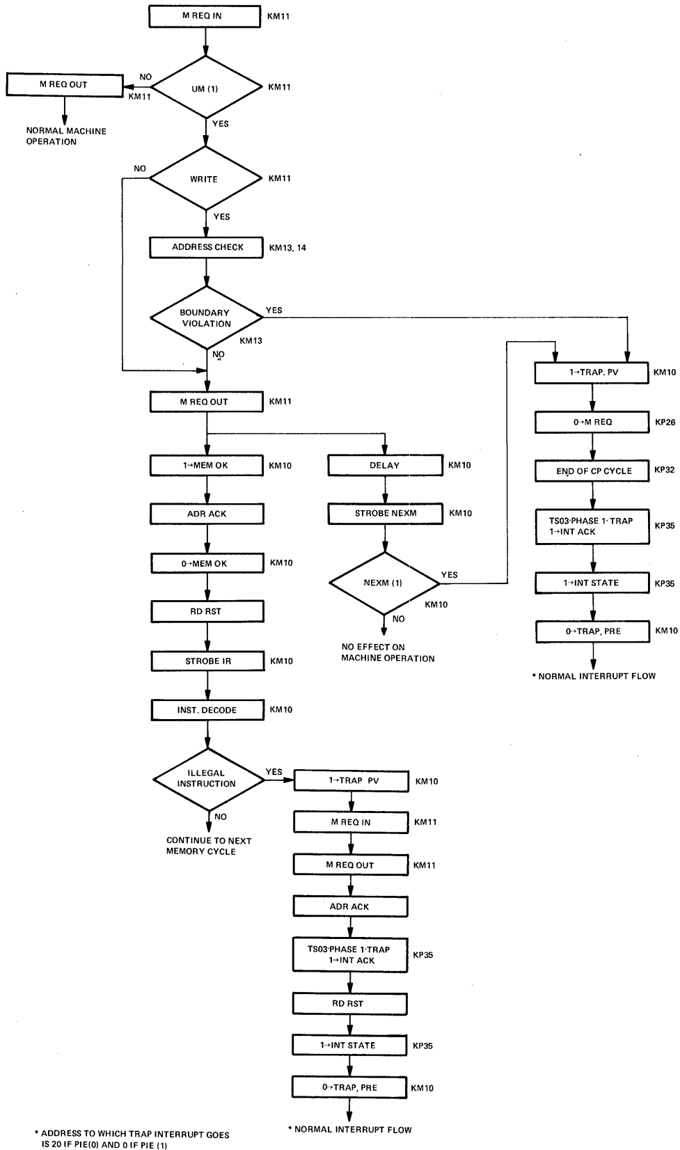
Figure 6-11 KM15 Memory Protect Flow Diagram
