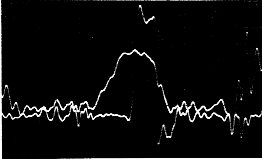
Figure 7-8 MEM Strobe/Sense Amp Output
