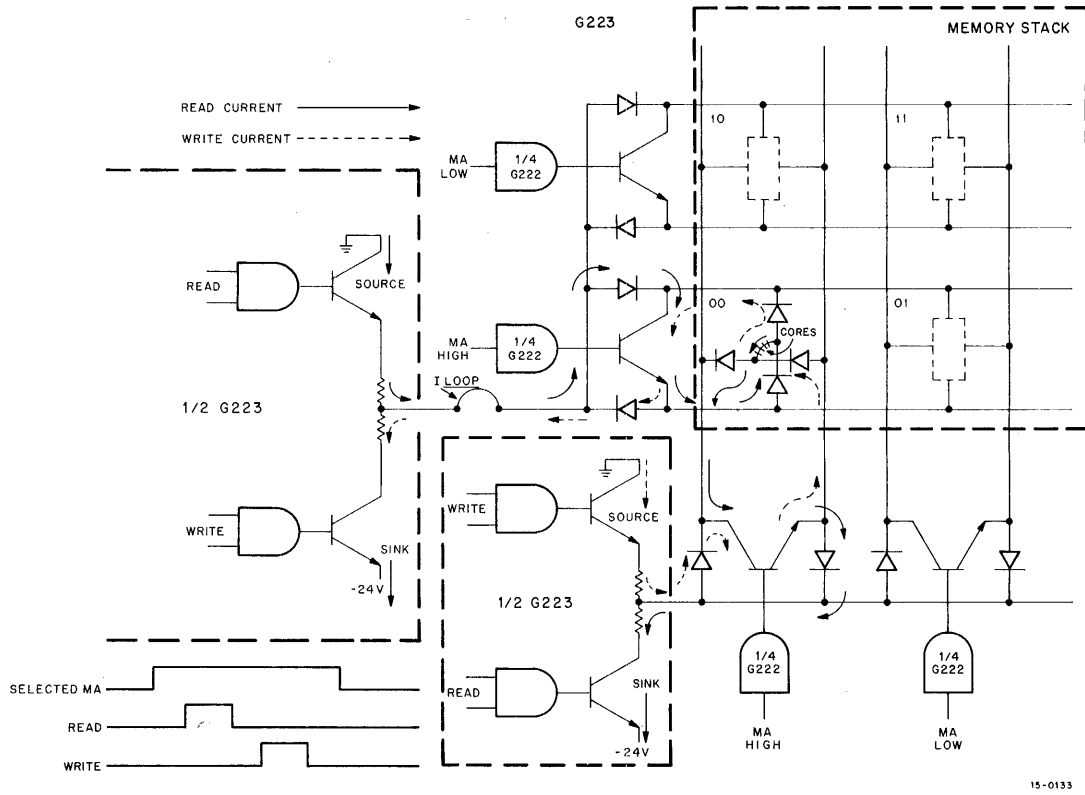
Figure 2-1 Current Path Diagram
