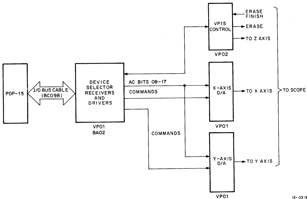
Figure 6-19 VP15 Controller, Simplified Block Diagram
