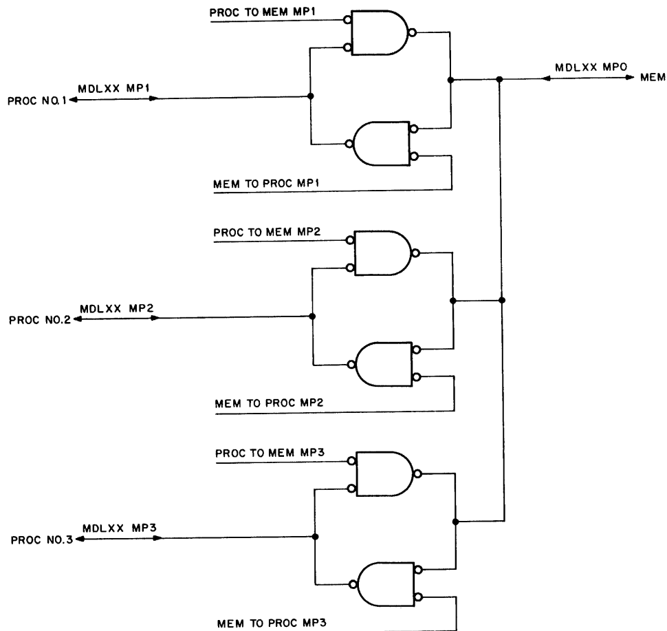
Figure 4-3 Bidirectional Switch
