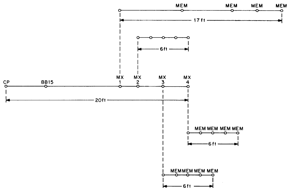
Figure 1-5 128K CP/Memory Cable Lengths
