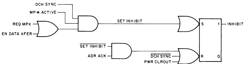
Figure 4-7 Inhibit Logic
