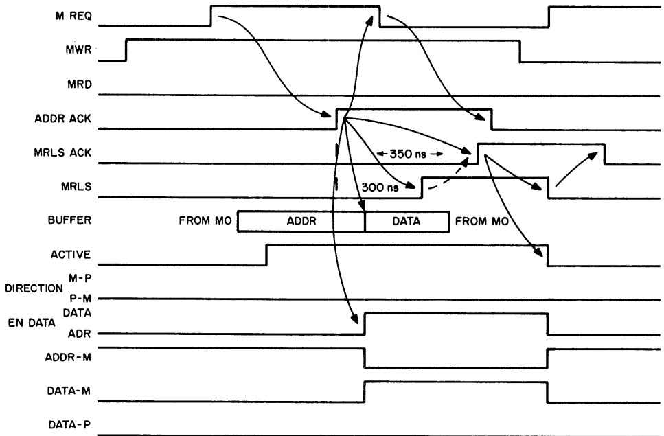
Figure 4-2b MX15-A Timing Diagram
