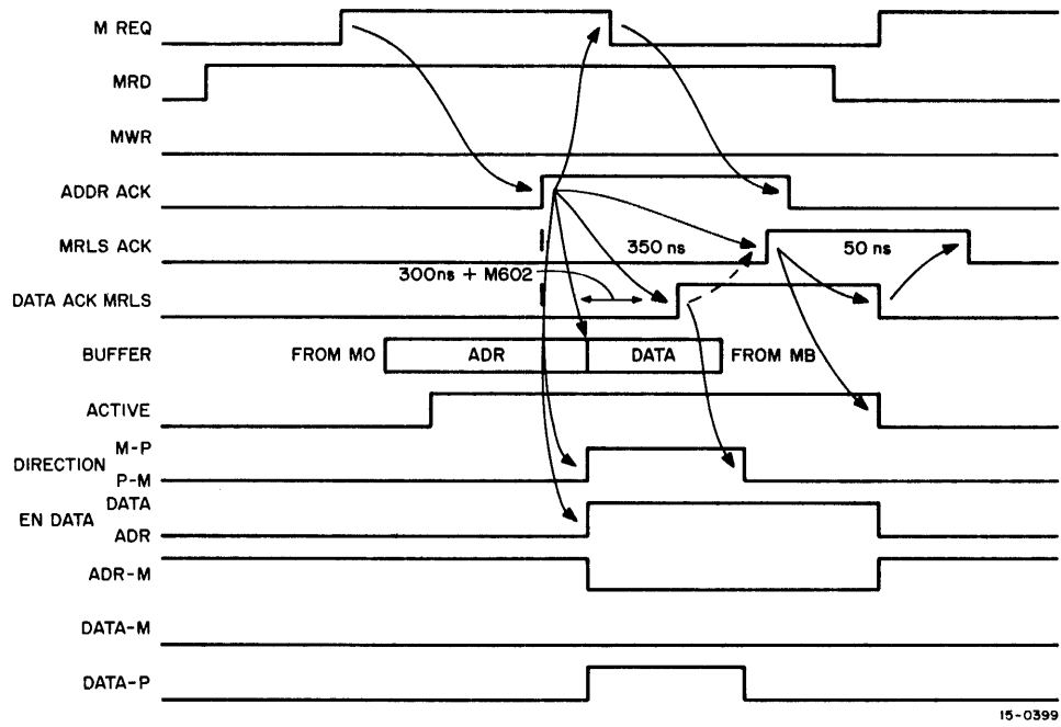
Figure 4-2a MX15-A Timing Diagram
