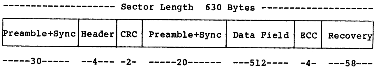
Figure 2-3 Sector Format
