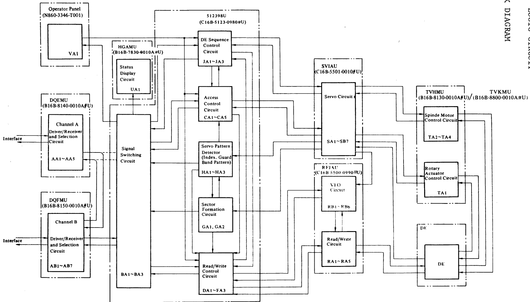
The number at the bottom of each box indicates the circuit diagram number in chapter 17.
