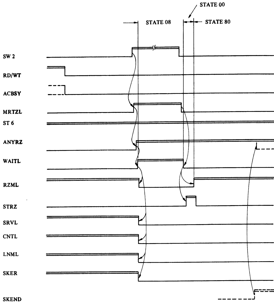
Figure 8.6-2 Manual RTZ Sequence
