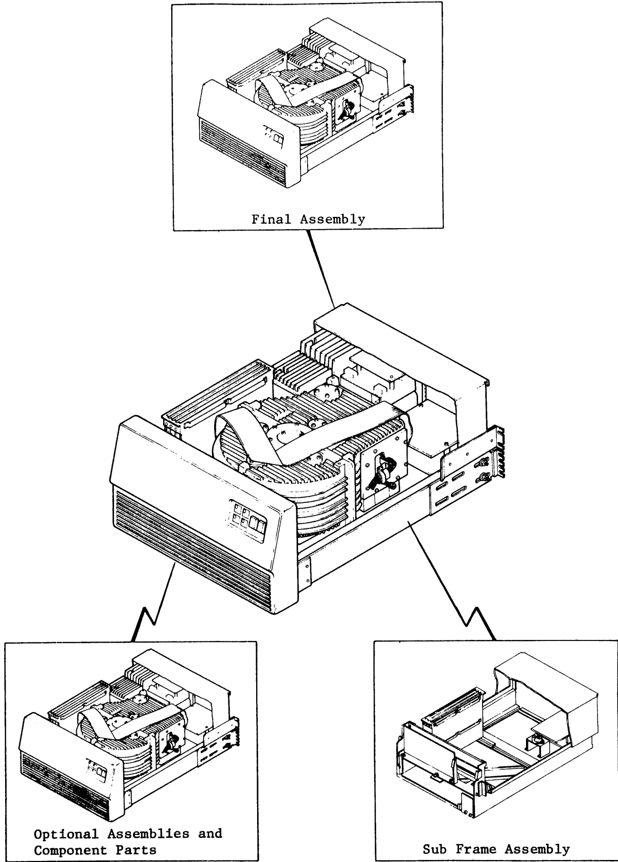
Figure 5.7-5 Visual Index Mini-Disk Drive
