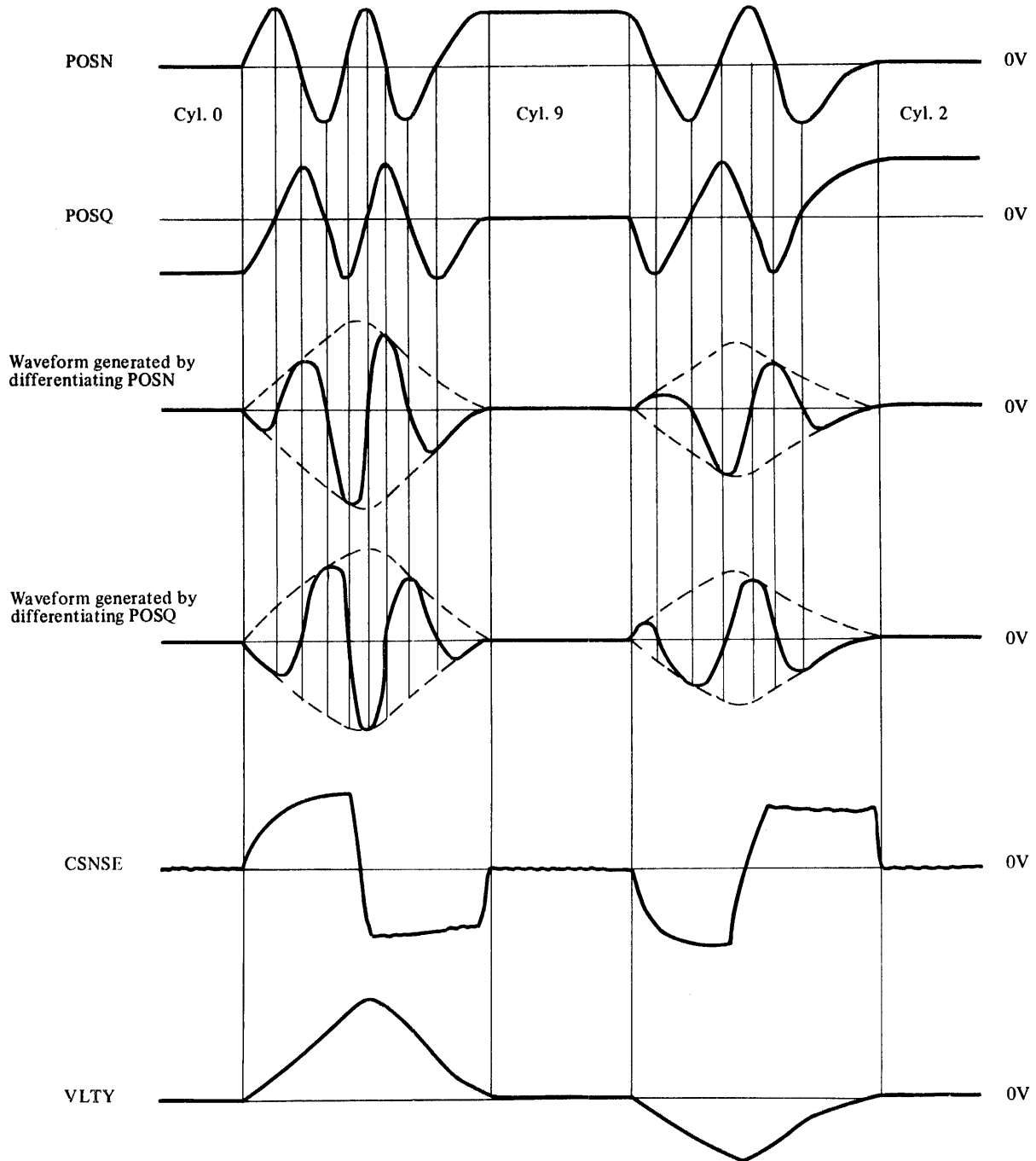
Figure 9.5-12 Velocity
