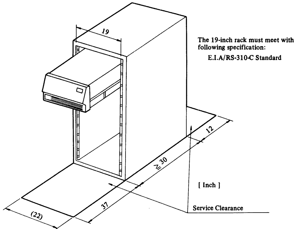
Fig. 1.1-2 Physical Dimensions
