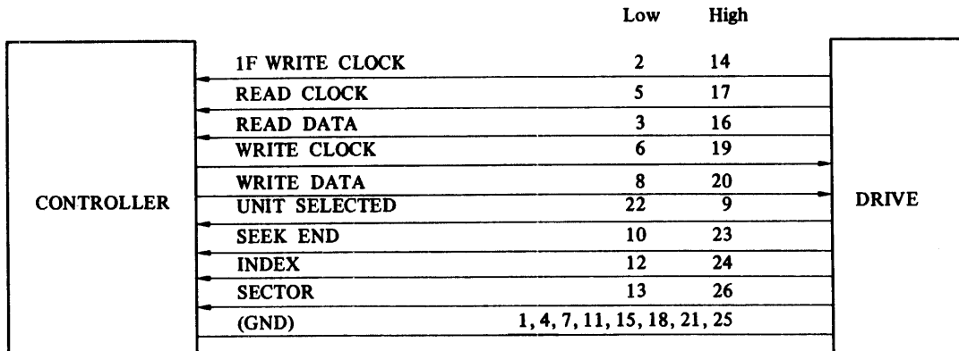
Fig. 7.2-2 B-Cable
