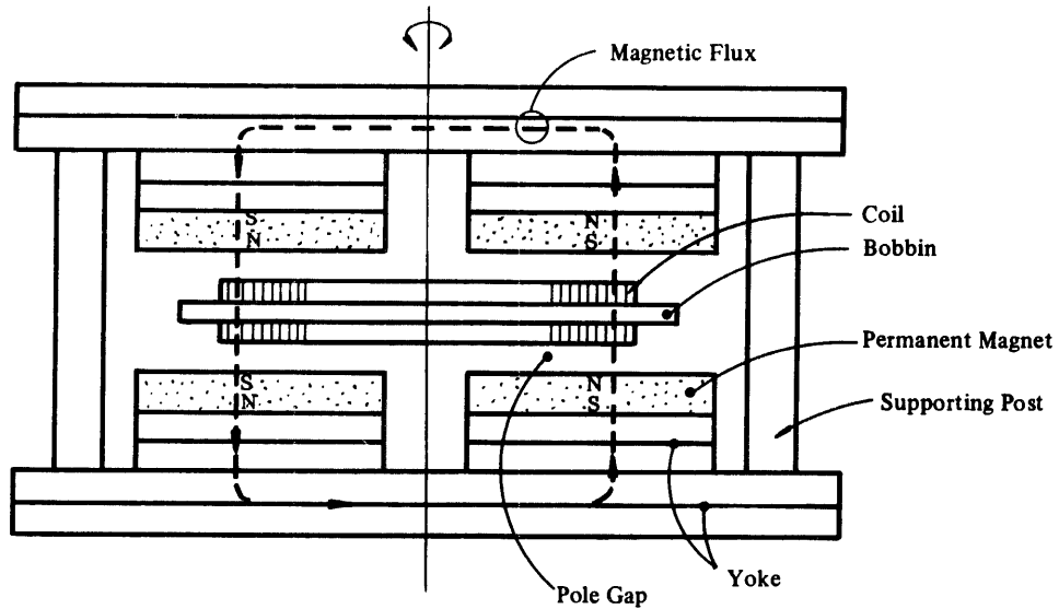
Figure 5.3-2 Magnetic Circuit
