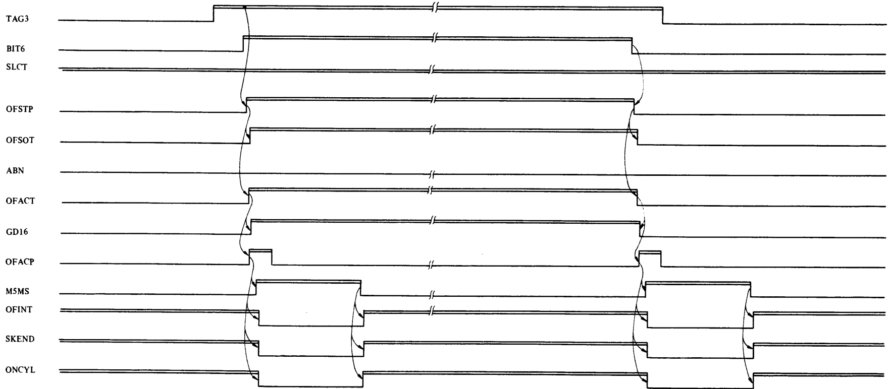
Figure 8.8-1 Offset Sequence
