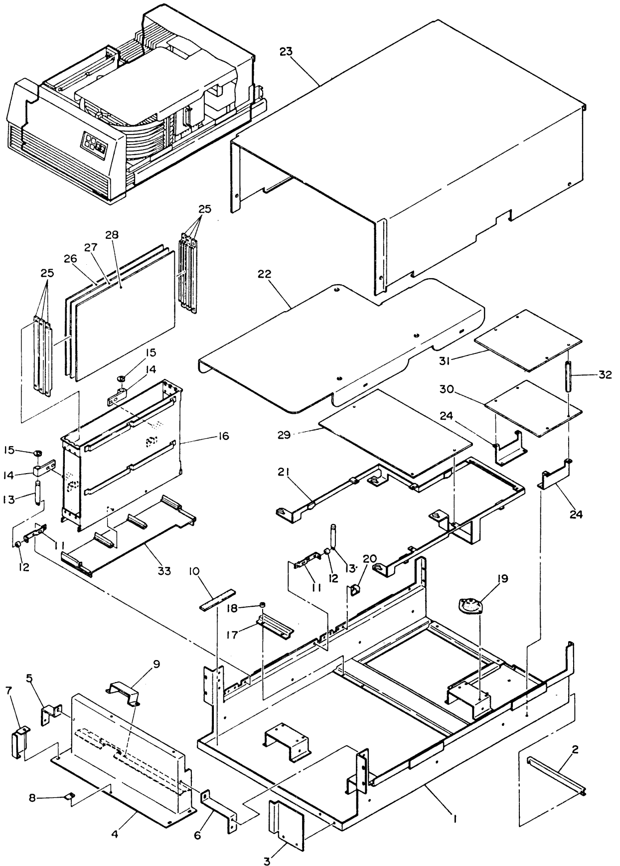
Figure 5.7-3 Sub-Frame Assembly
