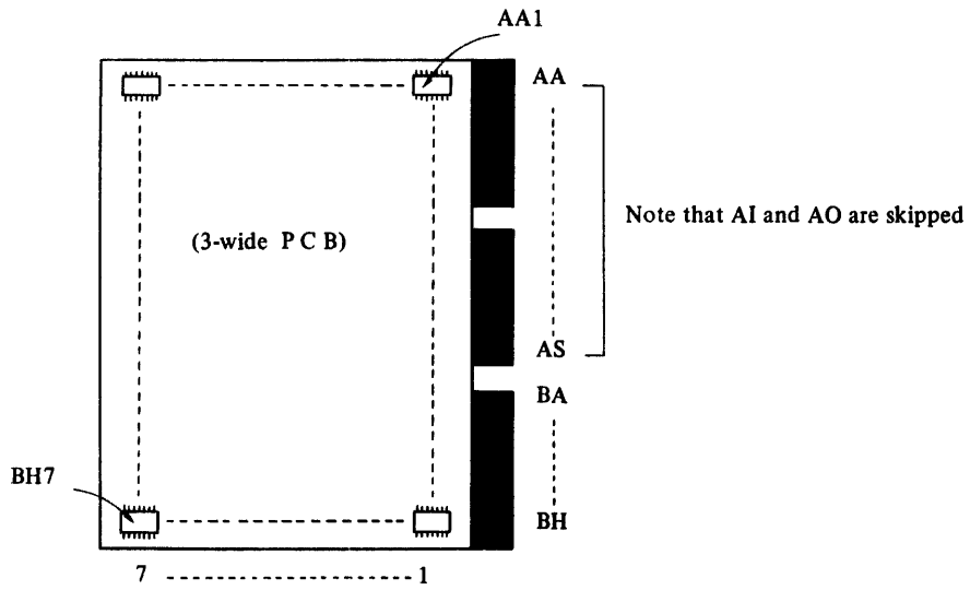
Figure 14.1-2 IC Location
