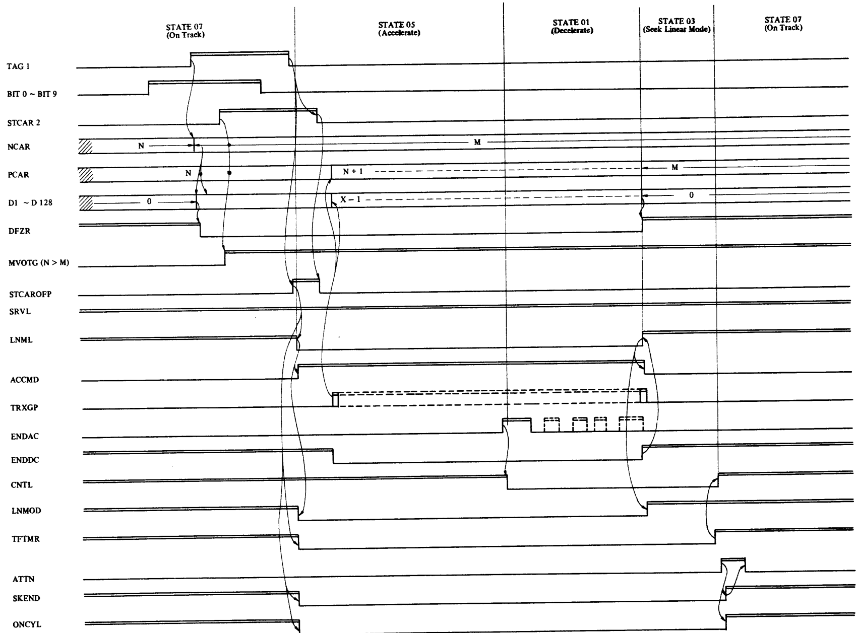
Figure 8.7-1 Seek Sequence
