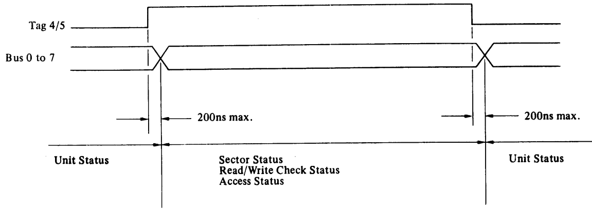
Fig. 7.7-15 Tag 4/5 Timing
