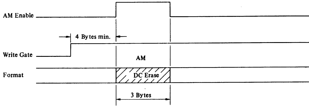
Fig. 7.7-11 AM Write
