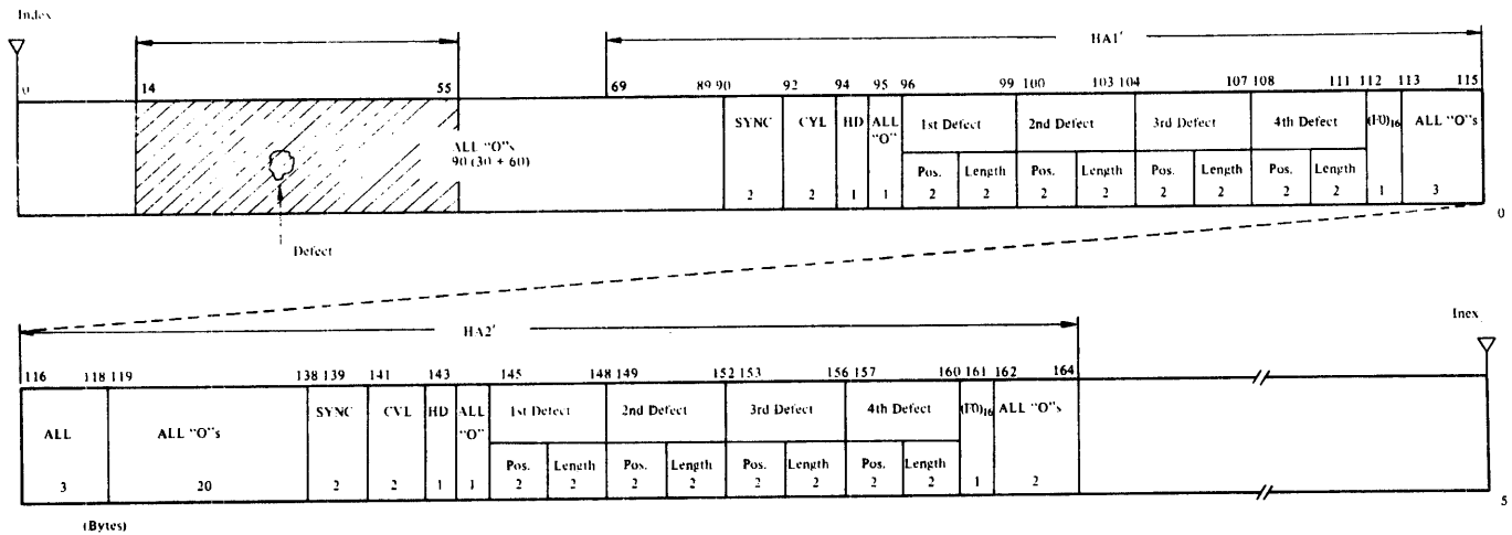
Figure 6.3-2 Format 2
