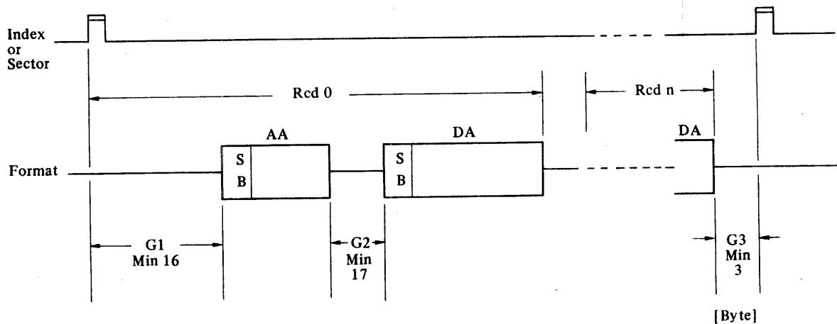
Figure 6.1-2 Fixed Sector Format
