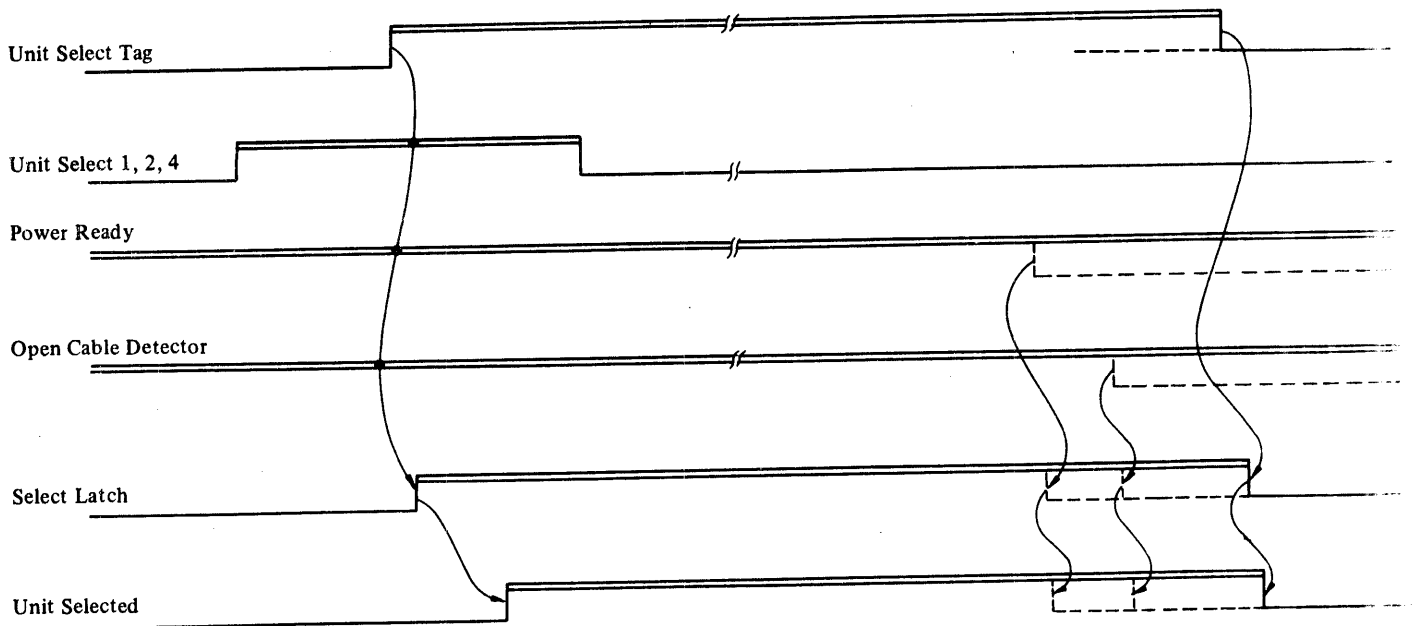
Figure 8.3-1 Unit Selection
