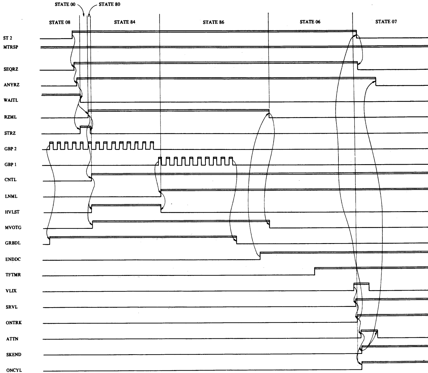
Figure 8.5-1 Sequence RTZ
