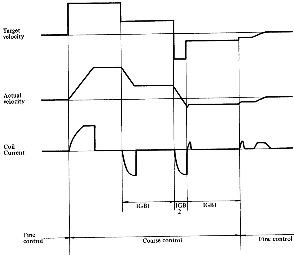
Figure 9.4-1 Rezero Control
