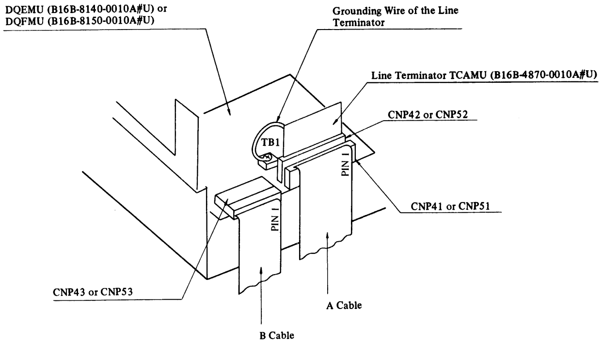
Fig. 4.1-1 Cable Connection
