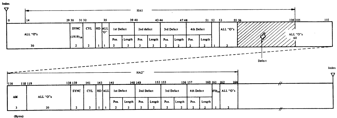
Figure 6.3-3 Format 3
