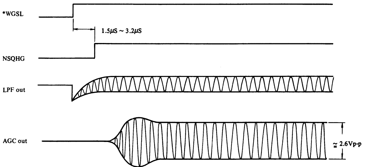
Fig. 10.2-3 AGC Squelch Function
