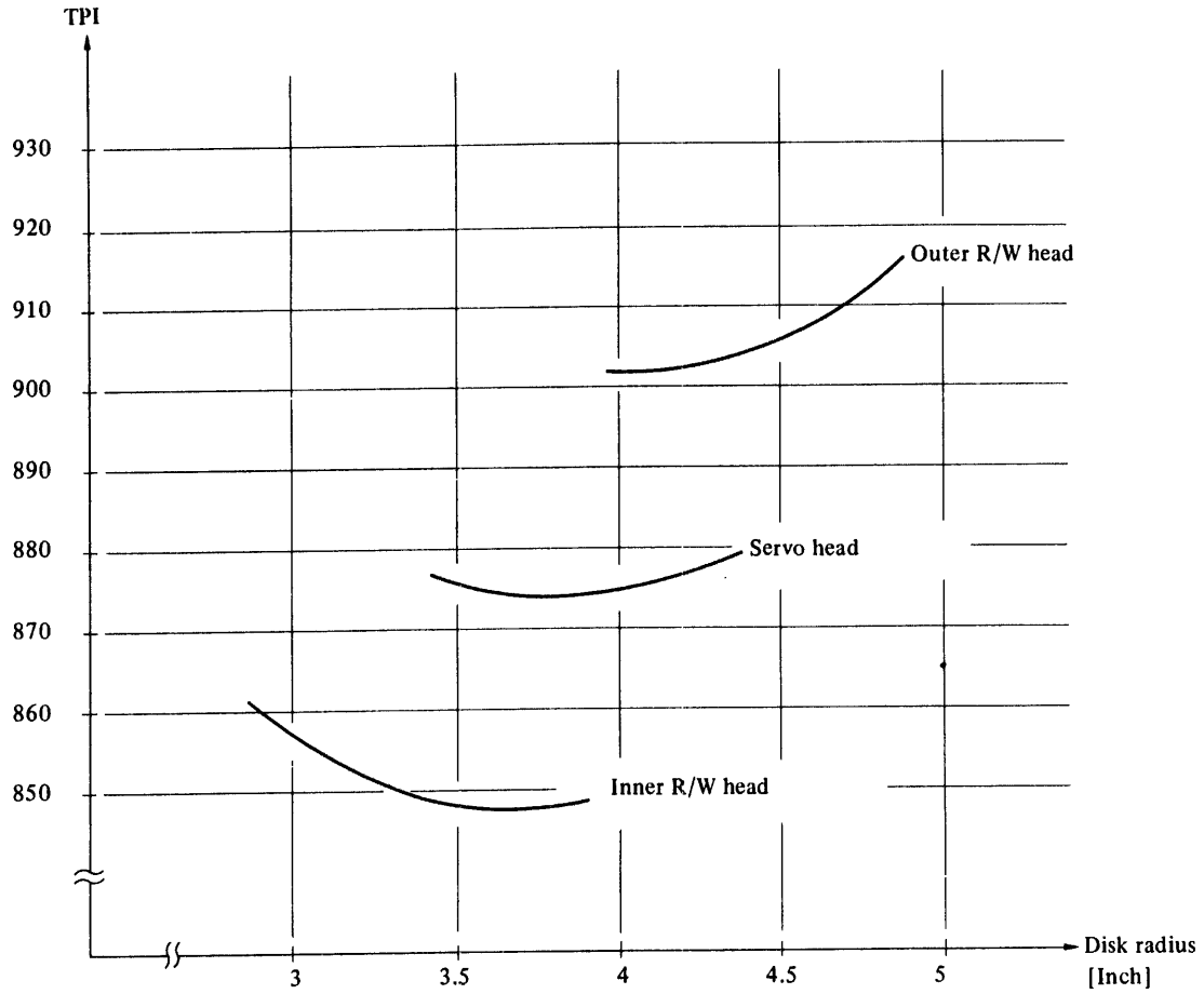
Figure 9.1-2 Track Pitch
