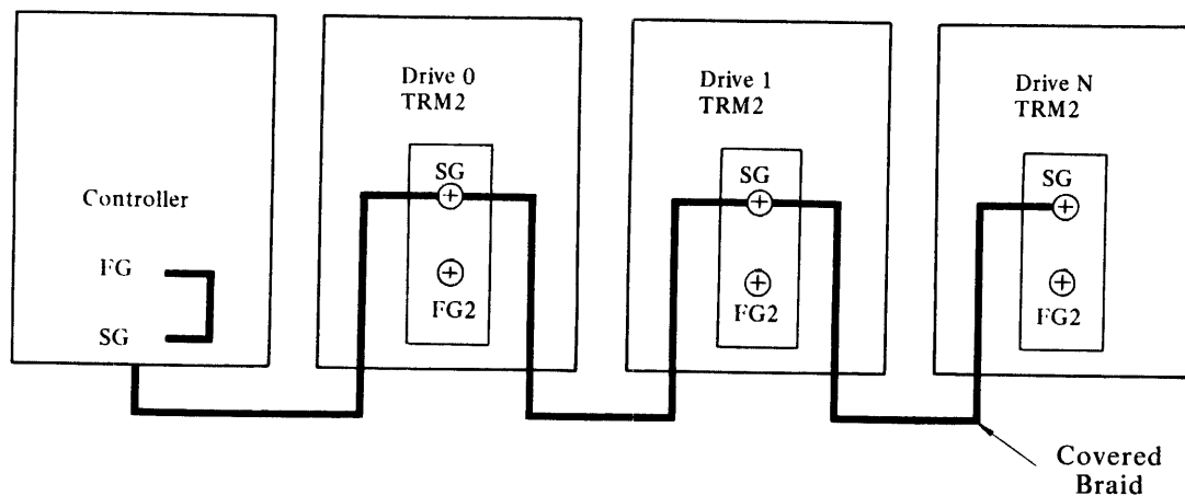
Fig. 4.3-4 SG/FG Isolated
