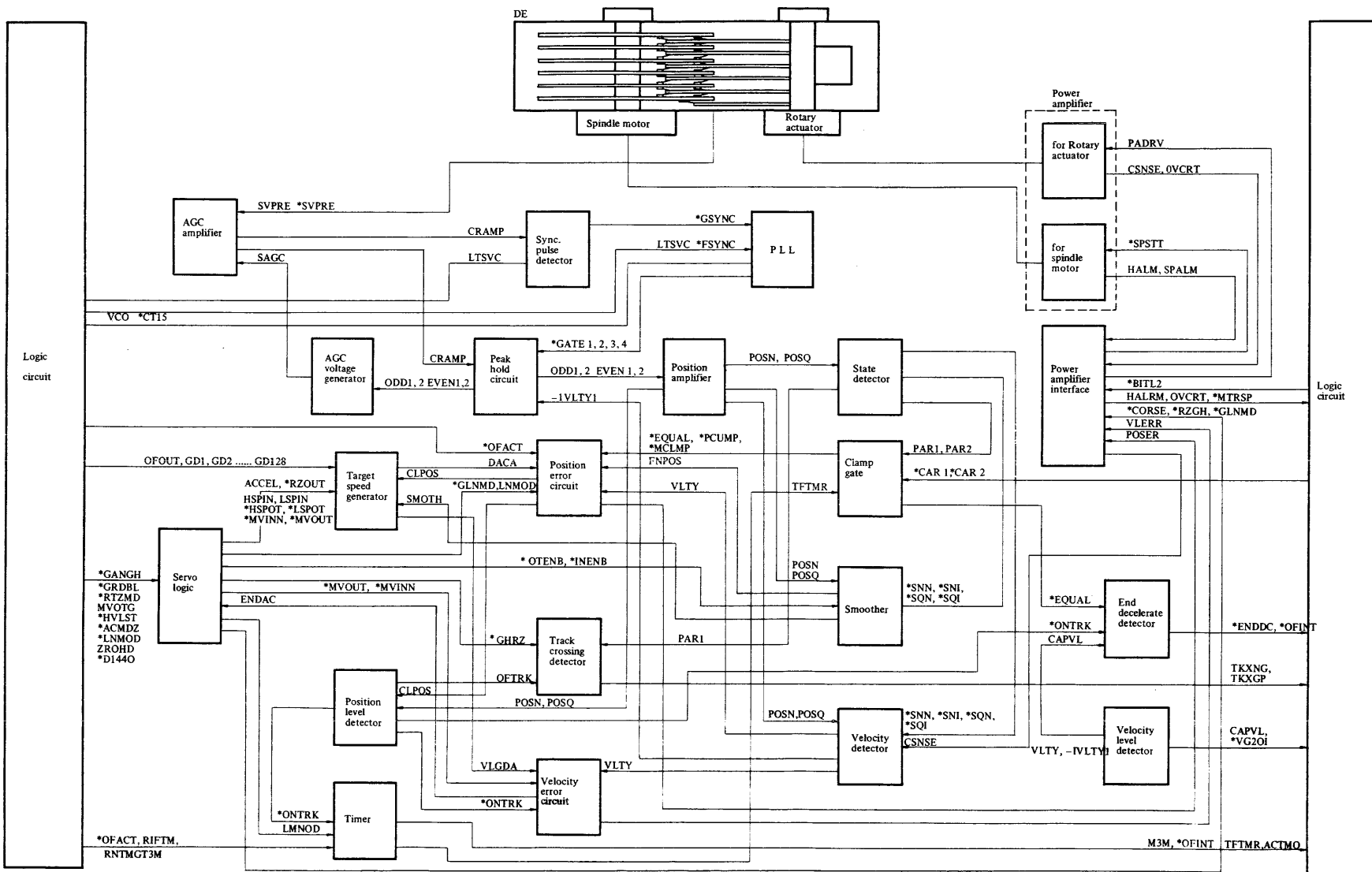
Figure 9.5-1 Servo Block Diagram
