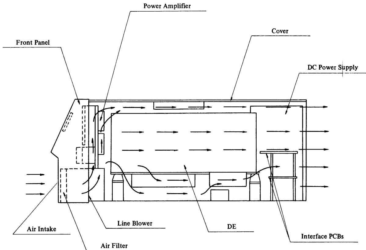
Figure 5.6-2 Air-Flow
