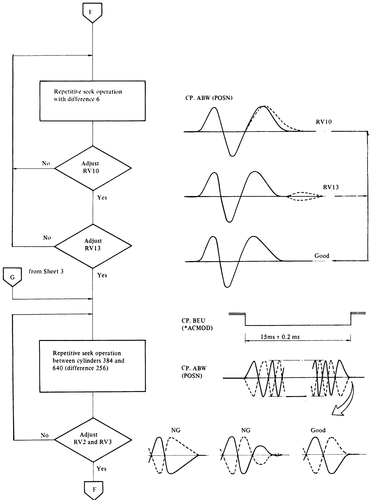
Figure 14.2-4 Dynamic Adjustment of Servo Circuit (Sheet 2 of 3)
