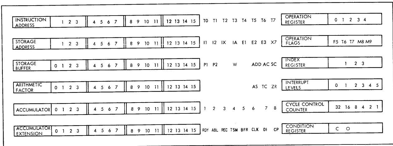
Figure 25. Console Panel
