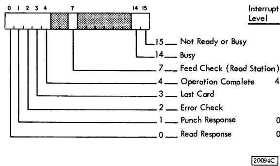
Figure 39. 1442 Device Status Word
