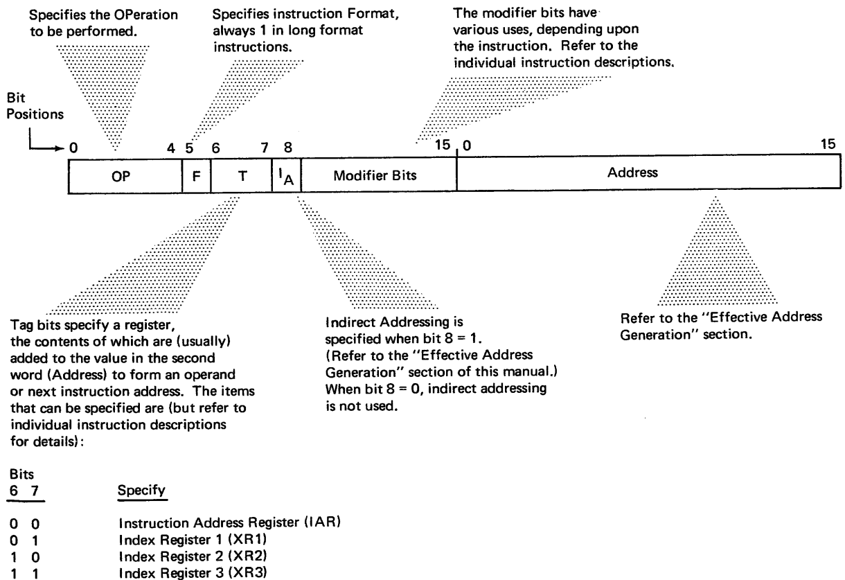
Figure 6. Long-Instruction Format
