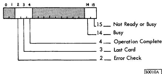
Figure 41. 2501 Device Status Word
