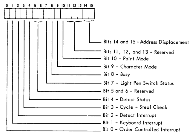
Figure 67. 2250 Device Status Word
