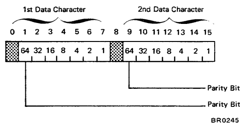
● Figure 51. 1403 Data Format Hexadecimal Bits
