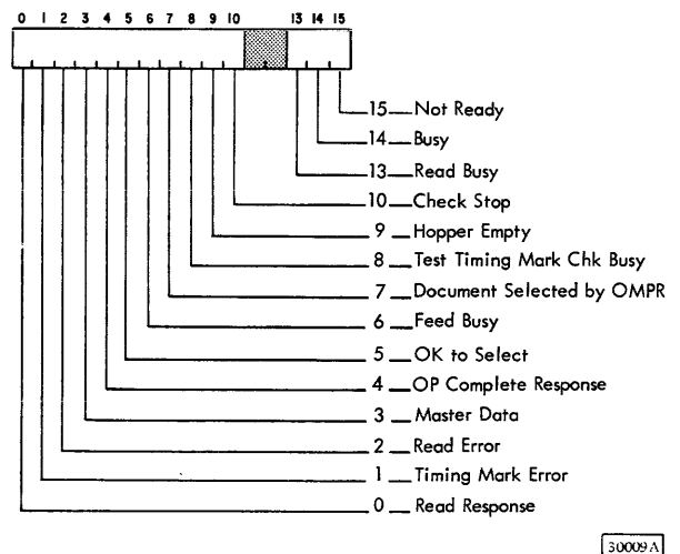
Figure 65. 1231 Device Status Word
