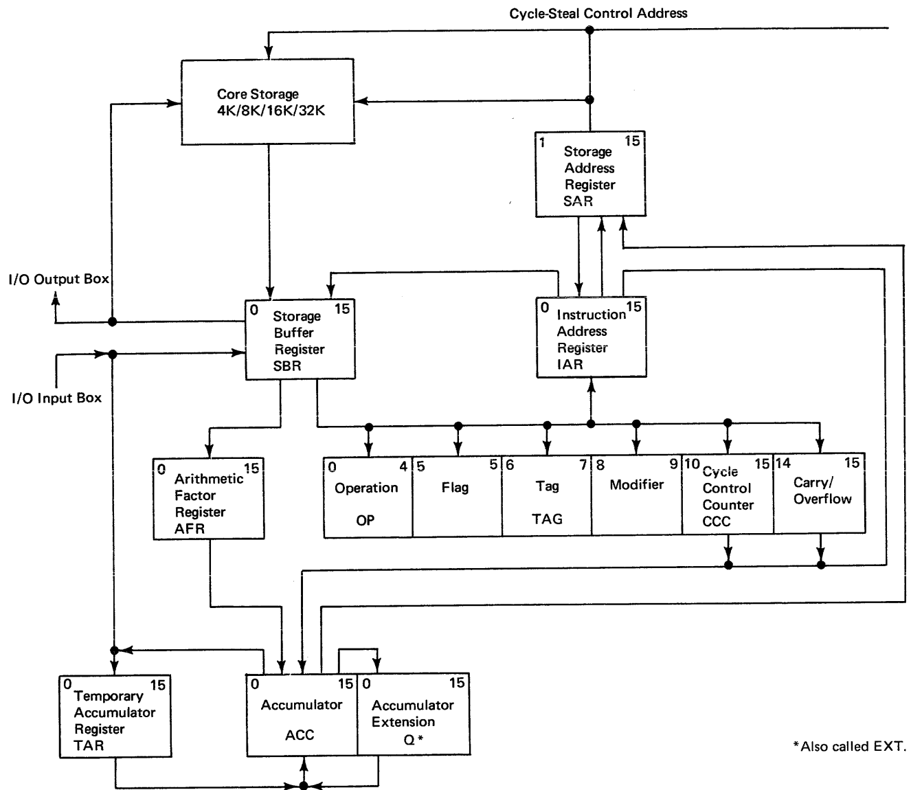
Figure 14. CPU Controls and Data Flow
