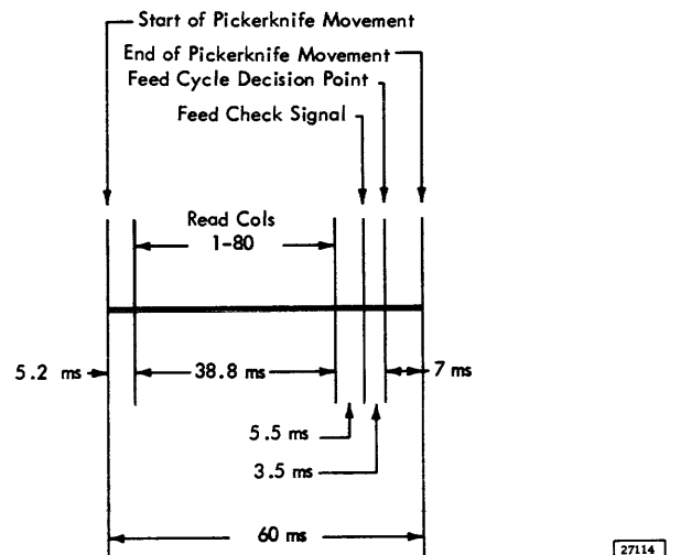
Figure 42. 2501 Timing Schematic
