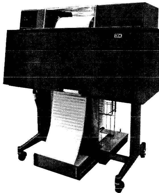
Figure 50. IBM 1403 Printer
