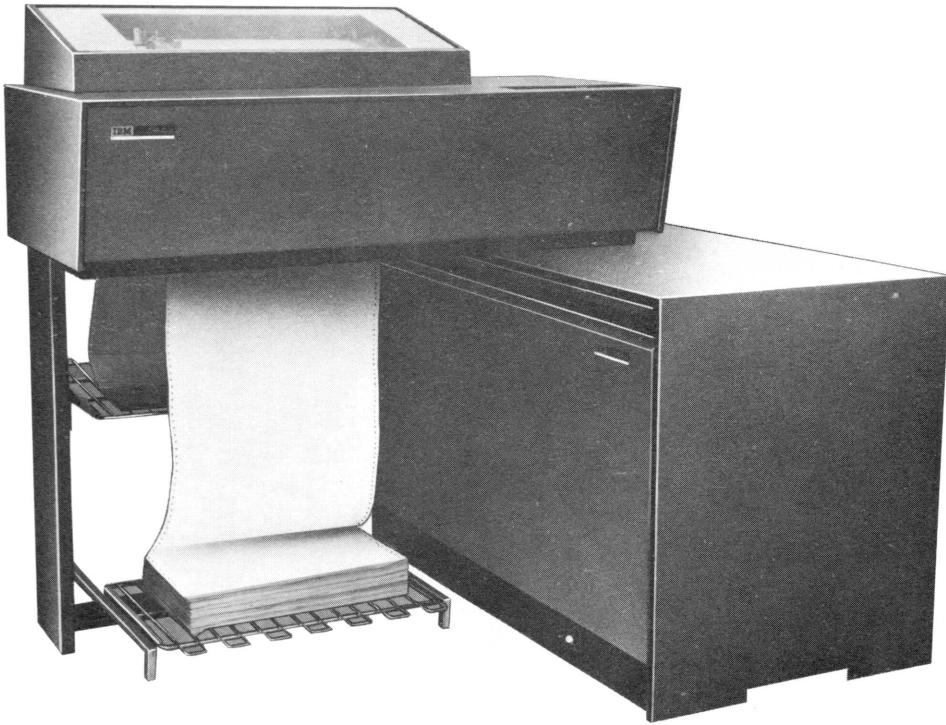
Figure 7. 1443 Printer
