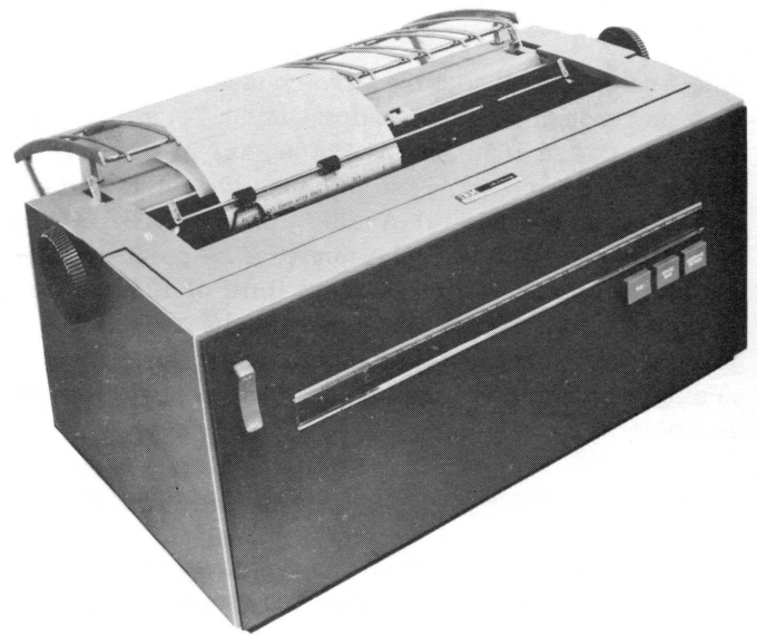
Figure 5. 1053 Printer
