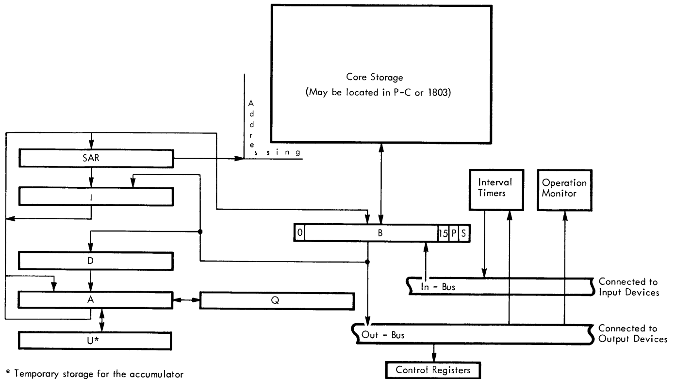
Figure 6. Processor-Controller Data Flow
