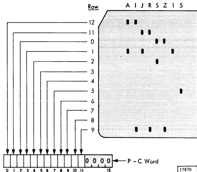
Figure 69. 1442 Card Image Format, Read or Punch
