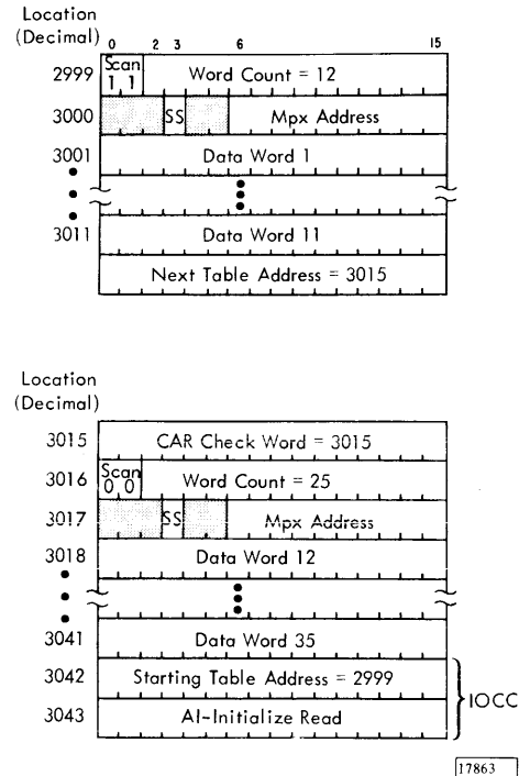
Figure 38. Analog Input Data Tables, Chained Sequential Mode
