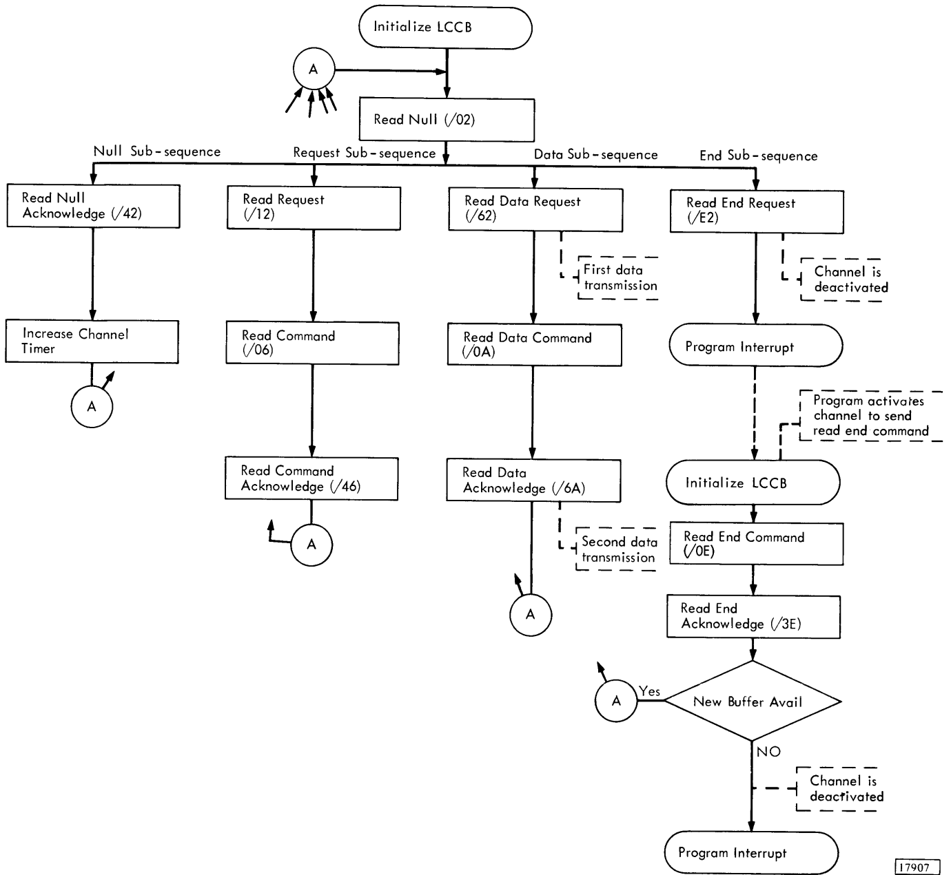
Figure 132. 2790 Adapter Read Sequence
