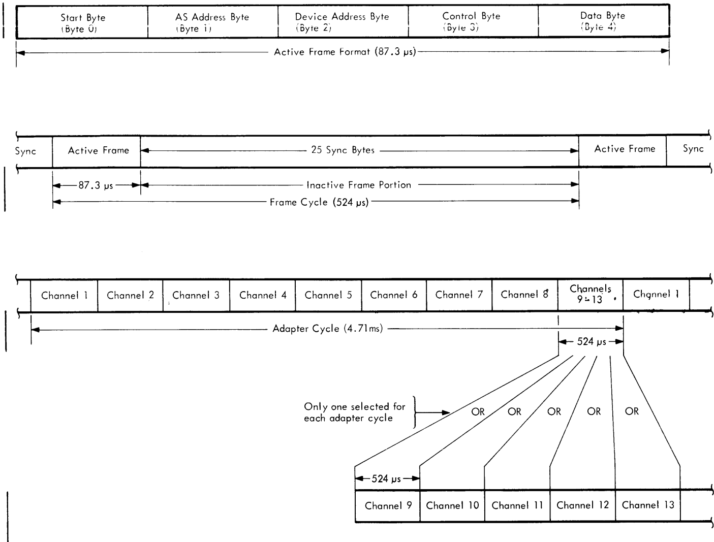
Figure 120. Data Transmission Format
