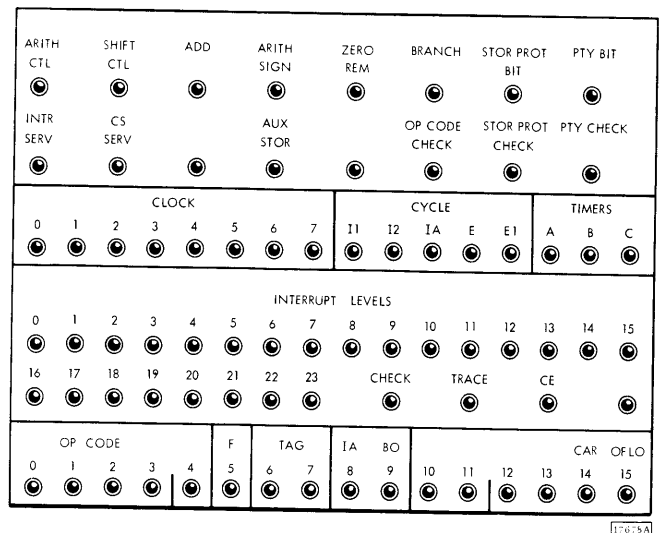
Figure 28. Console Status Indicators
