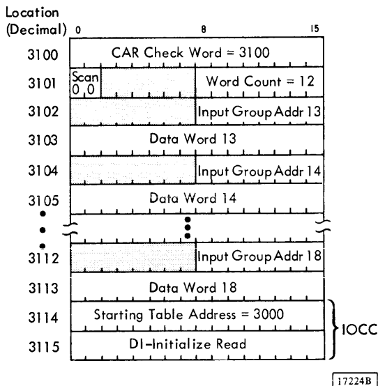
Figure 47. Digital Input Data Tables, Chained Random Mode
