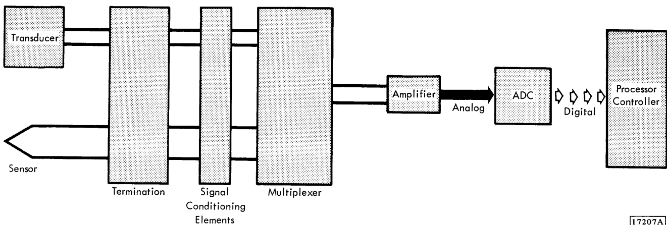
Figure 30. Analog Input Data Path
