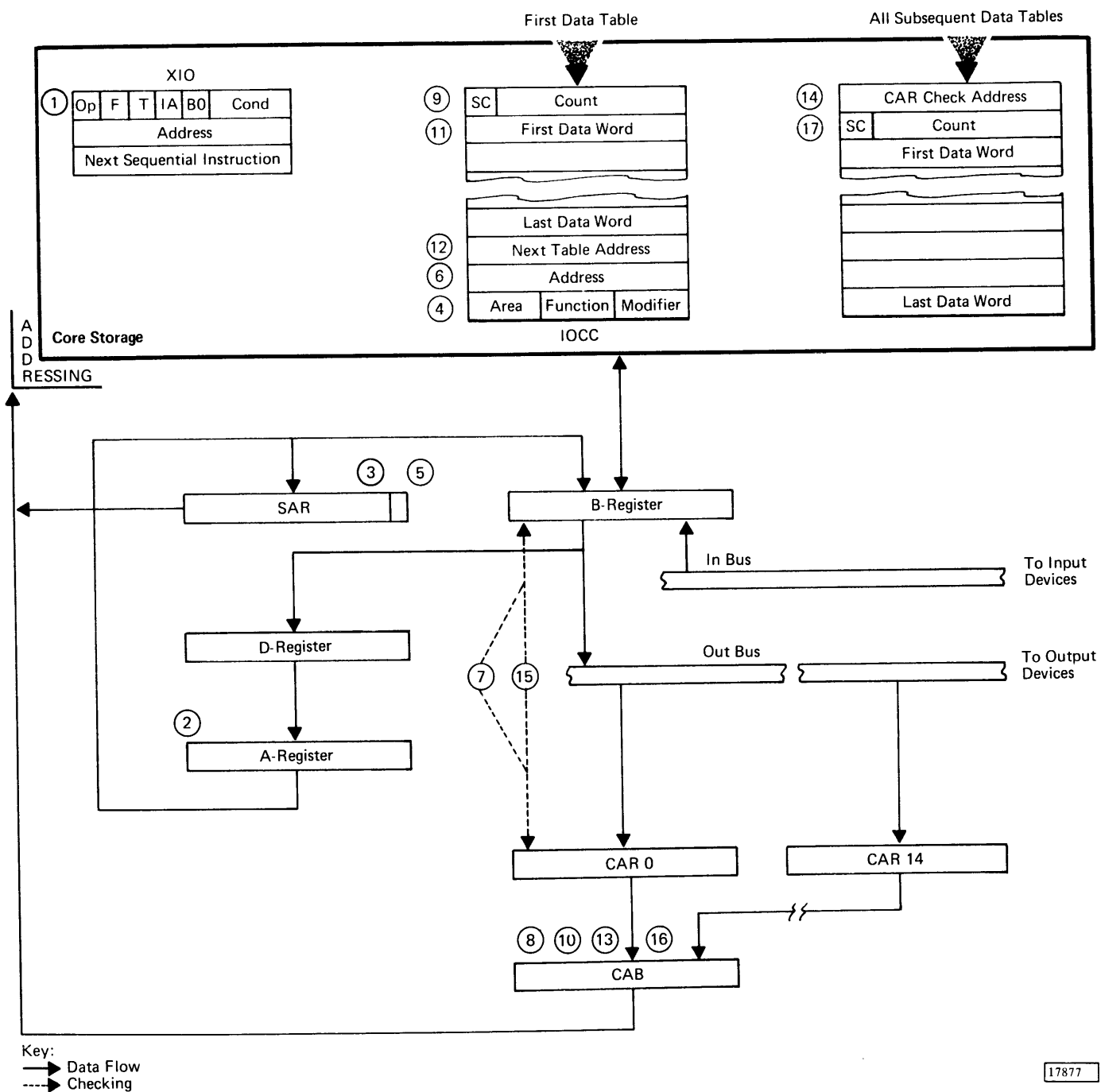
Figure 14. Data Channel Control Operation
