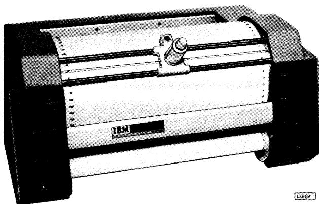
Figure 78. IBM 1627 Plotter
