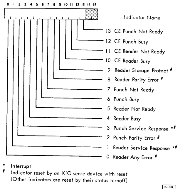
Figure 66. 1054/1055 Device Status Word
