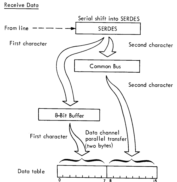
Figure 92. CA Data Flow
