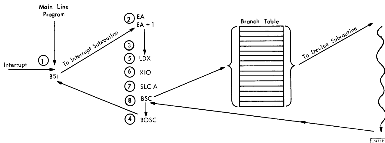
Figure 18. Program Identification of Interrupts
