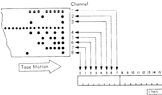
Figure 64. 1054/1055 Word Format
