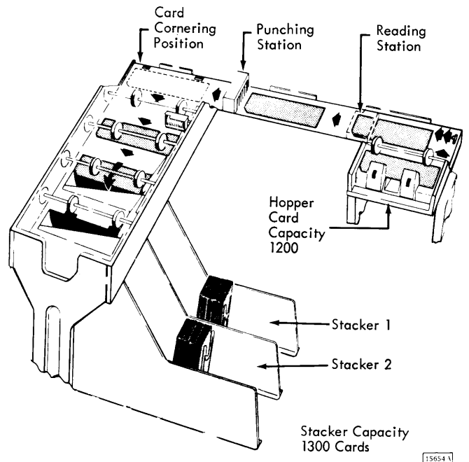
Figure 68. 1442 Card Path
