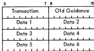
Figure 125. 2790 Adapter Data Buffer Formats
