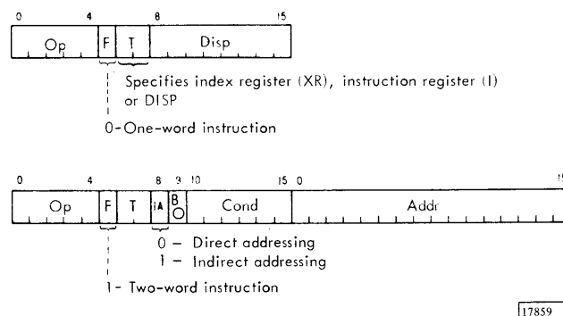
Figure 5. Effective Address Generation
