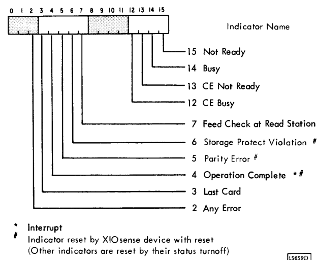
Figure 72. 1442 Device Status Word
