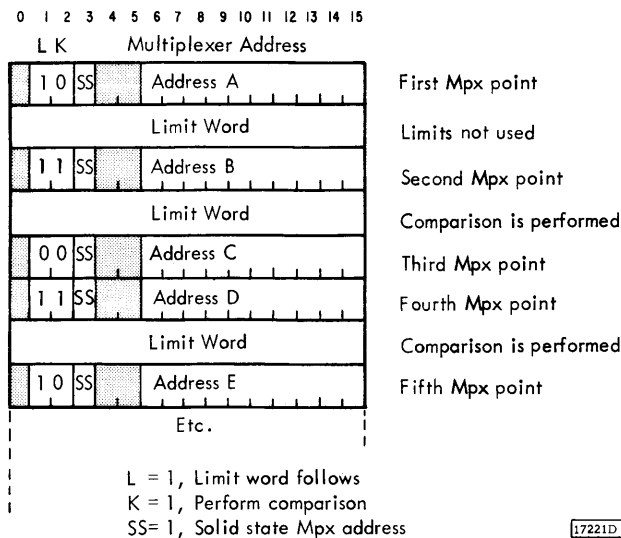
Figure 35. Multiplexer Address Table with Comparator Limit Words
