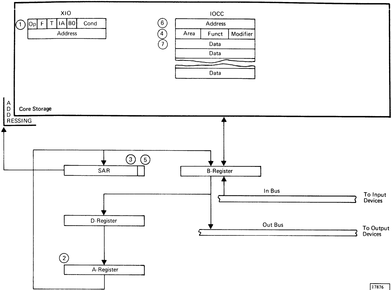
Figure 13. Direct Program Control Operation
