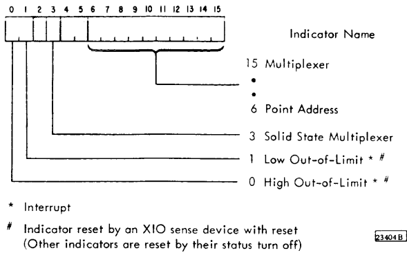
Figure 42. Comparator Device Status Word
