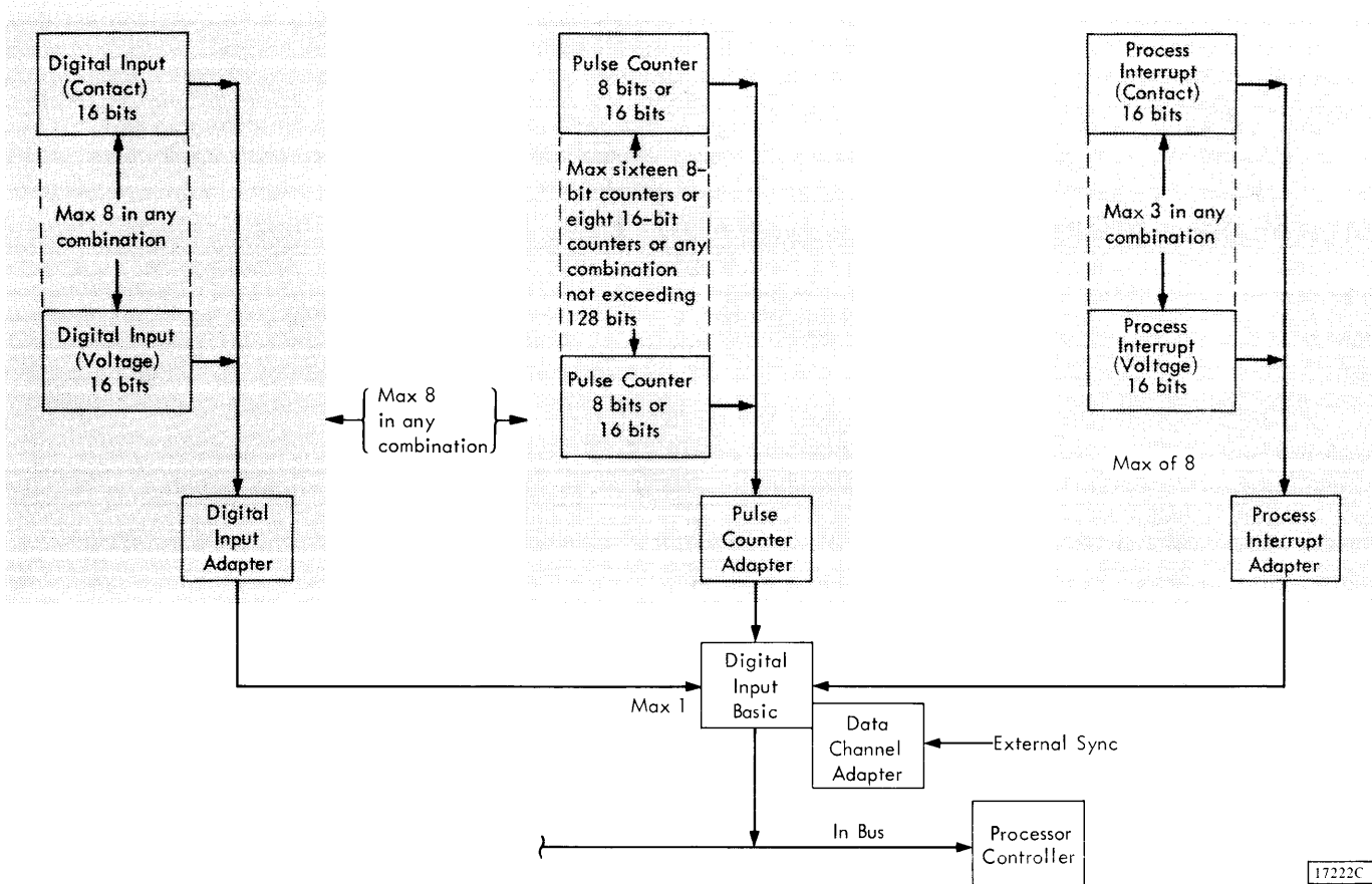
Figure 44. Digital Input Configuration
