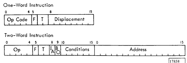
Figure 4. Instruction Formats
